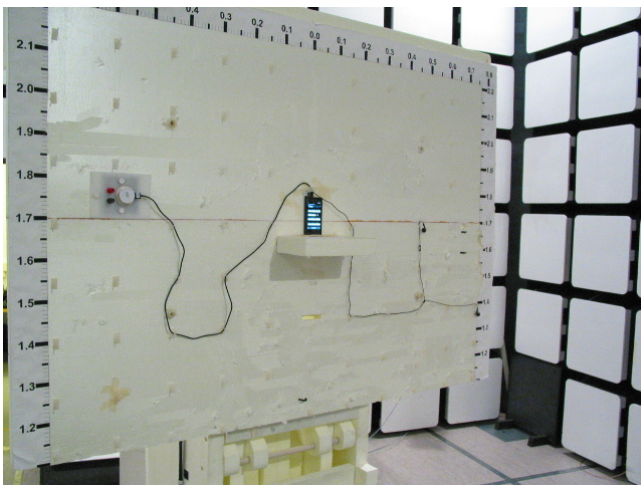
Picture 2. FCC Part 15C Radiated Emissions
