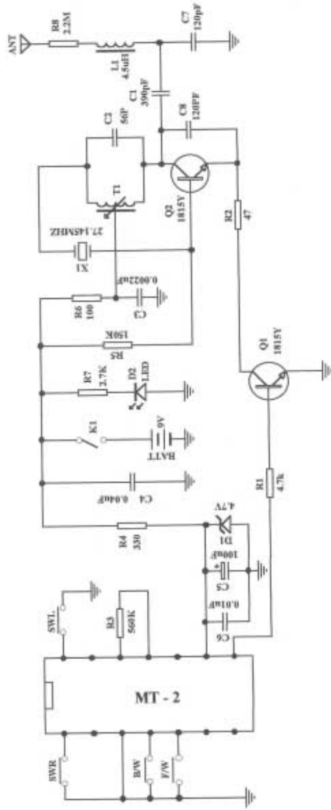
Figure 4.1 System Schematics
