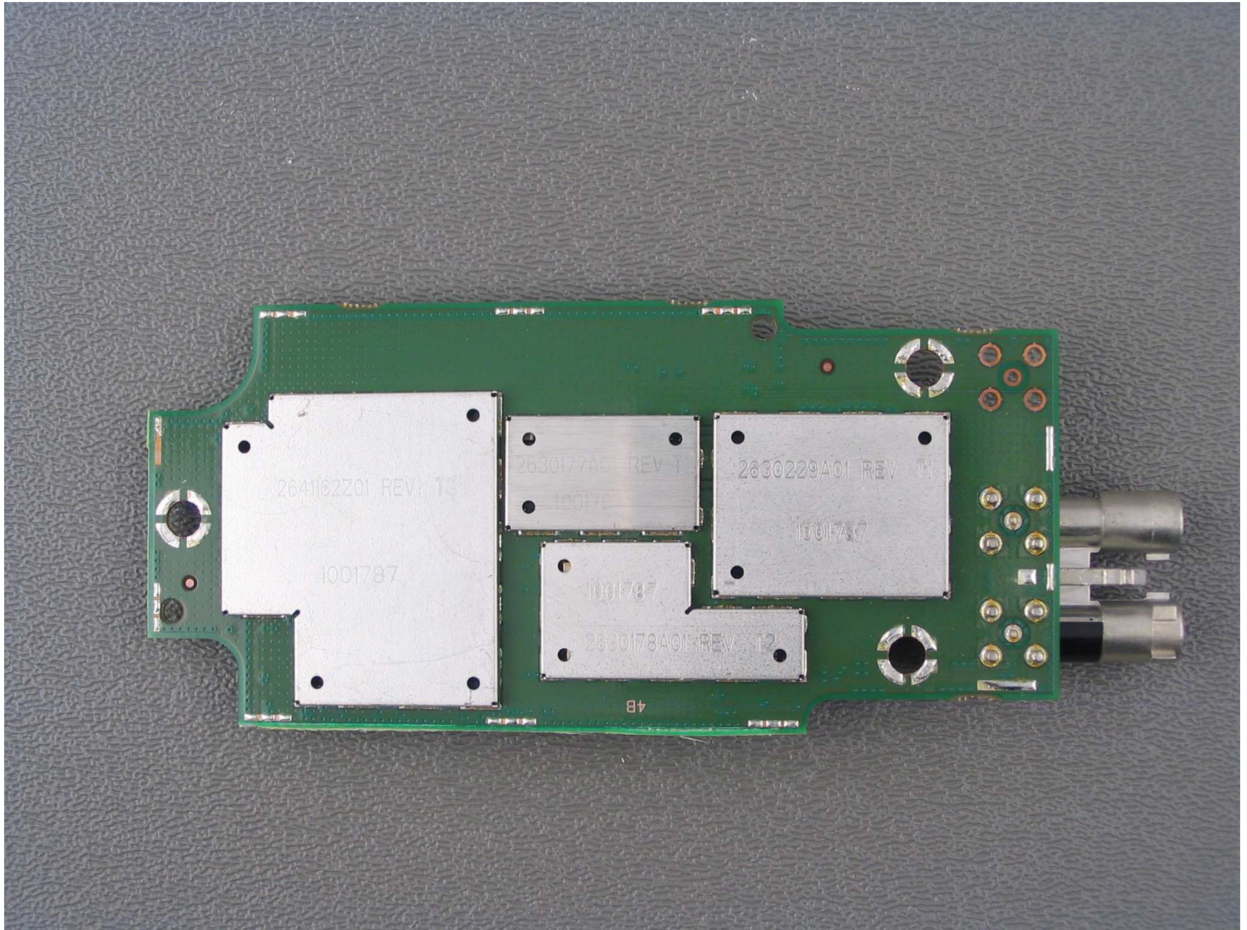
Daughter Board Front Side
