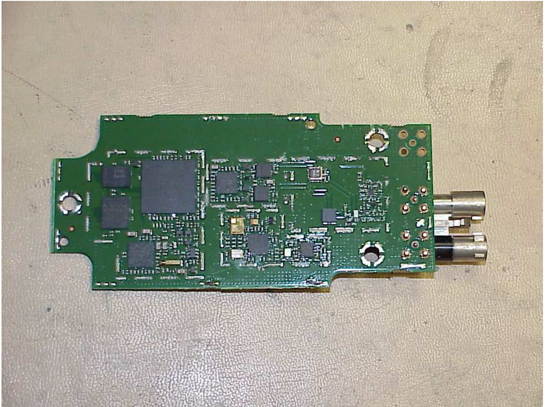
Daughter Board Front Side – Shields Removed
