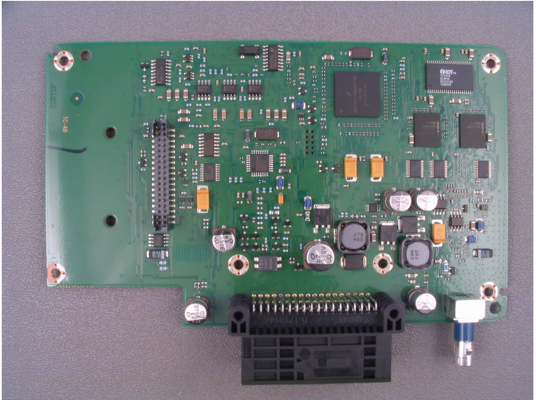
Main Board Front Side
