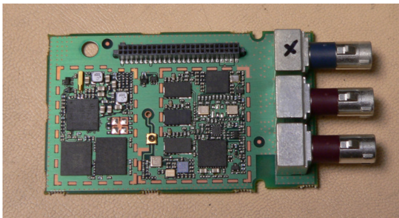
Pic. 2. HNAD – Top side without shields
