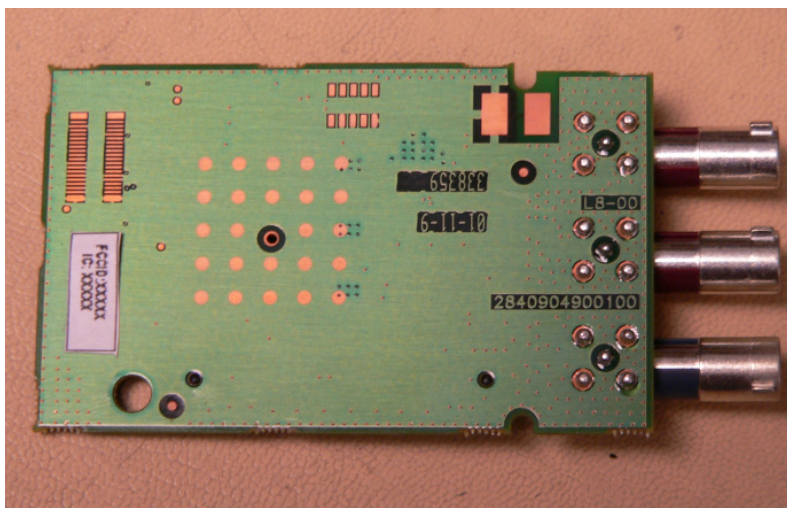
Pic. 3. HNAD – Bottom side.
