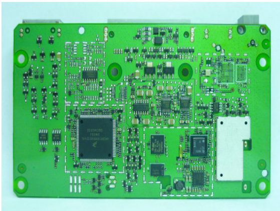
Fig. 3 Internal view: bottom side pcb with shields
