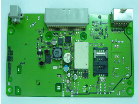
Fig. 1 Internal view: top side pcb with shields
