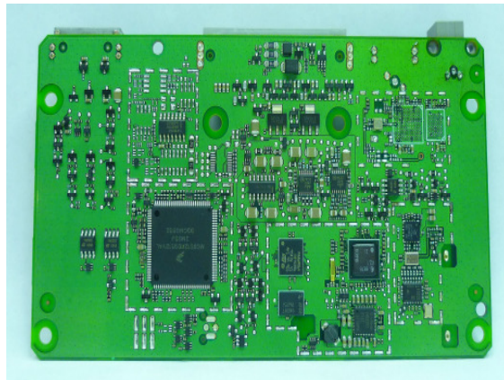
Fig. 4 Internal View: bottom side pcb without shields
