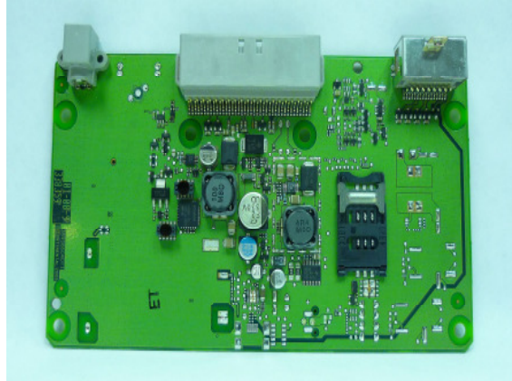
Fig. 2 Internal view: top side pcb without shields
