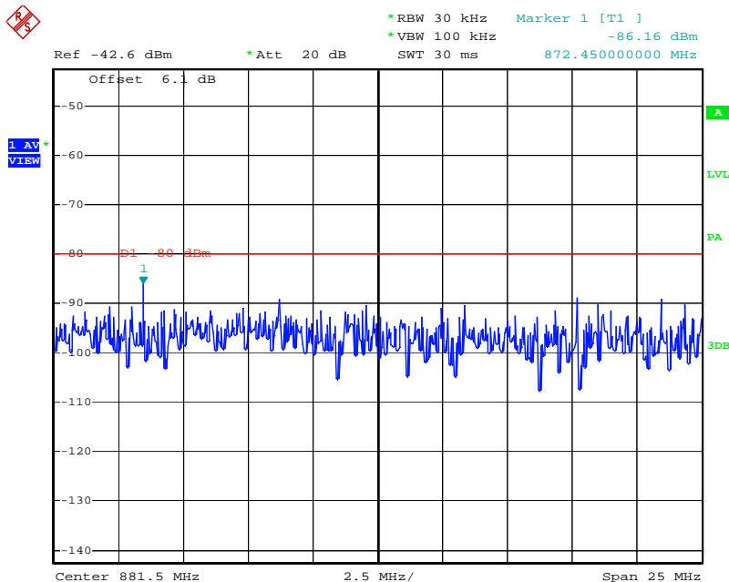
Figure 8-13: Mean Power of Emissions in Base Station Band (AMPS, Voice Mode) – High Channel
