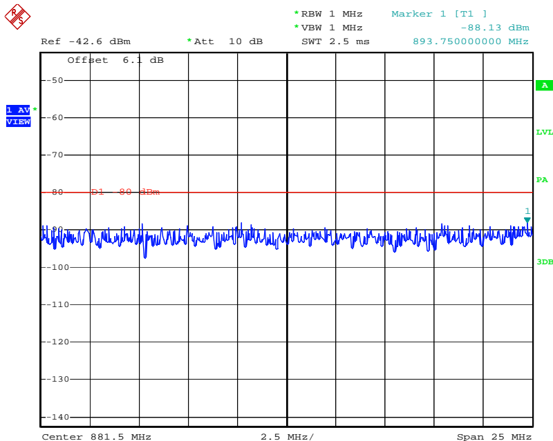
Figure 8-19: Mean Power of Emissions in Base Station Band (CDMA Mode) – High Channel
