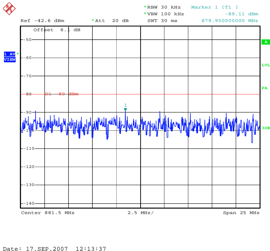
Figure 8-12: Mean Power of Emissions in Base Station Band (AMPS, Voice Mode) – Mid Channel
