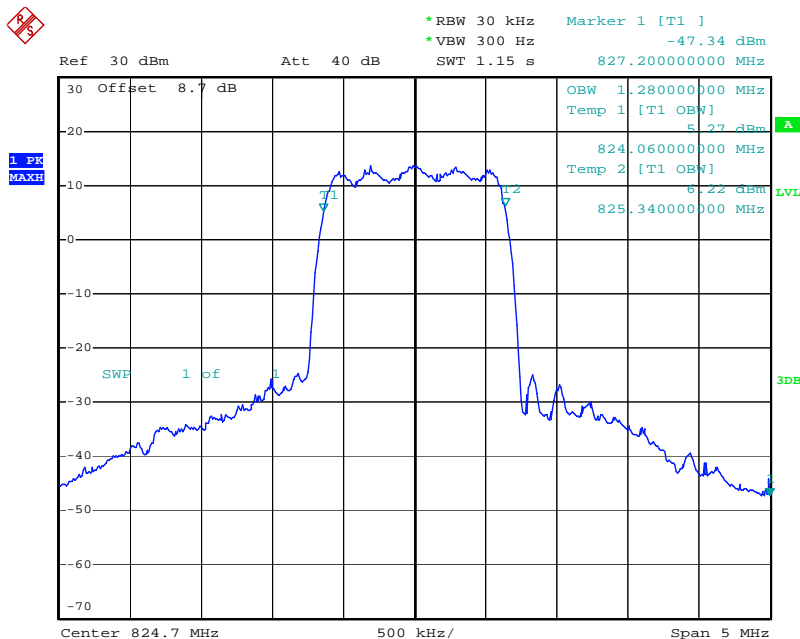
Figure 7-1: Occupied Bandwidth – Cell Channel 1013
