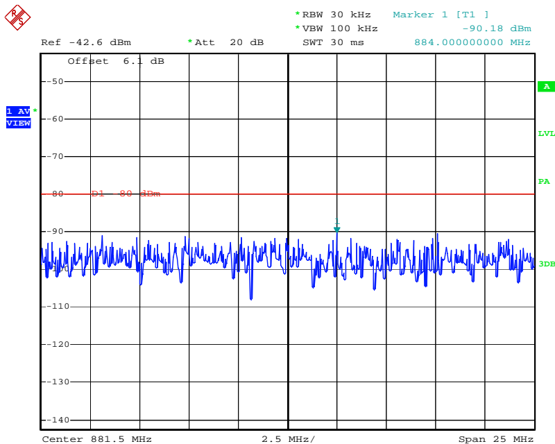
Figure 8-14: Mean Power of Emissions in Base Station Band (AMPS, Wide Band Data Mode) – Low Channel
