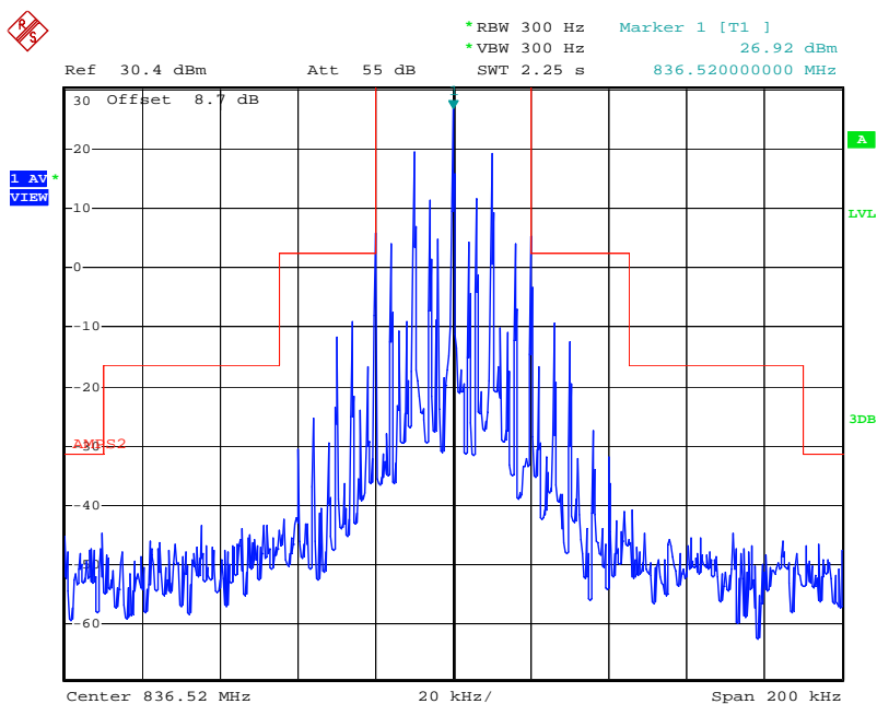
Figure 10-6: Sideband Power Attenuation – SAT & ST
