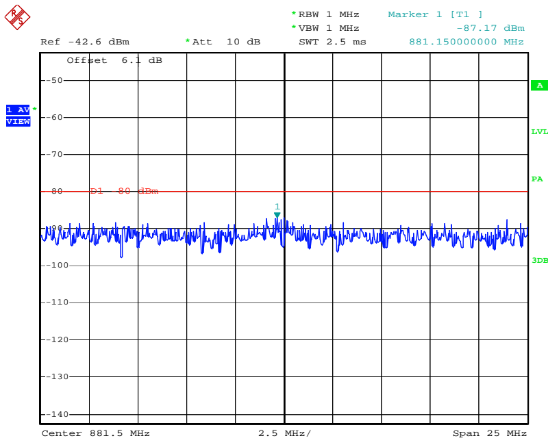
Figure 8-18: Mean Power of Emissions in Base Station Band (CDMA Mode) – Mid Channel
