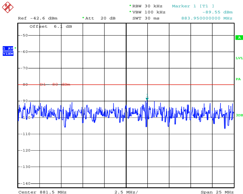
Figure 8-15: Mean Power of Emissions in Base Station Band (AMPS, Wide Band Data Mode) – Mid Channel
