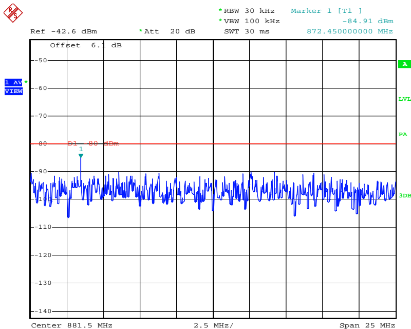
Figure 8-16: Mean Power of Emissions in Base Station Band (AMPS, Wide Band Data Mode) – High Channel
