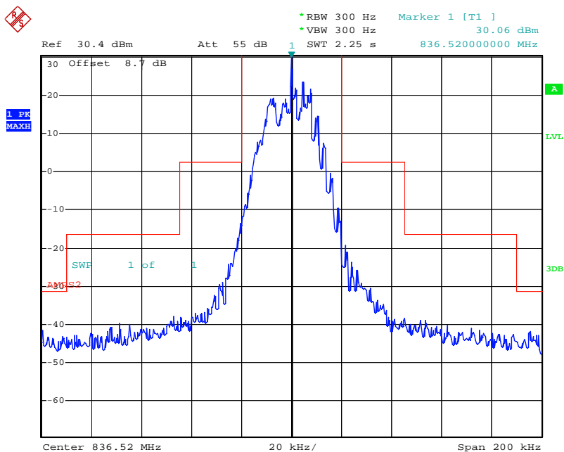
Figure 10-7: Sideband Power Attenuation – Voice & SAT
