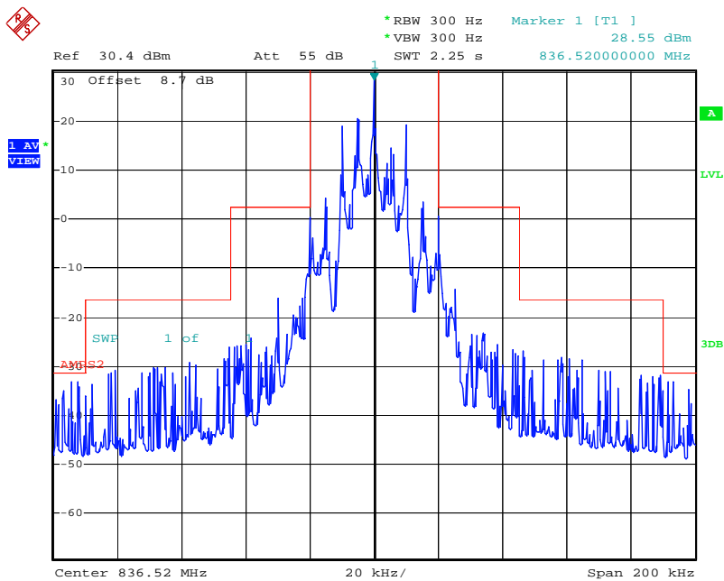
Figure 10-8: Sideband Power Attenuation – Wideband Data
