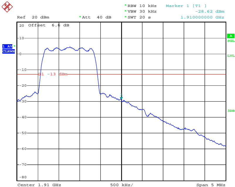
Figure 8-10: Emissions within 1 MHz of band edge, CDMA 1900 Channel 1175
