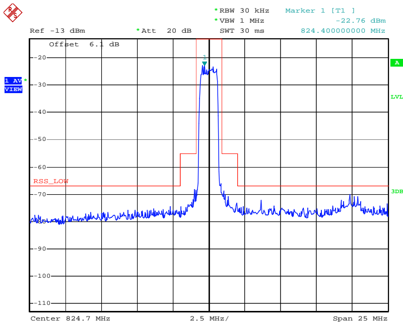
Figure 8-20: Mobile Station Spurious Emissions When Transmitting (CDMA Mode) – Low Channel
