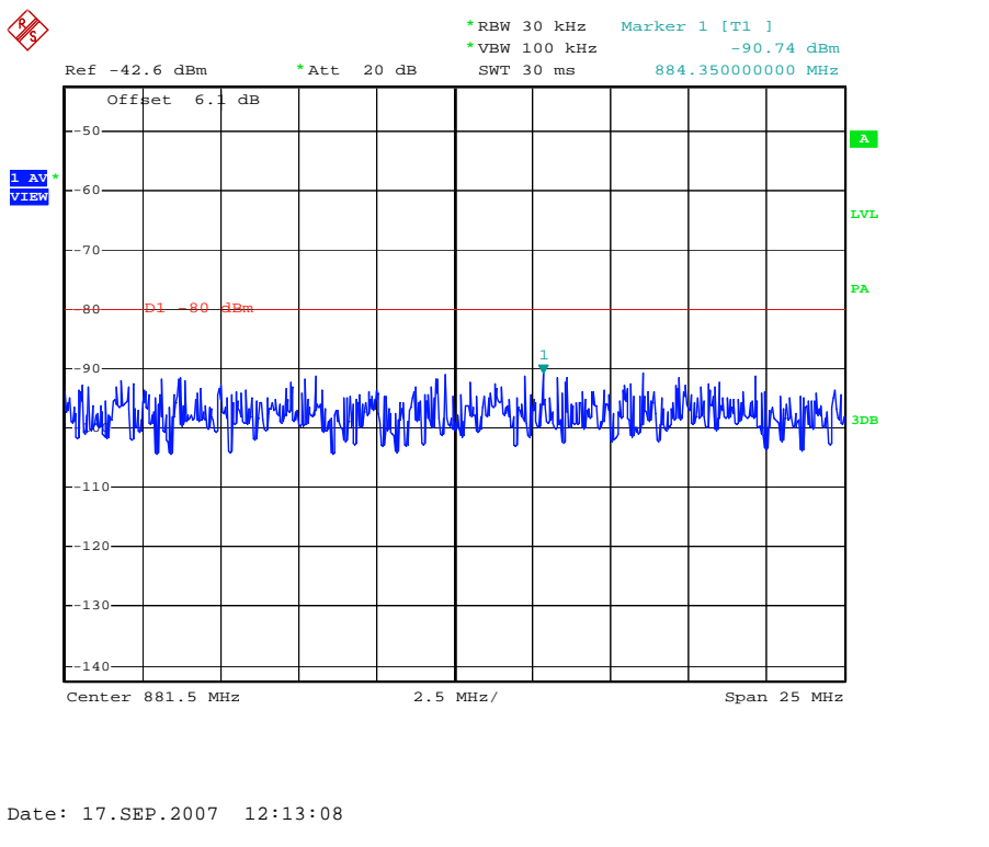
Figure 8-12: Mean Power of Emissions in Base Station Band (AMPS, Voice Mode) – Mid Channel
