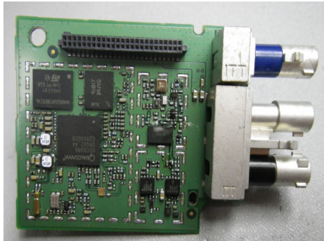
Fig. 2 Internal view: top side pcb without shields
