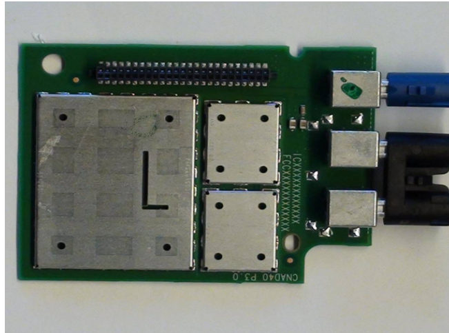
Fig. 1 Internal view: top side pcb with shields
