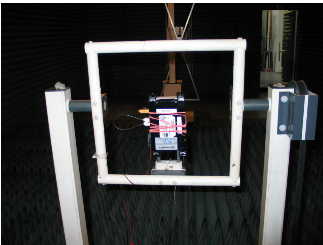
PHOTO No. 3: setup for radiated measurements
