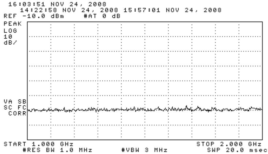
Figure 6.2. Emissions measured at 3 meters in chamber, 1000-2000 MHz.
