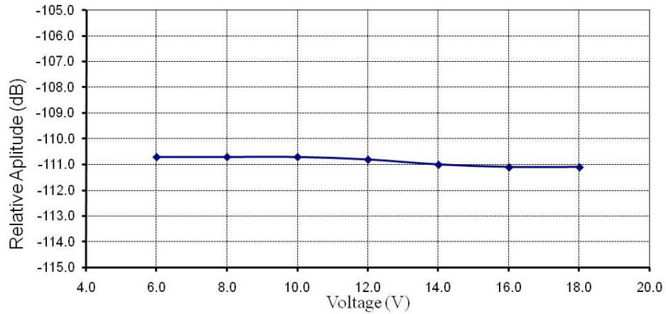
Figure 6.4. Relative emission vs. supply voltage.
