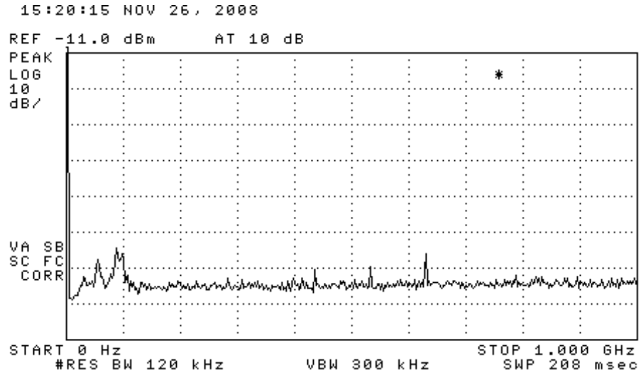
Figure 6.1. Emissions measured at 3 meters in chamber, 0-1000 MHz.
