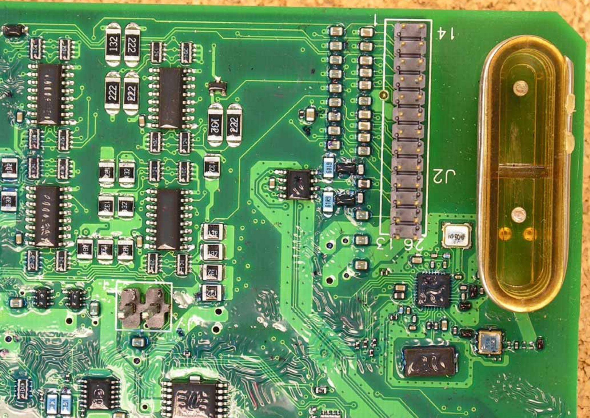
PCB (top)
