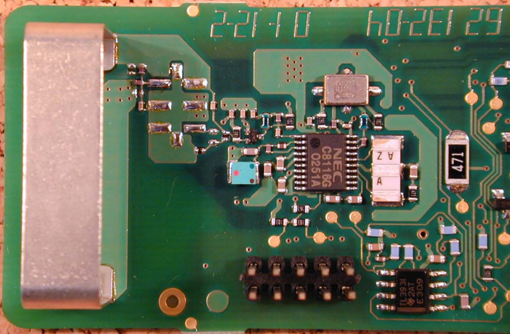
PCB RF Section (top)
