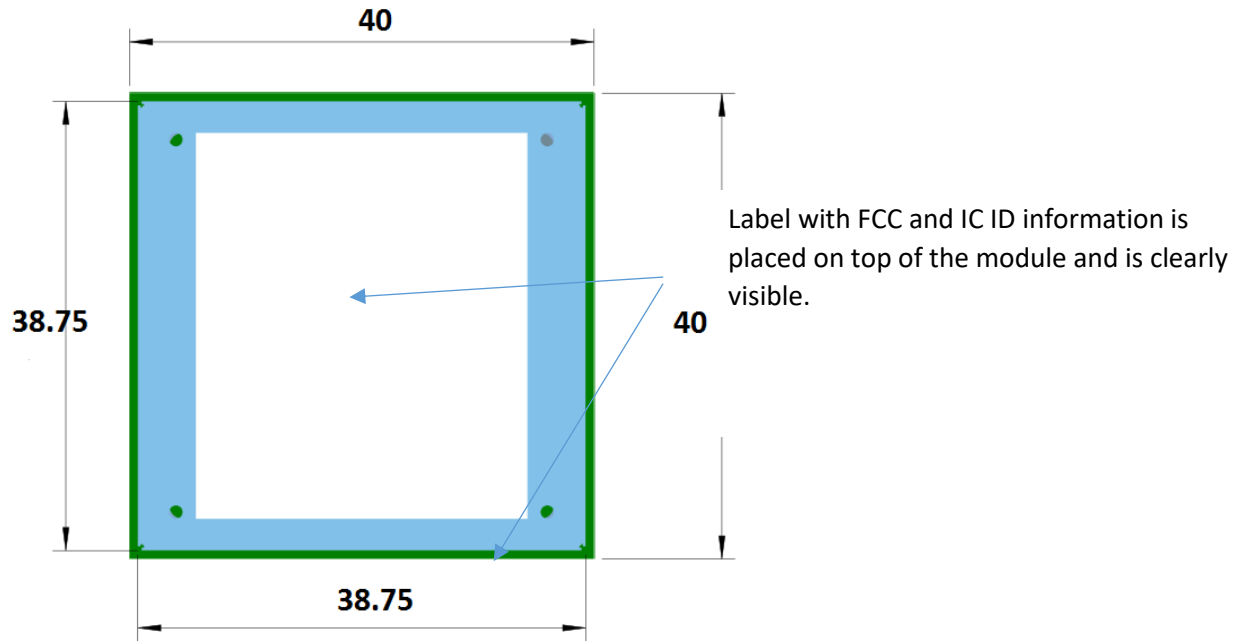
Figure 1: Label placed on top of the module.
