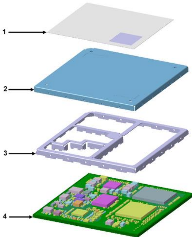
Figure 2: Module Exploded View
