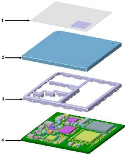
Figure 2] Module Exploded View
