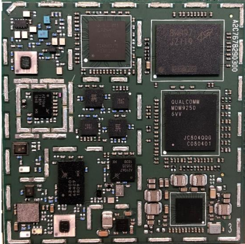
Fig. 3 WT05NA02 module top view without shield frame
