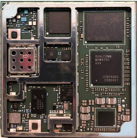
Fig. 2 WT05NA02 module top view without shield cover
