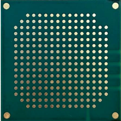
Fig. 2. WT05NA02 module bottom view
