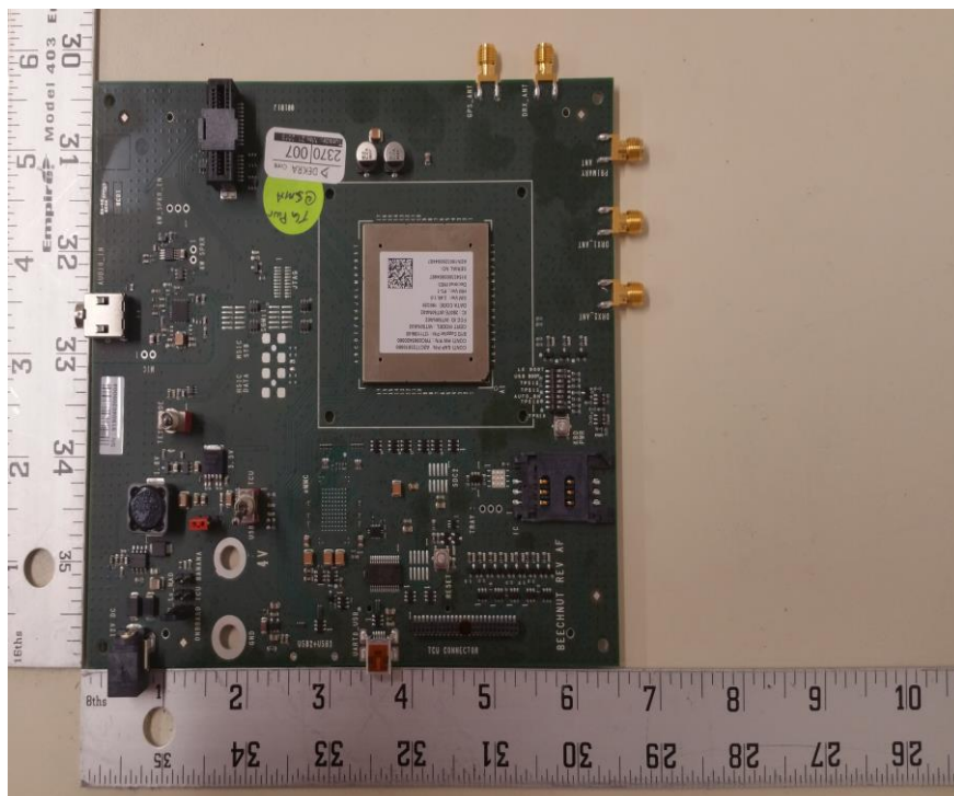
Figure B2. DUT Module only top view
