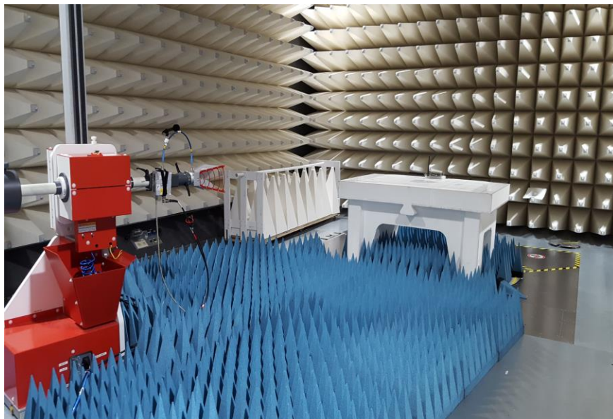
Figure B4. High range Radiated emission Set up Horn antenna
