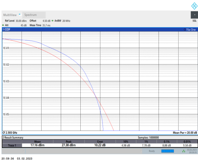
Band41-20MHz-QPSK-40620-100RB#0
