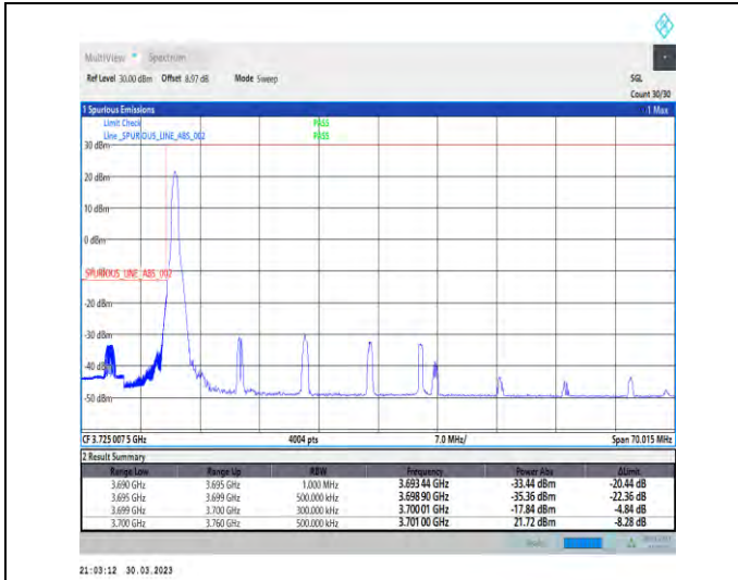
1-N77-3700-3980-30-60-L-1-DFT-PI2BPSK-Edge_1RB_Left-1@0-Ant1-1--PASS-see graph
