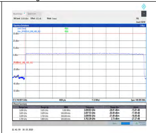
1-N77-3700-3980-30-100-L-3-DFT-PI2BPSK-Outer_Full-270@0-Ant1-1--PASS-see graph
