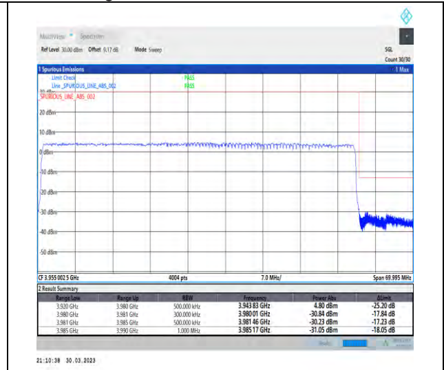
1-N77-3700-3980-30-60-H-3-DFT-PI2BPSK-Outer_Full-162@0-Ant1-1--PASS-see graph
