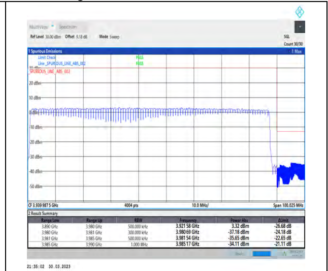
1-N77-3700-3980-30-90-H-3-DFT-PI2BPSK-Outer_Full-240@0-Ant1-1--PASS-see graph
