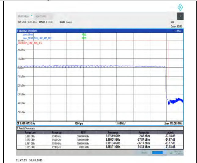
1-N77-3700-3980-30-100-H-3-DFT-PI2BPSK-Outer_Full-270@0-Ant1-1--PASS-see graph
