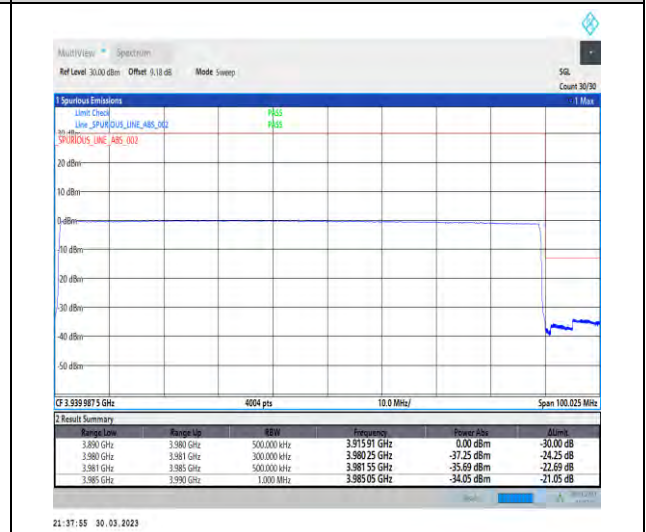
1-N77-3700-3980-30-90-H-6-CP-QPSK-Outer_Full-245@0-Ant1-1--PASS-see graph
