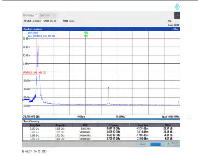
1-N77-3700-3980-30-100-L-4-CP-QPSK-Edge_1RB_Left-1@0-Ant1-1--PASS-see graph
