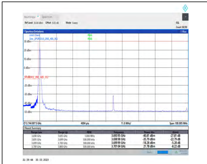
1-N77-3700-3980-30-100-L-1-DFT-PI2BPSK-Edge_1R_B_Left-1@0-Ant1-1--PASS-see graph
