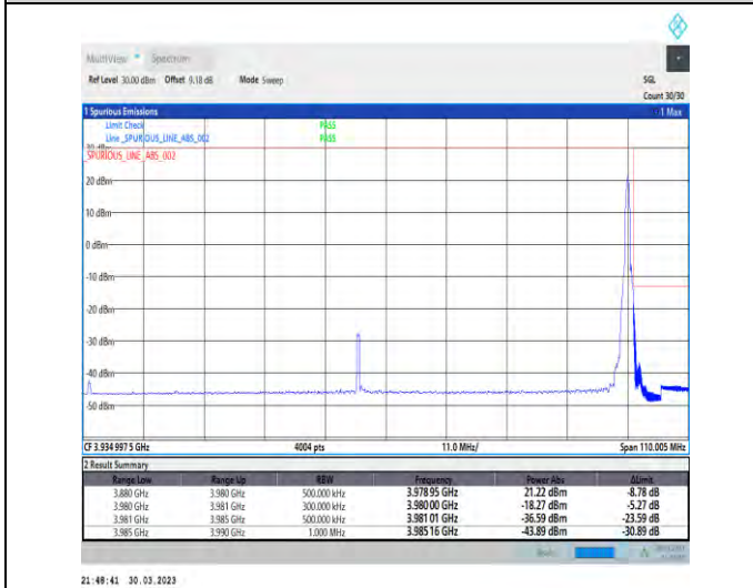
1-N77-3700-3980-30-100-H-5-CP-QPSK-Edge_1RB_Right-1@272-Ant1-1--PASS-see graph
