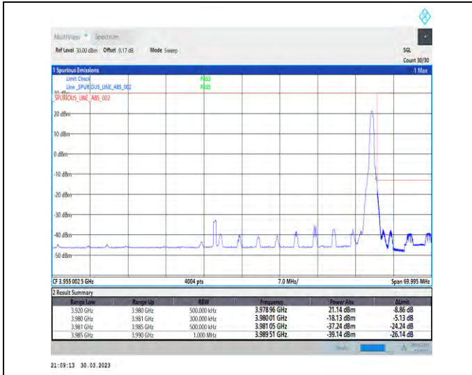
1-N77-3700-3980-30-60-H-2-DFT-PI2BPSK-Edge_1R_B_Right-1@161-Ant1-1--PASS-see graph
