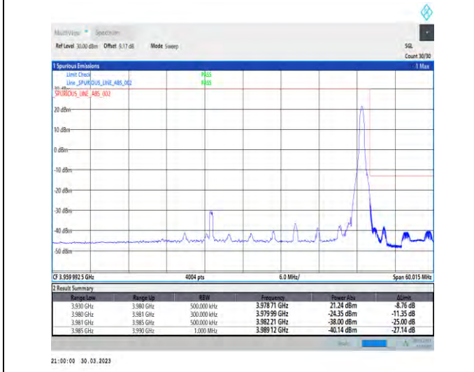
1-N77-3700-3980-30-50-H-5-CP-QPSK-Edge_1RB_Right-1@132-Ant1-1--PASS-see graph
