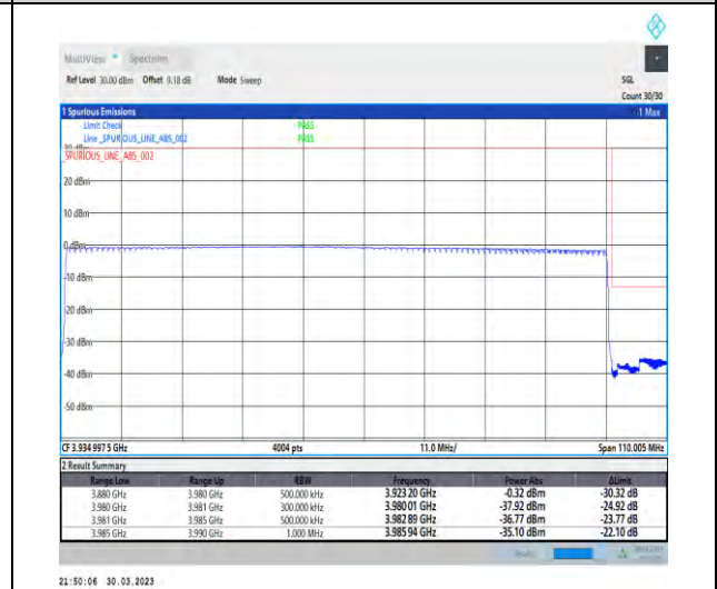
1-N77-3700-3980-30-100-H-6-CP-QPSK-Outer_Full-273@0-Ant1-1--PASS-see graph
