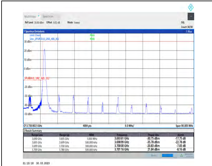
1-N77-3700-3980-30-80-L-1-DFT-PI2BPSK-Edge_1RB_Left-1@0-Ant1-1--PASS-see graph
