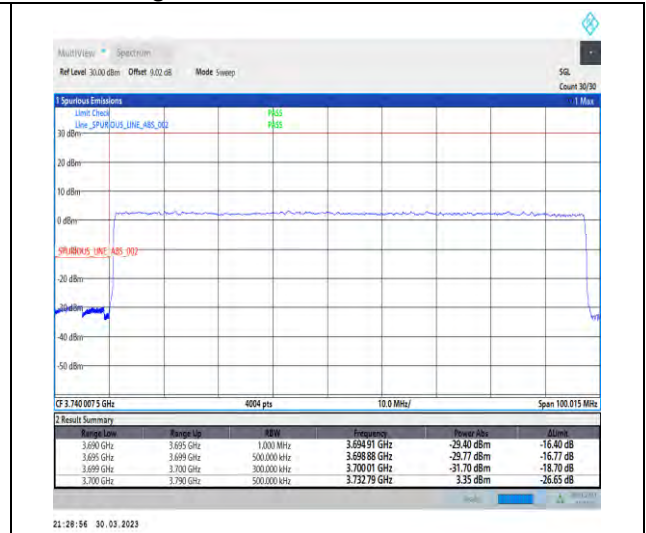
1-N77-3700-3980-30-90-L-3-DFT-PI2BPSK-Outer _Full-240@0-Ant1-1--PASS-see graph
