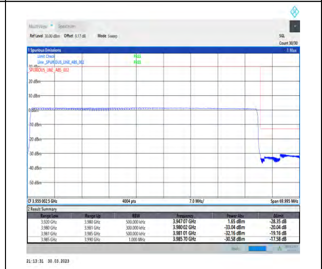
1-N77-3700-3980-30-60-H-6-CP-QPSK-Outer_Full-162@0-Ant1-1--PASS-see graph
