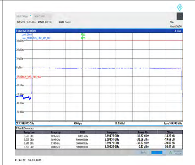
1-N77-3700-3980-30-100-L-6-CP-QPSK-Outer_Full-273@0-Ant1-1--PASS-see graph
