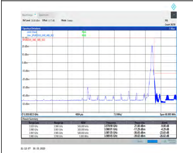
1-N77-3700-3980-30-60-H-5-CP-QPSK-Edge_1RB_Right-1@161-Ant1-1--PASS-see graph
