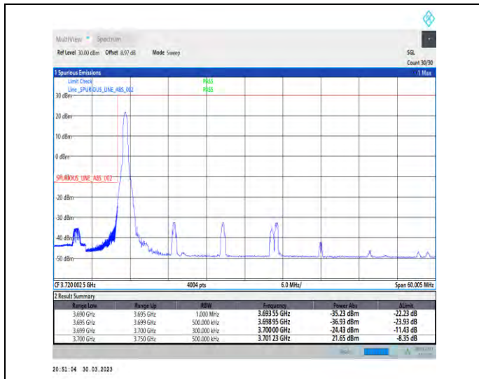
1-N77-3700-3980-30-50-L-1-DFT-PI2BPSK-Edge_1RB_Left-1@0-Ant1-1--PASS-see graph
