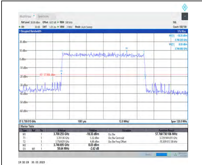
1-N77-3700-3980-30-60-L-9-CP-256QAM-Outer_Ful I-162@0-Ant1-57.769-59.640-≤60-PASS
