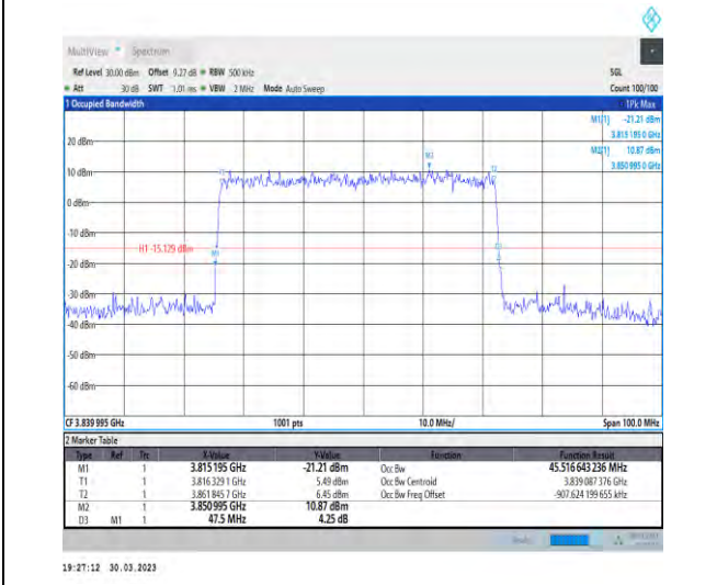
1-N77-3700-3980-30-50-M-5-DFT-256QAM-Outer_F ull-128@0-Ant1-45.517-47.500-≤50-PASS
