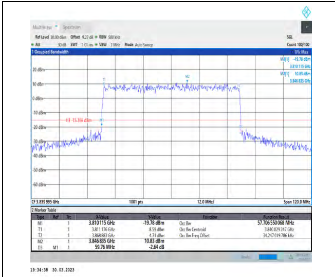
1-N77-3700-3980-30-60-M-8-CP-64QAM-Outer_Full -162@0-Ant1-57.707-59.760-≤60-PASS
