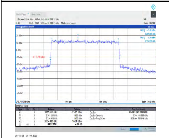
1-N77-3700-3980-30-90-L-1-DFT-QPSK-Outer_Full-240@0-Ant1-85.684-88.920-<=90-PASS
