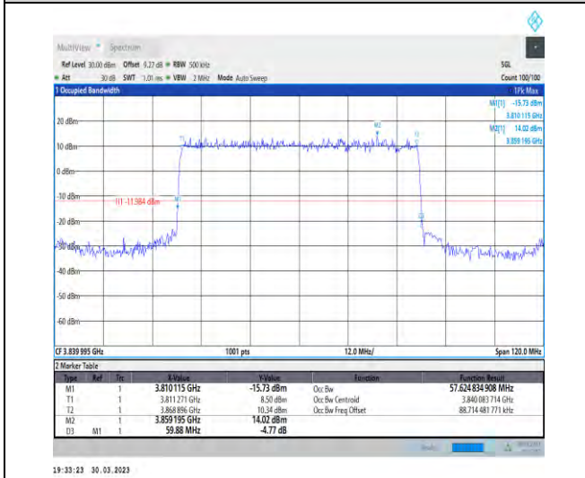
1-N77-3700-3980-30-60-M-2-DFT-PI2BPSK-Outer_Ful Full-162@0-Ant1-57.625-59.880-≤60-PASS
