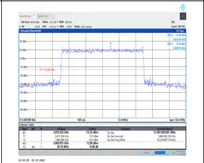
1-N77-3700-3980-30-60-M-3-DFT-16QAM-Outer_Ful I-162@0-Ant1-57.902-59.760-≤60-PASS
