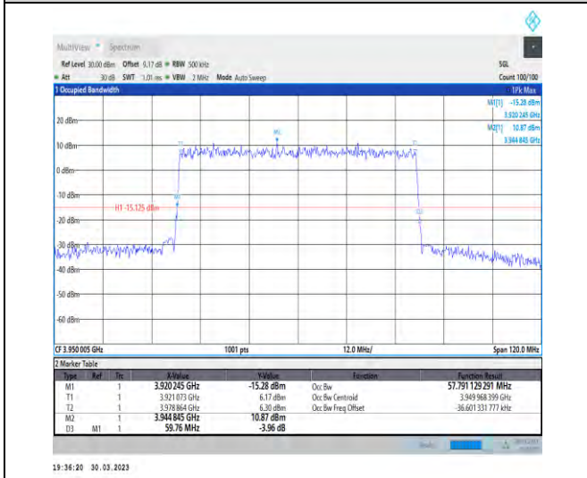
1-N77-3700-3980-30-60-H-5-DFT-256QAM-Outer_Full ull-162@0-Ant1-57.791-59.760-≤60-PASS
