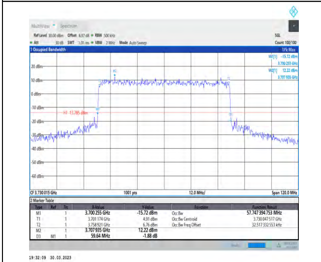
1-N77-3700-3980-30-60-L-7-CP-16QAM-Outer_Full-162@0-Ant1-57.747-59.640-≤60-PASS
