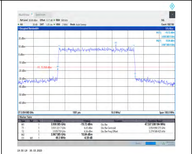
1-N77-3700-3980-30-50-H-9-CP-256QAM-Outer_Full-133@0-Ant1-47.537-49.300-≤50-PASS
