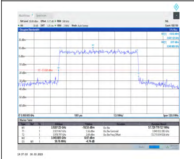
1-N77-3700-3980-30-60-H-9-CP-256QAM-Outer_Ful-162@0-Ant1-57.73-59.760-≤60-PASS
