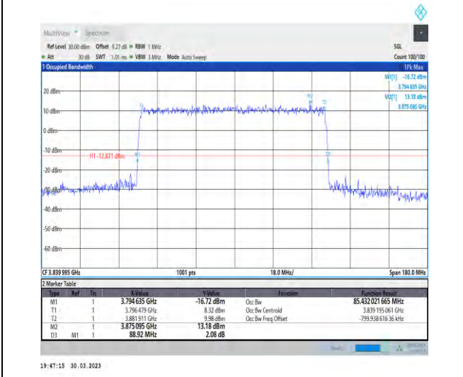
1-N77-3700-3980-30-90-M-4-DFT-64QAM-Outer_Full-240@0-Ant1-85.432-88.920-≤90-PASS
