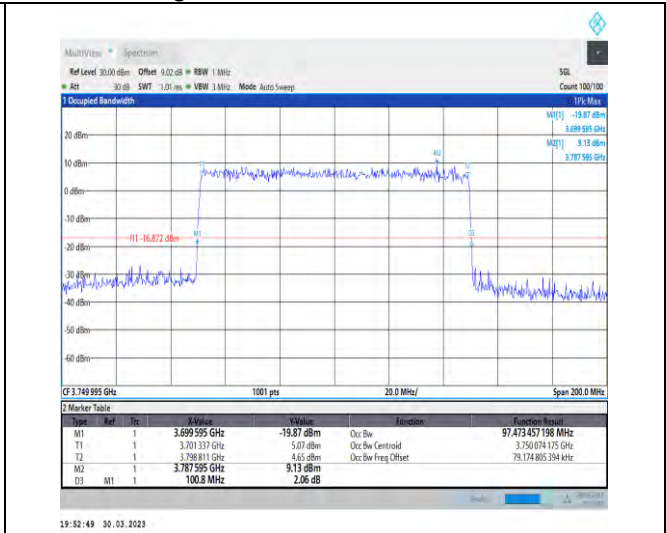
1-N77-3700-3980-30-100-L-9-CP-256QAM-Outer_Fu II-273@0-Ant1-97.473-100.800-≤100-PASS
