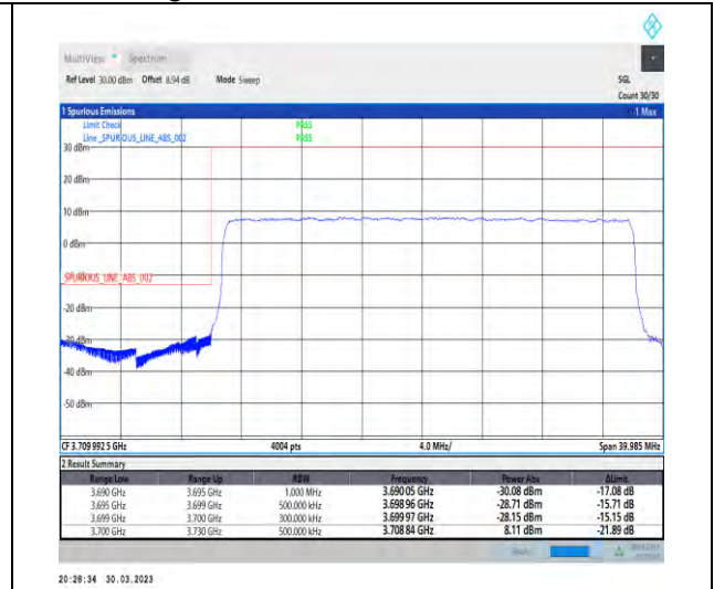
1-N77-3700-3980-30-30-L-3-DFT-PI2BPSK-Outer_Full-75@0-Ant1-1--PASS-see graph
