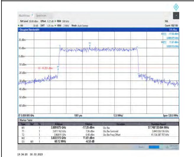
1-N77-3700-3980-30-60-M-6-CP-QPSK-Outer_Full-162@0-Ant1-57.748-60.120-≤60-PASS
