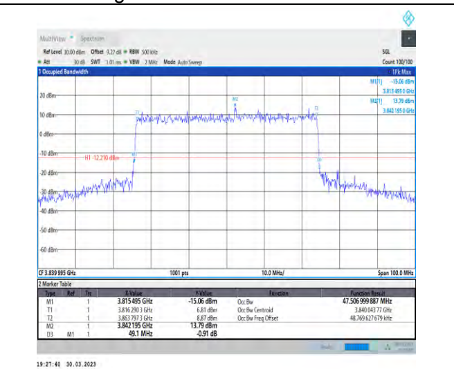
1-N77-3700-3980-30-50-M-8-CP-64QAM-Outer_Full -133@0-Ant1-47.507-49.100-≤50-PASS
