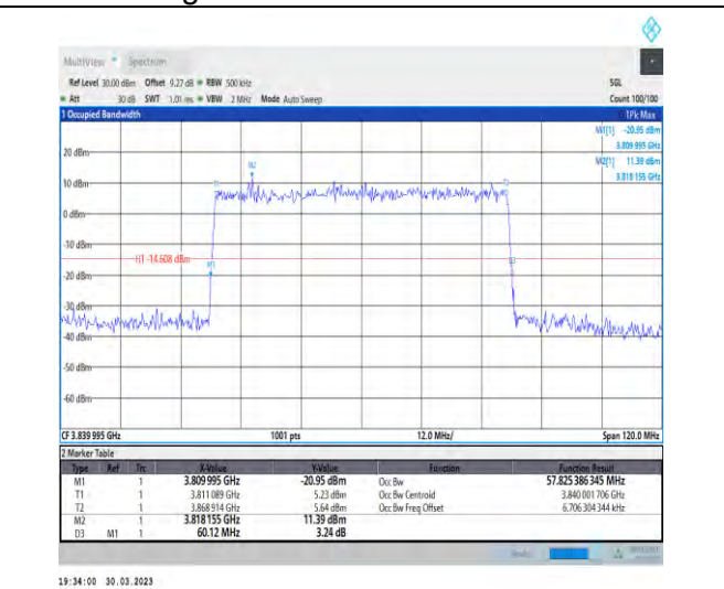
1-N77-3700-3980-30-60-M-5-DFT-256QAM-Outer_Full-162@0-Ant1-57.825-60.120-≤60-PASS
