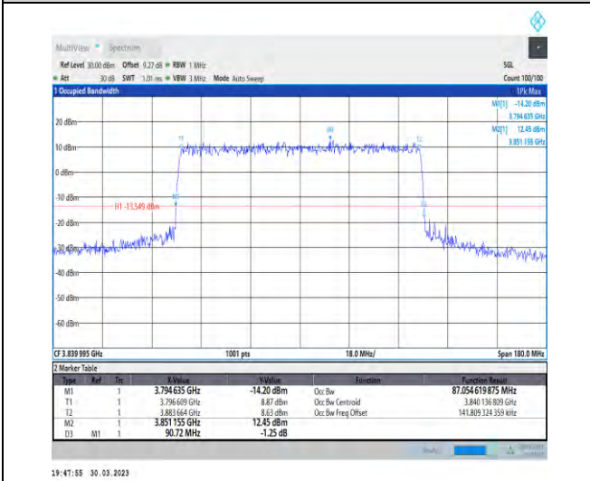
1-N77-3700-3980-30-90-M-8-CP-64QAM-Outer_Full-245@0-Ant1-87.055-90.720-≤90-PASS
