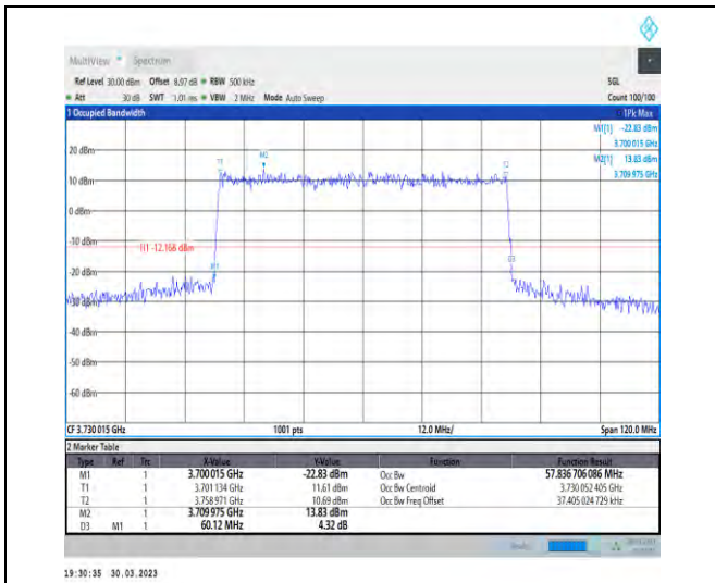
1-N77-3700-3980-30-60-L-1-DFT-QPSK-Outer_Full-162@0-Ant1-57.837-60.120-≤60-PASS
