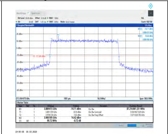
1-N77-3700-3980-30-90-H-6-CP-QPSK-Outer_Full-245@0-Ant1-87.217-90.720-<=90-PASS
