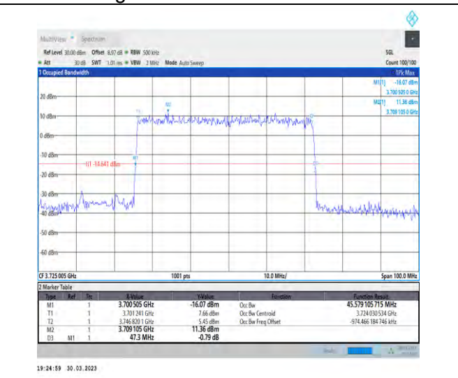
1-N77-3700-3980-30-50-L-5-DFT-256QAM-Outer_Fu ll-128@0-Ant1-45.579-47.300-≤50-PASS
