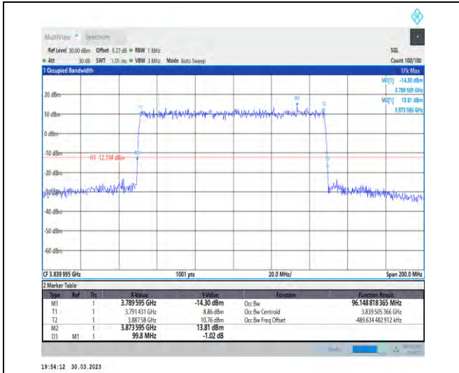
1-N77-3700-3980-30-100-M-3-DFT-16QAM-Outer_Full-270@0-Ant1-96.149-99.800-≤100-PASS
