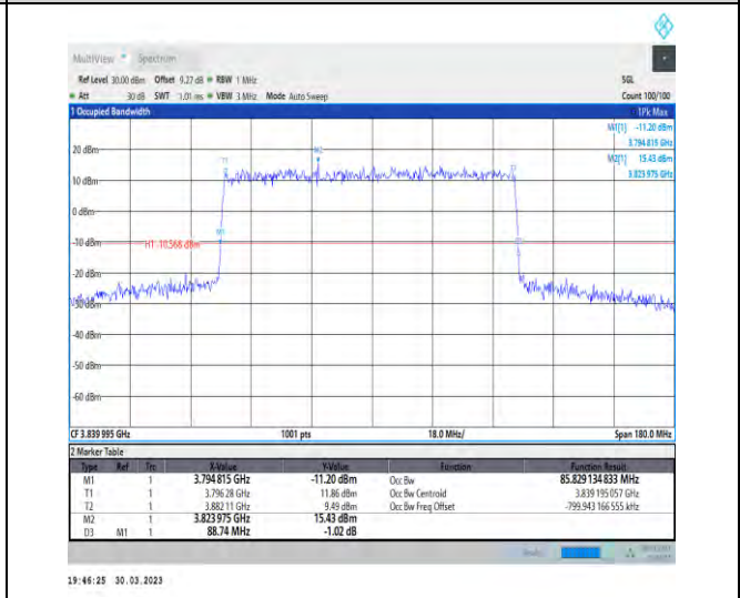
1-N77-3700-3980-30-90-M-1-DFT-QPSK-Outer_Full-240@0-Ant1-85.829-88.740-≤90-PASS
