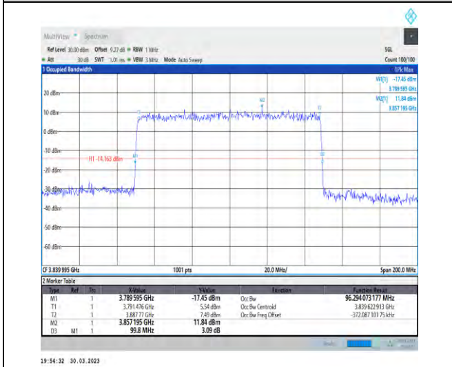
1-N77-3700-3980-30-100-M-5-DFT-256QAM-Outer_Full-270@0-Ant1-96.294-99.800-≤100-PASS
