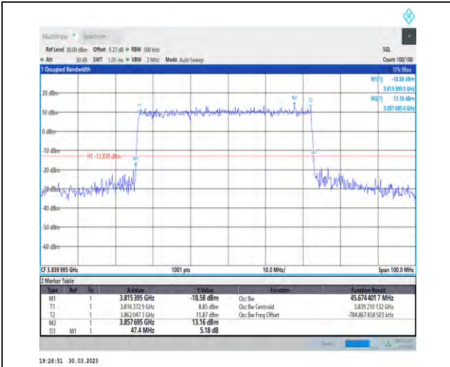
1-N77-3700-3980-30-50-M-3-DFT-16QAM-Outer_Fu I1-128@0-Ant1-45.674-47.400-≤50-PASS
