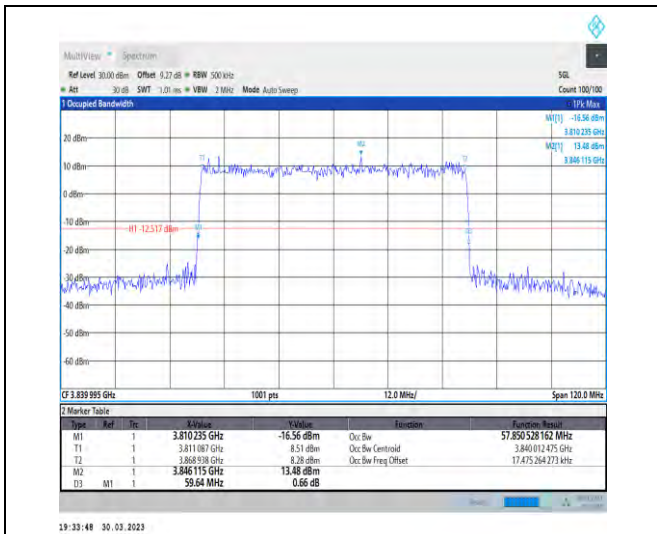
1-N77-3700-3980-30-60-M-4-DFT-64QAM-Outer_Fu II-162@0-Ant1-57.851-59.640-≤60-PASS
