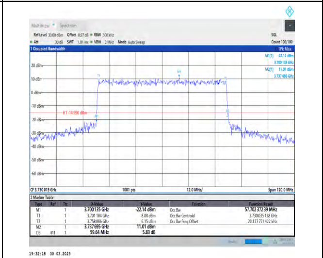
1-N77-3700-3980-30-60-L-8-CP-64QAM-Outer_Full-162@0-Ant1-57.702-59.640-≤60-PASS
