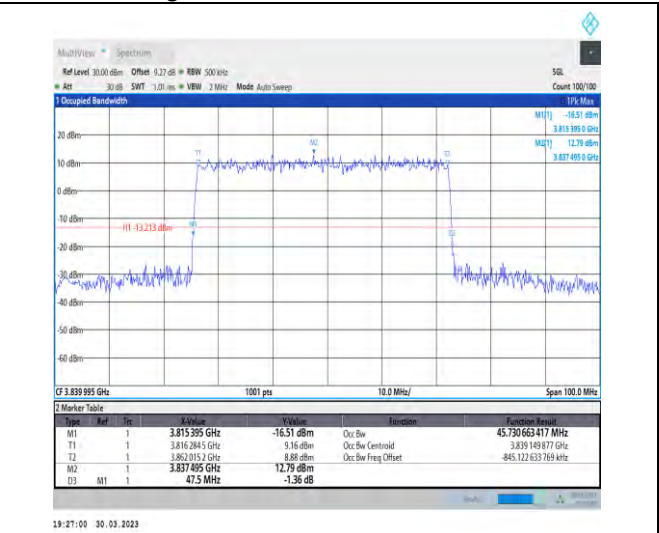
1-N77-3700-3980-30-50-M-4-DFT-64QAM-Outer_Ful I1-128@0-Ant1-45.731-47.500-≤50-PASS
