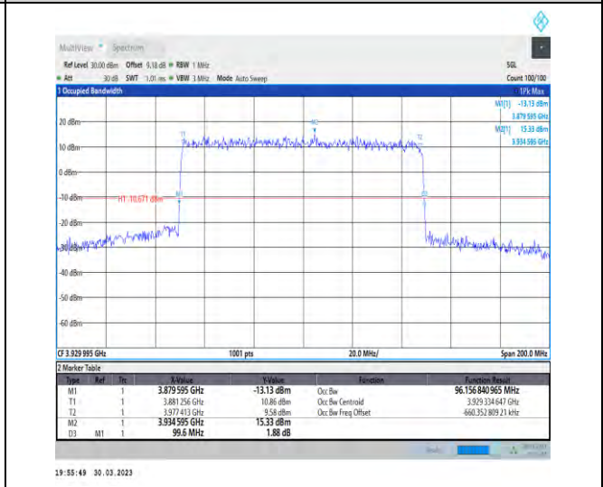
1-N77-3700-3980-30-100-H-1-DFT-QPSK-Outer_Full -270@0-Ant1-96.157-99.600-≤100-PASS
