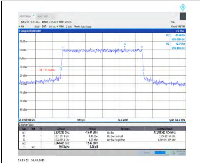
1-N77-3700-3980-30-50-H-6-CP-QPSK-Outer_Full-133@0-Ant1-47.384-49.300-≤50-PASS
