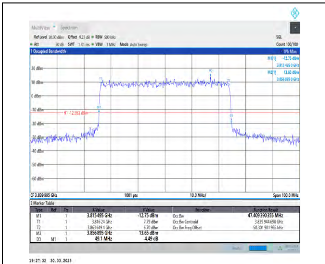
1-N77-3700-3980-30-50-M-7-CP-16QAM-Outer_Full -133@0-Ant1-47.409-49.100-≤50-PASS
