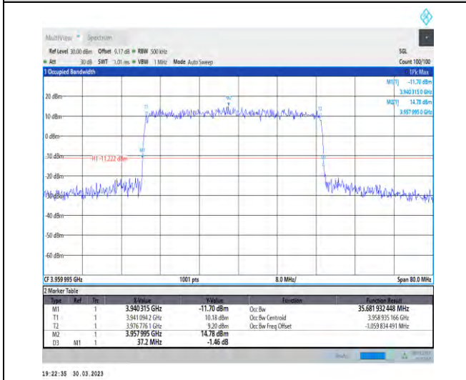
1-N77-3700-3980-30-40-H-3-DFT-16QAM-Outer_Full-100@0-Ant1-35.682-37.200-≤40-PASS
