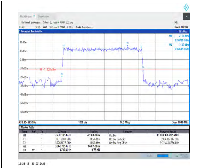
1-N77-3700-3980-30-50-H-2-DFT-PI2BPSK-Outer_Full-128@0-Ant1-45.659-47.600-≤50-PASS
