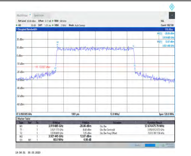
1-N77-3700-3980-30-60-H-6-CP-QPSK-Outer_Full-1 62@0-Ant1-57.674-60.000-≤60-PASS
