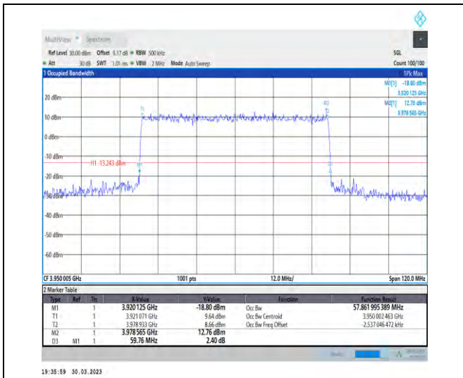
1-N77-3700-3980-30-60-H-3-DFT-16QAM-Outer_Full I-162@0-Ant1-57.862-59.760-≤60-PASS
