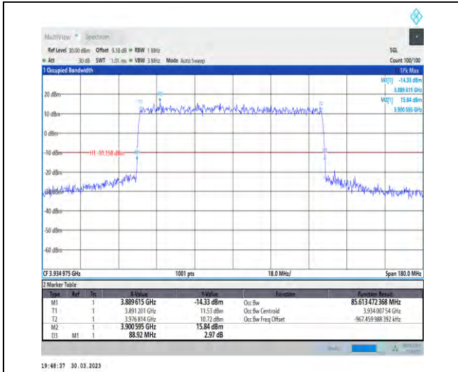
1-N77-3700-3980-30-90-H-1-DFT-QPSK-Outer_Full-240@0-Ant1-85.613-88.920-≤90-PASS
