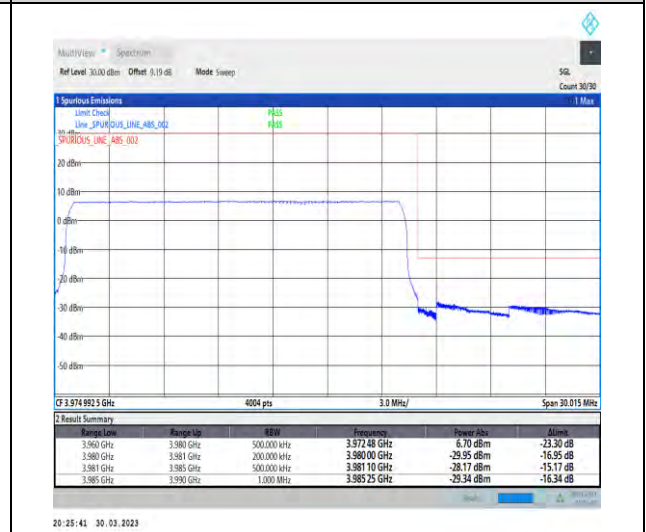
1-N77-3700-3980-30-20-H-6-CP-QPSK-Outer_Full-51@0-Ant1-1--PASS-see graph
