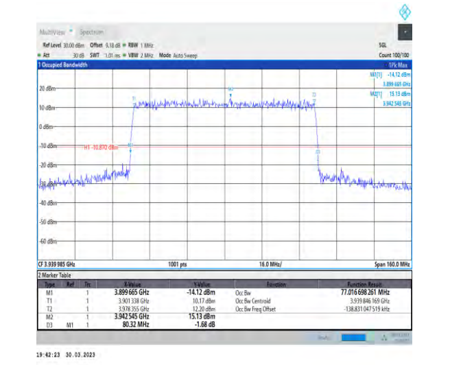
1-N77-3700-3980-30-80-H-3-DFT-16QAM-Outer_Full-216@0-Ant1-77.017-80.320-≤80-PASS
