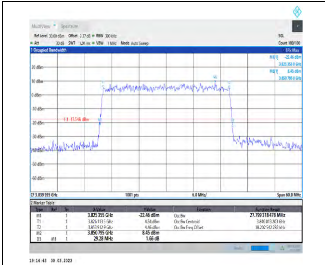
1-N77-3700-3980-30-30-M-9-CP-256QAM-Outer_Fu ll-78@0-Ant1-27.799-29.280-≤30-PASS
