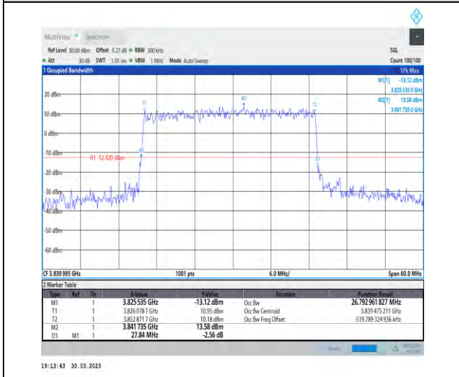
1-N77-3700-3980-30-30-M-3-DFT-16QAM-Outer_Full-75@0-Ant1-26.793-27.840-≤30-PASS
