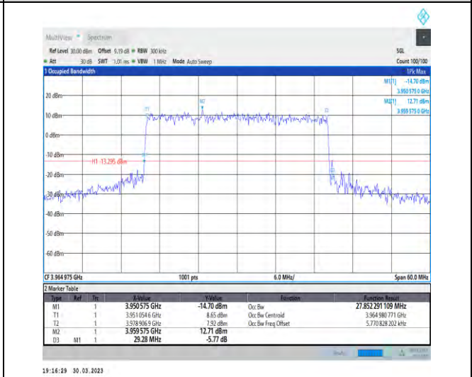
1-N77-3700-3980-30-30-H-7-CP-16QAM-Outer_Full-78@0-Ant1-27.852-29.280-≤30-PASS
