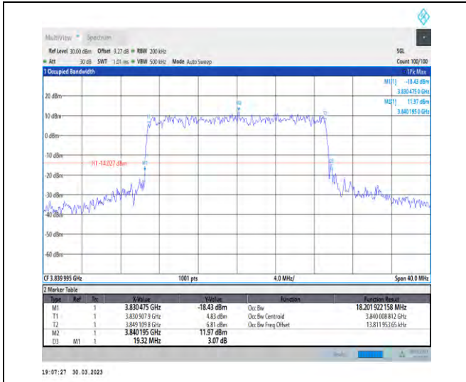
1-N77-3700-3980-30-20-M-8-CP-64QAM-Outer_Full -51@0-Ant1-18.202-19.320-≤20-PASS
