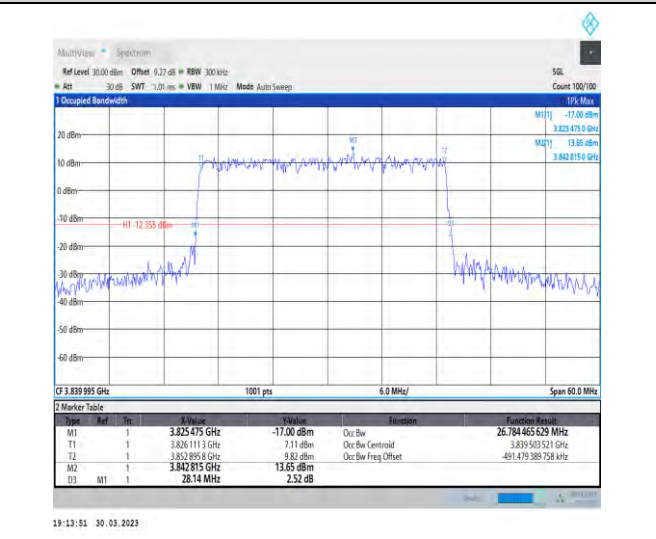
1-N77-3700-3980-30-30-M-4-DFT-64QAM-Outer_Full-75@0-Ant1-26.784-28.140-≤30-PASS
