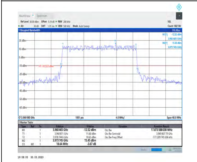
1-N77-3700-3980-30-20-H-1-DFT-QPSK-Outer_Full-50@0-Ant1-17.874-18.640-≤20-PASS
