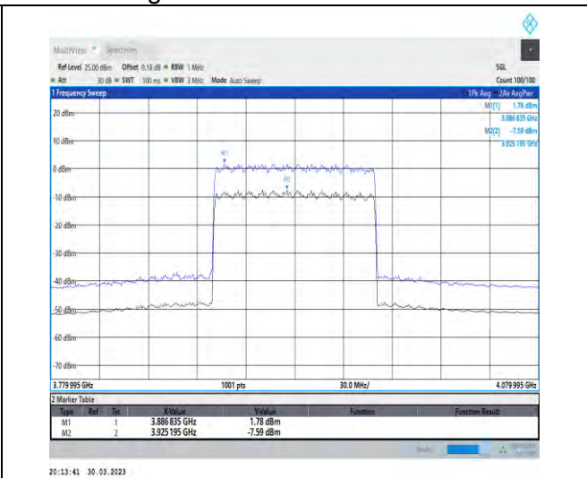
1-N77-3700-3980-30-100-H-2-CP-256QAM-Outer_Full-273@0-Ant1-9.37-100%-0.00-9.37-PASS-≤13
