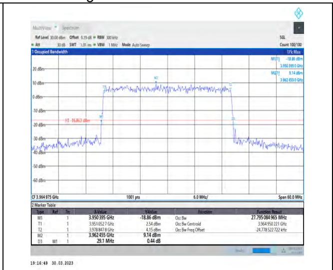
1-N77-3700-3980-30-30-H-9-CP-256QAM-Outer_Full-78@0-Ant1-27.795-29.100-≤30-PASS
