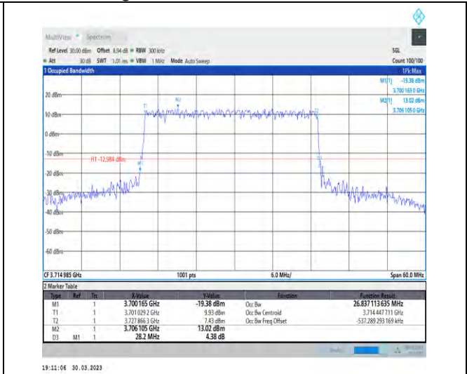
1-N77-3700-3980-30-30-L-3-DFT-16QAM-Outer_Full-75@0-Ant1-26.837-28.200-≤30-PASS
