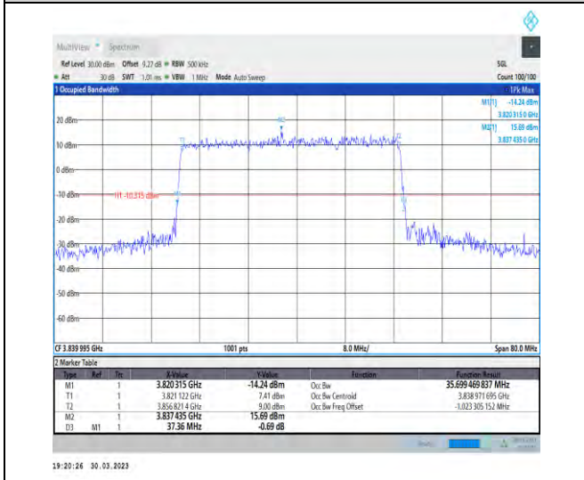
1-N77-3700-3980-30-40-M-4-DFT-64QAM-Outer_Full-100@0-Ant1-35.699-37.360-<=40-PASS
