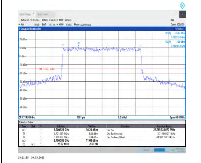
1-N77-3700-3980-30-30-L-8-CP-64QAM-Outer_Full-78@0-Ant1-27.785-28.920-≤30-PASS
