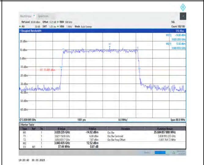
1-N77-3700-3980-30-40-M-5-DFT-256QAM-Outer_Full-100@0-Ant1-35.685-37.440-<=40-PASS
