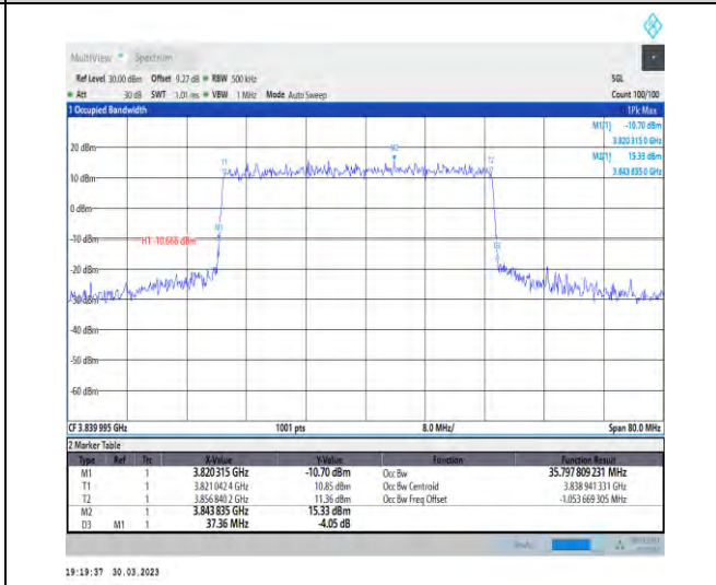
1-N77-3700-3980-30-40-M-1-DFT-QPSK-Outer_Full-100@0-Ant1-35.798-37.360-≤40-PASS
