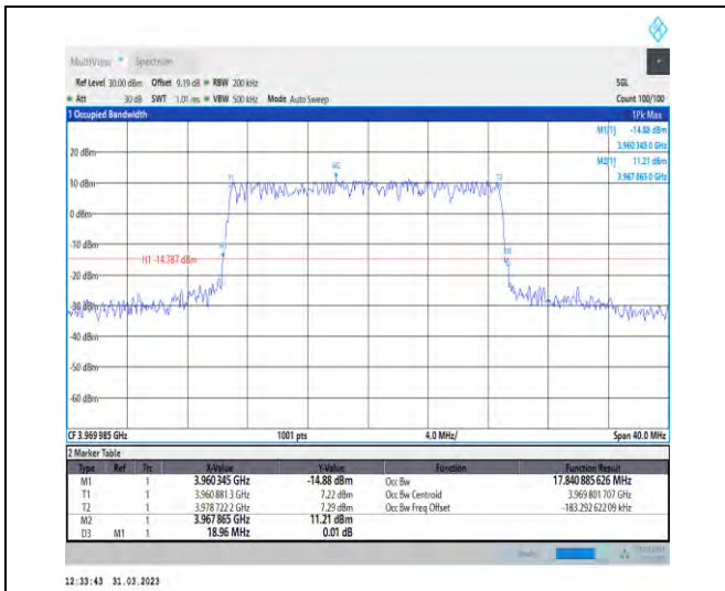
1-N77-3700-3980-30-20-H-3-DFT-16QAM-Outer_Full I-50@0-Ant1-17.841-18.960-≤20-PASS
