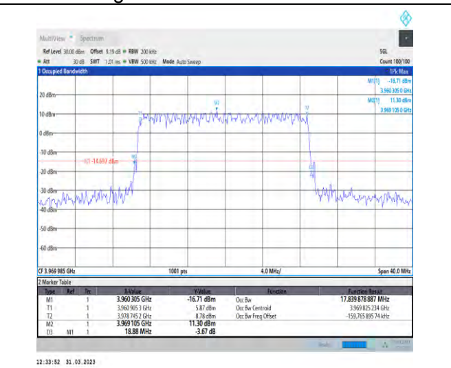
1-N77-3700-3980-30-20-H-4-DFT-64QAM-Outer_Full -50@0-Ant1-17.84-18.880-≤20-PASS
