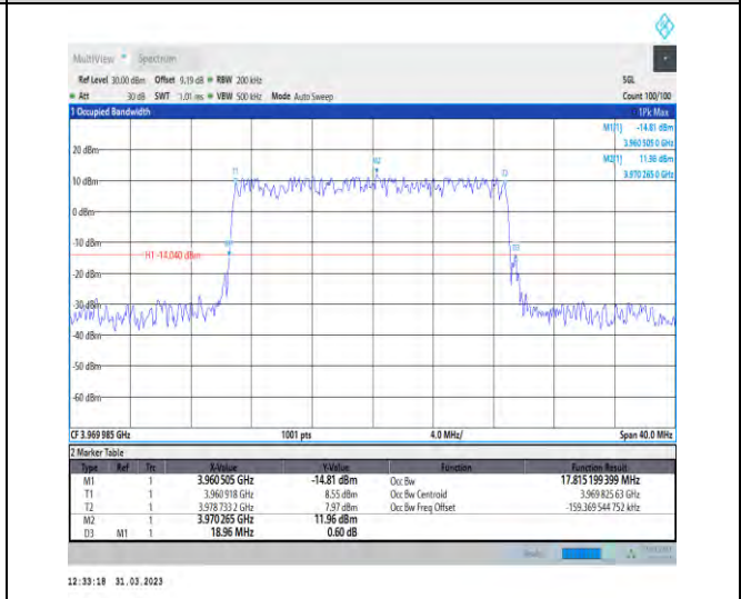
1-N77-3700-3980-30-20-H-2-DFT-PI2BPSK-Outer_Full-50@0-Ant1-17.815-18.960-≤20-PASS
