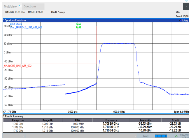
Band4-1.4MHz-QPSK-19957-6RB#0
