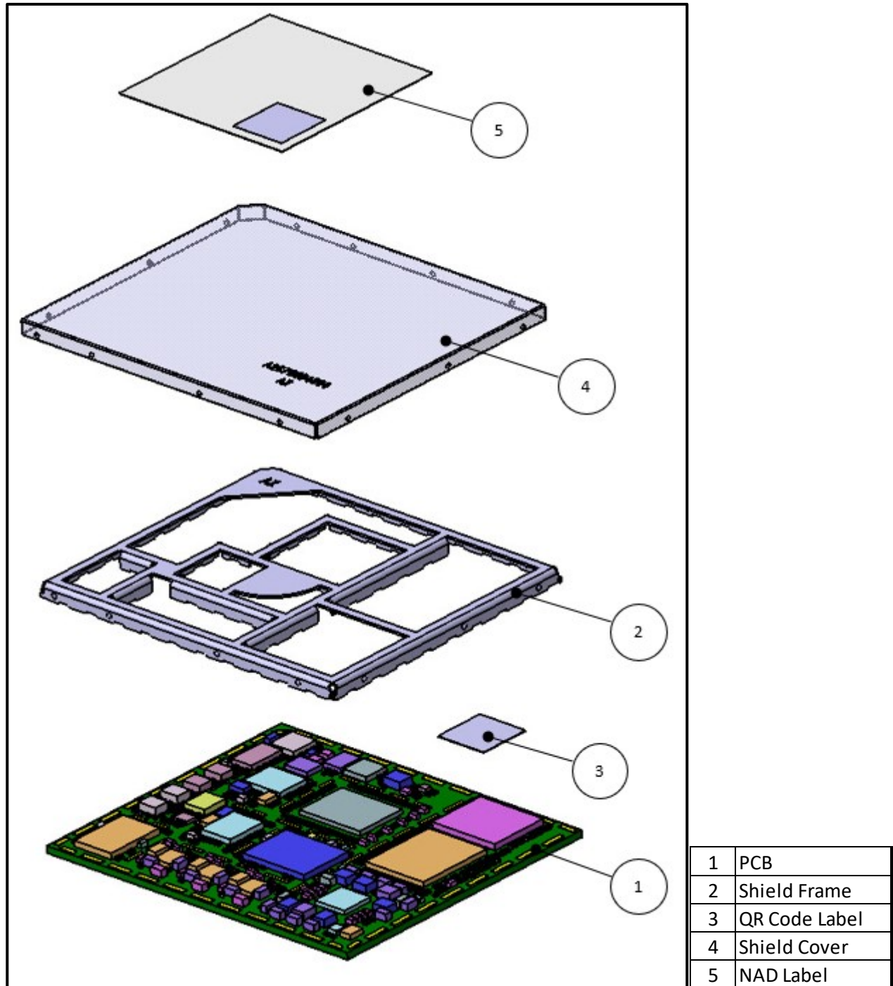
Figure 6-1: Module Exploded View
