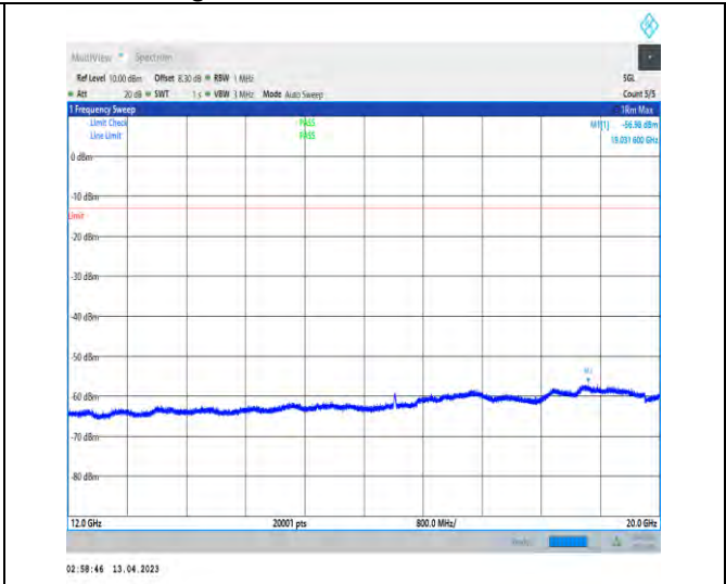
1-DC_2A_n5A-PC3-15-5+20-M+L-1-N/A-N/A-N/A-DF T-PI2BPSK-Inner_1RB_Left-1@1-12000-20000-1893 7.20--56.98--13-PASS
