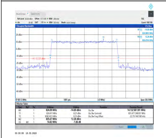
1-DC_2A_n5A-PC3-15-5+15-M+L-9-N/A-N/A-N/A-C P-256QAM-Outer_Full-79@0-Ant1-14.133-14.820-≤ 15-PASS
