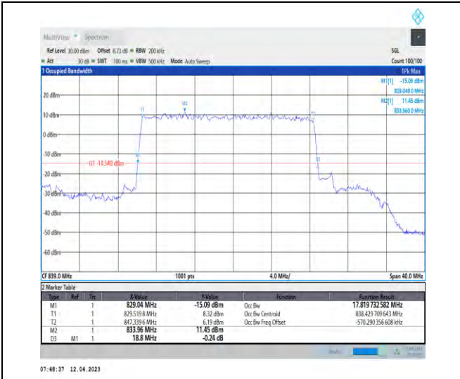
1-DC_2A_n5A-PC3-15-5+20-M+H-2-N/A-N/A-N/A-D FT-PI2BPSK-Outer_Full-100@0-Ant1-17.82-18.800- ≤20-PASS
