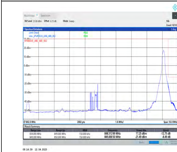
1-DC_2A_n5A-PC3-15-5+15-M+H-5-QPSK-Edge_1RB_Right-Edge_1_Right@N/A-CP-QPSK-Edge_1RB_Right-1@78-1-seegraph-PASS-see graph
