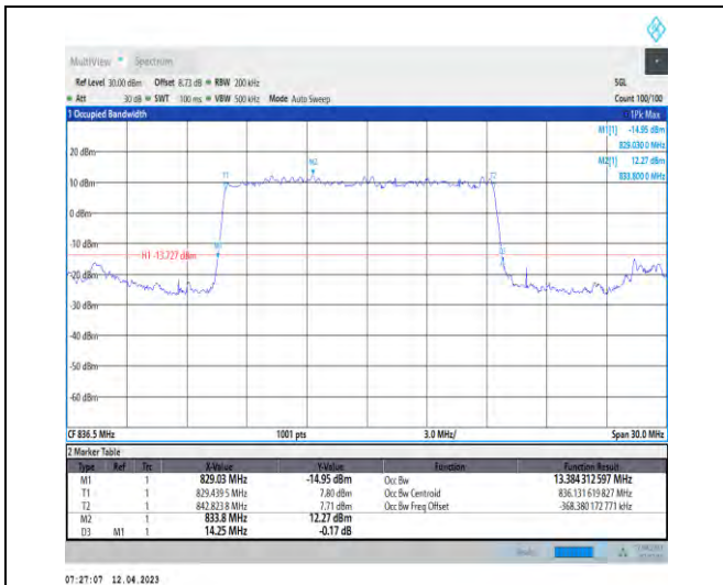
1-DC_2A_n5A-PC3-15-5+15-M+M-2-N/A-N/A-N/A-D FT-PI2BPSK-Outer_Full-75@0-Ant1-13.384-14.250- ≤15-PASS
