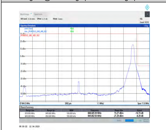
1-DC_2A_n5A-PC3-15-5+10-M+H-5-QPSK-Edge_1RB_Right-Edge_1_Right@N/A-CP-QPSK-Edge_1RB_Right-1@51-1-seegraph-PASS-see graph
