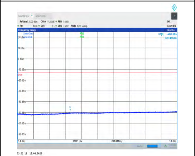
1-DC_2A_n5A-PC3-15-5+20-M+H-1-N/A-N/A-N/A-DF T-PI2BPSK-Inner_1RB_Left-1@1-1000-3000-1877.8 0--48.46--13-PASS
