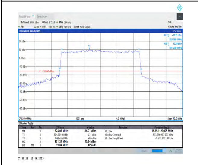
1-DC_2A_n5A-PC3-15-5+20-M+L-6-N/A-N/A-N/A-C P-QPSK-Outer_Full-106@0-Ant1-18.851-19.840-≤2 0-PASS
