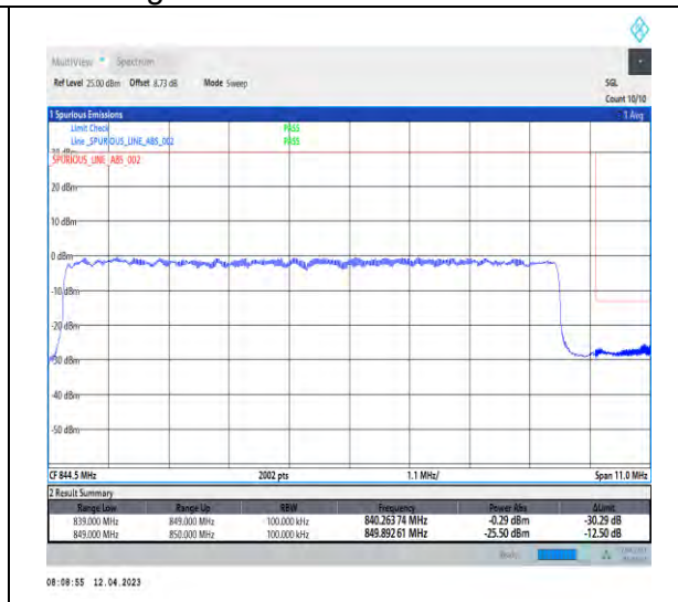
1-DC_2A_n5A-PC3-15-5+10-M+H-3-QPSK-Outer_Full-Outer_Full@N/A-DFT-PI2BPSK-Outer_Full-50@0-1-seegraph-PASS-see graph
