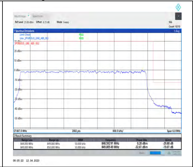
1-DC_2A_n5A-PC3-15-5+5-M+H-3-QPSK-Outer_Full-Outer_Full@N/A-DFT-PI2BPSK-Outer_Full-25@0-1-seegraph-PASS-see graph
