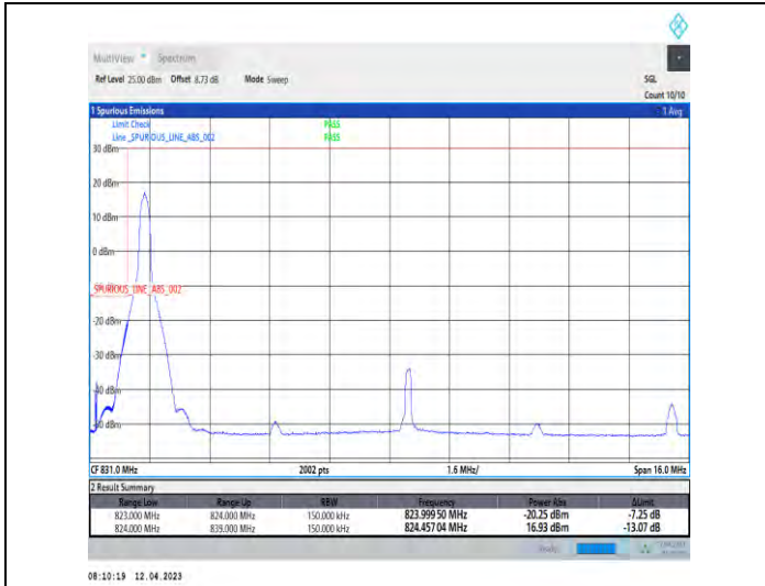
1-DC_2A_n5A-PC3-15-5+15-M+L-1-QPSK-Edge_1RB_Left-Edge_1_Left@N/A-DFT-PI2BPSK-Edge_1RB_Left-1@0-1-seegraph-PASS-see graph
