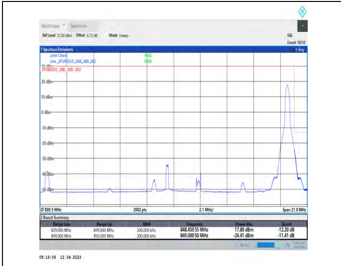
1-DC_2A_n5A-PC3-15-5+20-M+H-2-QPSK-Edge_1RB_Right-Edge_1_Right@N/A-DFT-PI2BPSK-Edge_1RB_Right-1@105-1-seegraph-PASS-see graph
