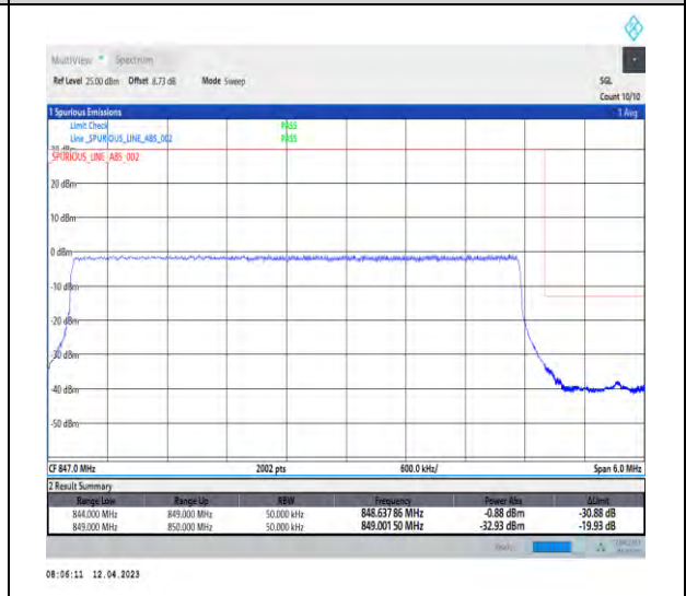
1-DC_2A_n5A-PC3-15-5+5-M+H-6-QPSK-Outer_Full-Outer_Full@N/A-CP-QPSK-Outer_Full-25@0-1-seegraph-PASS-see graph
