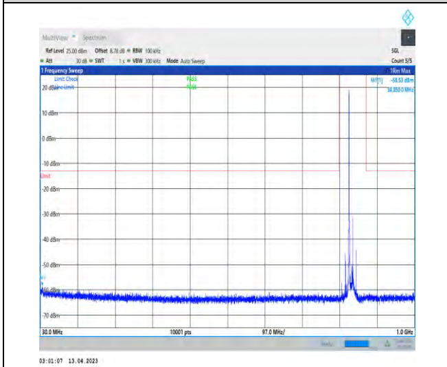
1-DC_2A_n5A-PC3-15-5+20-M+H-1-N/A-N/A-N/A-D FT-PI2BPSK-Inner_1RB_Left-1@1-30-1000-33.78-- 58.53--13-PASS
