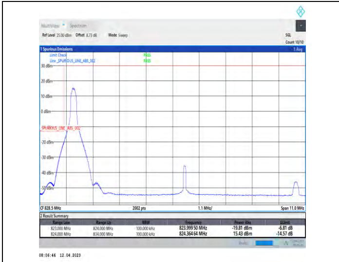
1-DC_2A_n5A-PC3-15-5+10-M+L-1-QPSK-Edge_1RB_Left-Edge_1_Left@N/A-DFT-PI2BPSK-Edge_1RB_Left-1@0-1-seegraph-PASS-see graph
