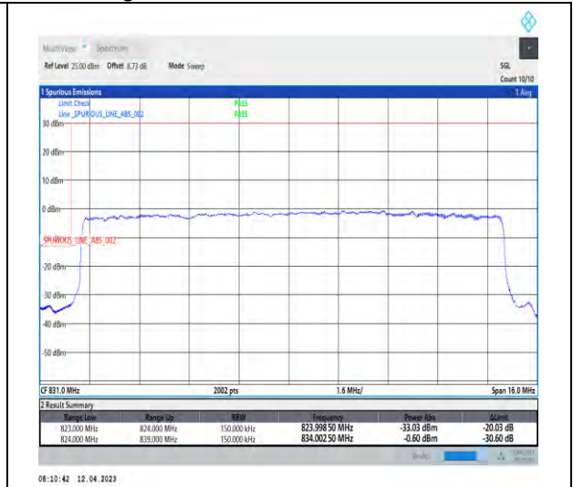
1-DC_2A_n5A-PC3-15-5+15-M+L-3-QPSK-Outer_Full-Outer_Full@N/A-DFT-PI2BPSK-Outer_Full-75@0-1-seegraph-PASS-see graph
