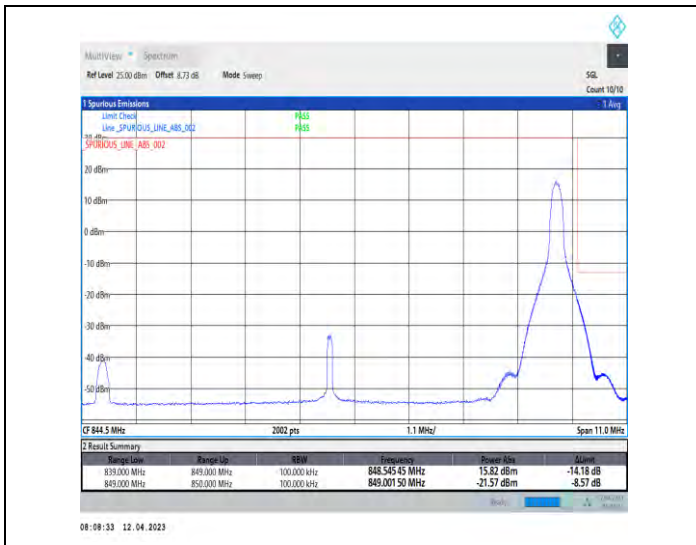
1-DC_2A_n5A-PC3-15-5+10-M+H-2-QPSK-Edge_1RB_Right-Edge_1_Right@N/A-DFT-PI2BPSK-Edge_1RB_Right-1@51-1-seegraph-PASS-see graph
