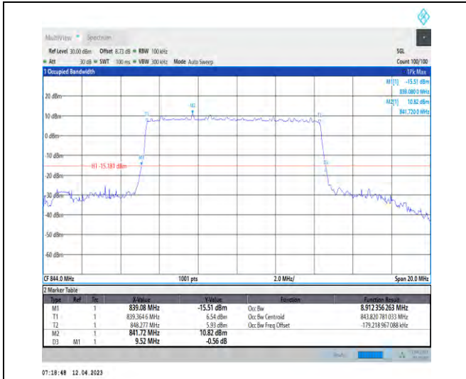
1-DC_2A_n5A-PC3-15-5+10-M+H-4-N/A-N/A-N/A-D FT-64QAM-Outer_Full-50@0-Ant1-8.912-9.520-≤10- PASS
