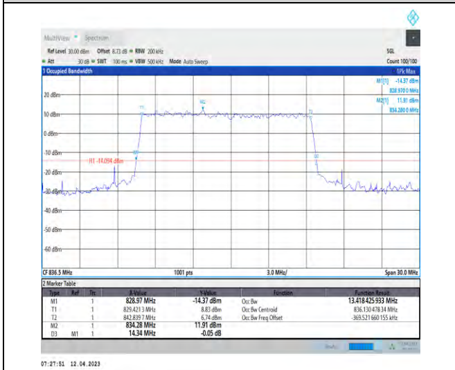
1-DC_2A_n5A-PC3-15-5+15-M+M-4-N/A-N/A-N/A-D FT-64QAM-Outer_Full-75@0-Ant1-13.418-14.340-≤ 15-PASS
