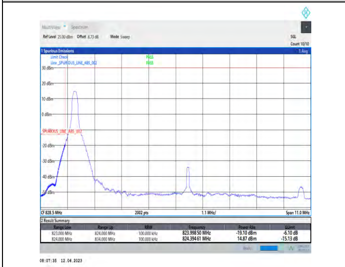
1-DC_2A_n5A-PC3-15-5+10-M+L-4-QPSK-Edge_1RB_Left-Edge_1_Left@N/A-CP-QPSK-Edge_1RB_Left-1@0-1-seegraph-PASS-see graph
