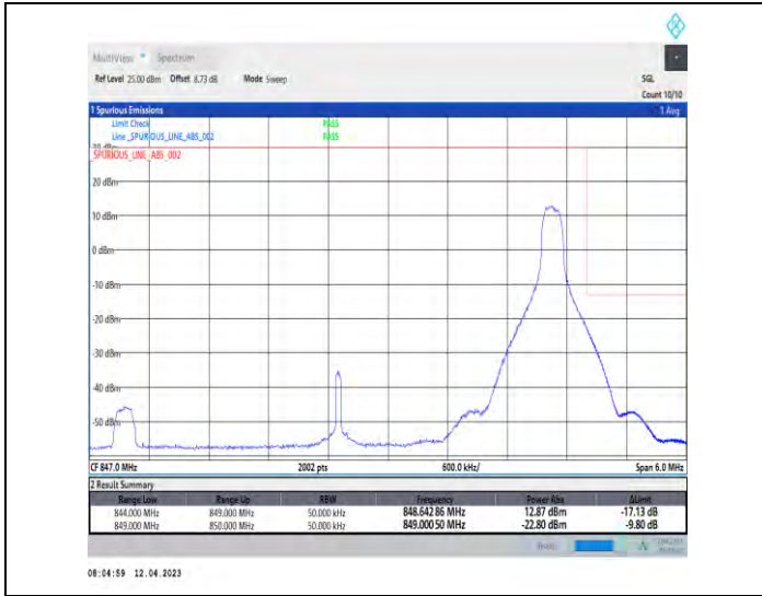
1-DC_2A_n5A-PC3-15-5+5-M+H-2-QPSK-Edge_1RB_Right-Edge_1_Right@N/A-DFT-PI2BPSK-Edge_1RB_Right-1@24-1-seegraph-PASS-see graph
