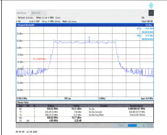
1-DC_2A_n5A-PC3-15-5+5-M+M-3-N/A-N/A-N/A-DF T-16QAM-Outer_Full-25@0-Ant1-4.48-4.890-≤5-PAS S
