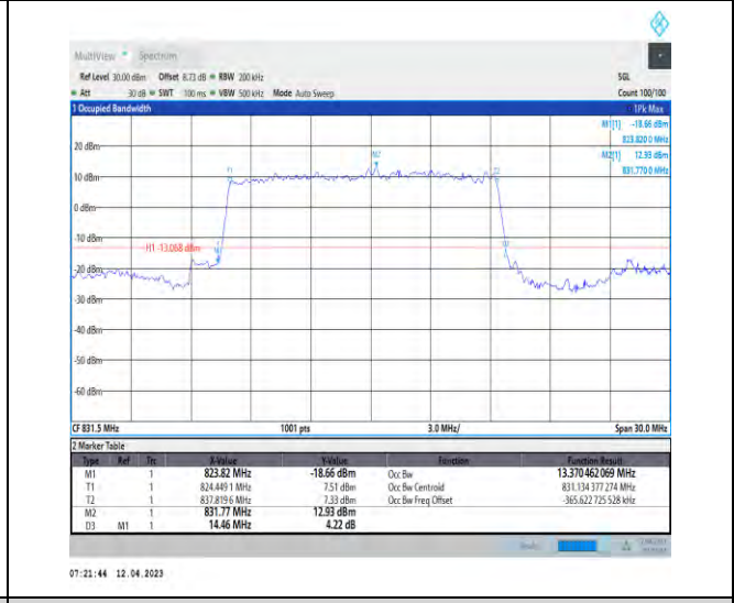
1-DC_2A_n5A-PC3-15-5+15-M+L-2-N/A-N/A-N/A-D FT-PI2BPSK-Outer_Full-75@0-Ant1-13.37-14.460-≤ 15-PASS
