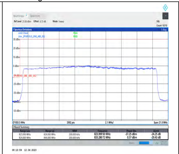
1-DC_2A_n5A-PC3-15-5+20-M+L-3-QPSK-Outer_Full-Outer_Full@N/A-DFT-PI2BPSK-Outer_Full-100@0-1-seegraph-PASS-see graph
