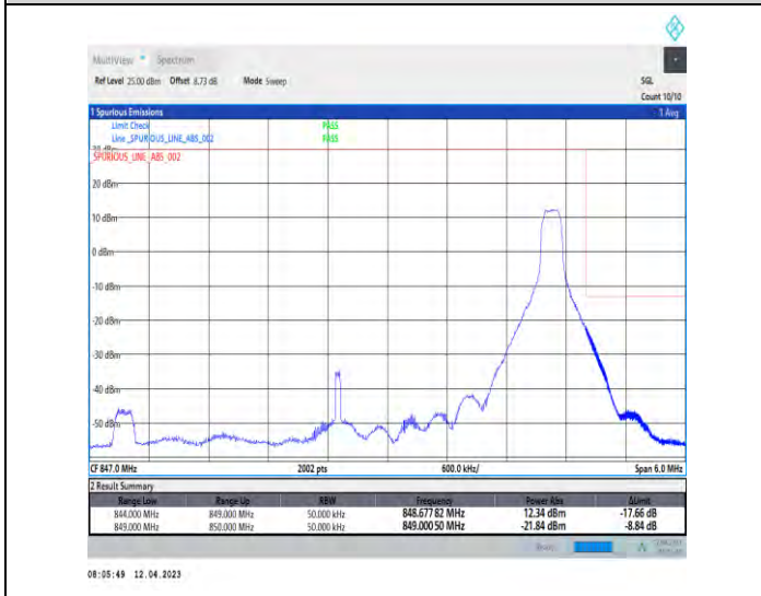
1-DC_2A_n5A-PC3-15-5+5-M+H-5-QPSK-Edge_1RB_Right-Edge_1_Right@N/A-CP-QPSK-Edge_1RB_Right-1@24-1-seegraph-PASS-see graph
