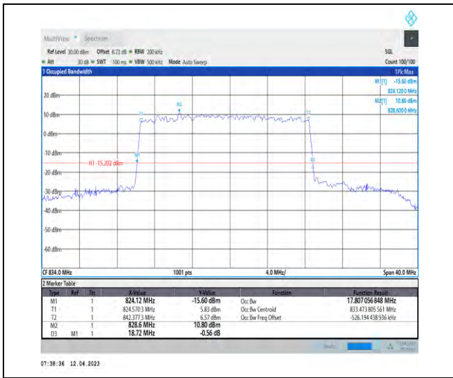
1-DC_2A_n5A-PC3-15-5+20-M+L-4-N/A-N/A-N/A-D FT-64QAM-Outer_Full-100@0-Ant1-17.807-18.720- ≤20-PASS
