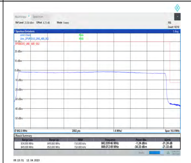
1-DC_2A_n5A-PC3-15-5+15-M+H-6-QPSK-Outer_Full-Outer_Full@N/A-CP-QPSK-Outer_Full-79@0-1-seegraph-PASS-see graph
