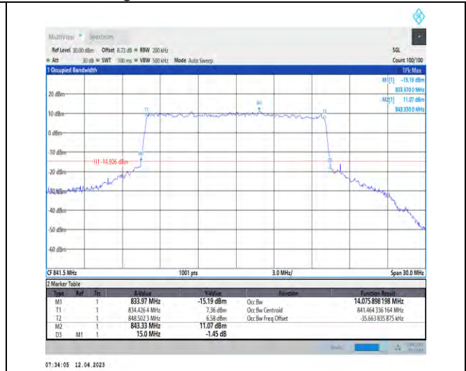
1-DC_2A_n5A-PC3-15-5+15-M+H-6-N/A-N/A-N/A-C P-QPSK-Outer_Full-79@0-Ant1-14.076-15.000-≤15- PASS
