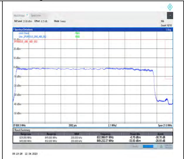
1-DC_2A_n5A-PC3-15-5+20-M+H-3-QPSK-Outer_Full-Outer_Full@N/A-DFT-PI2BPSK-Outer_Full-100@0-1-seegraph-PASS-see graph
