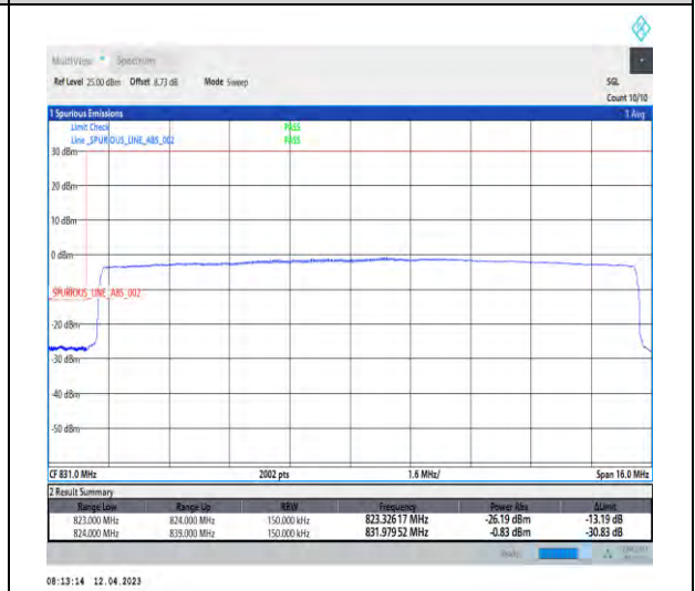
1-DC_2A_n5A-PC3-15-5+15-M+L-6-QPSK-Outer_Full-Outer_Full@N/A-CP-QPSK-Outer_Full-79@0-1-seegraph-PASS-see graph
