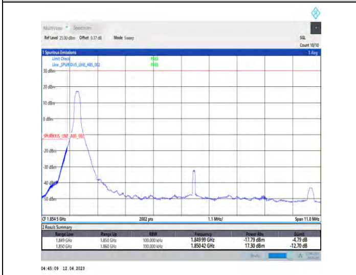
1-DC_5A_n2A-PC3-15-5+10-M+L-4-QPSK-Edge_1RB_Left-Edge_1_Left@N/A-CP-QPSK-Edge_1RB_Left-1@0-1-seegraph-PASS-see graph
