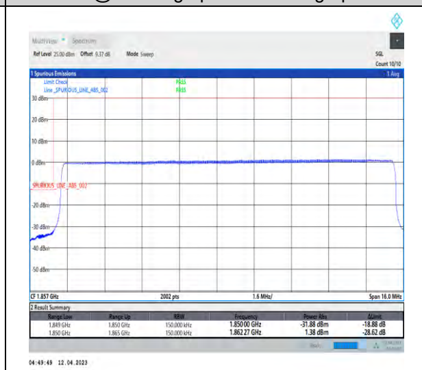
1-DC_5A_n2A-PC3-15-5+15-M+L-6-QPSK-Outer_Full-Outer_Full@N/A-CP-QPSK-Outer_Full-79@0-1-seegraph-PASS-see graph
