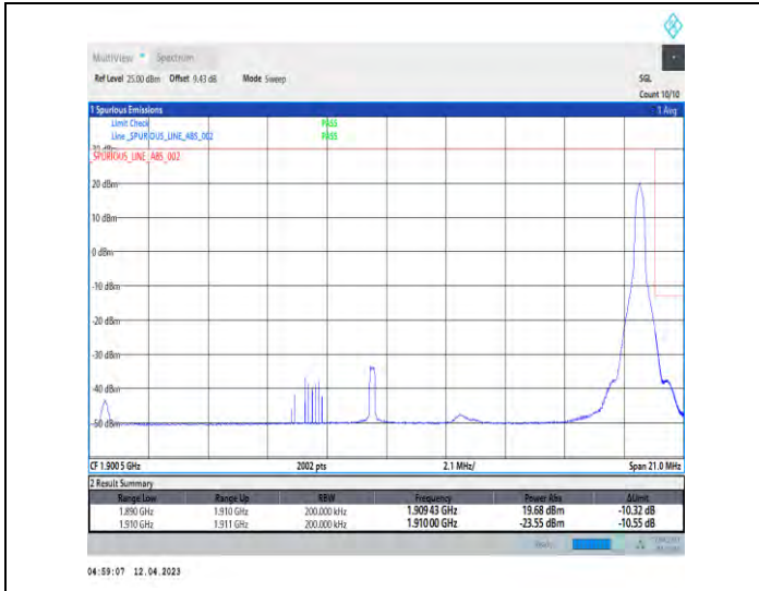
1-DC_5A_n2A-PC3-15-5+20-M+H-2-QPSK-Edge_1RB_Right-Edge_1_Right@N/A-DFT-PI2BPSK-Edge_1RB_Right-1@105-1-seegraph-PASS-see graph
