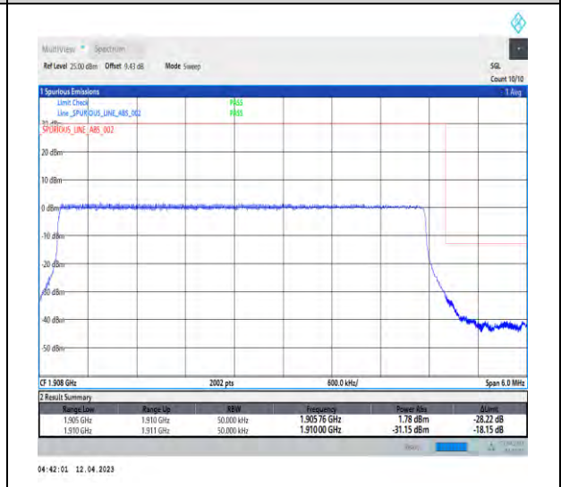
1-DC_5A_n2A-PC3-15-5+5-M+H-6-QPSK-Outer_Full-Outer_Full@N/A-CP-QPSK-Outer_Full-25@0-1-seegraph-PASS-see graph
