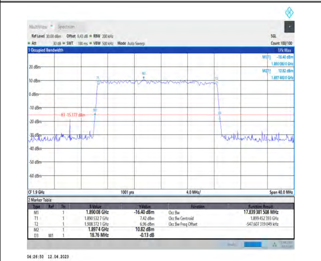
1-DC_5A_n2A-PC3-15-5+20-M+H-5-N/A-N/A-N/A-D FT-256QAM-Outer_Full-100@0-Ant1-17.839-18.760- ≤20-PASS
