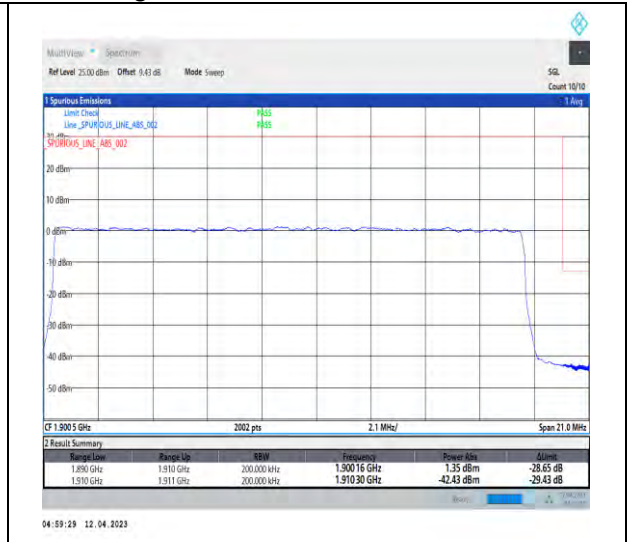
1-DC_5A_n2A-PC3-15-5+20-M+H-3-QPSK-Outer_Full-Outer_Full@N/A-DFT-PI2BPSK-Outer_Full-100@0-1-seegraph-PASS-see graph
