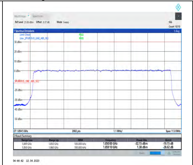
1-DC_5A_n2A-PC3-15-5+10-M+L-3-QPSK-Outer_Full-Outer_Full@N/A-DFT-PI2BPSK-Outer_Full-50@0-1-seegraph-PASS-see graph
