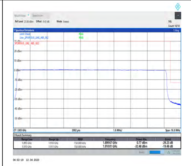
1-DC_5A_n2A-PC3-15-5+15-M+H-6-QPSK-Outer_Full-Outer_Full@N/A-CP-QPSK-Outer_Full-79@0-1-seegraph-PASS-see graph
