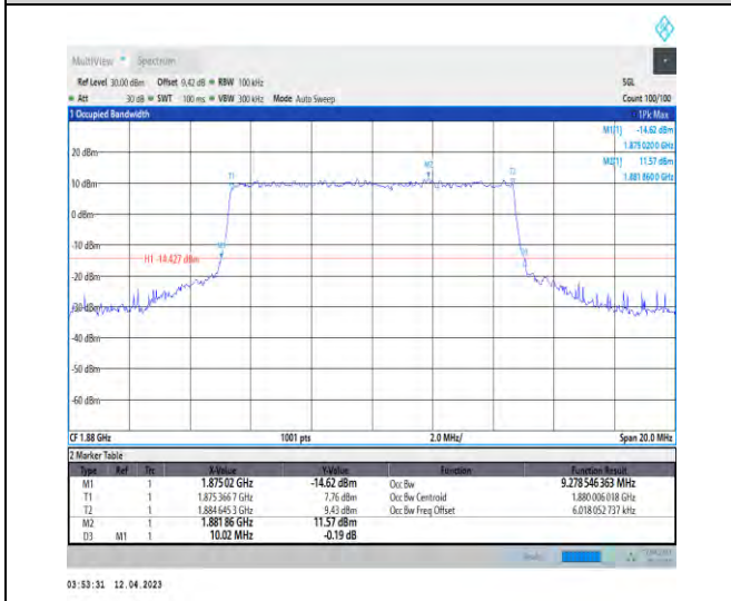
1-DC_5A_n2A-PC3-15-5+10-M+M-7-N/A-N/A-N/A-C P-16QAM-Outer_Full-52@0-Ant1-9.279-10.020-≤10- PASS
