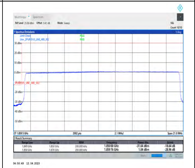
1-DC_5A_n2A-PC3-15-5+20-M+L-6-QPSK-Outer_Full-Outer_Full@N/A-CP-QPSK-Outer_Full-106@0-1-seegraph-PASS-see graph
