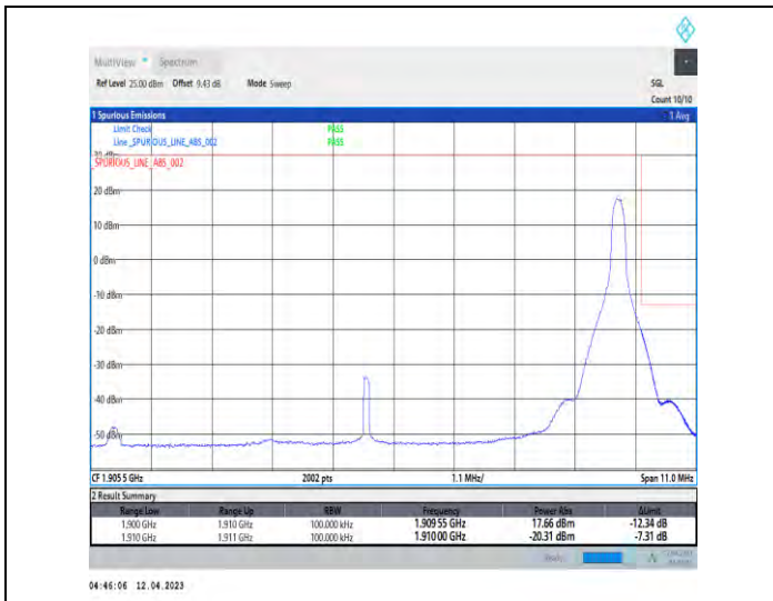
1-DC_5A_n2A-PC3-15-5+10-M+H-2-QPSK-Edge_1RB_Right-Edge_1_Right@N/A-DFT-PI2BPSK-Edge_1RB_Right-1@51-1-seegraph-PASS-see graph
