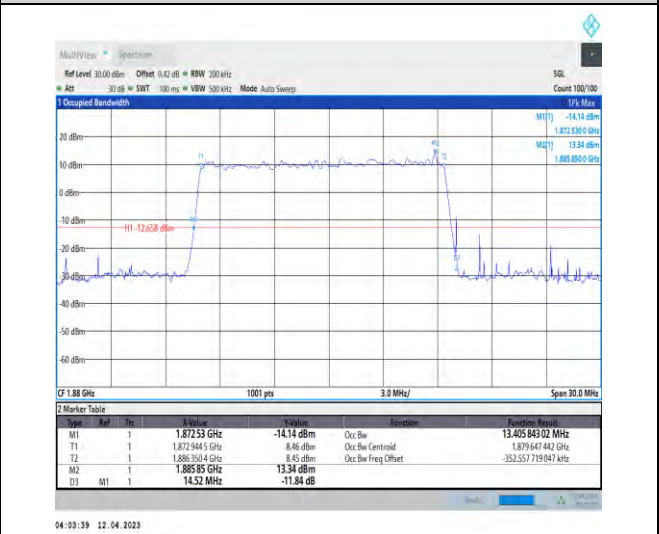
1-DC_5A_n2A-PC3-15-5+15-M+M-5-N/A-N/A-N/A-D FT-256QAM-Outer_Full-75@0-Ant1-13.406-14.520-≤15-PASS
