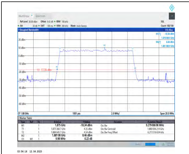
1-DC_5A_n2A-PC3-15-5+10-M+M-9-N/A-N/A-N/A-C P-256QAM-Outer_Full-52@0-Ant1-9.279-9.980≤10-PASS
