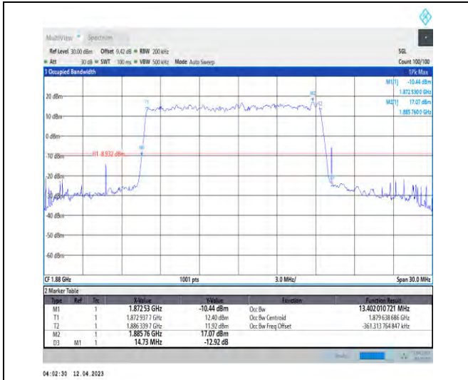
1-DC_5A_n2A-PC3-15-5+15-M+M-2-N/A-N/A-N/A-D FT-PI2BPSK-Outer_Full-75@0-Ant1-13.402-14.730- ≤15-PASS
