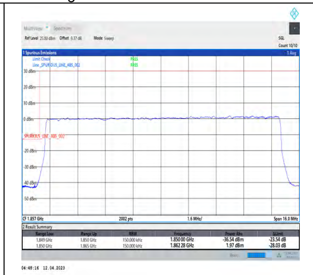
1-DC_5A_n2A-PC3-15-5+15-M+L-3-QPSK-Outer_Full-Outer_Full@N/A-DFT-PI2BPSK-Outer_Full-75@0-1-seegraph-PASS-see graph
