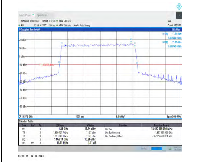
1-DC_5A_n2A-PC3-15-5+15-M+L-1-N/A-N/A-N/A-D FT-QPSK-Outer_Full-75@0-Ant1-13.42-14.310-≤15-P PASS
