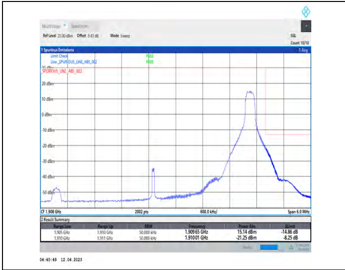
1-DC_5A_n2A-PC3-15-5+5-M+H-2-QPSK-Edge_1RB_Right-Edge_1_Right@N/A-DFT-PI2BPSK-Edge_1RB_Right-1@24-1-seegraph-PASS-see graph
