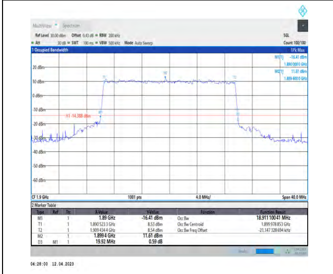
1-DC_5A_n2A-PC3-15-5+20-M+H-8-N/A-N/A-N/A-C P-64QAM-Outer_Full-106@0-Ant1-18.911-19.920-≤20 0-PASS
