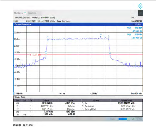
1-DC_5A_n2A-PC3-15-5+20-M+M-6-N/A-N/A-N/A-C P-QPSK-Outer_Full-106@0-Ant1-18.9-19.880-≤20-P ASS
