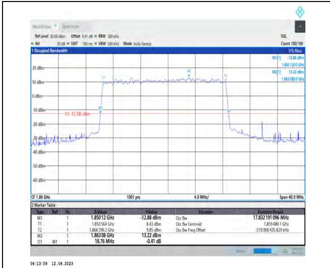
1-DC_5A_n2A-PC3-15-5+20-M+L-4-N/A-N/A-N/A-D FT-64QAM-Outer_Full-100@0-Ant1-17.832-18.760-≤ 20-PASS
