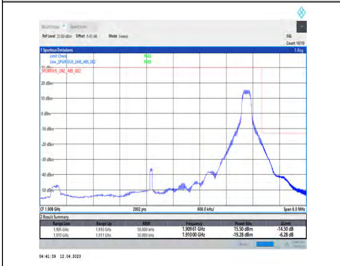
1-DC_5A_n2A-PC3-15-5+5-M+H-5-QPSK-Edge_1RB_Right-Edge_1_Right@N/A-CP-QPSK-Edge_1RB_Right-1@24-1-seegraph-PASS-see graph
