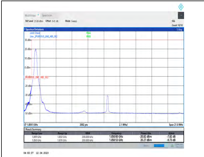
1-DC_5A_n2A-PC3-15-5+20-M+L-1-QPSK-Edge_1RB_Left-Edge_1_Left@N/A-DFT-PI2BPSK-Edge_1RB_Left-1@0-1-seegraph-PASS-see graph
