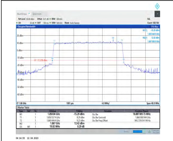
1-DC_5A_n2A-PC3-15-5+20-M+L-6-N/A-N/A-N/A-C P-QPSK-Outer_Full-106@0-Ant1-18.887-19.920-≤20 -PASS
