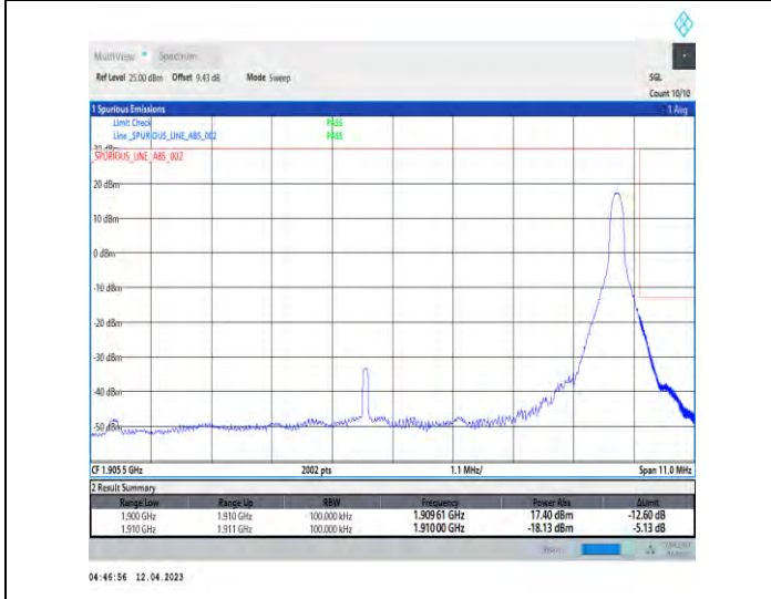
1-DC_5A_n2A-PC3-15-5+10-M+H-5-QPSK-Edge_1RB_Right-Edge_1_Right@N/A-CP-QPSK-Edge_1RB_Right-1@51-1-seegraph-PASS-see graph
