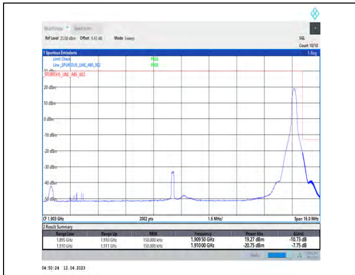
1-DC_5A_n2A-PC3-15-5+15-M+H-2-QPSK-Edge_1RB_Right-Edge_1_Right@N/A-DFT-PI2BPSK-Edge_1RB_Right-1@78-1-seegraph-PASS-see graph
