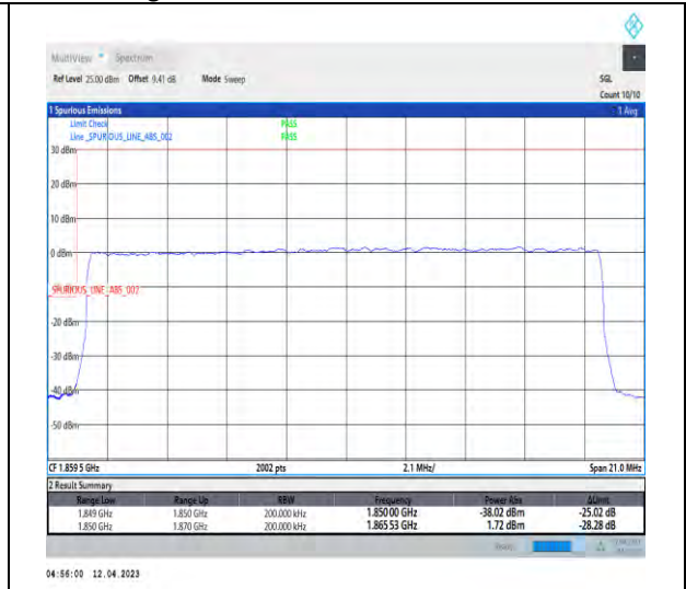
1-DC_5A_n2A-PC3-15-5+20-M+L-3-QPSK-Outer_Full-Outer_Full@N/A-DFT-PI2BPSK-Outer_Full-100@0-1-seegraph-PASS-see graph
