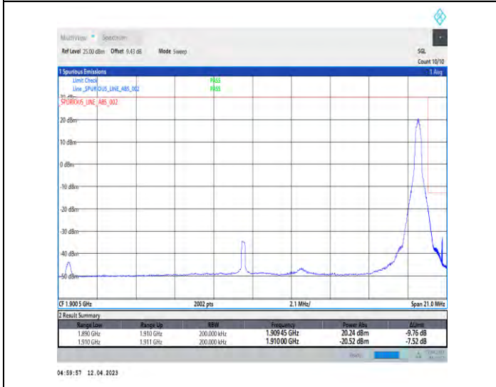
1-DC_5A_n2A-PC3-15-5+20-M+H-5-QPSK-Edge_1RB_Right-Edge_1_Right@N/A-CP-QPSK-Edge_1RB_Right-1@105-1-seegraph-PASS-see graph
