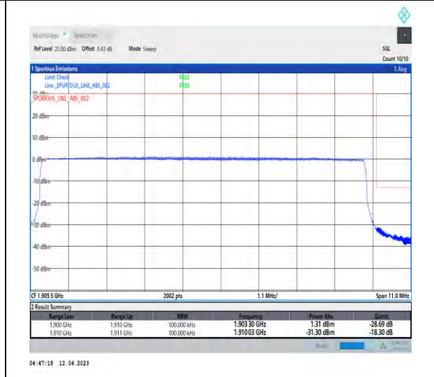
1-DC_5A_n2A-PC3-15-5+10-M+H-6-QPSK-Outer_Full-Outer_Full@N/A-CP-QPSK-Outer_Full-52@0-1-seegraph-PASS-see graph
