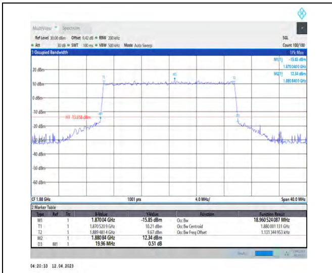
1-DC_5A_n2A-PC3-15-5+20-M+M-7-N/A-N/A-N/A-C P-16QAM-Outer_Full-106@0-Ant1-18.961-19.960-≤ 20-PASS
