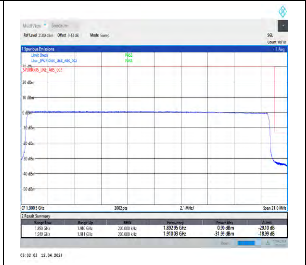
1-DC_5A_n2A-PC3-15-5+20-M+H-6-QPSK-Outer_Full-Outer_Full@N/A-CP-QPSK-Outer_Full-106@0-1-seegraph-PASS-see graph
