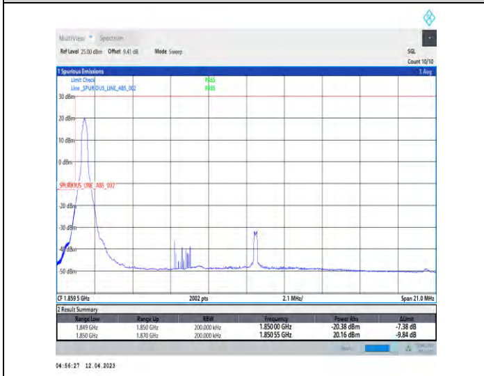
1-DC_5A_n2A-PC3-15-5+20-M+L-4-QPSK-Edge_1RB_Left-Edge_1_Left@N/A-CP-QPSK-Edge_1RB_Left-1@0-1-seegraph-PASS-see graph
