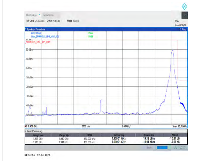
1-DC_5A_n2A-PC3-15-5+15-M+H-5-QPSK-Edge_1RB_Right-Edge_1_Right@N/A-CP-QPSK-Edge_1RB_Right-1@78-1-seegraph-PASS-see graph
