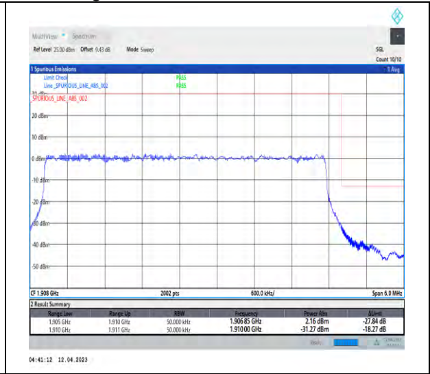
1-DC_5A_n2A-PC3-15-5+5-M+H-3-QPSK-Outer_Full-Outer_Full@N/A-DFT-PI2BPSK-Outer_Full-25@0-1-seegraph-PASS-see graph
