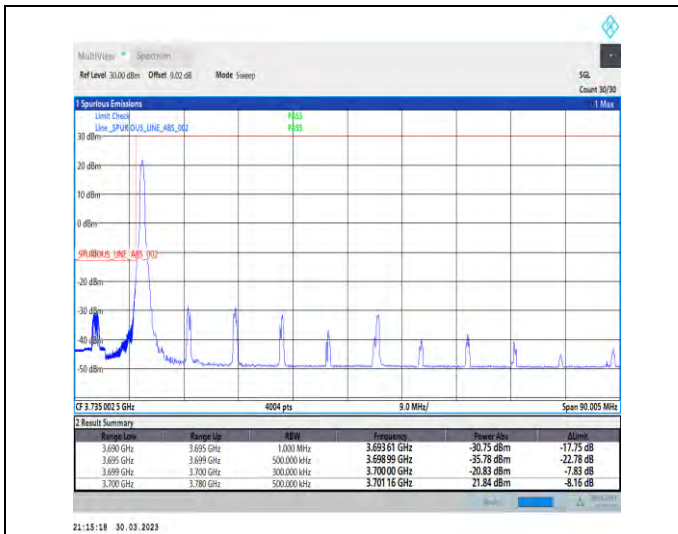
1-N77-3700-3980-30-80-L-1-DFT-PI2BPSK-Edge_1RB_Left-1@0-Ant1-1--PASS-see graph
