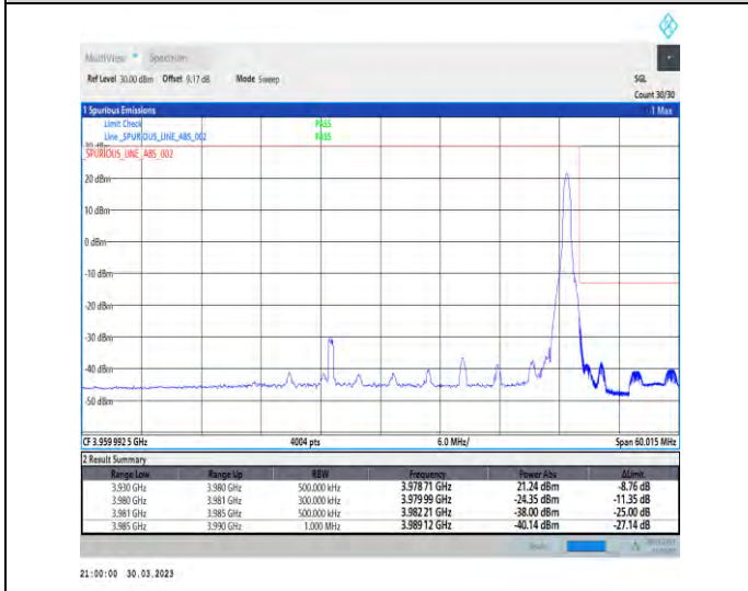
1-N77-3700-3980-30-50-H-5-CP-QPSK-Edge_1RB_Right-1@132-Ant1-1--PASS-see graph
