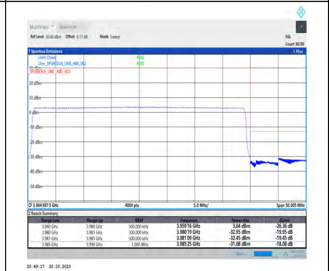
1-N77-3700-3980-30-40-H-6-CP-QPSK-Outer_Full-106@0-Ant1-1--PASS-see graph
