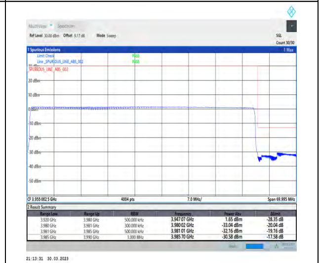
1-N77-3700-3980-30-60-H-6-CP-QPSK-Outer_Full-162@0-Ant1-1--PASS-see graph
