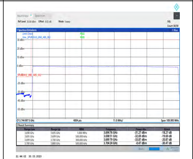
1-N77-3700-3980-30-100-L-6-CP-QPSK-Outer_Full-273@0-Ant1-1--PASS-see graph
