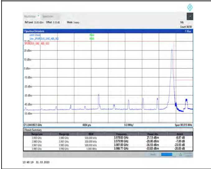
1-N77-3700-3980-30-80-H-5-CP-QPSK-Edge_1RB_Right-1@216-Ant1-1--PASS-see graph
