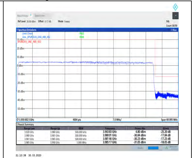
1-N77-3700-3980-30-60-H-3-DFT-PI2BPSK-Outer_Full-162@0-Ant1-1--PASS-see graph
