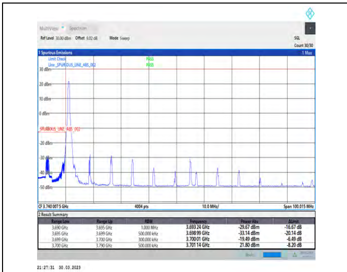
1-N77-3700-3980-30-90-L-1-DFT-PI2BPSK-Edge_1RB_Left-1@0-Ant1-1--PASS-see graph
