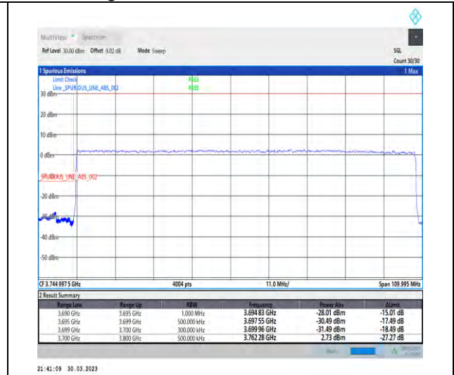
1-N77-3700-3980-30-100-L-3-DFT-PI2BPSK-Outer_Full-270@0-Ant1-1--PASS-see graph
