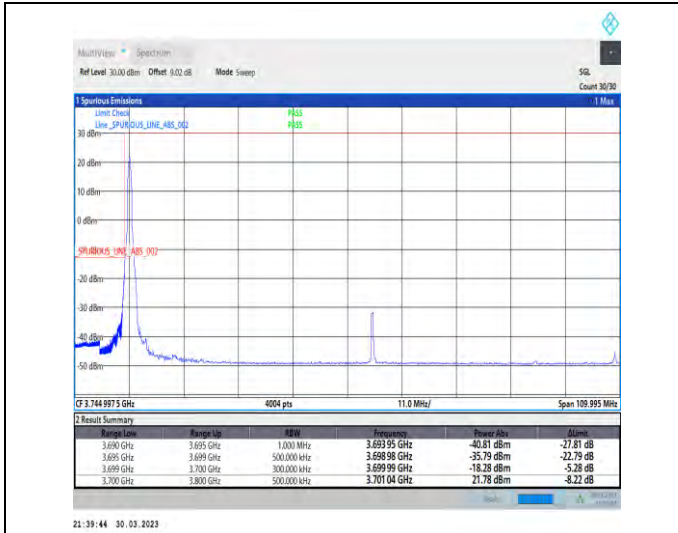
1-N77-3700-3980-30-100-L-1-DFT-PI2BPSK-Edge_1R_B_Left-1@0-Ant1-1--PASS-see graph
