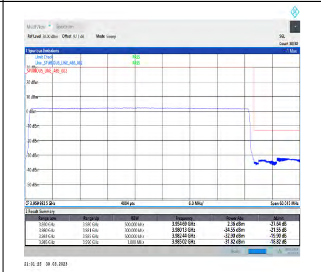
1-N77-3700-3980-30-50-H-6-CP-QPSK-Outer_Full-133@0-Ant1-1--PASS-see graph
