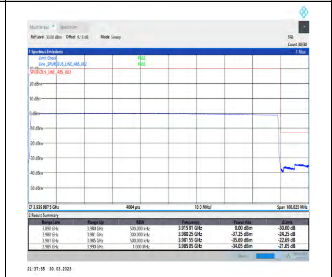
1-N77-3700-3980-30-90-H-6-CP-QPSK-Outer_Full-245@0-Ant1-1--PASS-see graph
