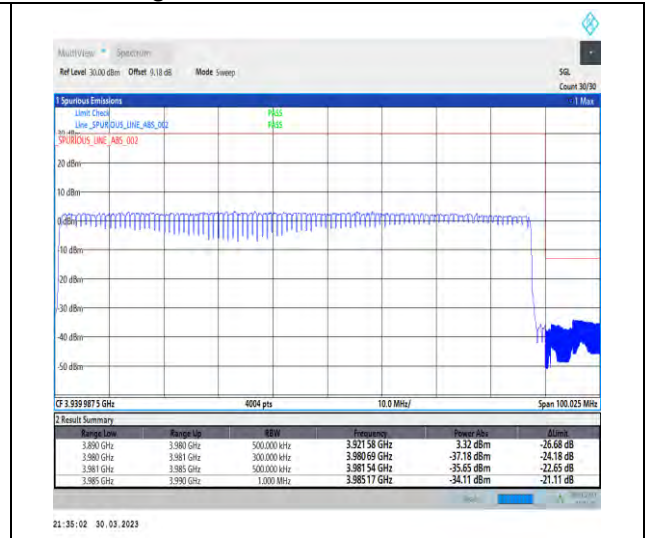
1-N77-3700-3980-30-90-H-3-DFT-PI2BPSK-Outer_Full-240@0-Ant1-1--PASS-see graph
