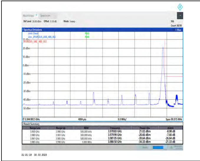
1-N77-3700-3980-30-80-H-2-DFT-PI2BPSK-Edge_1R_B_Right-1@216-Ant1-1--PASS-see graph
