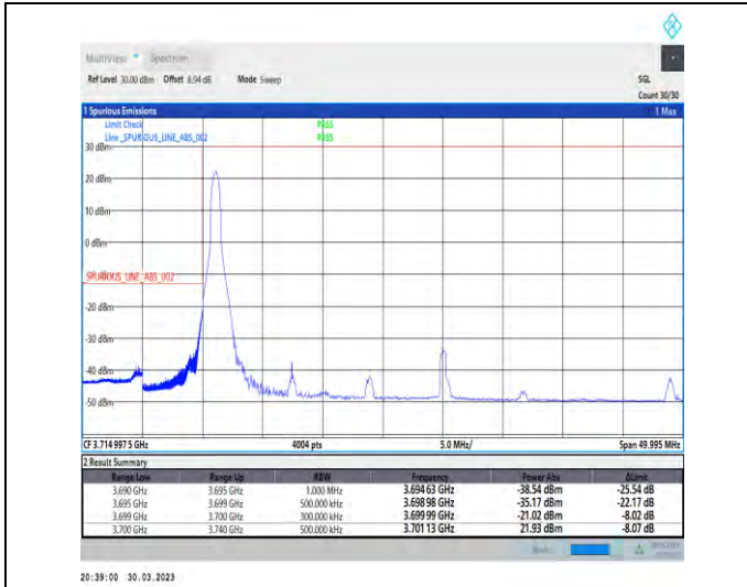
1-N77-3700-3980-30-40-L-1-DFT-PI2BPSK-Edge_1RB_Left-1@0-Ant1-1--PASS-see graph
