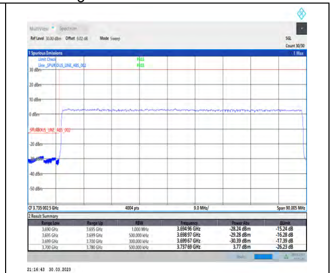
1-N77-3700-3980-30-80-L-3-DFT-PI2BPSK-Outer_Full-216@0-Ant1-1--PASS-see graph
