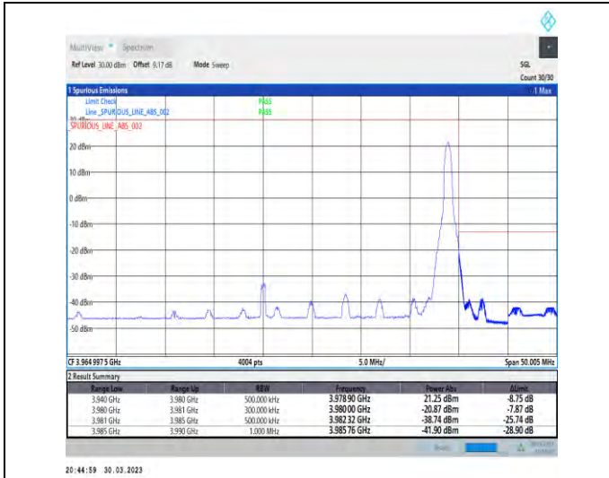
1-N77-3700-3980-30-40-H-2-DFT-PI2BPSK-Edge_1R_B_Right-1@105-Ant1-1--PASS-see graph
