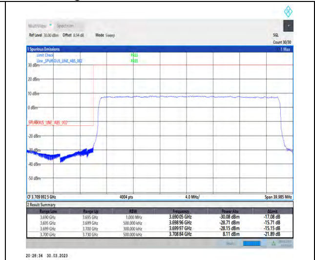
1-N77-3700-3980-30-30-L-3-DFT-PI2BPSK-Outer_Full-75@0-Ant1-1--PASS-see graph
