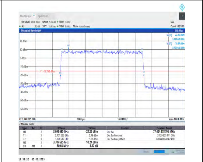
1-N77-3700-3980-30-80-L-9-CP-256QAM-Outer_Full-217@0-Ant1-77.424-80.640-≤80-PASS
