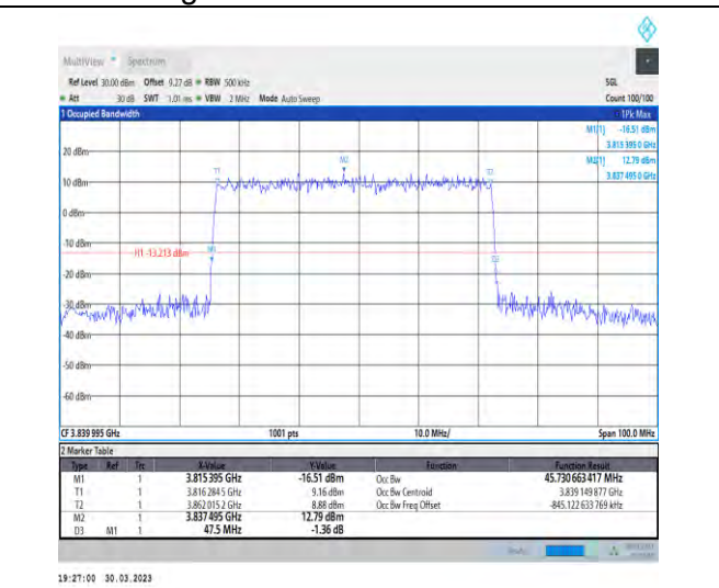
1-N77-3700-3980-30-50-M-4-DFT-64QAM-Outer_Ful I1-128@0-Ant1-45.731-47.500-≤50-PASS
