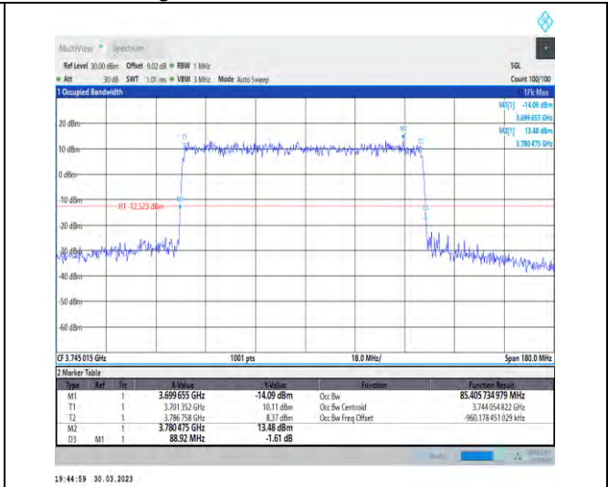
1-N77-3700-3980-30-90-L-4-DFT-64QAM-Outer_Full -240@0-Ant1-85.406-88.920-≤90-PASS
