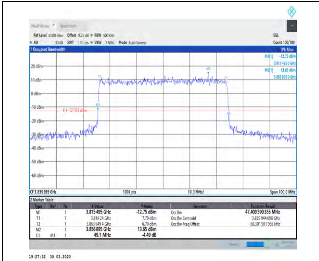
1-N77-3700-3980-30-50-M-7-CP-16QAM-Outer_Full -133@0-Ant1-47.409-49.100-≤50-PASS
