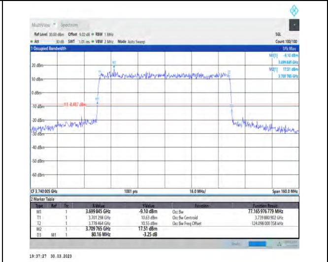
1-N77-3700-3980-30-80-L-1-DFT-QPSK-Outer_Full-216@0-Ant1-77.166-80.160-≤80-PASS
