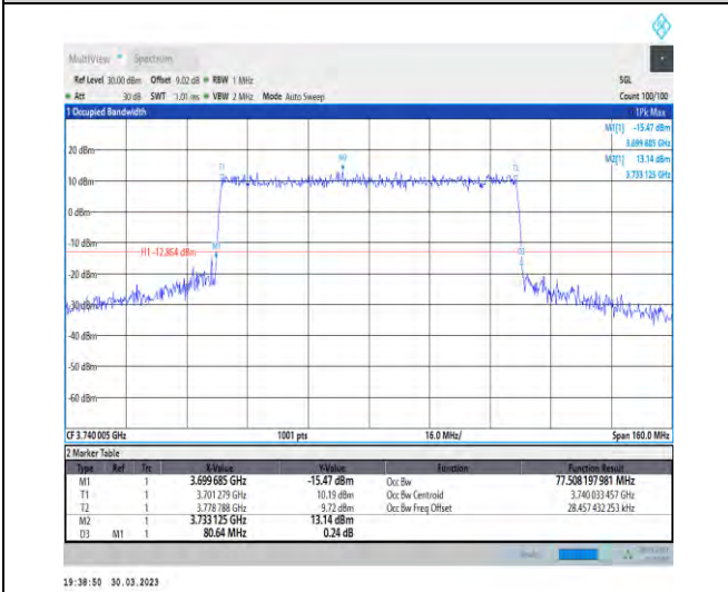
1-N77-3700-3980-30-80-L-8-CP-64QAM-Outer_Full-217@0-Ant1-77.508-80.640-≤80-PASS
