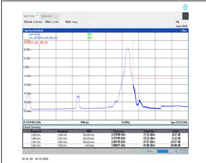
1-N77-3700-3980-30-20-H-2-DFT-PI2BPSK-Edge_1R_B_Right-1@50-Ant1-1--PASS-see graph
