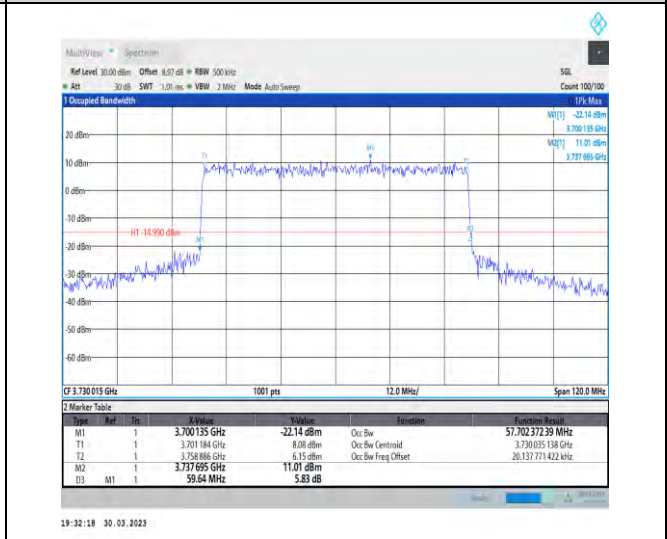
1-N77-3700-3980-30-60-L-8-CP-64QAM-Outer_Full-162@0-Ant1-57.702-59.640-≤60-PASS
