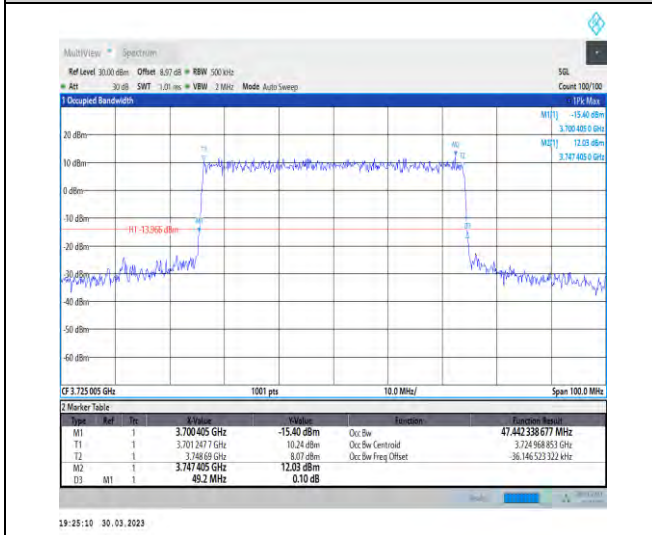
1-N77-3700-3980-30-50-L-6-CP-QPSK-Outer_Full-1 33@0-Ant1-47.442-49.200-≤50-PASS
