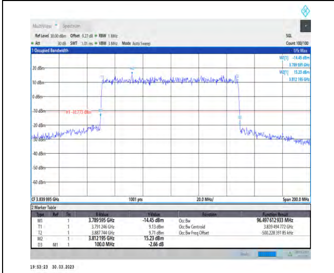
1-N77-3700-3980-30-100-M-1-DFT-QPSK-Outer_Ful I-270@0-Ant1-96.498-100.000-≤100-PASS
