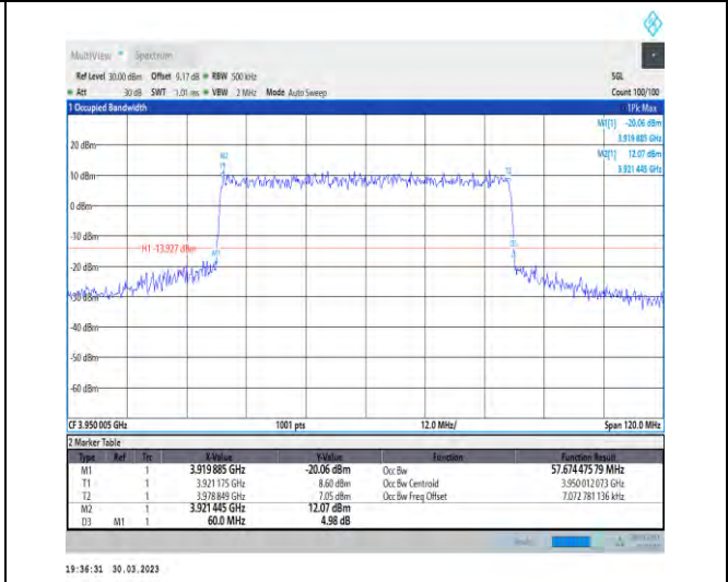
1-N77-3700-3980-30-60-H-6-CP-QPSK-Outer_Full-1 62@0-Ant1-57.674-60.000-≤60-PASS
