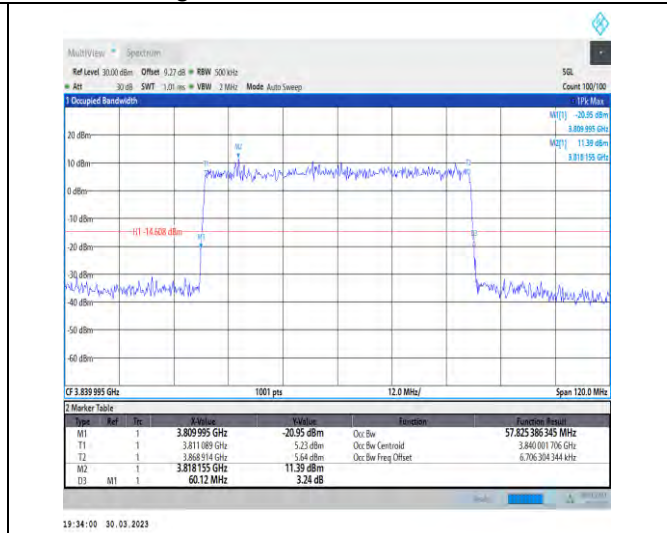
1-N77-3700-3980-30-60-M-5-DFT-256QAM-Outer_Full-162@0-Ant1-57.825-60.120-≤60-PASS
