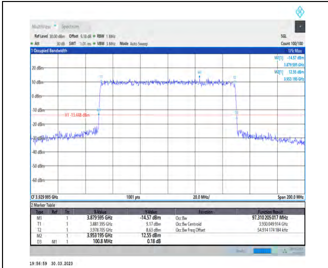
1-N77-3700-3980-30-100-H-6-CP-QPSK-Outer_Full-273@0-Ant1-97.31-100.800-≤100-PASS
