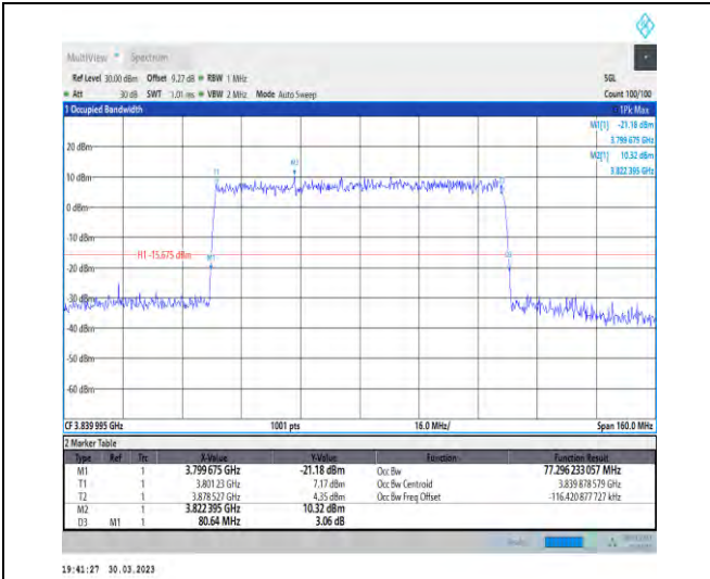
1-N77-3700-3980-30-80-M-9-CP-256QAM-Outer_Fu II-217@0-Ant1-77.296-80.640-≤80-PASS
