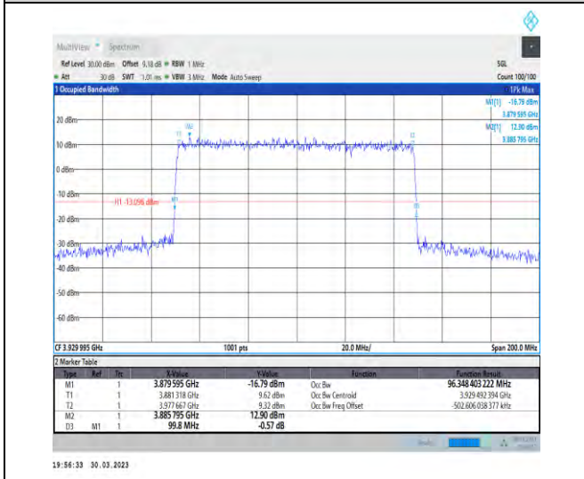
1-N77-3700-3980-30-100-H-4-DFT-64QAM-Outer_Full-270@0-Ant1-96.348-99.800-≤100-PASS
