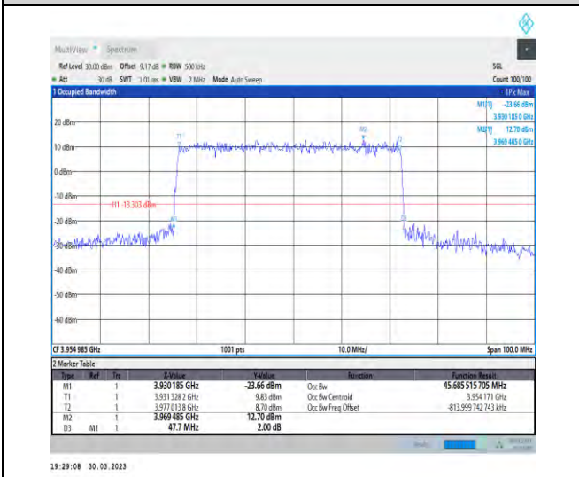
1-N77-3700-3980-30-50-H-4-DFT-64QAM-Outer_Full-128@0-Ant1-45.686-47.700-≤50-PASS
