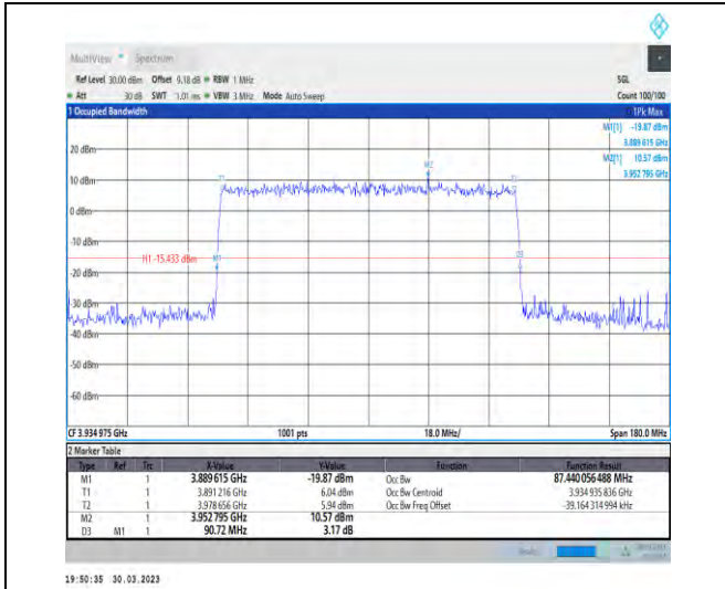
1-N77-3700-3980-30-90-H-9-CP-256QAM-Outer_Ful I-245@0-Ant1-87.44-90.720-<=90-PASS
