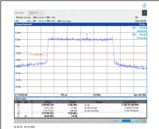
1-N77-3700-3980-30-80-L-6-CP-QPSK-Outer_Full-2 17@0-Ant1-77.385-80.640-≤80-PASS
