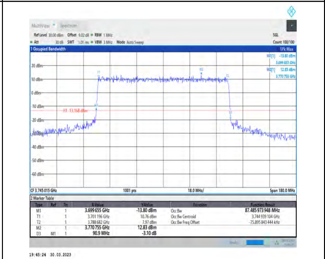
1-N77-3700-3980-30-90-L-6-CP-QPSK-Outer_Full-2 45@0-Ant1-87.486-90.900-≤90-PASS
