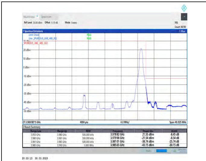
1-N77-3700-3980-30-30-H-2-DFT-PI2BPSK-Edge_1R_B_Right-1@77-Ant1-1--PASS-see graph
