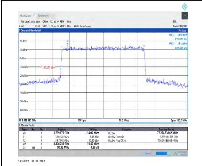
1-N77-3700-3980-30-80-M-3-DFT-16QAM-Outer_Full-216@0-Ant1-77.275-80.320-≤80-PASS
