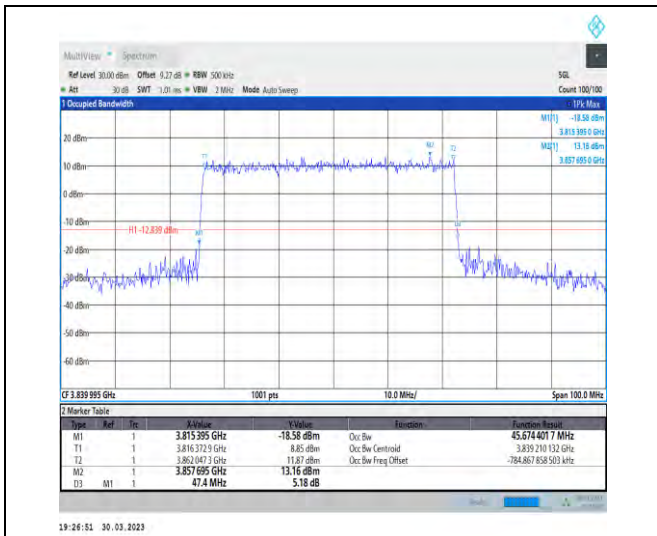
1-N77-3700-3980-30-50-M-3-DFT-16QAM-Outer_Fu I1-128@0-Ant1-45.674-47.400-≤50-PASS
