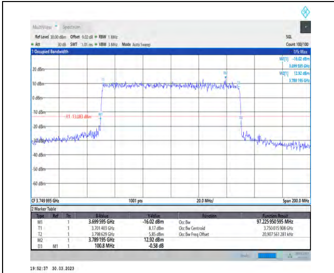
1-N77-3700-3980-30-100-L-8-CP-64QAM-Outer_Ful I-273@0-Ant1-97.226-100.800-≤100-PASS
