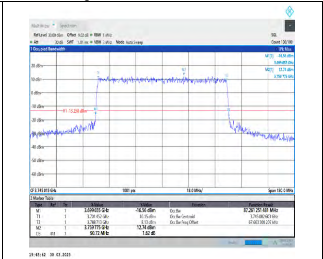
1-N77-3700-3980-30-90-L-8-CP-64QAM-Outer_Full-245@0-Ant1-87.261-90.720-≤90-PASS
