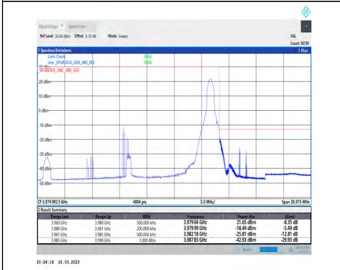
1-N77-3700-3980-30-20-H-5-CP-QPSK-Edge_1RB_Right-1@50-Ant1-1--PASS-see graph
