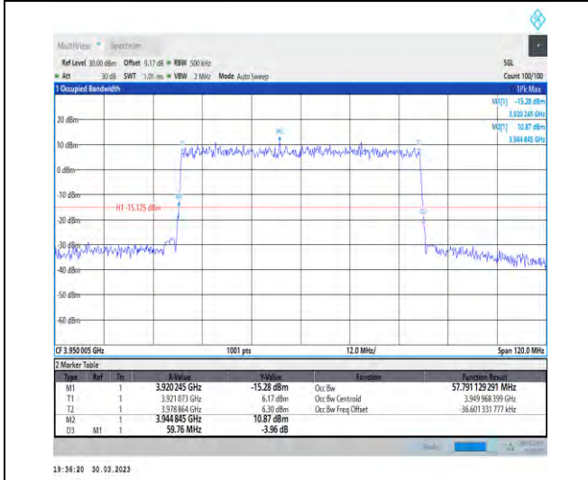
1-N77-3700-3980-30-60-H-5-DFT-256QAM-Outer_Full ull-162@0-Ant1-57.791-59.760-≤60-PASS
