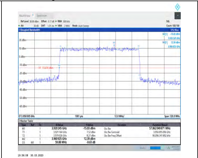
1-N77-3700-3980-30-60-H-4-DFT-64QAM-Outer_Full -162@0-Ant1-57.862-59.880-≤60-PASS
