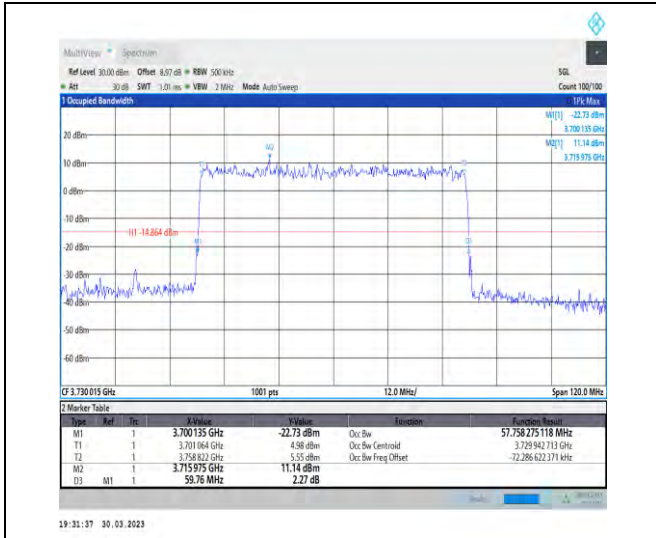
1-N77-3700-3980-30-60-L-5-DFT-256QAM-Outer_Full-162@0-Ant1-57.758-59.760-≤60-PASS
