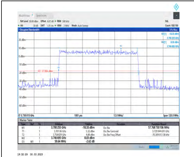
1-N77-3700-3980-30-60-L-9-CP-256QAM-Outer_Ful I-162@0-Ant1-57.769-59.640-≤60-PASS
