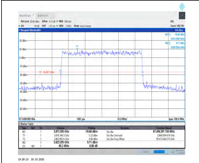
1-N77-3700-3980-30-50-M-9-CP-256QAM-Outer_Fu II-133@0-Ant1-47.496-49.200-≤50-PASS
