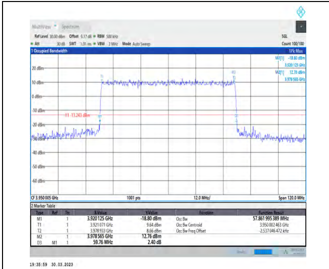
1-N77-3700-3980-30-60-H-3-DFT-16QAM-Outer_Full I-162@0-Ant1-57.862-59.760-≤60-PASS
