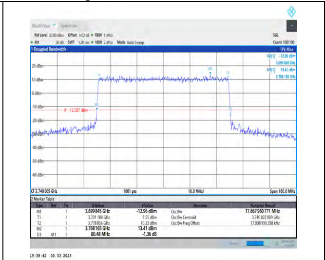
1-N77-3700-3980-30-80-L-7-CP-16QAM-Outer_Full-217@0-Ant1-77.668-80.480-≤80-PASS
