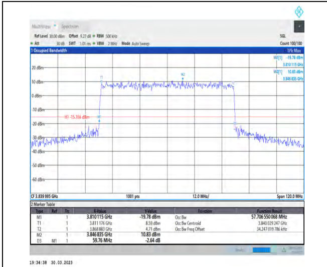
1-N77-3700-3980-30-60-M-8-CP-64QAM-Outer_Full -162@0-Ant1-57.707-59.760-≤60-PASS
