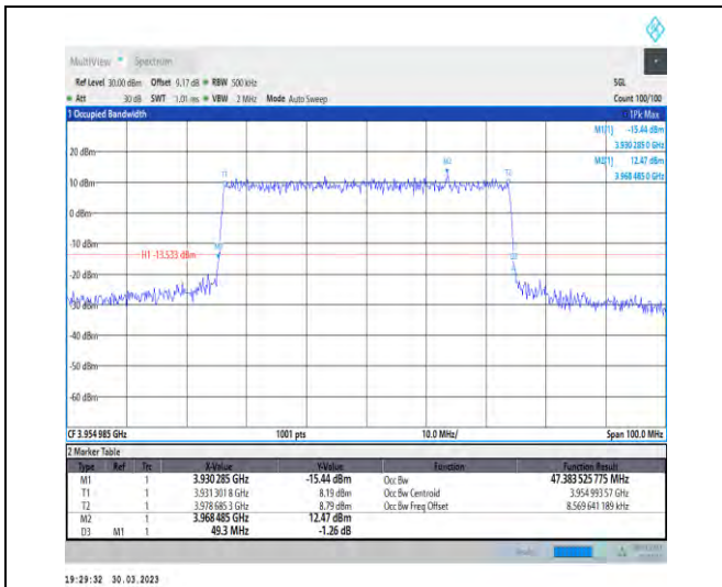
1-N77-3700-3980-30-50-H-6-CP-QPSK-Outer_Full-1 33@0-Ant1-47.384-49.300-≤50-PASS
