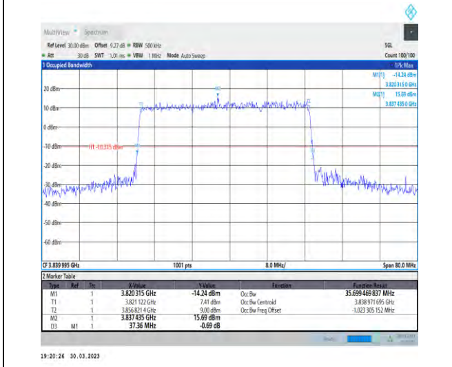
1-N77-3700-3980-30-40-M-4-DFT-64QAM-Outer_Full-100@0-Ant1-35.699-37.360-<=40-PASS
