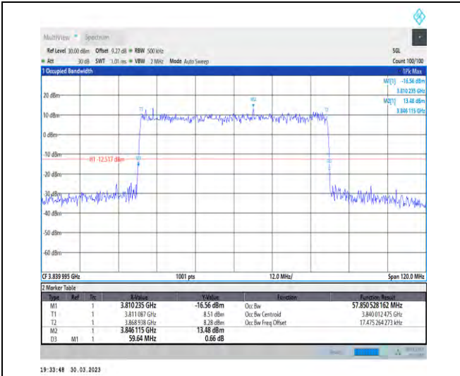
1-N77-3700-3980-30-60-M-4-DFT-64QAM-Outer_Fu II-162@0-Ant1-57.851-59.640-≤60-PASS
