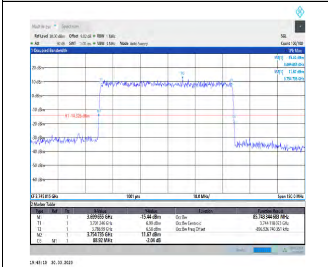
1-N77-3700-3980-30-90-L-5-DFT-256QAM-Outer_Full -240@0-Ant1-85.743-88.920-≤90-PASS
