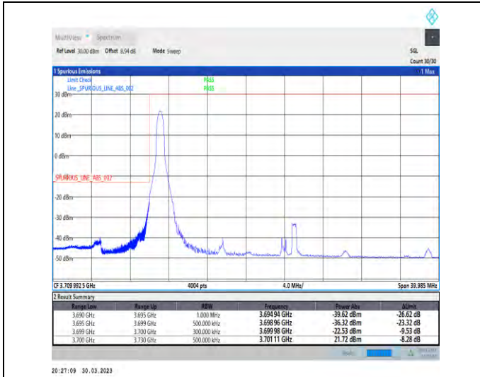
1-N77-3700-3980-30-30-L-1-DFT-PI2BPSK-Edge_1RB_Left-1@0-Ant1-1--PASS-see graph
