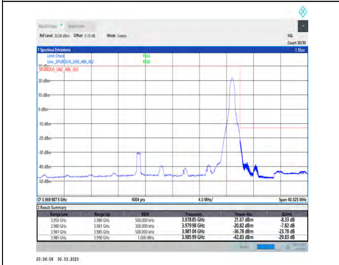
1-N77-3700-3980-30-30-H-5-CP-QPSK-Edge_1RB_Right-1@77-Ant1-1--PASS-see graph
