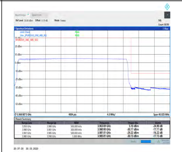
1-N77-3700-3980-30-30-H-6-CP-QPSK-Outer_Full-78@0-Ant1-1--PASS-see graph
