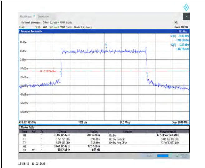
1-N77-3700-3980-30-100-M-7-CP-16QAM-Outer_Full-273@0-Ant1-97.575-101.200-≤100-PASS
