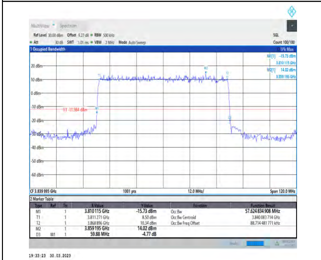
1-N77-3700-3980-30-60-M-2-DFT-PI2BPSK-Outer_Full Full-162@0-Ant1-57.625-59.880-≤60-PASS
