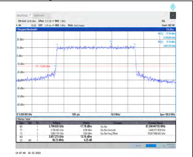
1-N77-3700-3980-30-90-M-7-CP-16QAM-Outer_Full-245@0-Ant1-87.34-90.720-<90-PASS
