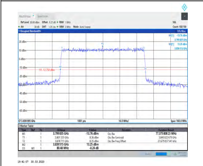
1-N77-3700-3980-30-80-M-7-CP-16QAM-Outer_Full-217@0-Ant1-77.376-80.480-<math>\leq 80</math>-PASS
