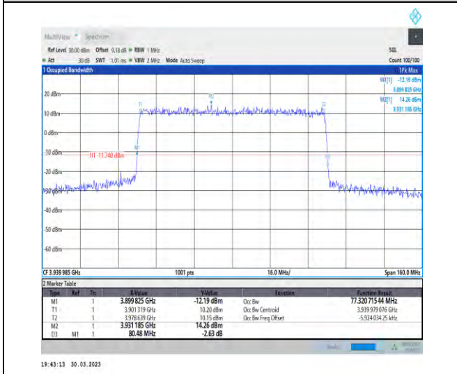
1-N77-3700-3980-30-80-H-6-CP-QPSK-Outer_Full-217@0-Ant1-77.321-80.480-≤80-PASS
