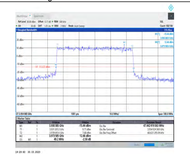
1-N77-3700-3980-30-50-H-7-CP-16QAM-Outer_Full-133@0-Ant1-47.442-49.200-≤50-PASS
