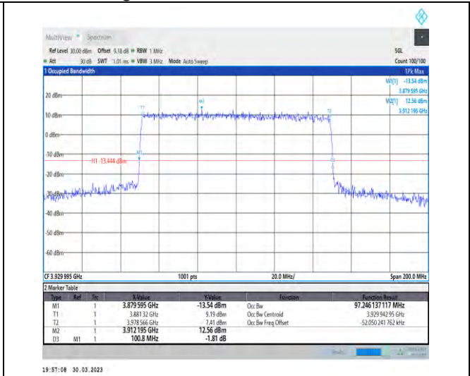
1-N77-3700-3980-30-100-H-7-CP-16QAM-Outer_Full-273@0-Ant1-97.246-100.800-≤100-PASS
