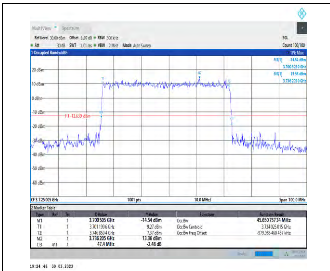
1-N77-3700-3980-30-50-L-4-DFT-64QAM-Outer_Full -128@0-Ant1-45.651-47.400-≤50-PASS
