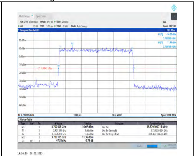
1-N77-3700-3980-30-50-L-5-DFT-256QAM-Outer_Fu ll-128@0-Ant1-45.579-47.300-≤50-PASS
