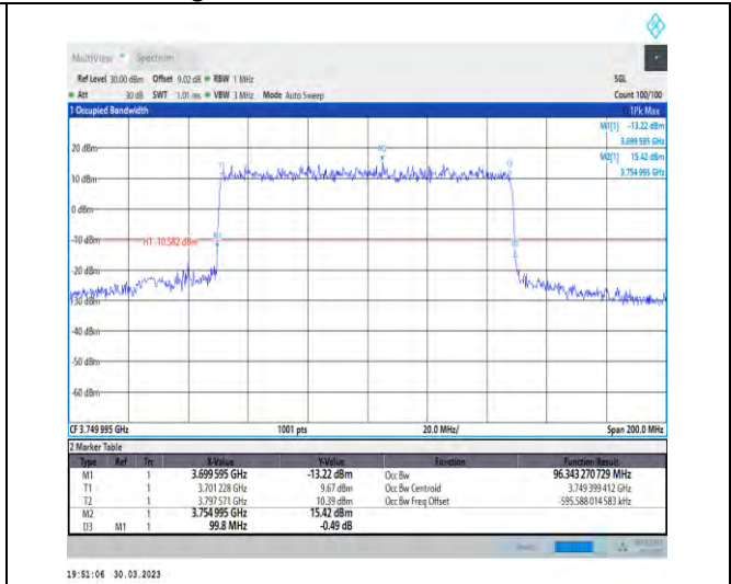
1-N77-3700-3980-30-100-L-1-DFT-QPSK-Outer_Full -270@0-Ant1-96.343-99.800-<=100-PASS
