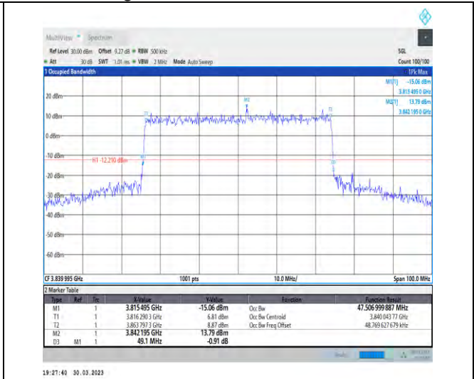
1-N77-3700-3980-30-50-M-8-CP-64QAM-Outer_Full -133@0-Ant1-47.507-49.100-≤50-PASS
