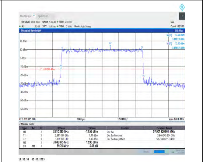
1-N77-3700-3980-30-60-M-3-DFT-16QAM-Outer_Full I-162@0-Ant1-57.902-59.760-≤60-PASS
