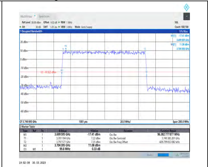
1-N77-3700-3980-30-100-L-5-DFT-256QAM-Outer_Full-270@0-Ant1-96.383-99.800-≤100-PASS
