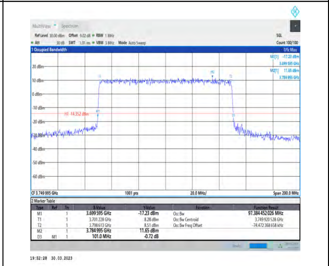
1-N77-3700-3980-30-100-L-7-CP-16QAM-Outer_Full-273@0-Ant1-97.384-101.000-≤100-PASS
