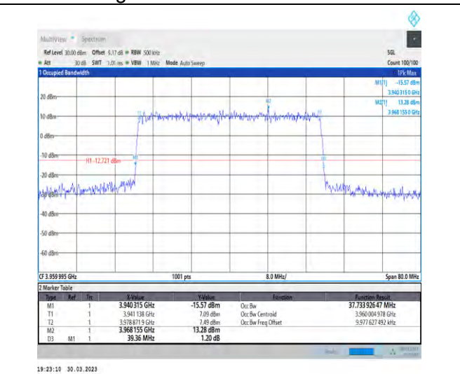
1-N77-3700-3980-30-40-H-6-CP-QPSK-Outer_Full-106@0-Ant1-37.734-39.360-<math>\leq 40</math>-PASS
