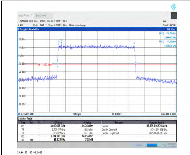
1-N77-3700-3980-30-90-L-3-DFT-16QAM-Outer_Full -240@0-Ant1-85.595-88.920-≤90-PASS
