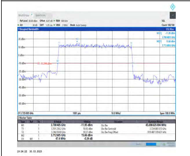
1-N77-3700-3980-30-50-L-2-DFT-PI2BPSK-Outer_Full-128@0-Ant1-45.699-47.400-≤50-PASS
