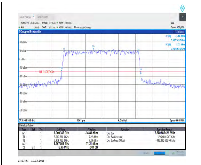
1-N77-3700-3980-30-20-H-3-DFT-16QAM-Outer_Full I-50@0-Ant1-17.841-18.960-<20-PASS
