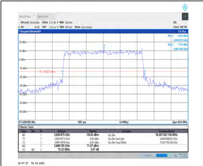
1-N77-3700-3980-30-20-M-8-CP-64QAM-Outer_Full -51@0-Ant1-18.202-19.320-≤20-PASS
