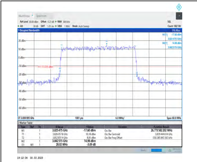
1-N77-3700-3980-30-30-M-1-DFT-QPSK-Outer_Full-75@0-Ant1-26.774-28.020-≤30-PASS
