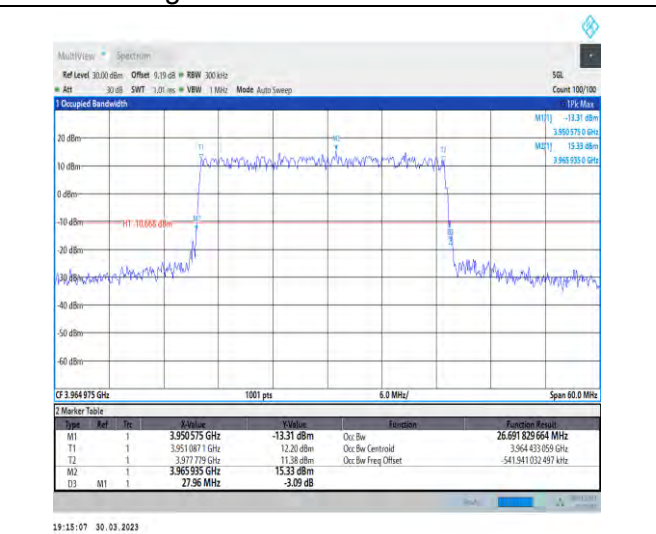
1-N77-3700-3980-30-30-H-1-DFT-QPSK-Outer_Full-75@0-Ant1-26.692-27.960-<30-PASS
