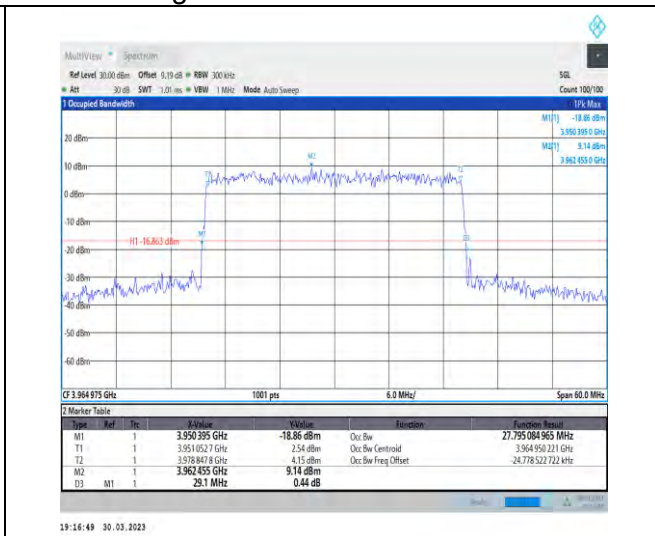
1-N77-3700-3980-30-30-H-9-CP-256QAM-Outer_Full-78@0-Ant1-27.795-29.100-≤30-PASS
