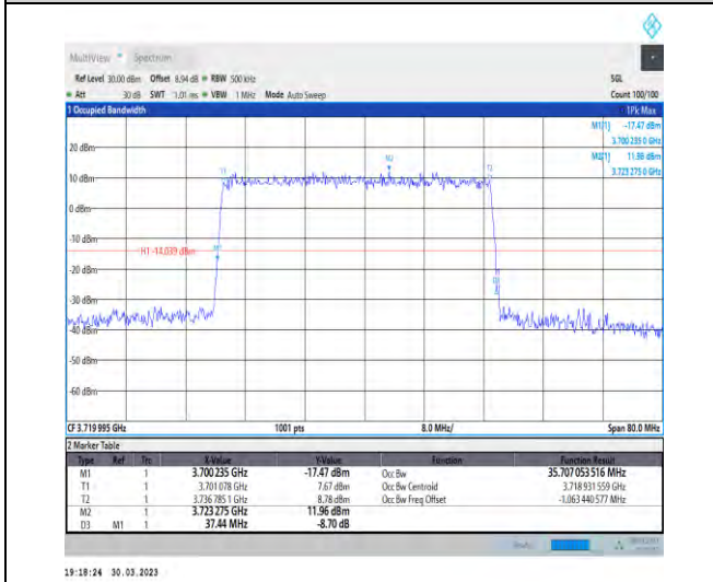
1-N77-3700-3980-30-40-L-5-DFT-256QAM-Outer_Full -100@0-Ant1-35.707-37.440-≤40-PASS
