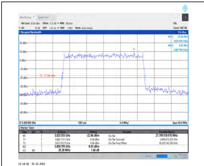
1-N77-3700-3980-30-30-M-9-CP-256QAM-Outer_Fu ll-78@0-Ant1-27.799-29.280-<30-PASS
