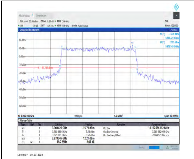
1-N77-3700-3980-30-20-H-7-CP-16QAM-Outer_Full-51@0-Ant1-18.193-19.200-≤20-PASS
