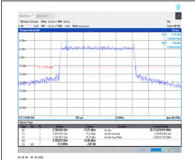
1-N77-3700-3980-30-40-L-3-DFT-16QAM-Outer_Full -100@0-Ant1-35.713-37.600-≤40-PASS
