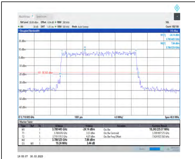
1-N77-3700-3980-30-20-L-9-CP-256QAM-Outer_Ful I-51@0-Ant1-18.243-19.240-<=20-PASS
