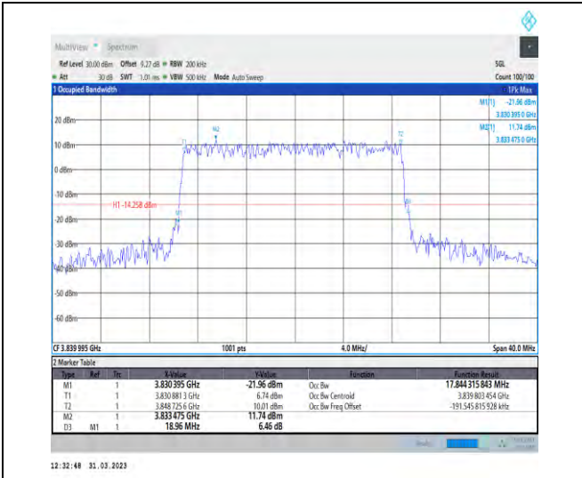
1-N77-3700-3980-30-20-M-4-DFT-64QAM-Outer_Fu ll-50@0-Ant1-17.844-18.960-<math>\leq 20</math>-PASS
