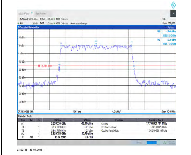
1-N77-3700-3980-30-20-M-2-DFT-PI2BPSK-Outer_Full-50@0-Ant1-17.798-18.840-<=20-PASS
