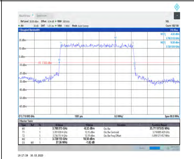
1-N77-3700-3980-30-40-L-2-DFT-PI2BPSK-Outer_Full-100@0-Ant1-35.712-37.360-≤40-PASS
