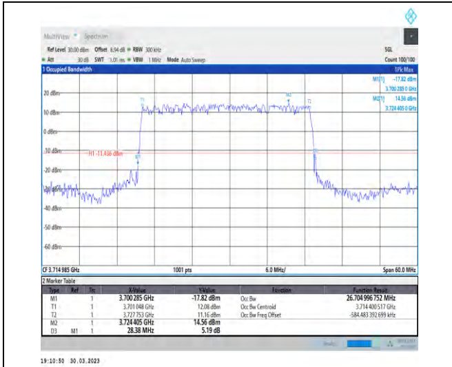
1-N77-3700-3980-30-30-L-2-DFT-PI2BPSK-Outer_Full-75@0-Ant1-26.705-28.380-≤30-PASS
