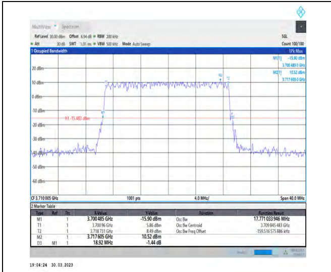
1-N77-3700-3980-30-20-L-5-DFT-256QAM-Outer_Full-50@0-Ant1-17.771-18.920-≤20-PASS
