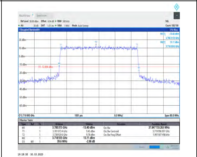
1-N77-3700-3980-30-40-L-6-CP-QPSK-Outer_Full -106@0-Ant1-37.847-39.600-≤40-PASS
