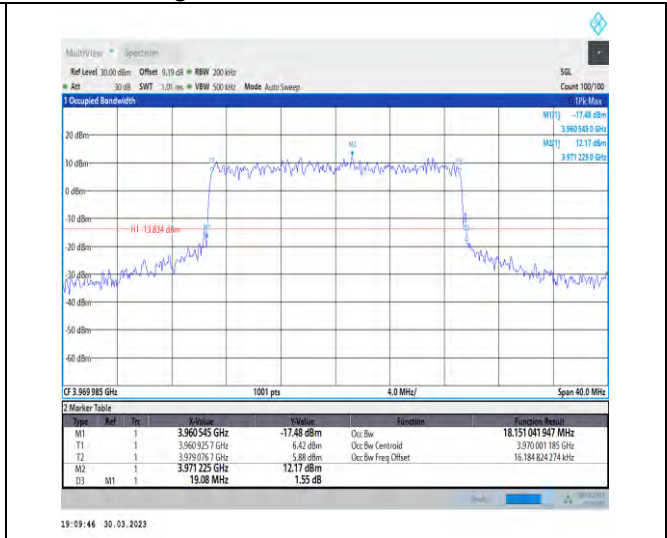
1-N77-3700-3980-30-20-H-8-CP-64QAM-Outer_Full-51@0-Ant1-18.151-19.080-≤20-PASS
