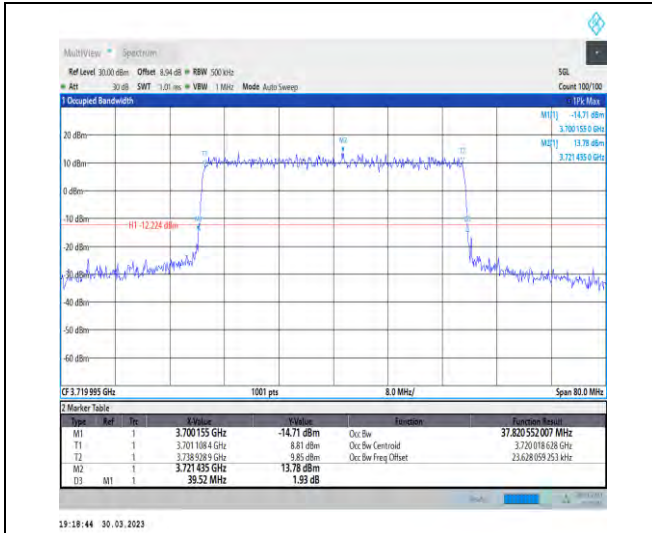
1-N77-3700-3980-30-40-L-7-CP-16QAM-Outer_Full-106@0-Ant1-37.821-39.520-≤40-PASS
