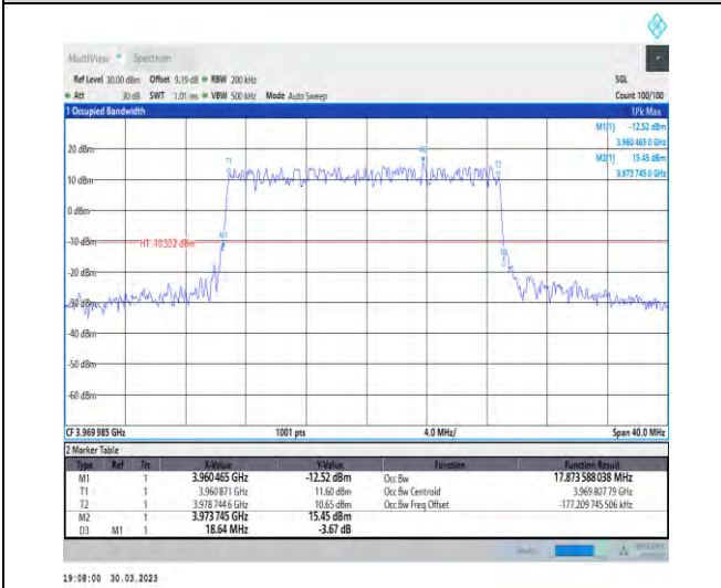
1-N77-3700-3980-30-20-H-1-DFT-QPSK-Outer_Full-50@0-Ant1-17.874-18.640-≤20-PASS
