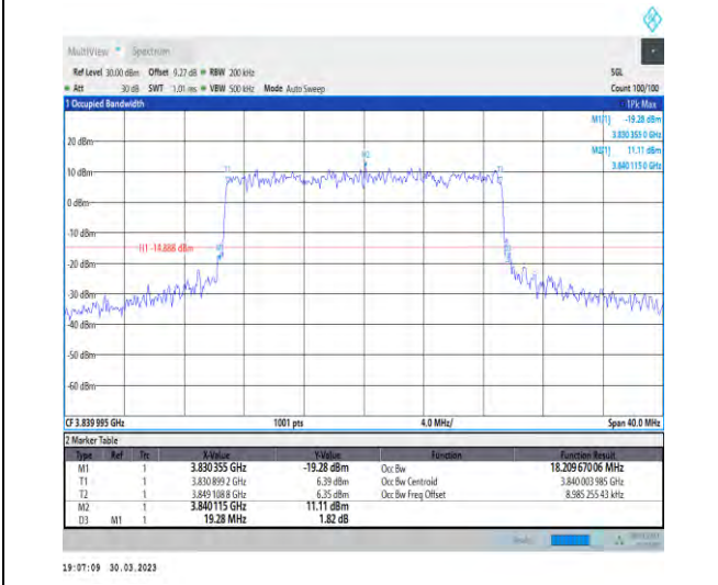
1-N77-3700-3980-30-20-M-6-CP-QPSK-Outer_Full- 51@0-Ant1-18.21-19.280-<math>\leq 20</math>-PASS
