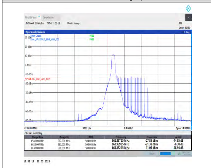
1-N71-15-5-L-4-CP-QPSK-Edge_1RB_Left-1@0-Ant1-1--PASS-see graph
