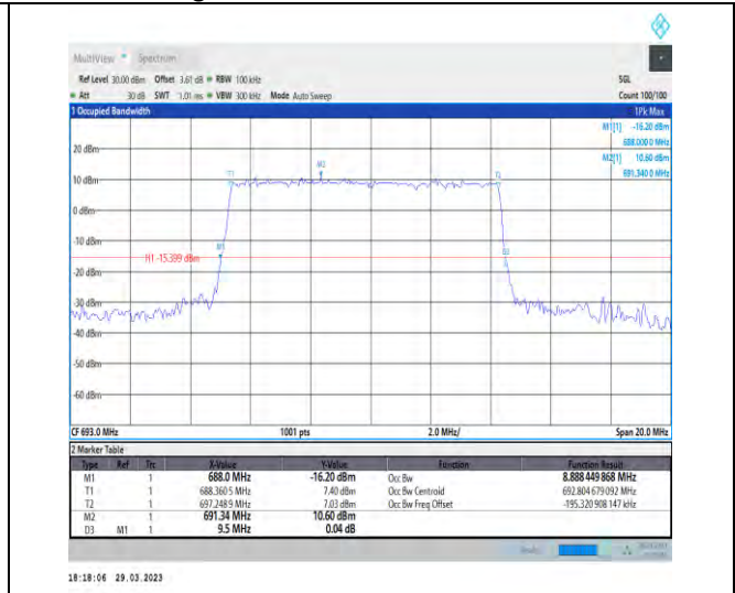
1-N71-15-10-H-5-DFT-256QAM-Outer_Full-50@0-A nt1-8.888-9.500≤10-PASS
