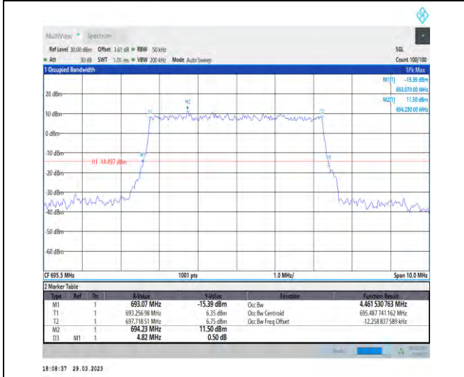
1-N71-15-5-H-5-DFT-256QAM-Outer_Full-25@0-Ant 1-4.462-4.820-≤5-PASS
