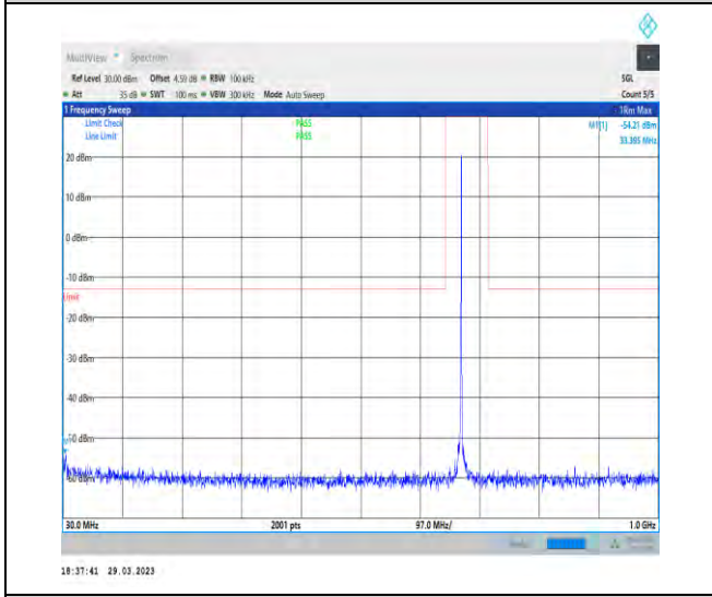
1-N71-15-20-H-1-DFT-PI2BPSK-Inner_1RB_Left-1 @ 1-30-1000-Ant1-33.40--54.21--13-PASS
