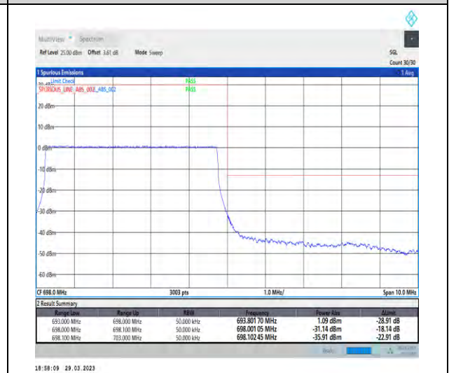
1-N71-15-5-H-6-CP-QPSK-Outer_Full-25@0-Ant1 -1--PASS-see graph
