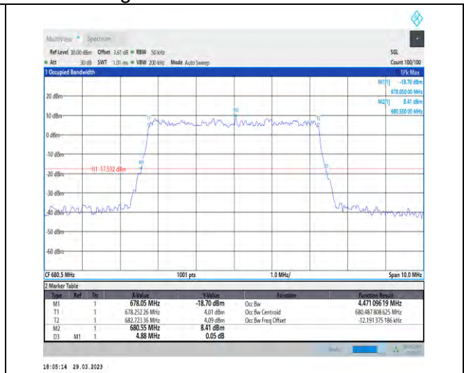
1-N71-15-5-M-5-DFT-256QAM-Outer_Full-25@0-Ant 1-4.471-4.880-≤5-PASS
