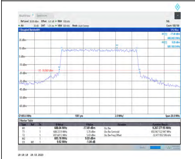
1-N71-15-10-H-6-CP-QPSK-Outer_Full-52@0-Ant1 9.267-9.920≤10-PASS
