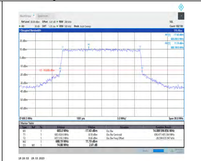
1-N71-15-15-H-6-CP-QPSK-Outer_Full-79@0-Ant1- 14.09-14.880-≤15-PASS
