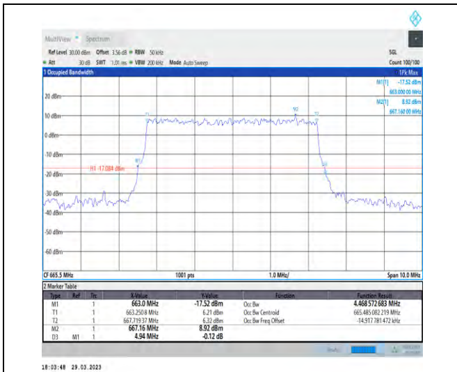
1-N71-15-5-L-9-CP-256QAM-Outer_Full-25@0-Ant1 -4.469-4.940-≤5-PASS
