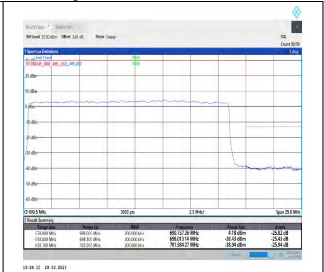
1-N71-15-20-H-3-DFT-PI2BPSK-Outer_Full-100@0-Ant1-1--PASS-see graph
