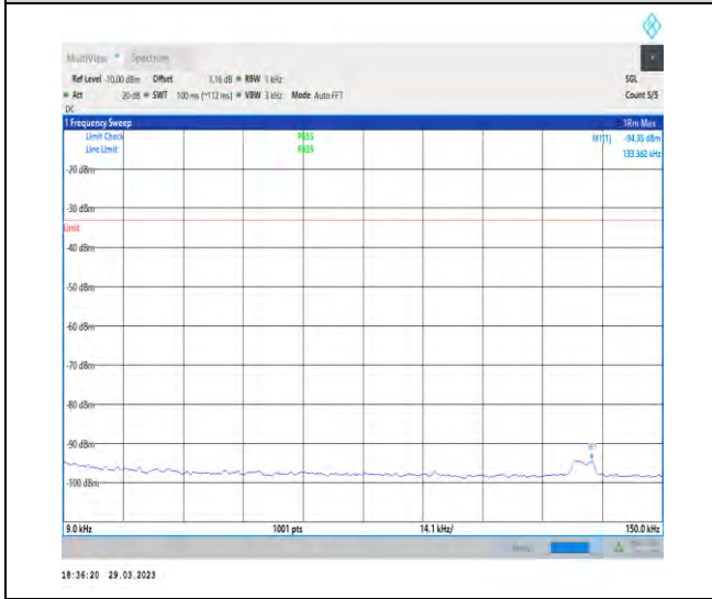
1-N71-15-20-M-1-DFT-PI2BPSK-Inner_1RB_Left-1 @ 1-0.009-0.15-Ant1-0.13--94.35--33-PASS
