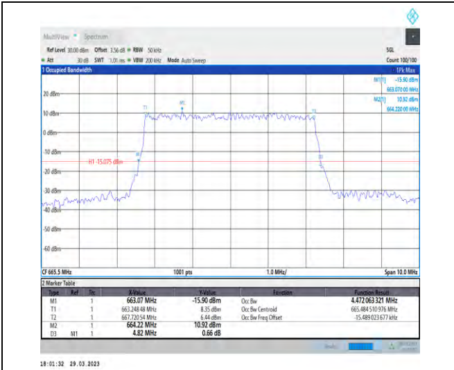
1-N71-15-5-L-5-DFT-256QAM-Outer_Full-25@0-Ant 1-4.472-4.820-≤5-PASS
