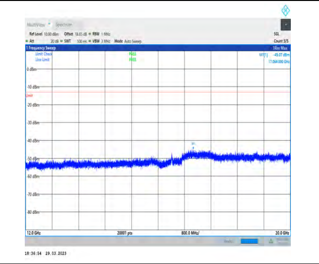
1-N71-15-20-M-1-DFT-PI2BPSK-Inner_1RB_Left-1@ 1-12000-20000-Ant1-17064.00--45.07--13-PASS
