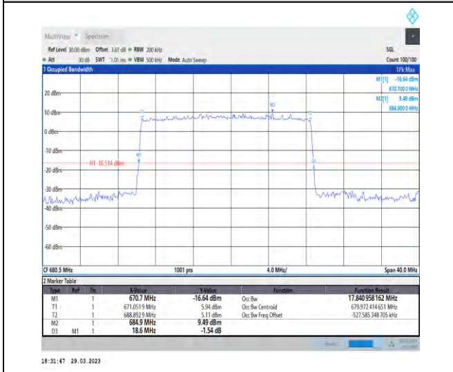
1-N71-15-20-M-5-DFT-256QAM-Outer_Full-100@0-A Ant1-17.841-18.600-≤20-PASS
