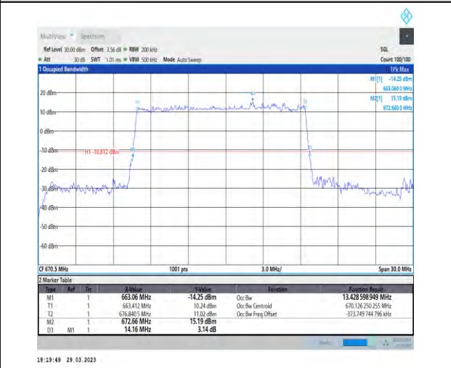
1-N71-15-15-L-2-DFT-PI2BPSK-Outer_Full-75@0-A nt1-13.429-14.160-≤15-PASS
