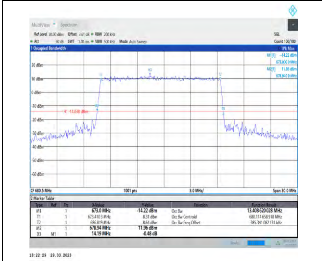
1-N71-15-15-M-4-DFT-64QAM-Outer_Full-75@0-Ant 1-13.409-14.190-≤15-PASS
