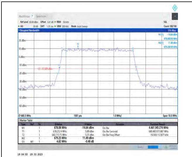
1-N71-15-5-M-4-DFT-64QAM-Outer_Full-25@0-Ant1 -4.461-4.820-≤5-PASS
