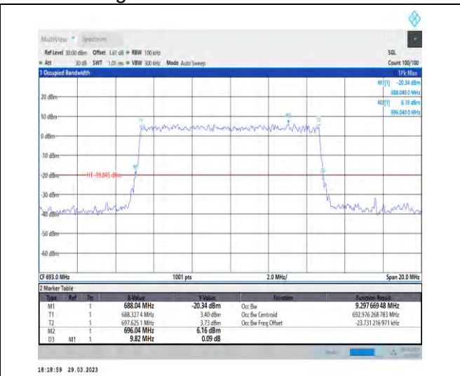
1-N71-15-10-H-9-CP-256QAM-Outer_Full-52@0-Ant 1-9.298-9.820-≤10-PASS
