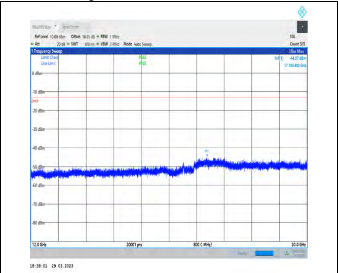
1-N71-15-20-H-1-DFT-PI2BPSK-Inner_1RB_Left-1@ 1-12000-20000-Ant1-17104.40--44.97--13-PASS
