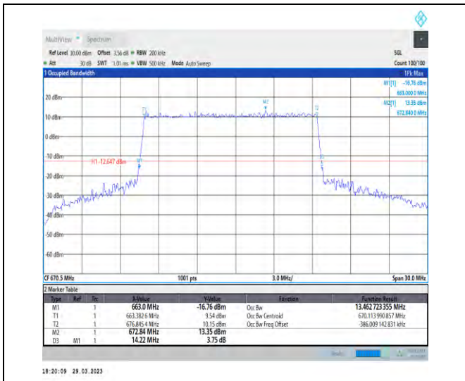
1-N71-15-15-L-3-DFT-16QAM-Outer_Full-75@0-Ant 1-13.463-14.220-≤15-PASS
