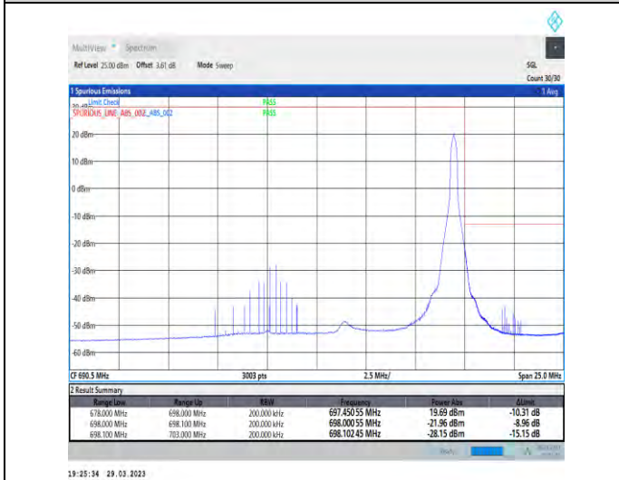
1-N71-15-20-H-5-CP-QPSK-Edge_1RB_Right-1@105-Ant1-1--PASS-see graph
