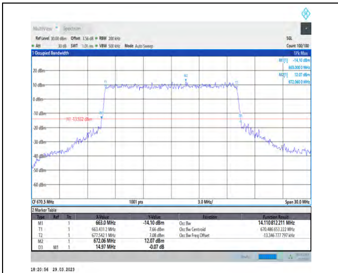
1-N71-15-15-L-7-CP-16QAM-Outer_Full-79@0-Ant1 -14.111-14.970-≤15-PASS
