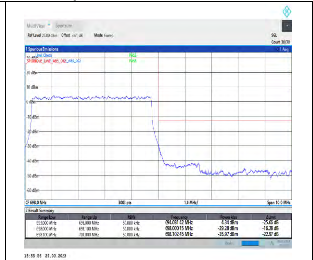
1-N71-15-5-H-3-DFT-PI2BPSK-Outer_Full-25@0- Ant1-1--PASS-see graph
