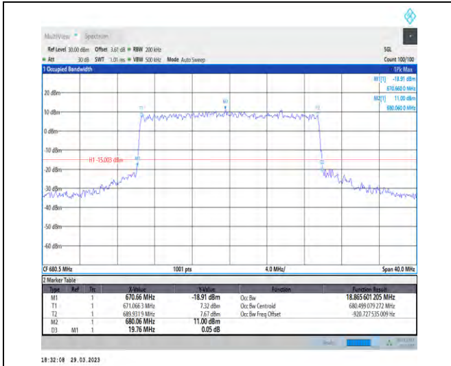
1-N71-15-20-M-7-CP-16QAM-Outer_Full-106@0-An t1-18.866-19.760-≤20-PASS
