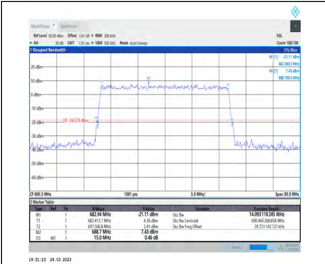
1-N71-15-15-H-9-CP-256QAM-Outer_Full-79@0-Ant 1-14.093-15.000-≤15-PASS
