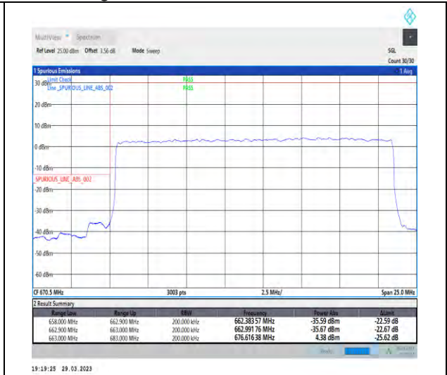
1-N71-15-20-L-3-DFT-PI2BPSK-Outer_Full-100@0-Ant1-1--PASS-see graph
