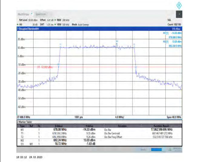
1-N71-15-20-H-1-DFT-QPSK-Outer_Full-100@0-Ant 1-17.863-18.720-≤20-PASS
