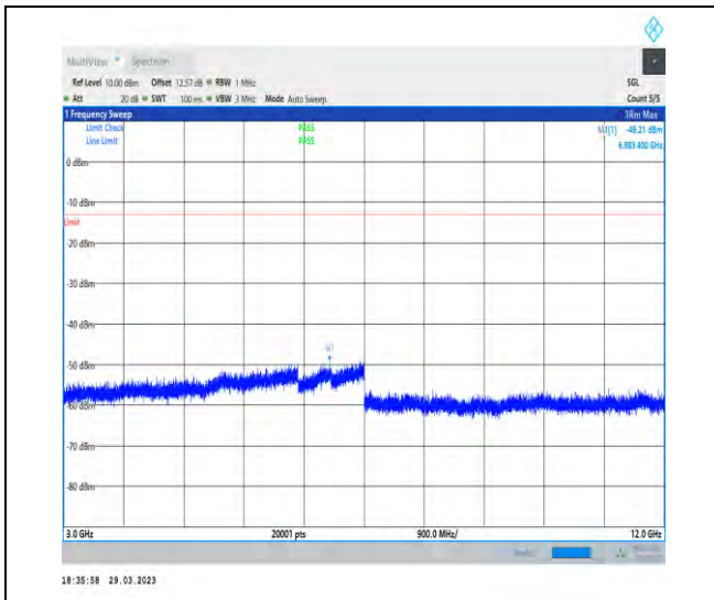
1-N71-15-20-L-1-DFT-PI2BPSK-Inner_1RB_Left-1 @ 1-3000-12000-Ant1-6983.40--49.21--13-PASS
