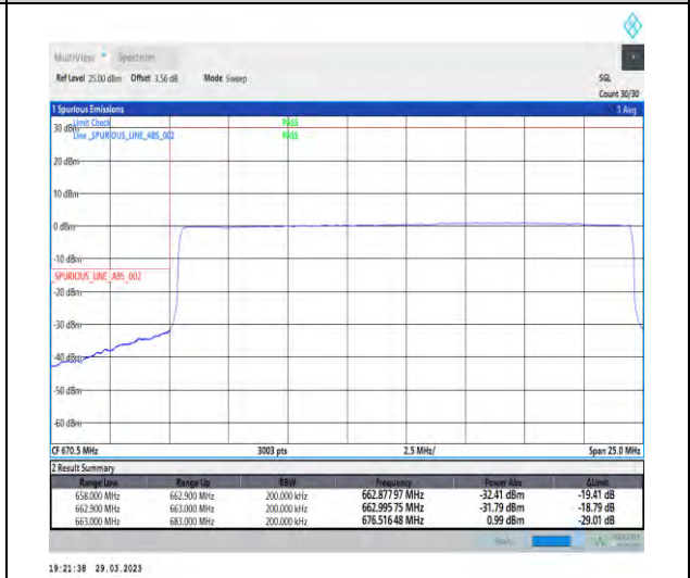
1-N71-15-20-L-6-CP-QPSK-Outer_Full-106@0-Ant1-1--PASS-see graph
