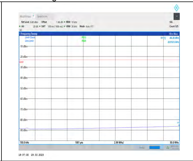
1-N71-15-20-H-1-DFT-PI2BPSK-Inner_1RB_Left-1 @ 1-0.15-30-Ant1-29.91--86.28--23-PASS
