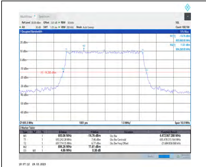
1-N71-15-5-H-3-DFT-16QAM-Outer_Full-25@0-Ant1 -4.472-4.860-≤5-PASS
