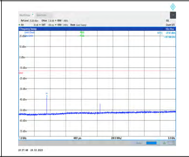
1-N71-15-20-H-1-DFT-PI2BPSK-Inner_1RB_Left-1 @ 1-1000-3000-Ant1-1357.50--37.81--13-PASS
