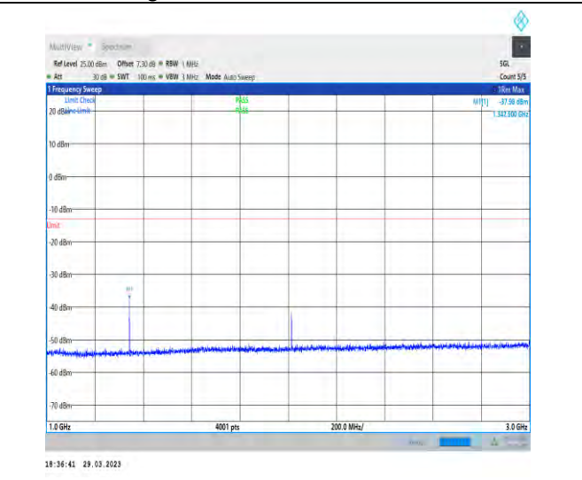
1-N71-15-20-M-1-DFT-PI2BPSK-Inner_1RB_Left-1@ 1-1000-3000-Ant1-1342.50--37.98--13-PASS
