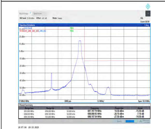
1-N71-15-5-H-5-CP-QPSK-Edge_1RB_Right-1@24-An t1-1--PASS-see graph
