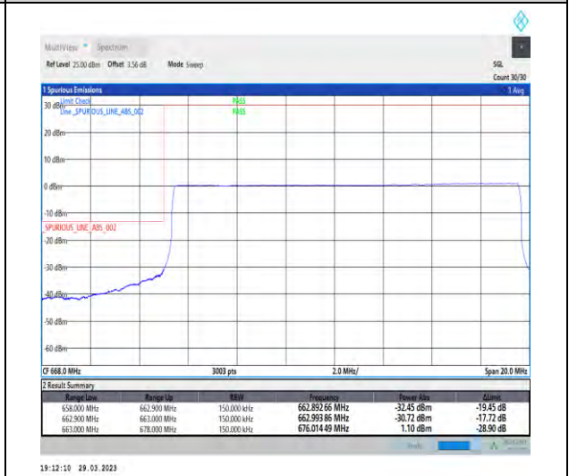
1-N71-15-15-L-6-CP-QPSK-Outer_Full-79@0-Ant1-1--PASS-see graph
