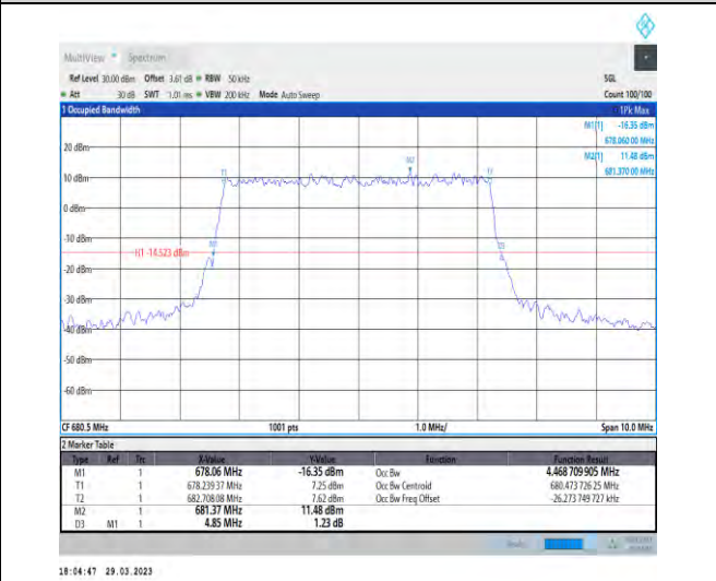
1-N71-15-5-M-3-DFT-16QAM-Outer_Full-25@0-Ant1 -4.469-4.850-≤5-PASS
