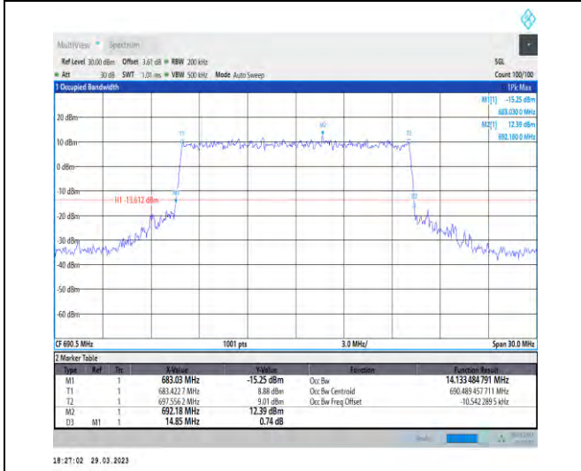
1-N71-15-15-H-7-CP-16QAM-Outer_Full-79@0-Ant1 -14.133-14.850-≤15-PASS
