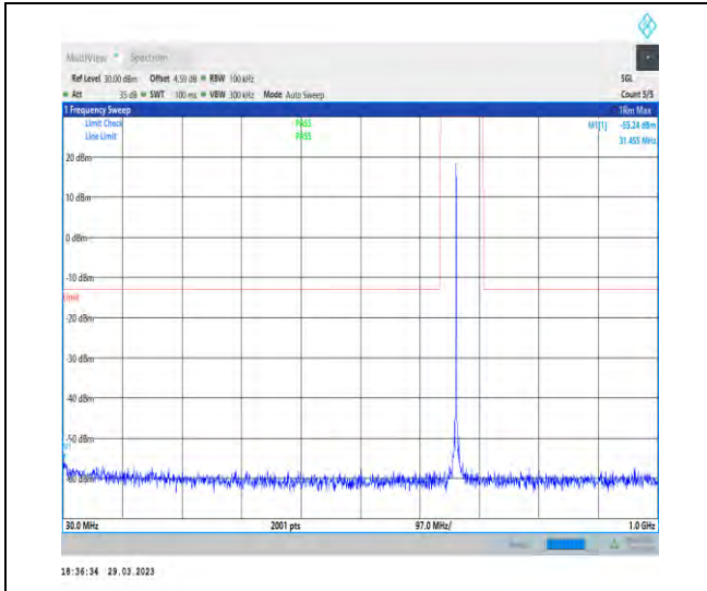
1-N71-15-20-M-1-DFT-PI2BPSK-Inner_1RB_Left-1 @1-30-1000-Ant1-31.46--55.24--13-PASS
