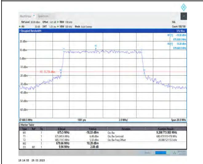
1-N71-15-10-M-7-CP-16QAM-Outer_Full-52@0-Ant 1-9.269-9.940-≤10-PASS
