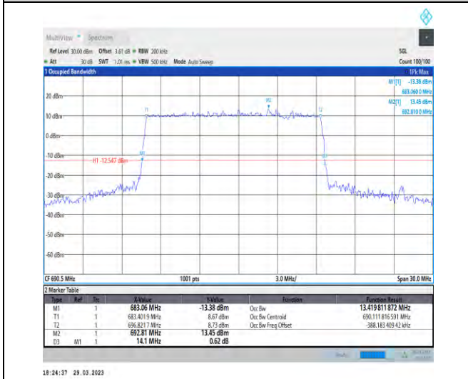
1-N71-15-15-H-3-DFT-16QAM-Outer_Full-75@0-Ant1 1-13.42-14.100≤15-PASS
