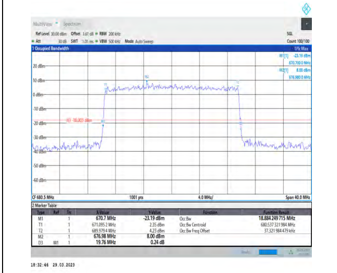
1-N71-15-20-M-9-CP-256QAM-Outer_Full-106@0-A nt1-18.884-19.760-≤20-PASS
