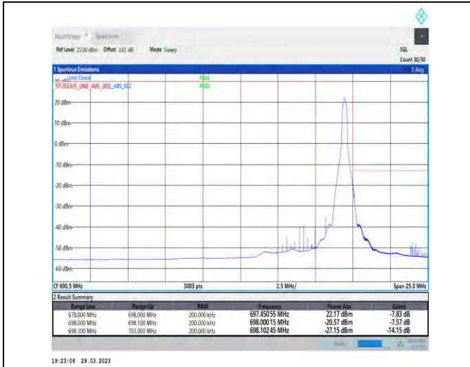
1-N71-15-20-H-2-DFT-PI2BPSK-Edge_1RB_Right-1@105-Ant1-1--PASS-see graph
