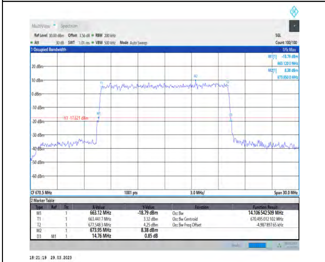
1-N71-15-15-L-9-CP-256QAM-Outer_Full-79@0-Ant 1-14.107-14.760-≤15-PASS
