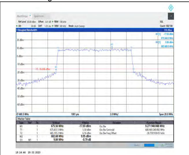
1-N71-15-10-M-6-CP-QPSK-Outer_Full-52@0-Ant1- 9.272-9.840-≤10-PASS
