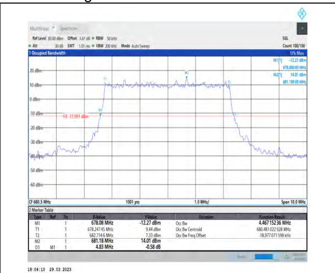
1-N71-15-5-M-1-DFT-QPSK-Outer_Full-25@0-Ant1- 4.467-4.830-≤5-PASS
