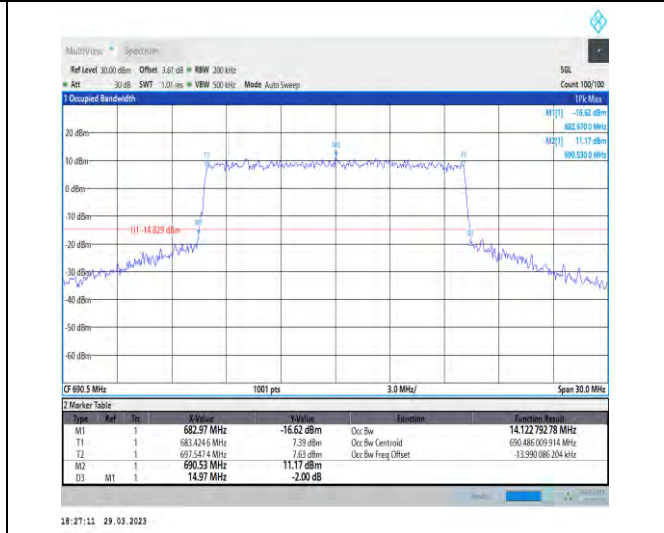
1-N71-15-15-H-8-CP-64QAM-Outer_Full-79@0-Ant1 -14.123-14.970-≤15-PASS
