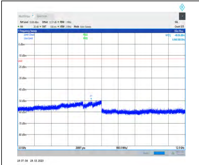
1-N71-15-20-H-1-DFT-PI2BPSK-Inner_1RB_Left-1 @ 1-3000-12000-Ant1-6946.50--49.06--13-PASS
