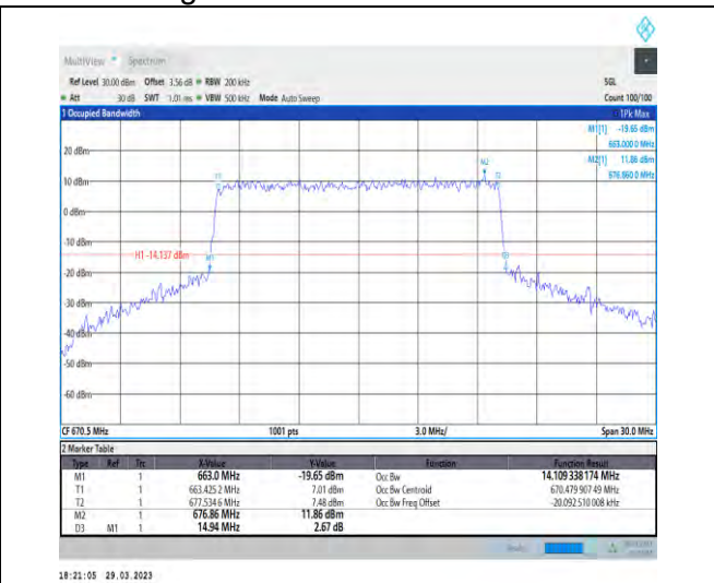
1-N71-15-15-L-8-CP-64QAM-Outer_Full-79@0-Ant1 14.109-14.940-≤15-PASS
