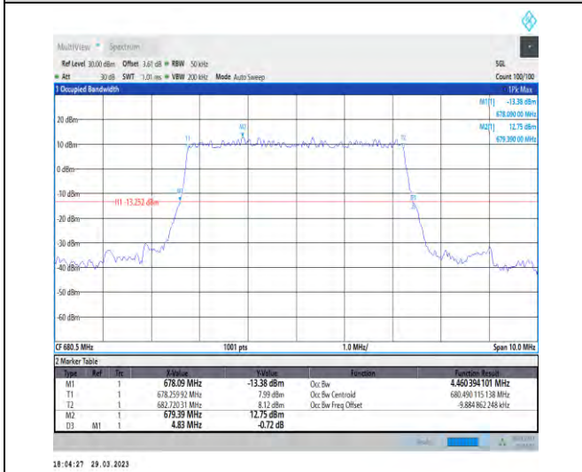
1-N71-15-5-M-2-DFT-PI2BPSK-Outer_Full-25@0-Ant1 t1-4.46-4.830-≤5-PASS
