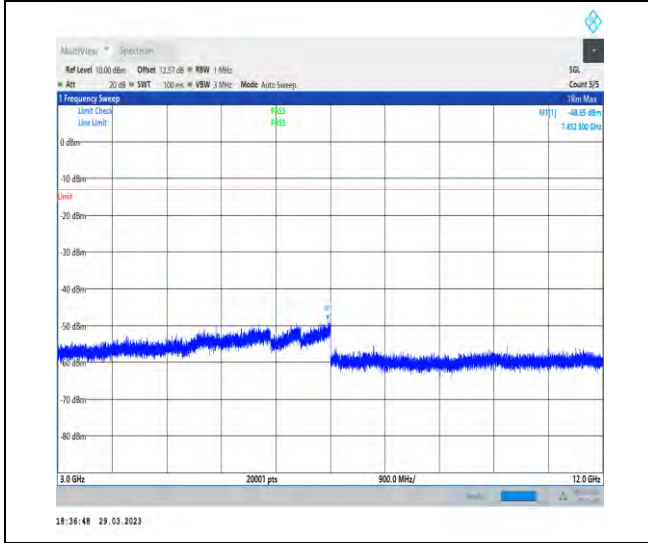
1-N71-15-20-M-1-DFT-PI2BPSK-Inner_1RB_Left-1 @1-3000-12000-Ant1-7452.30--48.65--13-PASS
