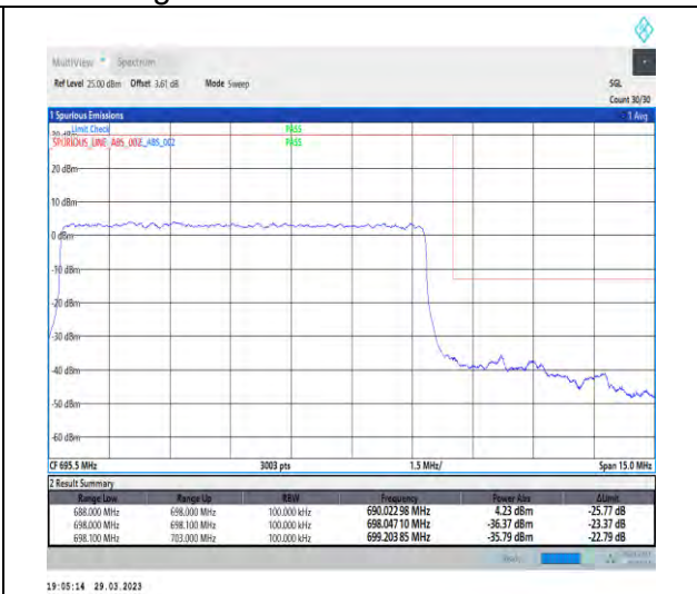
1-N71-15-10-H-3-DFT-PI2BPSK-Outer_Full-50@0-Ant1-1--PASS-see graph
