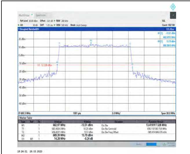
1-N71-15-15-H-1-DFT-QPSK-Outer_Full-75@0-Ant1 -13.42-14.280≤15-PASS
