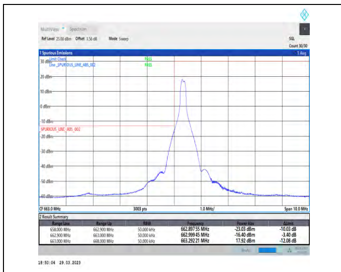
1-N71-15-5-L-1-DFT-PI2BPSK-Edge_1RB_Left-1@0-A nt1-1--PASS-see graph
