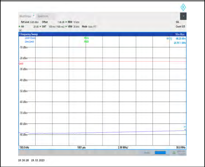
1-N71-15-20-M-1-DFT-PI2BPSK-Inner_1RB_Left-1 @ 1-0.15-30-Ant1-29.79--86.26--23-PASS
