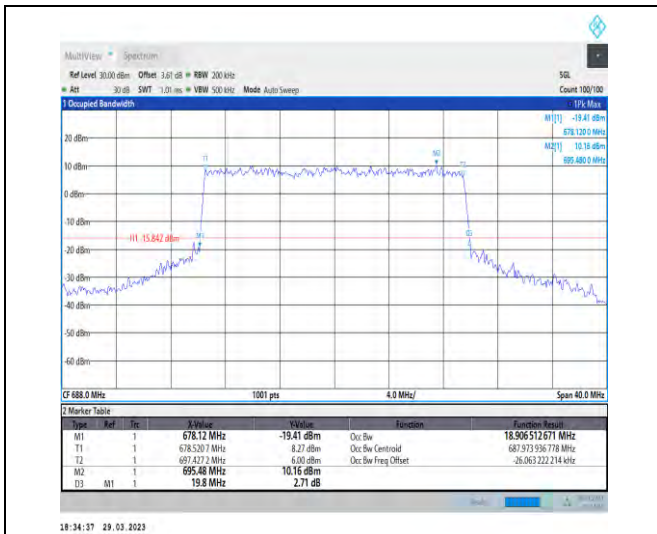
1-N71-15-20-H-6-CP-QPSK-Outer_Full-106@0-Ant1 -18.907-19.800-≤20-PASS
