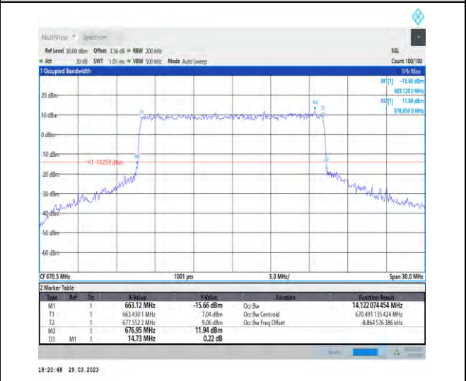
1-N71-15-15-L-6-CP-QPSK-Outer_Full-79@0-Ant1-1 4.122-14.730-≤15-PASS
