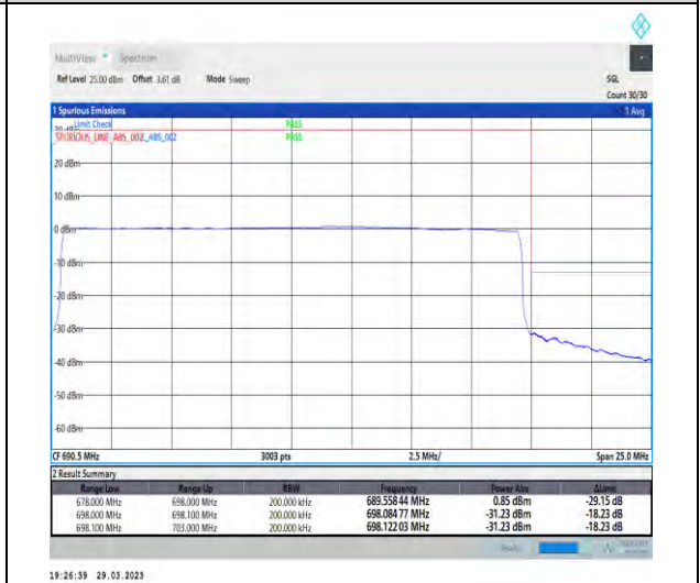
1-N71-15-20-H-6-CP-QPSK-Outer_Full-106@0-Ant1-1--PASS-see graph
