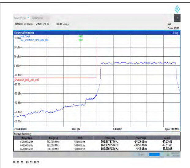
1-N71-15-5-L-3-DFT-PI2BPSK-Outer_Full-25@0-A Ant1-1--PASS-see graph
