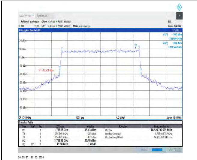
1-N66-15-20-M-7-CP-16QAM-Outer_Full-106@0-Ant 1-18.93-19.880-≤20-PASS
