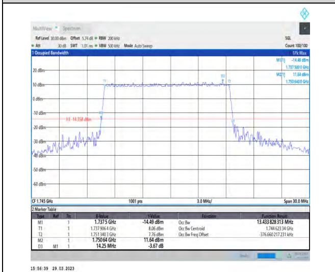
1-N66-15-15-M-4-DFT-64QAM-Outer_Full-75@0-Ant 1-13.434-14.250-≤15-PASS
