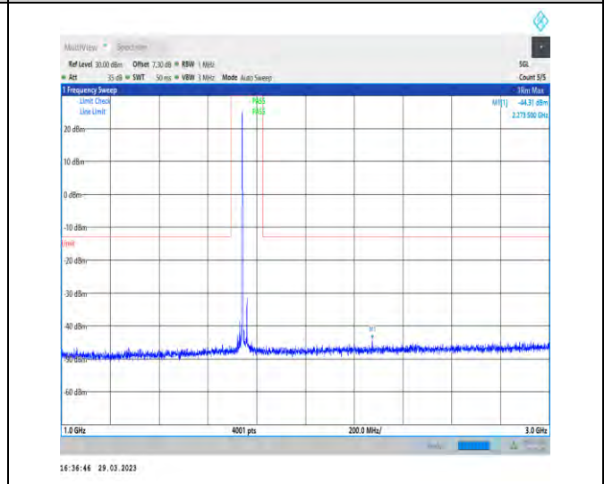
1-N66-15-40-H-1-DFT-PI2BPSK-Inner_1RB_Left-1 @ 1-1000-3000-Ant1-2273.50--44.31--13-PASS
