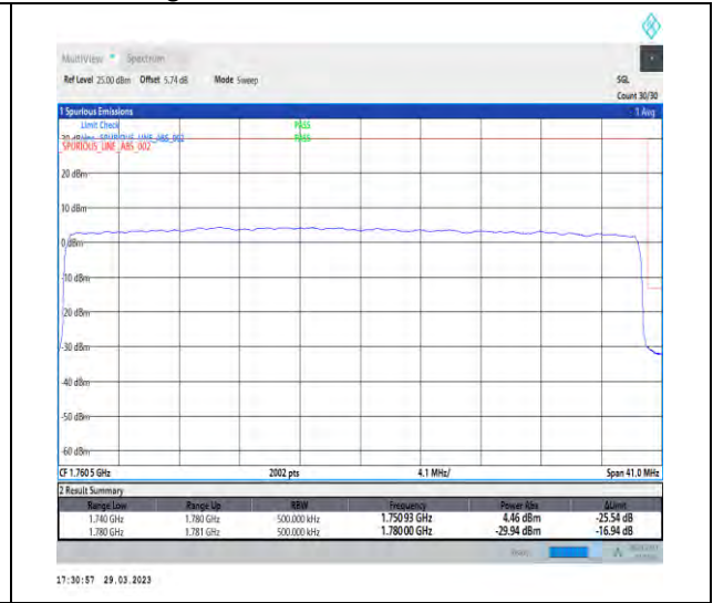
1-N66-15-40-H-3-DFT-PI2BPSK-Outer_Full-216@0-Ant1-1-seegraph-PASS-see graph
