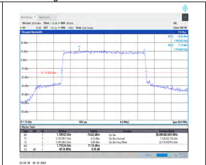
1-N66-15-40-L-6-CP-QPSK-Outer_Full-216@0-Ant1- 38.497-40.160-≤40-PASS
