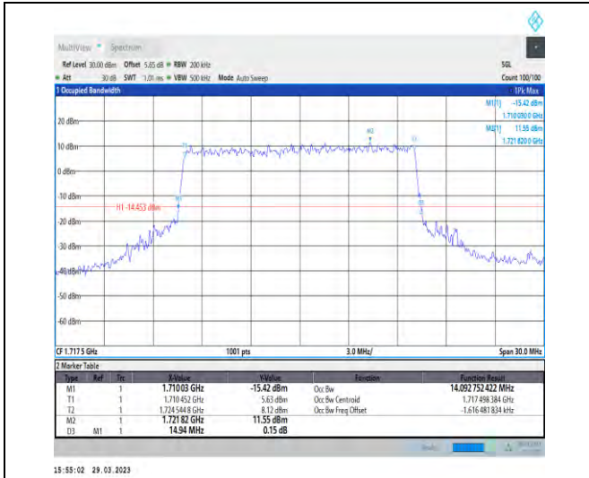
1-N66-15-15-L-7-CP-16QAM-Outer_Full-79@0-Ant1 -14.093-14.940≤15-PASS
