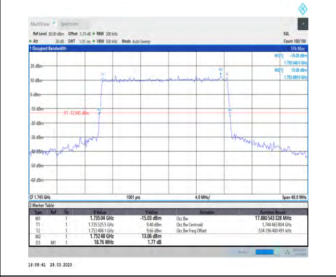
1-N66-15-20-M-2-DFT-PI2BPSK-Outer_Full-100@0-Ant 1-17.881-18.760-≤20-PASS
