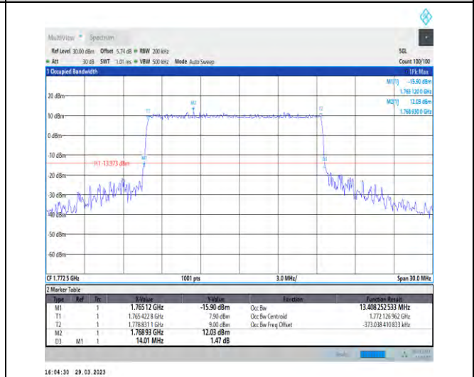
1-N66-15-15-H-4-DFT-64QAM-Outer_Full-75@0-Ant1 1-13.408-14.010-≤15-PASS
