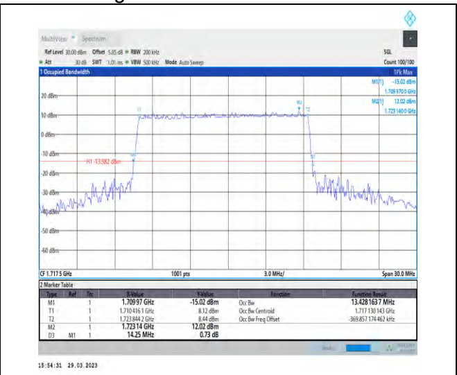
1-N66-15-15-L-4-DFT-64QAM-Outer_Full-75@0-Ant 1-13.428-14.250-≤15-PASS
