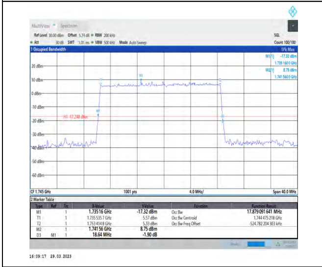
1-N66-15-20-M-5-DFT-256QAM-Outer_Full-100@0-A Ant1-17.879-18.640-≤20-PASS
