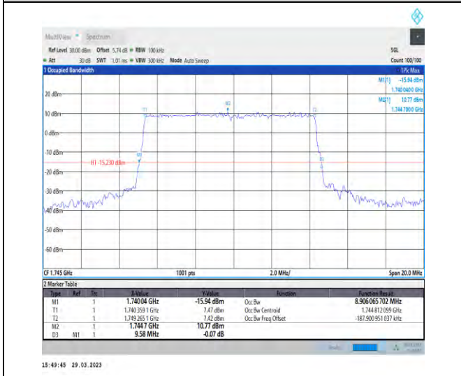
1-N66-15-10-M-3-DFT-16QAM-Outer_Full-50@0-Ant1 1-8.906-9.580-≤10-PASS
