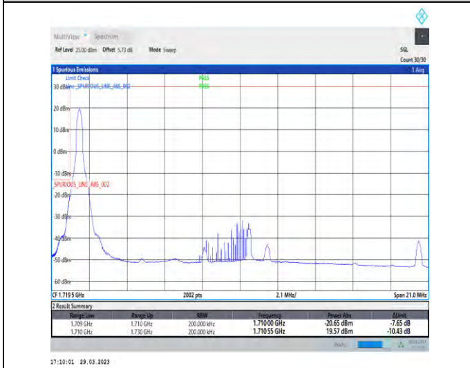
1-N66-15-20-L-4-CP-QPSK-Edge_1RB_Left-1@0-Ant1-1-seegraph-PASS-see graph
