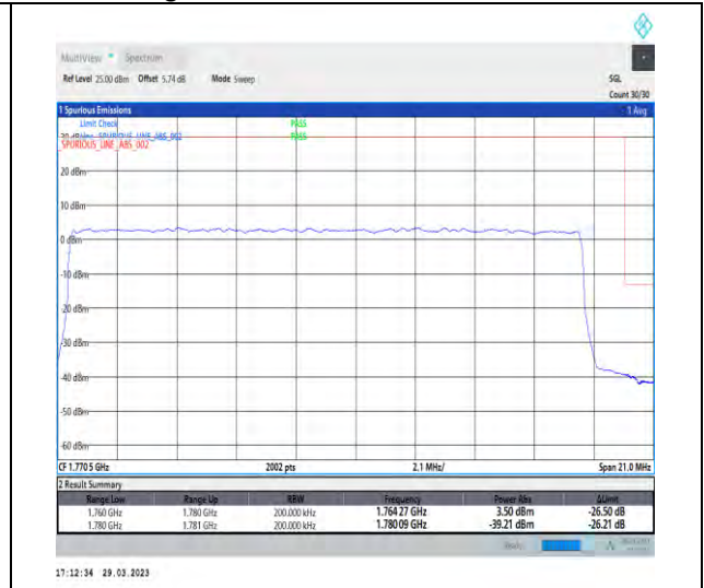
1-N66-15-20-H-3-DFT-PI2BPSK-Outer_Full-100@0-Ant1-1-seegraph-PASS-see graph
