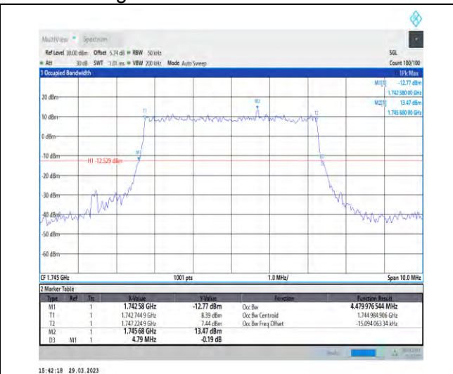
1-N66-15-5-M-1-DFT-QPSK-Outer_Full-25@0-Ant1- 4.48-4.790-≤5-PASS
