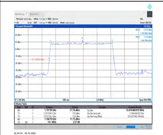
1-N66-15-15-M-5-DFT-256QAM-Outer_Full-75@0-A nt1-13.416-14.100-≤15-PASS
