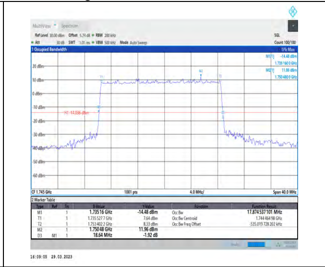
1-N66-15-20-M-4-DFT-64QAM-Outer_Full-100@0-A nt1-17.875-18.640-≤20-PASS
