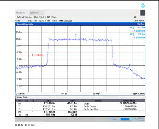
1-N66-15-40-H-6-CP-QPSK-Outer_Full-216@0-Ant1 -38.487-40.080-≤40-PASS
