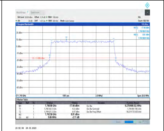
1-N66-15-10-M-8-CP-64QAM-Outer_Full-52@0-Ant1 -9.279-9.860-≤10-PASS
