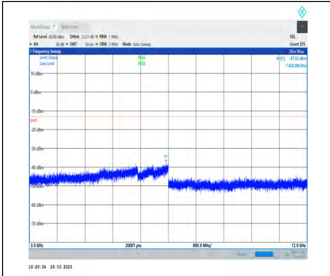
1-N66-15-40-L-1-DFT-PI2BPSK-Inner_1RB_Left-1 @ 1-3000-12000-Ant1-7426.20--37.52--13-PASS
