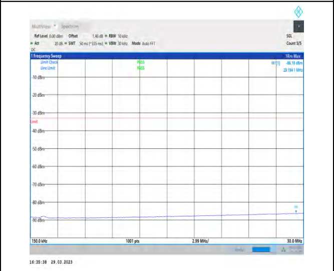
1-N66-15-40-M-1-DFT-PI2BPSK-Inner_1RB_Left-1 @ 1-0.15-30-Ant1-29.19--86.18--33-PASS
