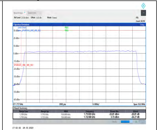
1-N66-15-15-L-3-DFT-PI2BPSK-Outer_Full-75@0-Ant1-1-seegraph-PASS-see graph
