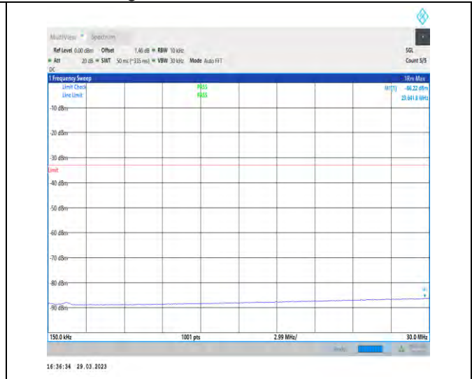
1-N66-15-40-H-1-DFT-PI2BPSK-Inner_1RB_Left-1 @ 1-0.15-30-Ant1-29.64--86.22--33-PASS
