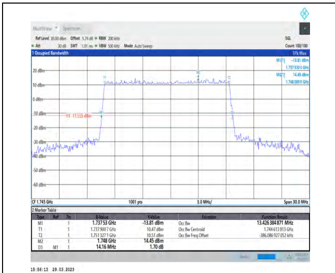
1-N66-15-15-M-2-DFT-P12BPSK-Outer_Full-75@0-A nt1-13.426-14.160-≤15-PASS
