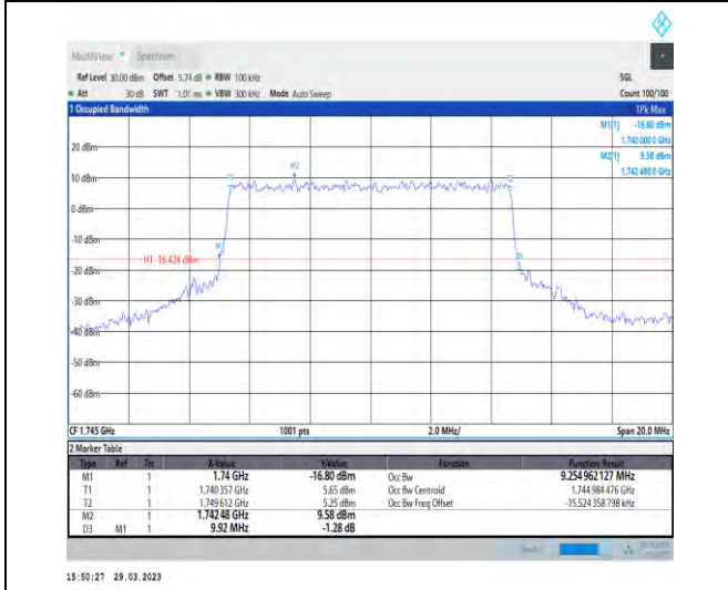
1-N66-15-10-M-7-CP-16QAM-Outer_Full-52@0-Ant1 -9.255-9.920-≤10-PASS
