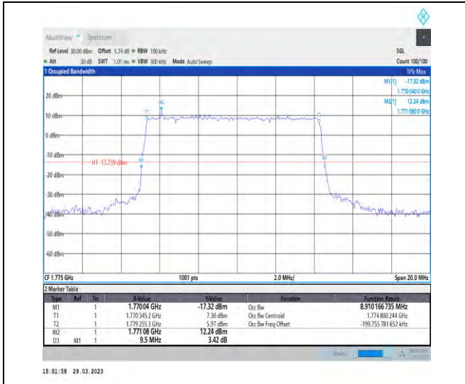
1-N66-15-10-H-4-DFT-64QAM-Outer_Full-50@0-Ant 1-8.91-9.500-≤10-PASS
