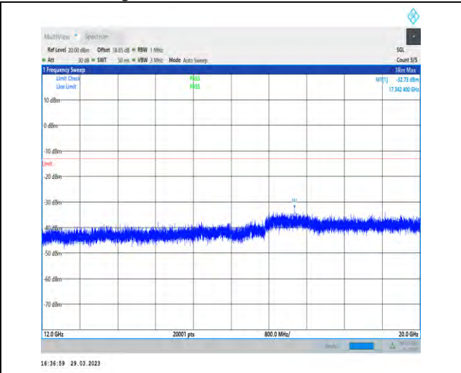
1-N66-15-40-H-1-DFT-PI2BPSK-Inner_1RB_Left-1@ 1-12000-20000-Ant1-17342.40--32.73--13-PASS
