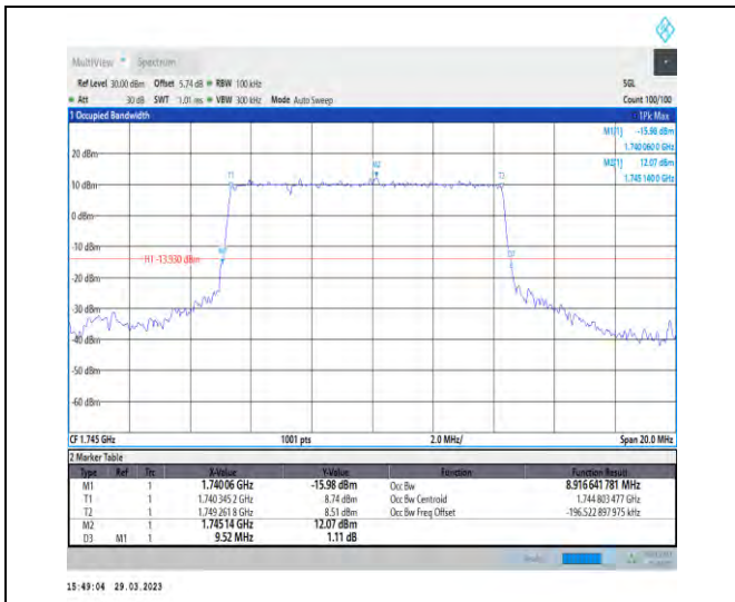
1-N66-15-10-M-1-DFT-QPSK-Outer_Full-50@0-Ant1 -8.917-9.520-≤10-PASS
