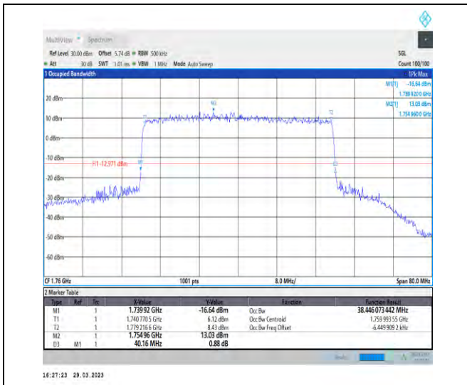
1-N66-15-40-H-3-DFT-16QAM-Outer_Full-216@0-A nt1-38.446-40.160-≤40-PASS
