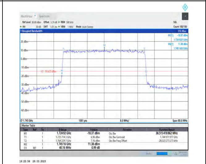
1-N66-15-40-M-7-CP-16QAM-Outer_Full-216@0-Ant 1-38.515-40.160-≤40-PASS
