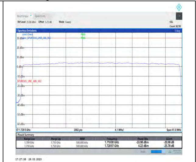
1-N66-15-40-L-3-DFT-PI2BPSK-Outer_Full-216@0-Ant1-1-seegraph-PASS-see graph
