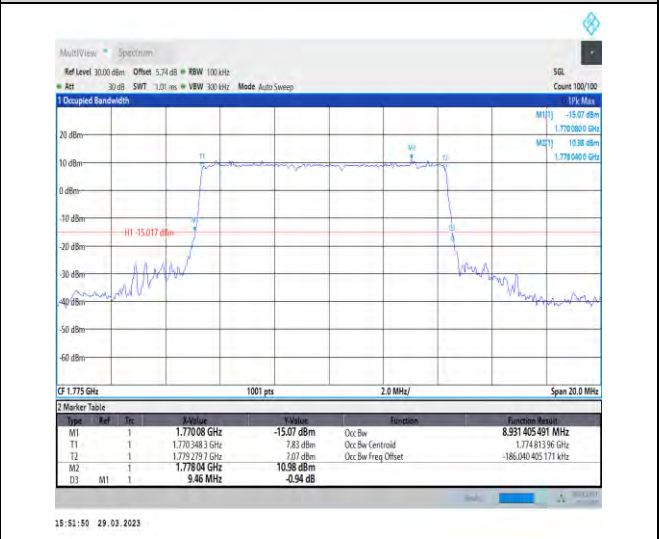
1-N66-15-10-H-3-DFT-16QAM-Outer_Full-50@0-Ant 1-8.931-9.460-≤10-PASS
