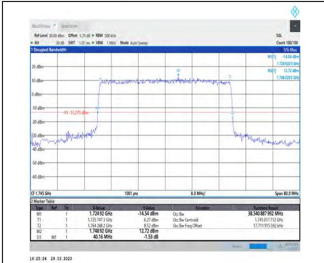
1-N66-15-40-M-4-DFT-64QAM-Outer_Full-216@0-A nt1-38.541-40.160-≤40-PASS
