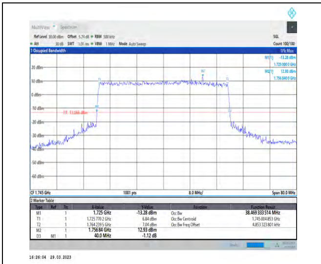
1-N66-15-40-M-8-CP-64QAM-Outer_Full-216@0-Ant 1-38.469-40.000-≤40-PASS
