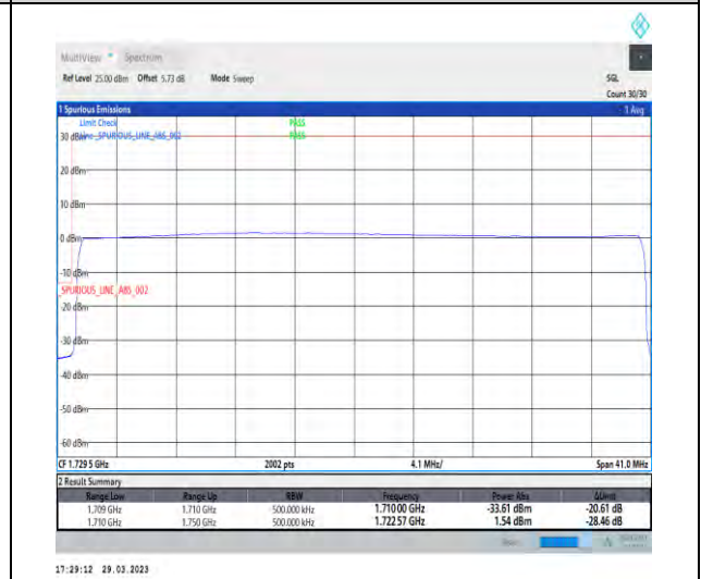
1-N66-15-40-L-6-CP-QPSK-Outer_Full-216@0-Ant1-1-seegraph-PASS-see graph
