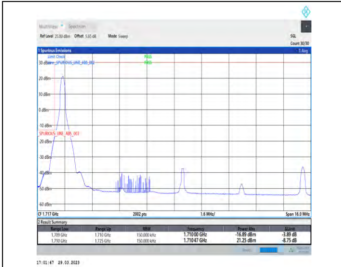
1-N66-15-15-L-1-DFT-PI2BPSK-Edge_1RB_Left-1@0-Ant1-1-seegraph-PASS-see graph
