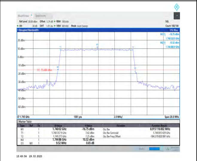
1-N66-15-10-M-4-DFT-64QAM-Outer_Full-50@0-Ant1 1-8.915-9.520-≤10-PASS
