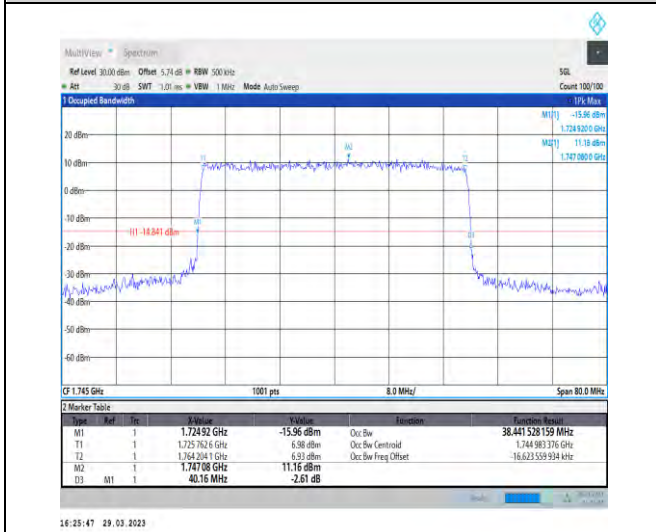
1-N66-15-40-M-6-CP-QPSK-Outer_Full-216@0-Ant1 -38.442-40.160-≤40-PASS
