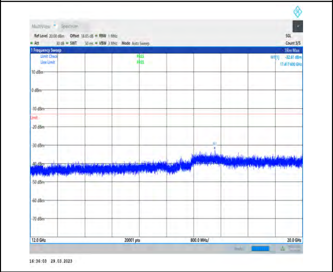
1-N66-15-40-M-1-DFT-PI2BPSK-Inner_1RB_Left-1 @ 1-12000-20000-Ant1-17417.60--32.61--13-PASS
