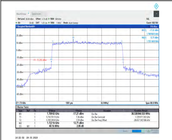
1-N66-15-40-L-3-DFT-16QAM-Outer_Full-216@0-Ant t1-38.539-40.160-≤40-PASS
