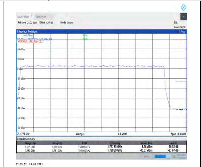
1-N66-15-15-H-3-DFT-PI2BPSK-Outer_Full-75@0-Ant1-1-seegraph-PASS-see graph
