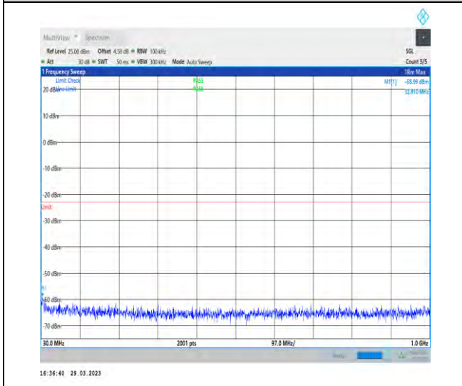
1-N66-15-40-H-1-DFT-PI2BPSK-Inner_1RB_Left-1 @ 1-30-1000-Ant1-32.91--58.99--23-PASS
