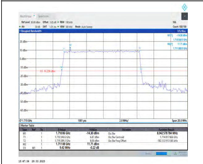
1-N66-15-10-L-4-DFT-64QAM-Outer_Full-50@0-Ant 1-8.943-9.420-≤10-PASS
