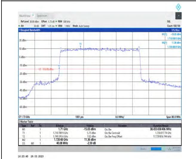
1-N66-15-40-L-7-CP-16QAM-Outer_Full-216@0-Ant 1-38.456-40.080-≤40-PASS
