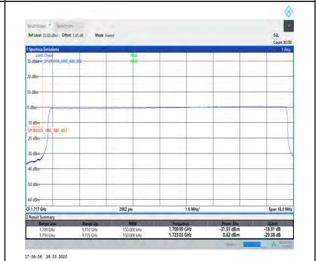
1-N66-15-15-L-6-CP-QPSK-Outer_Full-79@0-Ant1-1-seegraph-PASS-see graph
