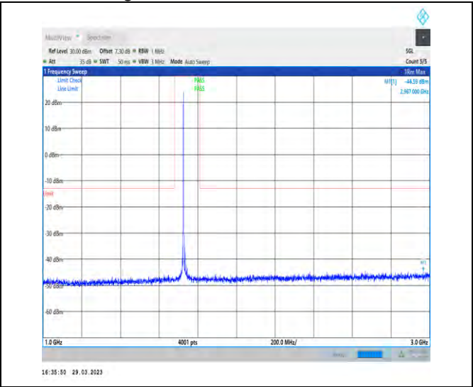
1-N66-15-40-M-1-DFT-PI2BPSK-Inner_1RB_Left-1 @ 1-1000-3000-Ant1-2967.00--44.59--13-PASS
