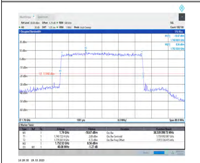
1-N66-15-40-H-9-CP-256QAM-Outer_Full-216@0-Ant 1-38.539-40.080-≤40-PASS
