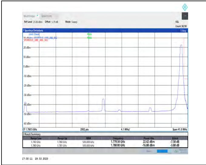
1-N66-15-40-H-2-DFT-PI2BPSK-Edge_1RB_Right-1@215-Ant1-1-seegraph-PASS-see graph
