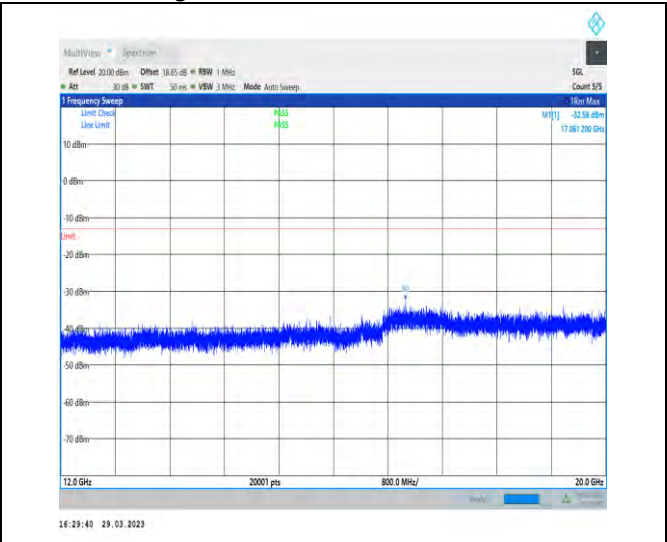
1-N66-15-40-L-1-DFT-PI2BPSK-Inner_1RB_Left-1 @ 1-12000-20000-Ant1-17061.20--32.58--13-PASS
