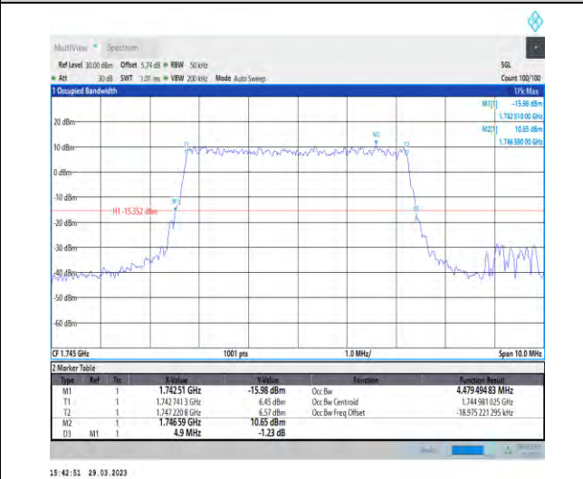
1-N66-15-5-M-3-DFT-16QAM-Outer_Full-25@0-Ant1 -4.479-4.900-≤5-PASS
