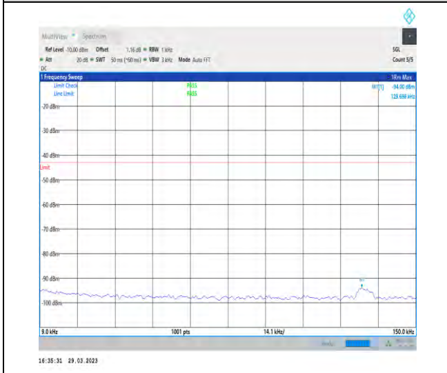
1-N66-15-40-M-1-DFT-PI2BPSK-Inner_1RB_Left-1 @ 1-0.009-0.15-Ant1-0.13--94.00--43-PASS
