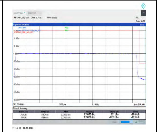
1-N66-15-20-H-6-CP-QPSK-Outer_Full-106@0-Ant1-1-seegraph-PASS-see graph
