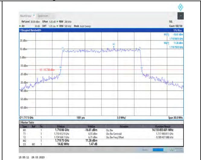
1-N66-15-15-L-8-CP-64QAM-Outer_Full-79@0-Ant1 -14.156-14.820≤15-PASS
