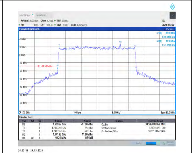
1-N66-15-40-L-8-CP-64QAM-Outer_Full-216@0-Ant 1-38.596-40.240-≤40-PASS
