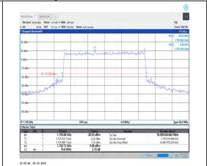
1-N66-15-20-M-8-CP-64QAM-Outer_Full-106@0-Ant 1-18.928-19.800-≤20-PASS
