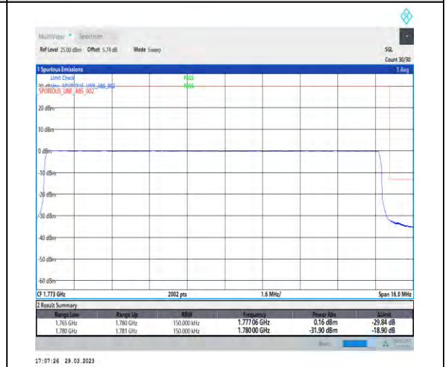
1-N66-15-15-H-6-CP-QPSK-Outer_Full-79@0-Ant1-1-seegraph-PASS-see graph
