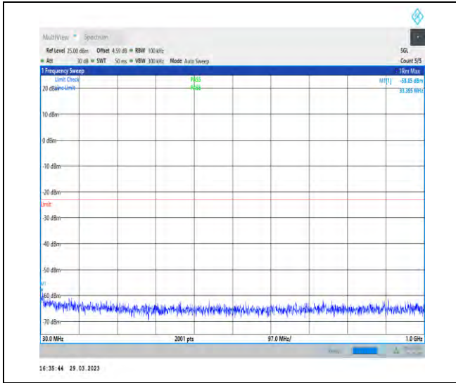
1-N66-15-40-M-1-DFT-PI2BPSK-Inner_1RB_Left-1 @ 1-30-1000-Ant1-33.40--58.85--23-PASS
