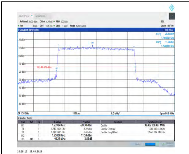
1-N66-15-40-H-7-CP-16QAM-Outer_Full-216@0-Ant 1-38.462-40.240-≤40-PASS
