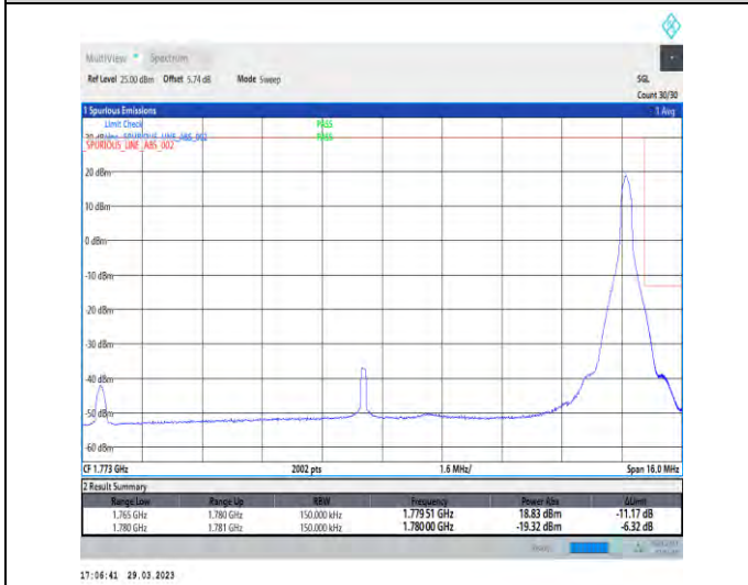
1-N66-15-15-H-5-CP-QPSK-Edge_1RB_Right-1@78-Ant1-1-seegraph-PASS-see graph
