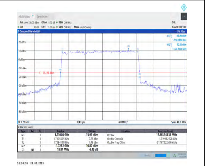
1-N66-15-20-L-3-DFT-16QAM-Outer_Full-100@0-Ant 1-17.863-18.840-≤20-PASS
