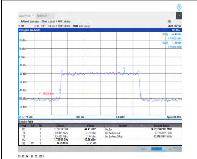
1-N66-15-15-L-9-CP-256QAM-Outer_Full-79@0-Ant 1-14.092-14.790≤15-PASS
