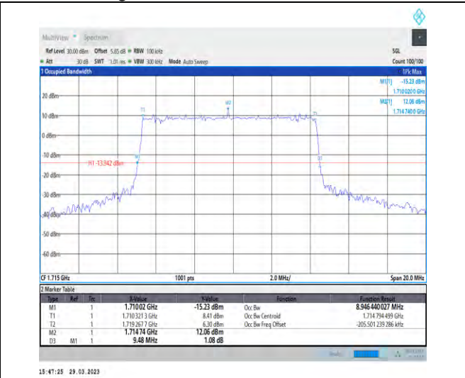
1-N66-15-10-L-3-DFT-16QAM-Outer_Full-50@0-Ant 1-8.946-9.480-≤10-PASS
