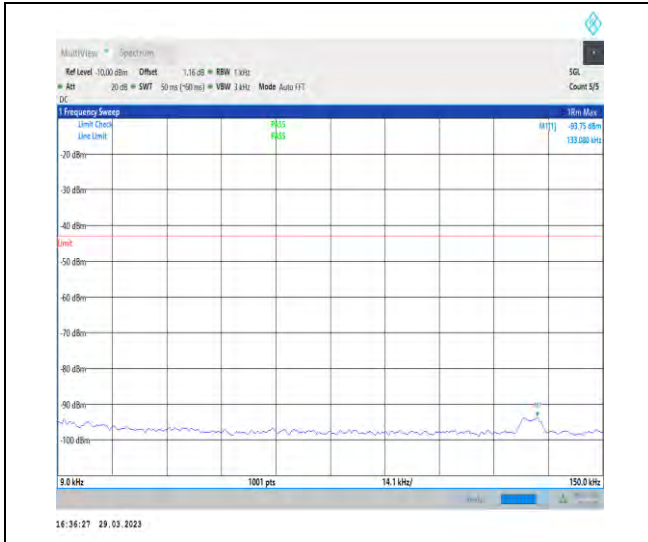
1-N66-15-40-H-1-DFT-PI2BPSK-Inner_1RB_Left-1 @ 1-0.009-0.15-Ant1-0.13--93.75--43-PASS
