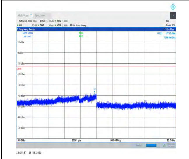
1-N66-15-40-M-1-DFT-PI2BPSK-Inner_1RB_Left-1 @ 1-3000-12000-Ant1-7396.50--37.17--13-PASS
