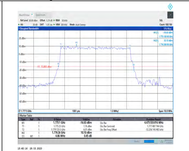
1-N66-15-5-H-4-DFT-64QAM-Outer_Full-25@0-Ant1 -4.476-4.860-≤5-PASS
