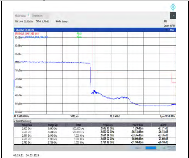
1-N41-30-90-H-3-DFT-PI2BPSK-Outer_Full-240@0-Ant1-1--PASS-see graph
