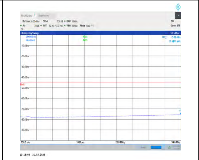
1-N41-30-100-M-1-DFT-PI2BPSK-Inner_1RB_Left-1 @1-0.15-30-Ant1-29.91--75.36--45-PASS
