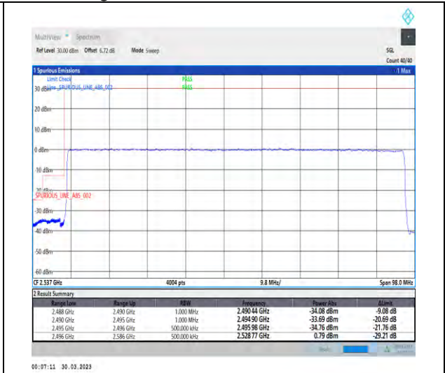
1-N41-30-90-L-3-DFT-PI2BPSK-Outer_Full-240@0-Ant1-1--PASS-see graph
