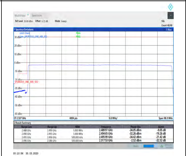
1-N41-30-90-L-6-CP-QPSK-Outer_Full-245@0-Ant1-1--PASS-see graph
