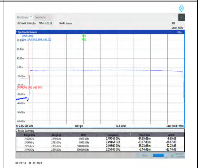
1-N41-30-100-L-6-CP-QPSK-Outer_Full-273@0-Ant1-1--PASS-see graph
