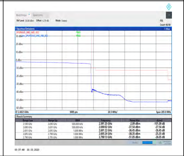
1-N41-30-100-H-6-CP-QPSK-Outer_Full-273@0-Ant1-1--PASS-see graph
