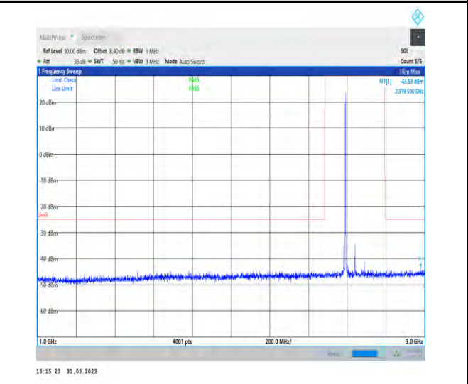
1-N41-30-100-H-1-DFT-PI2BPSK-Inner_1RB_Left-1 @1-1000-3000-Ant1-2961.50--43.53--25-PASS
