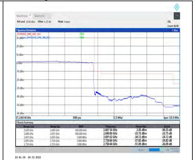
1-N41-30-60-H-3-DFT-PI2BPSK-Outer_Full-162@0-Ant1-1--PASS-see graph
