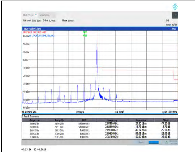
1-N41-30-90-H-2-DFT-PI2BPSK-Edge_1RB_Right-1@244-Ant1-1--PASS-see graph
