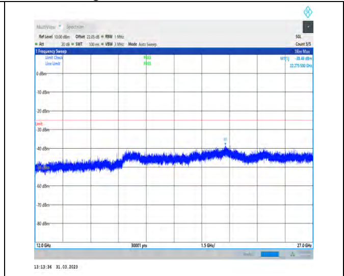
1-N41-30-100-L-1-DFT-PI2BPSK-Inner_1RB_Left-1 @1-12000-27000-Ant1-22237.00--38.49--25-PASS
