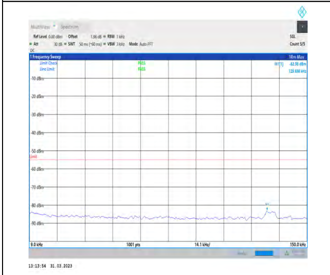
1-N41-30-100-M-1-DFT-PI2BPSK-Inner_1RB_Left-1 @1-0.009-0.15-Ant1-0.13--82.98--55-PASS
