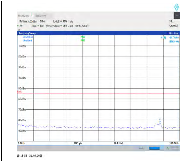
1-N41-30-100-H-1-DFT-PI2BPSK-Inner_1RB_Left-1 @1-0.009-0.15-Ant1-0.13--82.75--55-PASS
