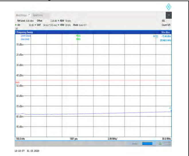
1-N41-30-100-H-1-DFT-PI2BPSK-Inner_1RB_Left-1 @1-0.15-30-Ant1-29.94--75.46--45-PASS
