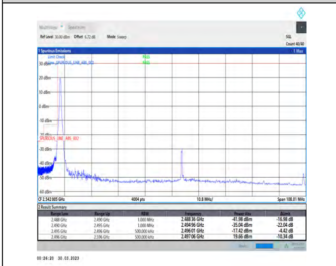
1-N41-30-100-L-4-CP-QPSK-Edge_1RB_Left-1@0-Ant1-1--PASS-see graph
