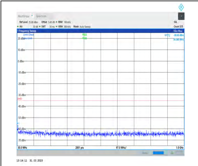
1-N41-30-100-M-1-DFT-PI2BPSK-Inner_1RB_Left-1 @1-30-1000-Ant1-34.37--58.60--35-PASS
