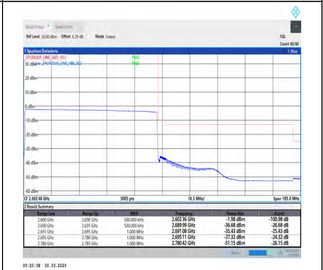
1-N41-30-90-H-6-CP-QPSK-Outer_Full-245@0-Ant1-1--PASS-see graph
