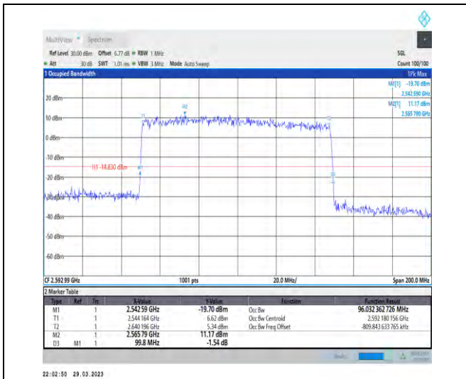
1-N41-30-100-M-3-DFT-16QAM-Outer_Full-270@0-Ant1-96.032-99.800-≤100-PASS
