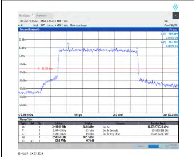
1-N41-30-100-L-6-CP-QPSK-Outer_Full-273@0-Ant 1-96.975-100.800-≤100-PASS
