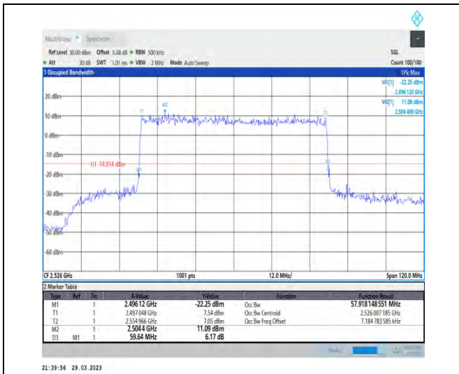
1-N41-30-60-L-1-DFT-QPSK-Outer_Full-162@0-Ant t1-57.918-59.640-≤60-PASS
