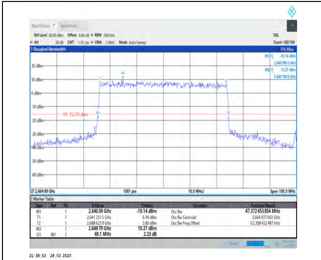
1-N41-30-50-H-6-CP-QPSK-Outer_Full-133@0-Ant1 -47.372-49.100-≤50-PASS
