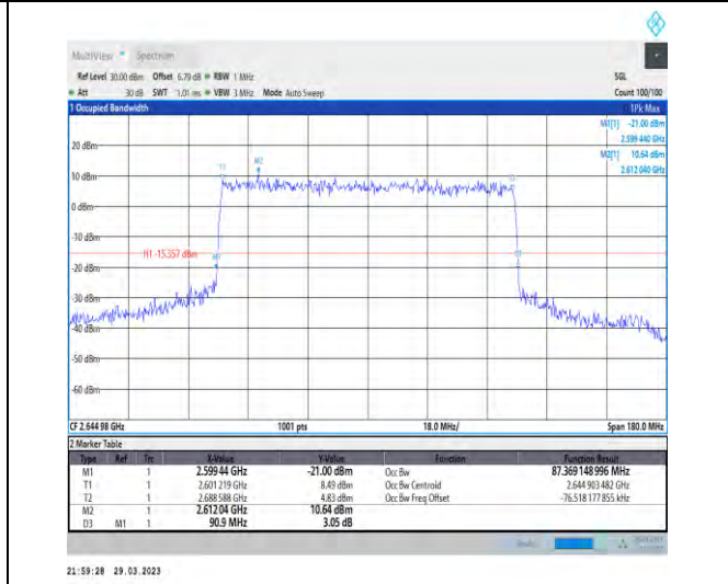
1-N41-30-90-H-8-CP-64QAM-Outer_Full-245@0-Ant1-87.369-90.900-<=90-PASS
