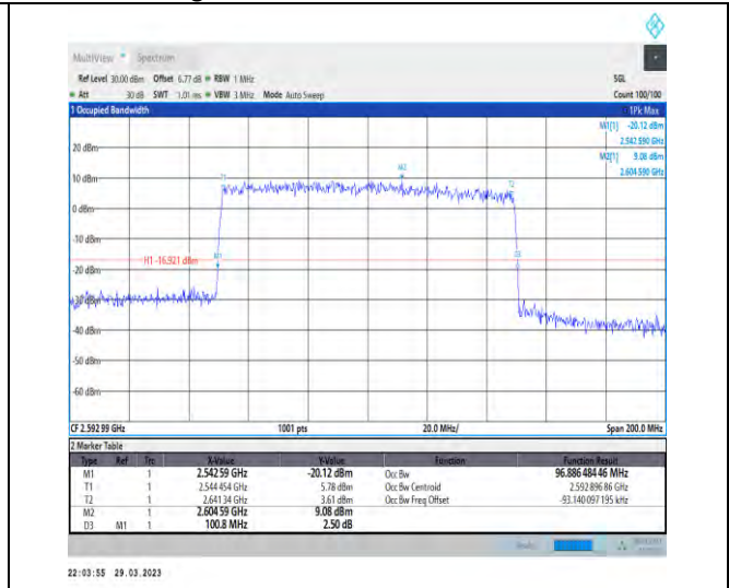
1-N41-30-100-M-8-CP-64QAM-Outer_Full-273@0-A nt1-96.886-100.800-≤100-PASS
