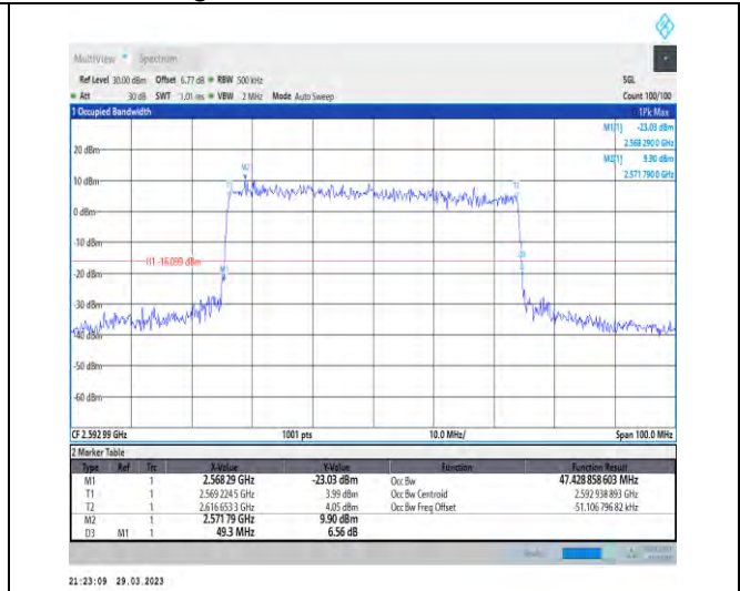
1-N41-30-50-M-8-CP-64QAM-Outer_Full-133@0-Ant t1-47.429-49.300-≤50-PASS
