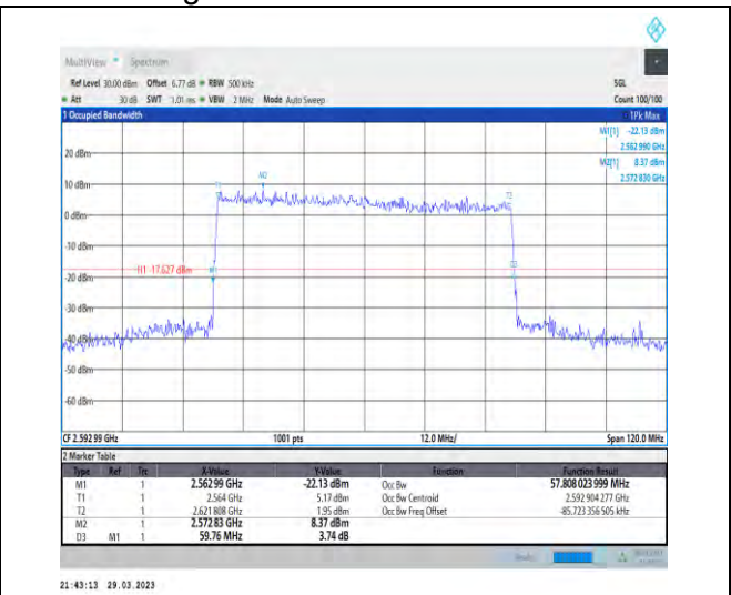
1-N41-30-60-M-5-DFT-256QAM-Outer_Full-162@0- Ant1-57.808-59.760-≤60-PASS
