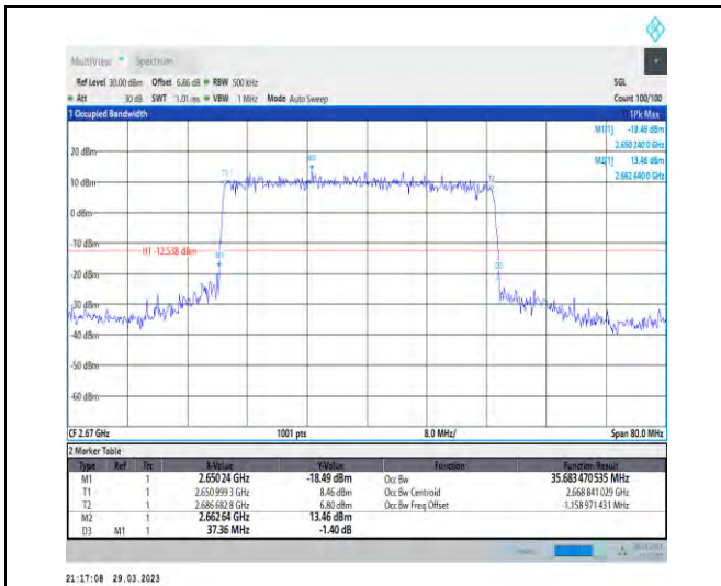
1-N41-30-40-H-1-DFT-QPSK-Outer_Full-100@0-Ant 1-35.683-37.360-≤40-PASS
