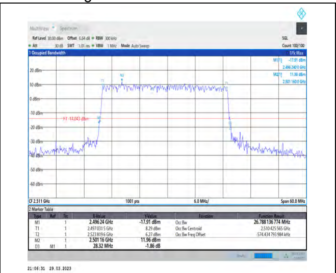
1-N41-30-30-L-3-DFT-16QAM-Outer_Full-75@0-Ant 1-26.788-28.320-≤30-PASS
