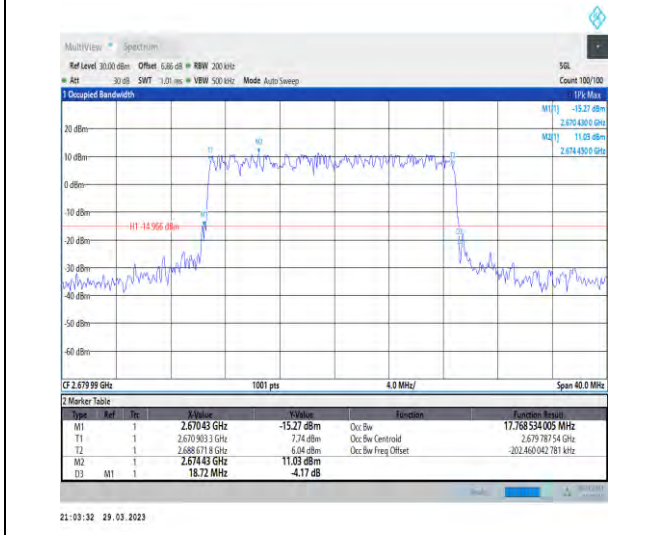
1-N41-30-20-H-1-DFT-QPSK-Outer_Full-50@0-Ant1 -17.769-18.720-≤20-PASS
