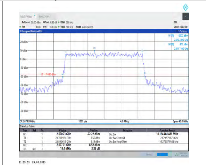
1-N41-30-20-H-8-CP-64QAM-Outer_Full-51@0-Ant1 -18.164-19.400-≤20-PASS
