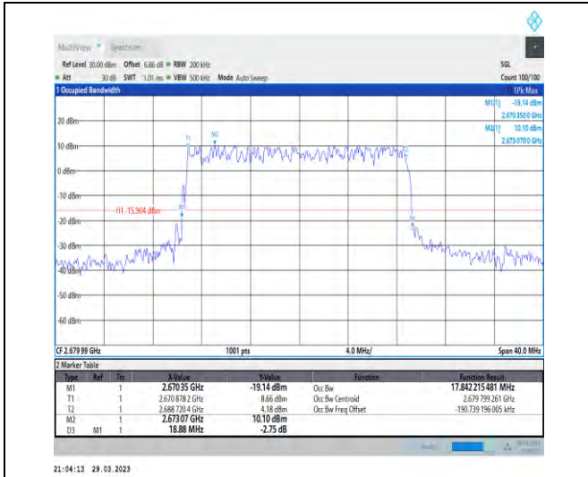
1-N41-30-20-H-3-DFT-16QAM-Outer_Full-50@0-Ant 1-17.842-18.880-≤20-PASS
