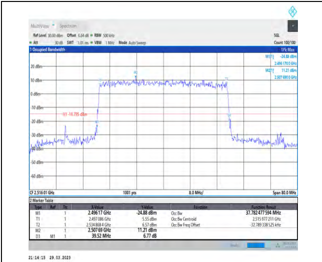
1-N41-30-40-L-7-CP-16QAM-Outer_Full-106@0-Ant 1-37.782-39.520-≤40-PASS
