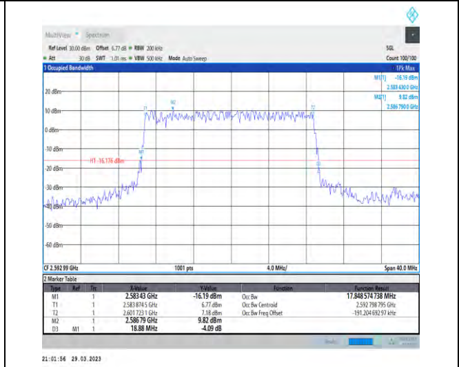
1-N41-30-20-M-3-DFT-16QAM-Outer_Full-50@0-Ant 1-17.849-18.880-≤20-PASS
