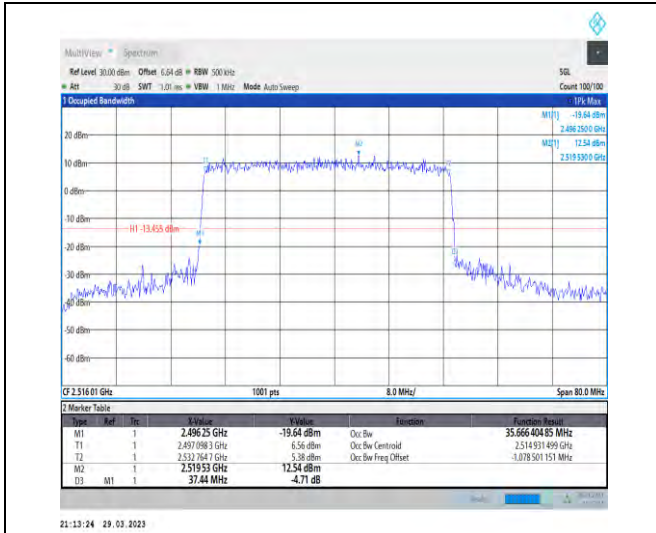
1-N41-30-40-L-3-DFT-16QAM-Outer_Full-100@0-An t1-35.666-37.440-≤40-PASS
