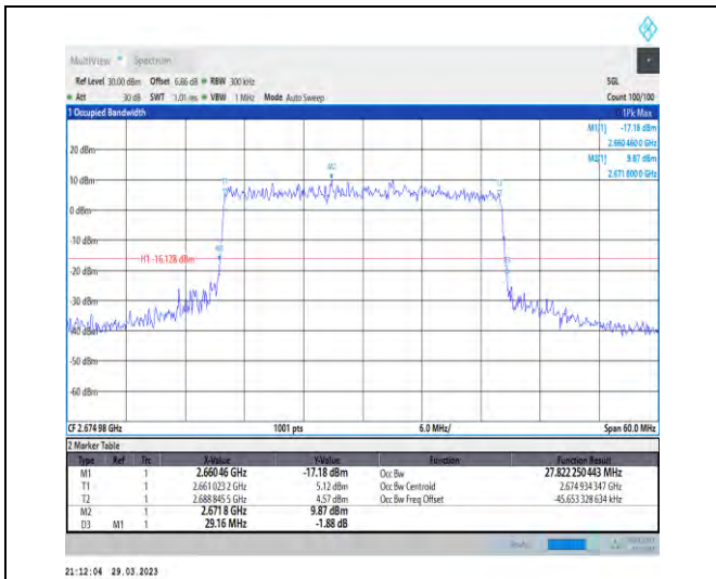
1-N41-30-30-H-8-CP-64QAM-Outer_Full-78@0-Ant1 -27.822-29.160-≤30-PASS
