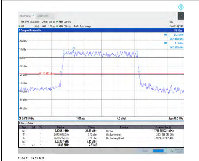
1-N41-30-20-H-5-DFT-256QAM-Outer_Full-50@0-A nt1-17.767-18.880-≤20-PASS
