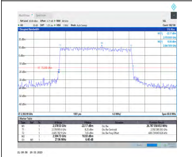
1-N41-30-30-M-3-DFT-16QAM-Outer_Full-75@0-Ant1 1-26.787-27.960-≤30-PASS
