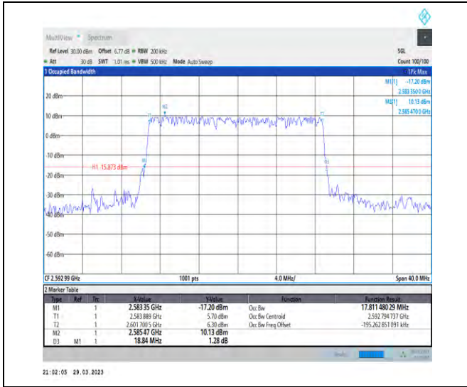
1-N41-30-20-M-4-DFT-64QAM-Outer_Full-50@0-Ant 1-17.811-18.840-≤20-PASS
