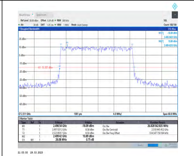
1-N41-30-30-L-1-DFT-QPSK-Outer_Full-75@0-Ant1 26.829-28.080-≤30-PASS
