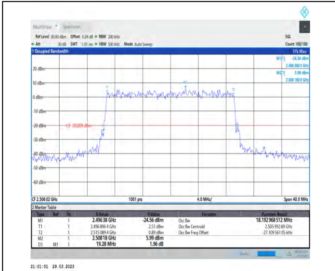
1-N41-30-20-L-9-CP-256QAM-Outer_Full-51@0-Ant 1-18.193-19.280-≤20-PASS
