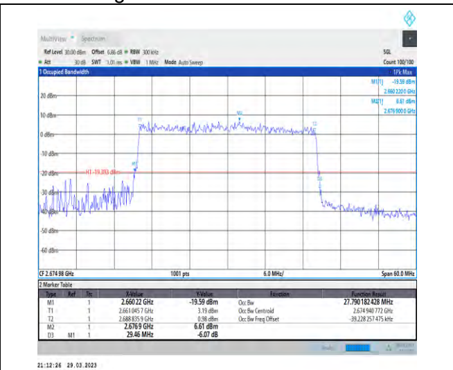
1-N41-30-30-H-9-CP-256QAM-Outer_Full-78@0-Ant1 1-27.79-29.460-≤30-PASS
