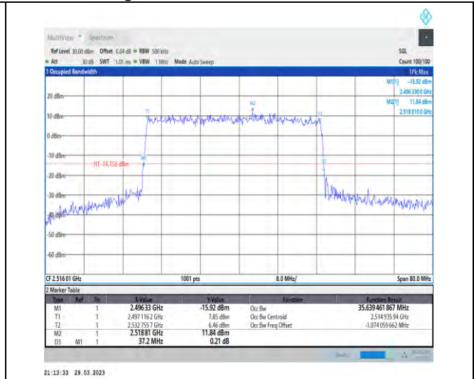
1-N41-30-40-L-4-DFT-64QAM-Outer_Full-100@0-An t1-35.639-37.200-≤40-PASS
