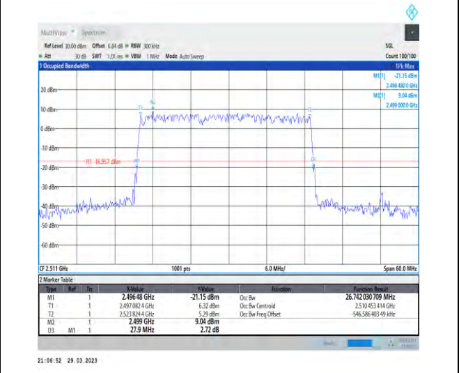
1-N41-30-30-L-5-DFT-256QAM-Outer_Full-75@0-Ant 1-26.742-27.900-≤30-PASS
