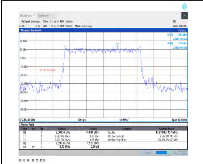
1-N41-30-20-M-2-DFT-PI2BPSK-Outer_Full-50@0-A nt1-17.879-18.720-≤20-PASS
