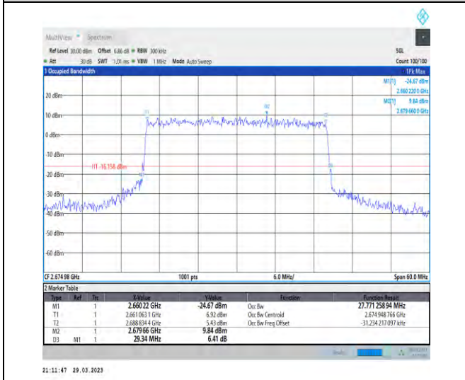
1-N41-30-30-H-6-CP-QPSK-Outer_Full-78@0-Ant1 27.771-29.340-≤30-PASS
