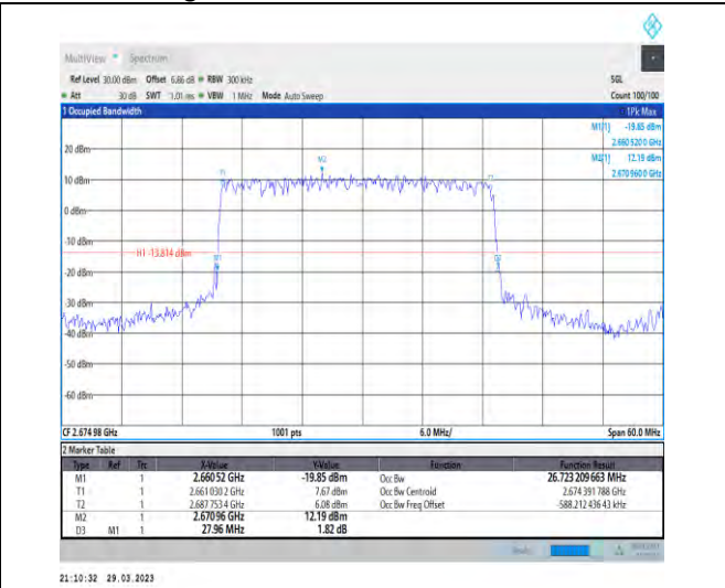
1-N41-30-30-H-1-DFT-QPSK-Outer_Full-75@0-Ant1-26.723-27.960-≤30-PASS
