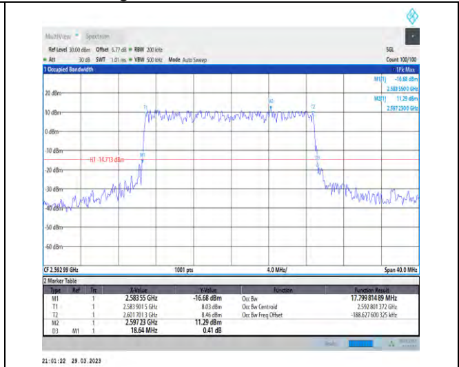
1-N41-30-20-M-1-DFT-QPSK-Outer_Full-50@0-Ant1 -17.8-18.640-≤20-PASS
