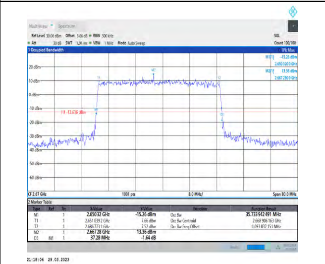
1-N41-30-40-H-4-DFT-64QAM-Outer_Full-100@0-Ant 1-35.734-37.280-≤40-PASS
