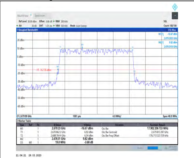
1-N41-30-20-H-4-DFT-64QAM-Outer_Full-50@0-Ant 1-17.902-19.000-≤20-PASS
