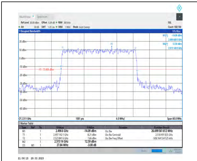
1-N41-30-30-L-2-DFT-PI2BPSK-Outer_Full-75@0-A nt1-26.7-27.840-≤30-PASS
