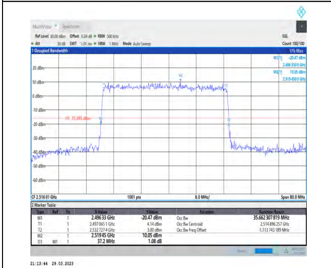
1-N41-30-40-L-5-DFT-256QAM-Outer_Full-100@0-A nt1-35.662-37.200-≤40-PASS
