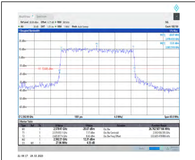
1-N41-30-30-M-1-DFT-QPSK-Outer_Full-75@0-Ant1 -26.763-27.960-≤30-PASS
