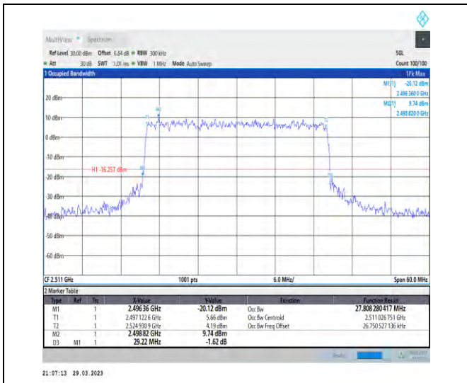
1-N41-30-30-L-6-CP-QPSK-Outer_Full-78@0-Ant1-27.808-29.220-≤30-PASS
