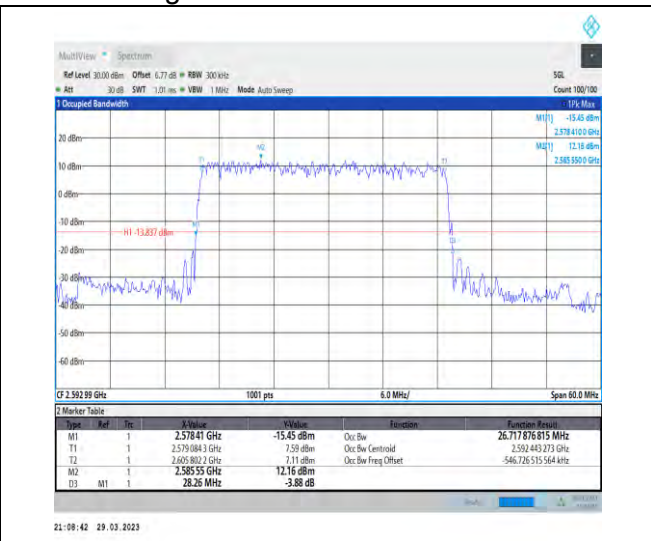
1-N41-30-30-M-2-DFT-PI2BPSK-Outer_Full-75@0-Ant1 -26.718-28.260-≤30-PASS
