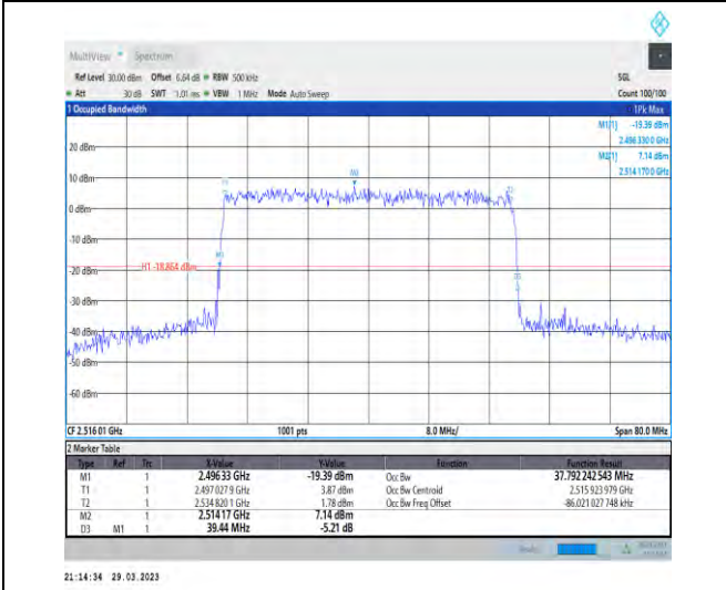
1-N41-30-40-L-9-CP-256QAM-Outer_Full-106@0-A nt1-37.792-39.440-≤40-PASS
