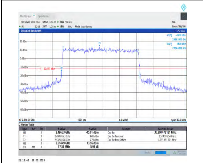
1-N41-30-40-L-1-DFT-QPSK-Outer_Full-100@0-Ant1 1-35.8-37.360-≤40-PASS
