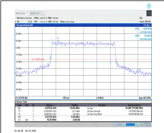
1-N41-30-20-H-7-CP-16QAM-Outer_Full-51@0-Ant1 -18.207-19.240-≤20-PASS
