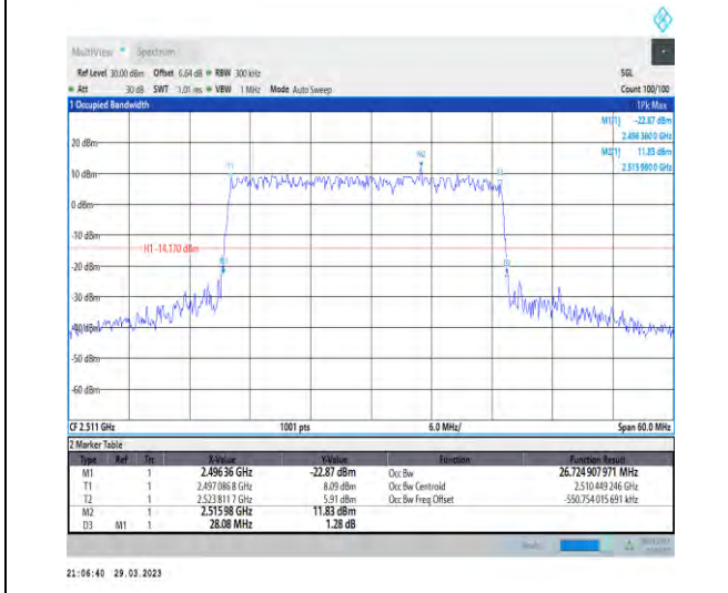
1-N41-30-30-L-4-DFT-64QAM-Outer_Full-75@0-Ant 1-26.725-28.080-≤30-PASS
