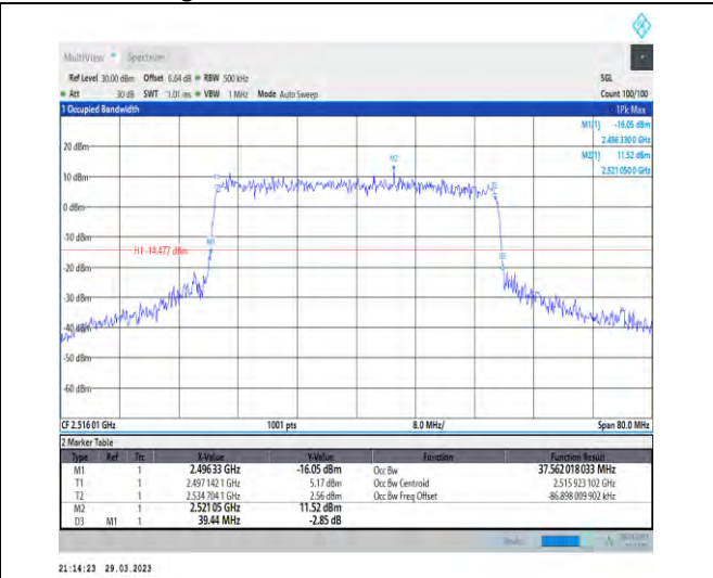
1-N41-30-40-L-8-CP-64QAM-Outer_Full-106@0-Ant 1-37.562-39.440-≤40-PASS
