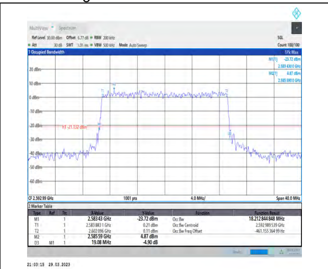
1-N41-30-20-M-9-CP-256QAM-Outer_Full-51@0-Ant 1-18.213-19.080-≤20-PASS
