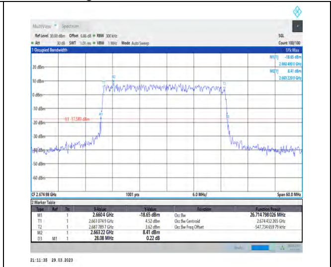
1-N41-30-30-H-5-DFT-256QAM-Outer_Full-75@0-Ant nt1-26.715-28.080-≤30-PASS
