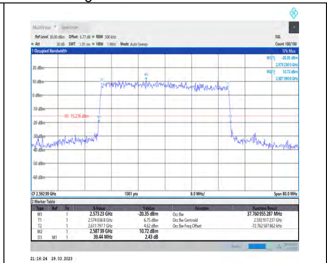
1-N41-30-40-M-7-CP-16QAM-Outer_Full-106@0-Ant1 -37.761-39.440-≤40-PASS
