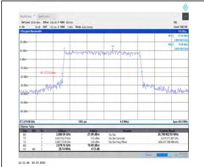
1-N41-30-30-H-4-DFT-64QAM-Outer_Full-75@0-Ant 1-26.701-28.140-≤30-PASS
