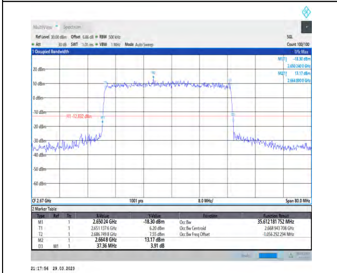
1-N41-30-40-H-3-DFT-16QAM-Outer_Full-100@0-Ant 1-35.612-37.360-≤40-PASS
