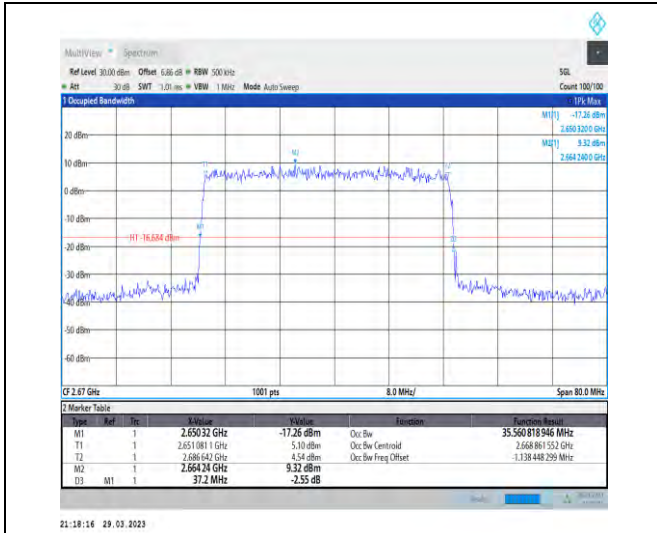
1-N41-30-40-H-5-DFT-256QAM-Outer_Full-100@0-Ant1-35.561-37.200-≤40-PASS
