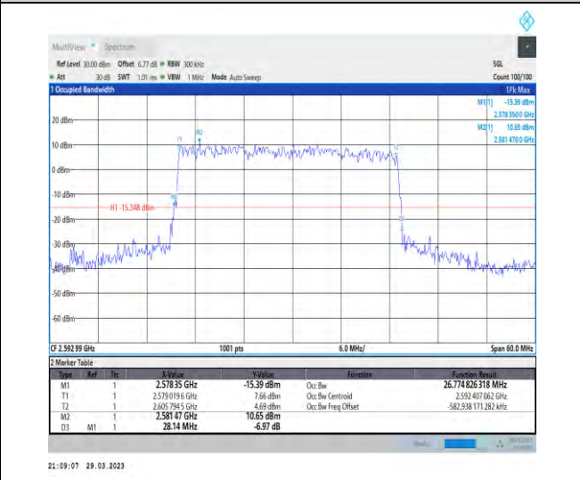
1-N41-30-30-M-4-DFT-64QAM-Outer_Full-75@0-Ant1 1-26.775-28.140-≤30-PASS
