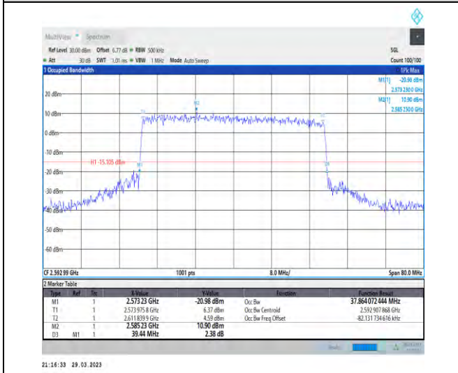
1-N41-30-40-M-8-CP-64QAM-Outer_Full-106@0-Ant1 t1-37.864-39.440-≤40-PASS
