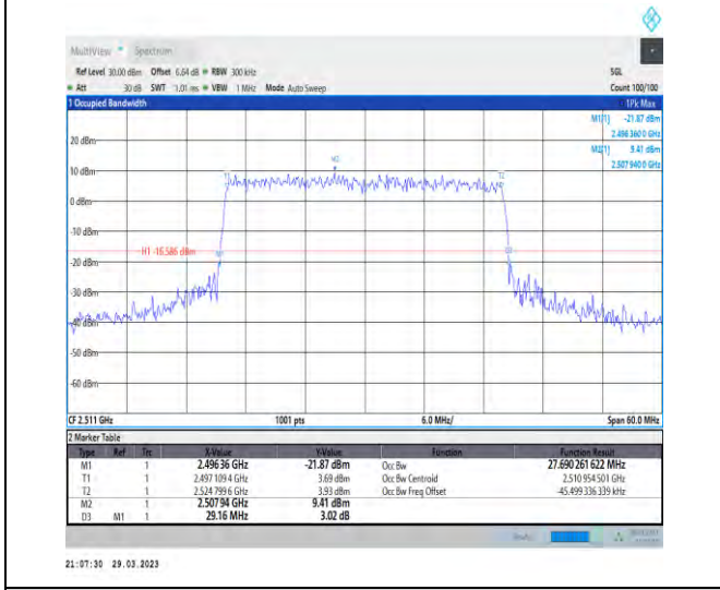
1-N41-30-30-L-8-CP-64QAM-Outer_Full-78@0-Ant1-27.69-29.160-≤30-PASS
