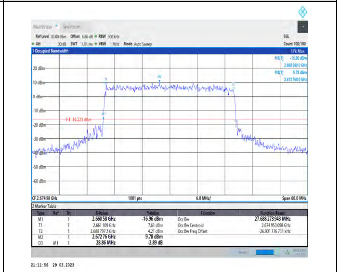
1-N41-30-30-H-7-CP-16QAM-Outer_Full-78@0-Ant1 -27.688-28.860-≤30-PASS
