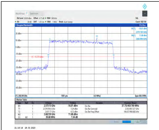
1-N41-30-40-M-6-CP-QPSK-Outer_Full-106@0-Ant1 -37.753-39.680-≤40-PASS
