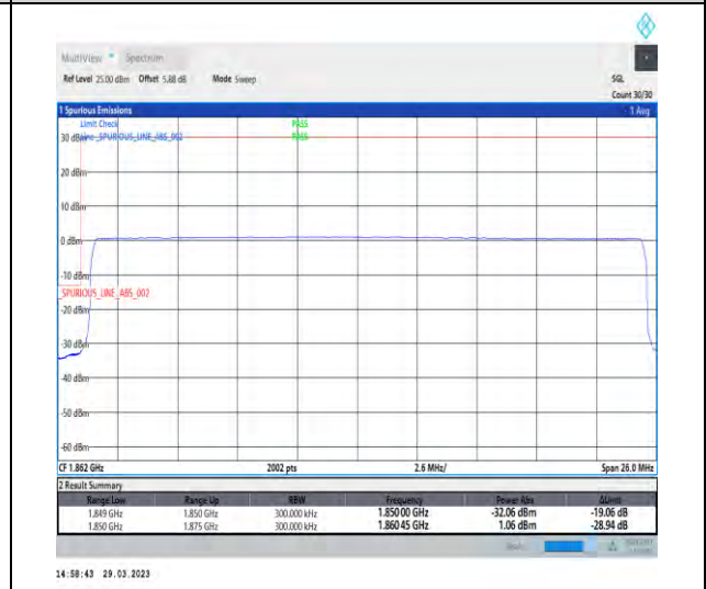
1-N25-15-25-L-6-CP-QPSK-Outer_Full-133@0-Ant1-1-seegraph-PASS-see graph
