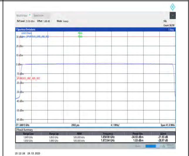
1-N25-15-40-L-6-CP-QPSK-Outer_Full-216@0-Ant1-1-seegraph-PASS-see graph
