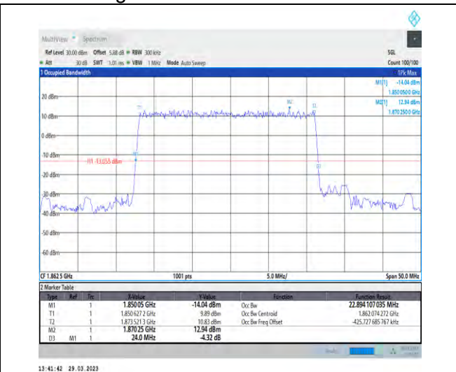
1-N25-15-25-L-2-DFT-PI2BPSK-Outer_Full-128@0-Ant 1-22.894-24.000-≤25-PASS
