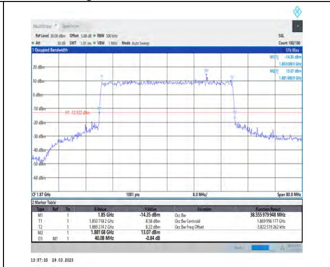
1-N25-15-40-L-8-CP-64QAM-Outer_Full-216@0-Ant 1-38.556-40.080-≤40-PASS
