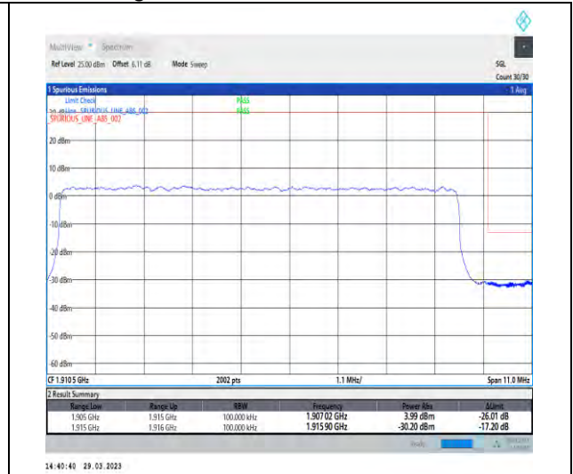
1-N25-15-10-H-3-DFT-PI2BPSK-Outer_Full-50@0-Ant1-1-seegraph-PASS-see graph
