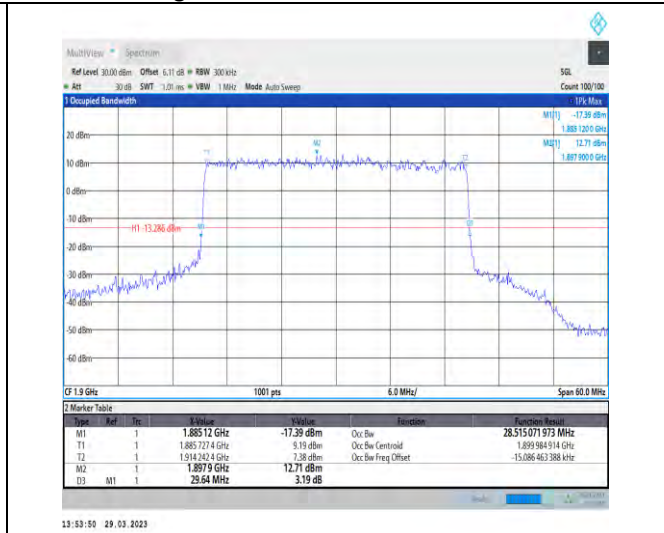
1-N25-15-30-H-1-DFT-QPSK-Outer_Full-160@0-Ant 1-28.515-29.640-≤30-PASS
