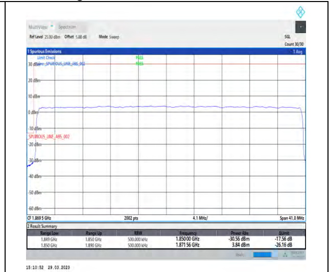
1-N25-15-40-L-3-DFT-PI2BPSK-Outer_Full-216@0-Ant1-1-seegraph-PASS-see graph
