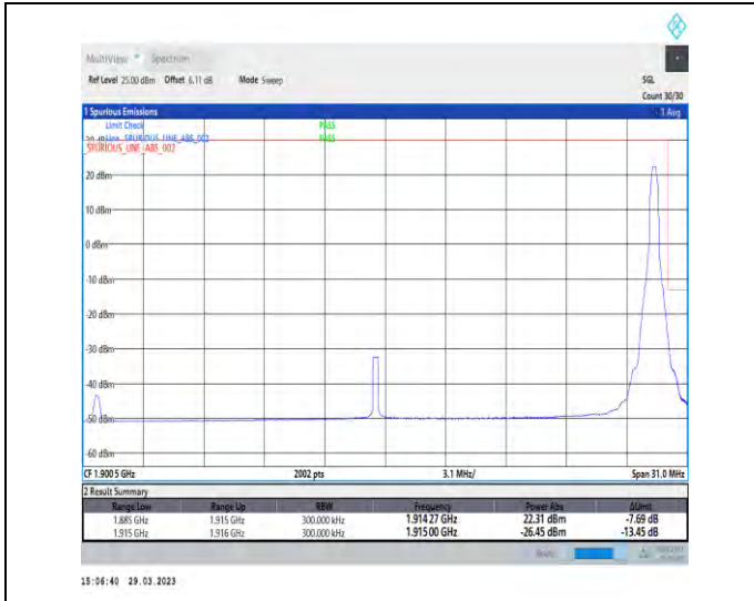
1-N25-15-30-H-2-DFT-PI2BPSK-Edge_1RB_Right-1@159-Ant1-1-seegraph-PASS-see graph
