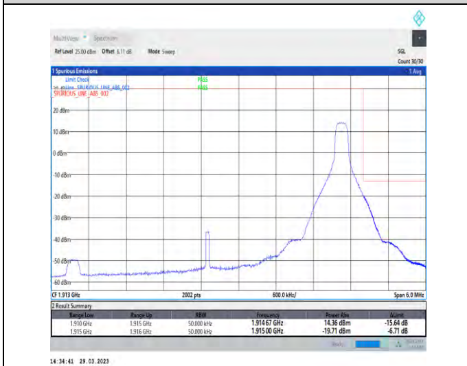
1-N25-15-5-H-5-CP-QPSK-Edge_1RB_Right-1@24-Ant1-1-seegraph-PASS-see graph
