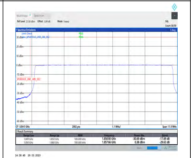
1-N25-15-10-L-6-CP-QPSK-Outer_Full-52@0-Ant1-1-seegraph-PASS-see graph
