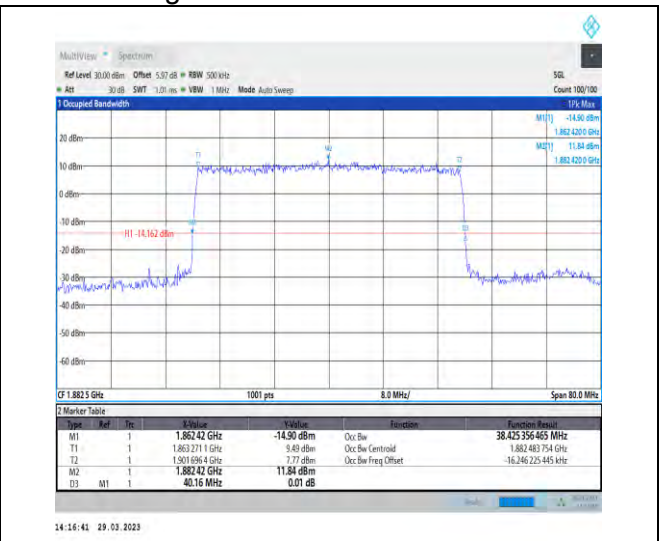
1-N25-15-40-M-7-CP-16QAM-Outer_Full-216@0-Ant1 1-38.425-40.160-≤40-PASS
