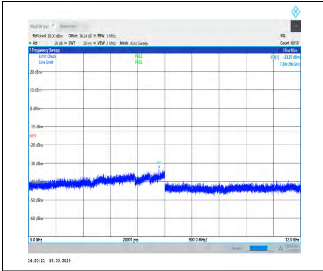
1-N25-15-40-L-1-DFT-PI2BPSK-Inner_1RB_Left-1 @ 1-3000-12000-Ant1-7309.20--33.07--13-PASS
