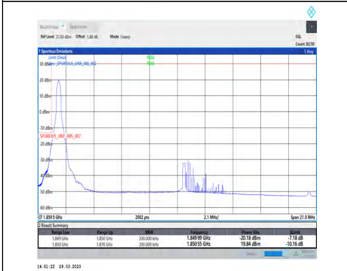
1-N25-15-20-L-4-CP-QPSK-Edge_1RB_Left-1@0-Ant1-1-seegraph-PASS-see graph
