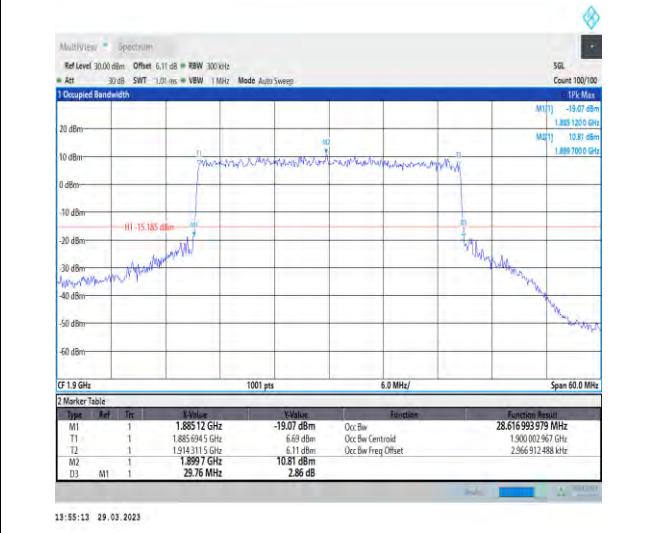
1-N25-15-30-H-7-CP-16QAM-Outer_Full-160@0-Ant1 1-28.617-29.760-≤30-PASS
