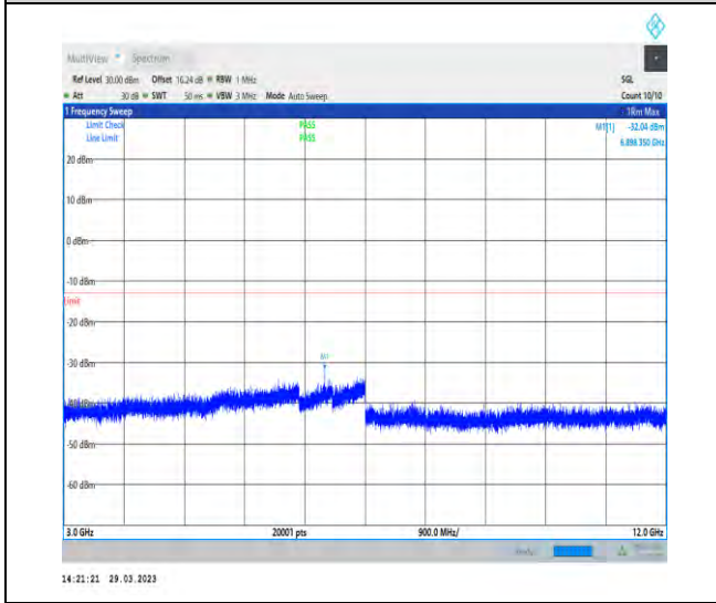
1-N25-15-40-M-1-DFT-PI2BPSK-Inner_1RB_Left-1 @ 1-3000-12000-Ant1-6898.35--32.04--13-PASS
