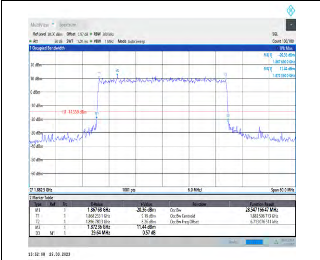
1-N25-15-30-M-3-DFT-16QAM-Outer_Full-160@0-Ant 1-28.547-29.640-≤30-PASS
