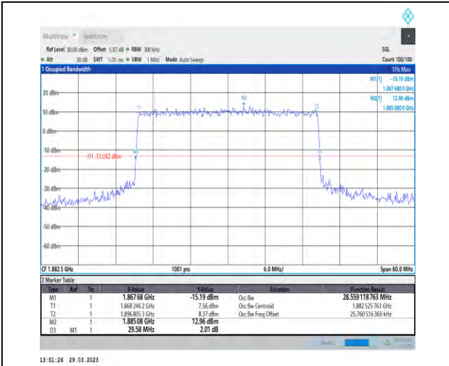
1-N25-15-30-M-1-DFT-QPSK-Outer_Full-160@0-Ant 1-28.559-29.580-≤30-PASS
