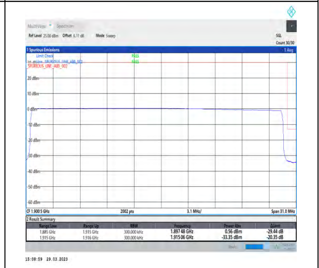
1-N25-15-30-H-6-CP-QPSK-Outer_Full-160@0-Ant1-1-seegraph-PASS-see graph
