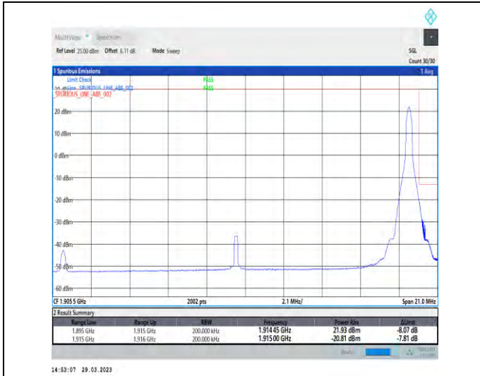
1-N25-15-20-H-2-DFT-PI2BPSK-Edge_1RB_Right-1@105-Ant1-1-seegraph-PASS-see graph
