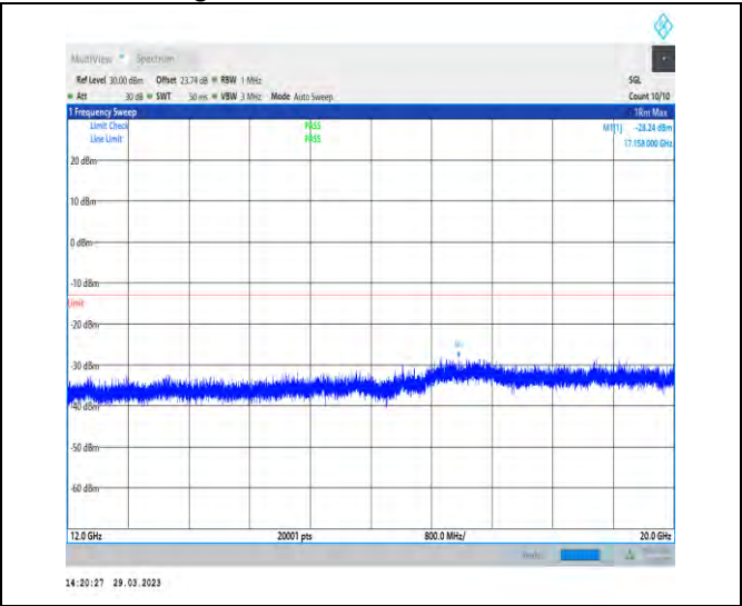
1-N25-15-40-L-1-DFT-PI2BPSK-Inner_1RB_Left-1 @ 1-12000-20000-Ant1-17158.00--28.24--13-PASS
