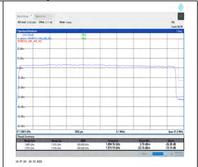
1-N25-15-30-H-3-DFT-PI2BPSK-Outer_Full-160@0-Ant1-1-seegraph-PASS-see graph
