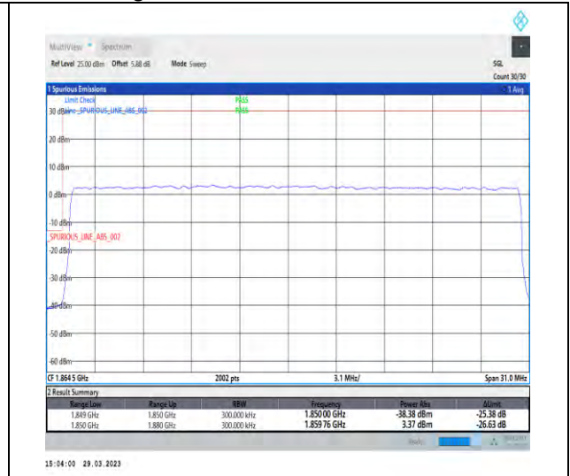
1-N25-15-30-L-3-DFT-PI2BPSK-Outer_Full-160@0-Ant1-1-seegraph-PASS-see graph
