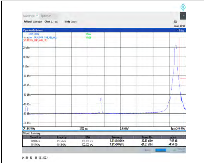
1-N25-15-25-H-2-DFT-PI2BPSK-Edge_1RB_Right-1@132-Ant1-1-seegraph-PASS-see graph
