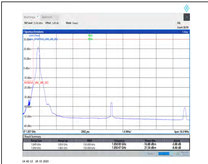
1-N25-15-15-L-1-DFT-PI2BPSK-Edge_1RB_Left-1@0-Ant1-1-seegraph-PASS-see graph
