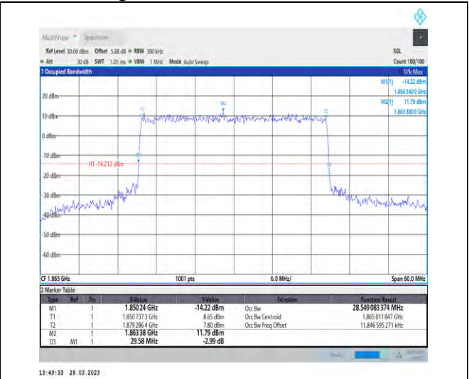
1-N25-15-30-L-3-DFT-16QAM-Outer_Full-160@0-An t1-28.549-29.580-≤30-PASS
