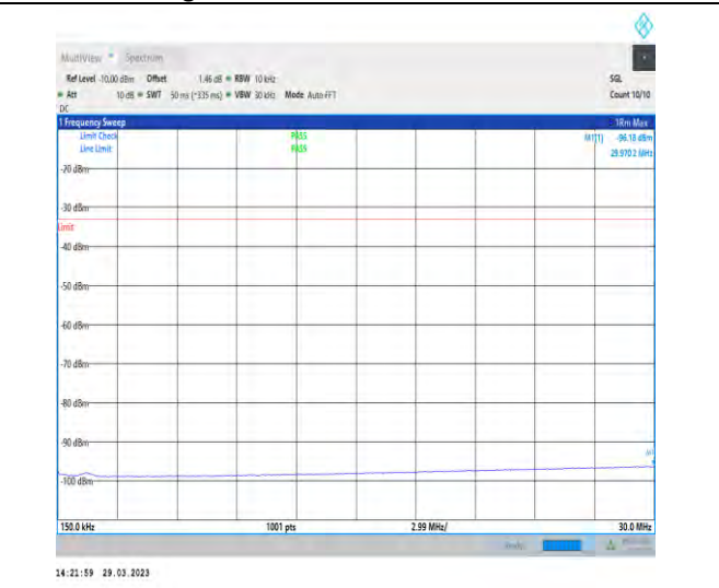
1-N25-15-40-H-1-DFT-PI2BPSK-Inner_1RB_Left-1 @ 1-0.15-30-Ant1-29.97--96.18--33-PASS
