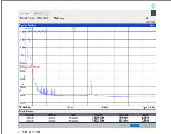
1-N25-15-20-L-1-DFT-PI2BPSK-Edge_1RB_Left-1@0-Ant1-1-seegraph-PASS-see graph
