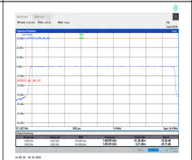
1-N25-15-15-L-6-CP-QPSK-Outer_Full-79@0-Ant1-1-seegraph-PASS-see graph
