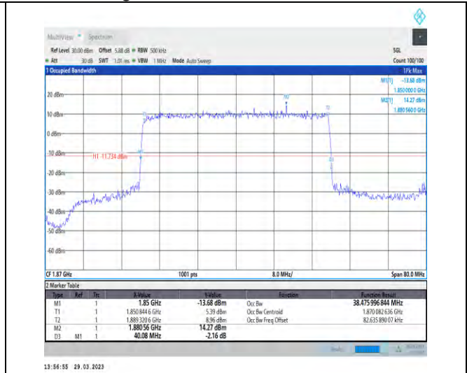
1-N25-15-40-L-4-DFT-64QAM-Outer_Full-216@0-An t1-38.476-40.080-≤40-PASS
