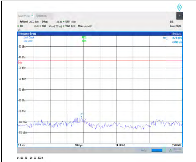
1-N25-15-40-H-1-DFT-PI2BPSK-Inner_1RB_Left-1 @ 1-0.009-0.15-Ant1-0.06--96.10--43-PASS
