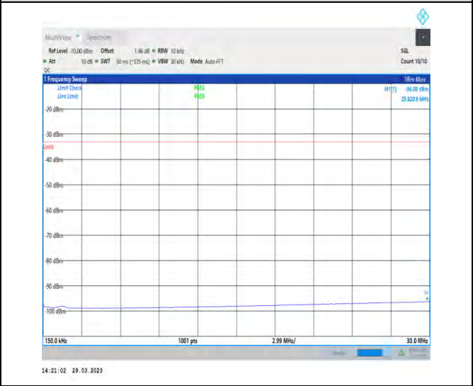
1-N25-15-40-M-1-DFT-PI2BPSK-Inner_1RB_Left-1 @ 1-0.15-30-Ant1-29.82--96.09--33-PASS
