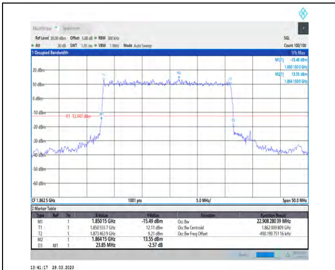
1-N25-15-25-L-1-DFT-QPSK-Outer_Full-128@0-Ant 1-22.908-23.850-≤25-PASS
