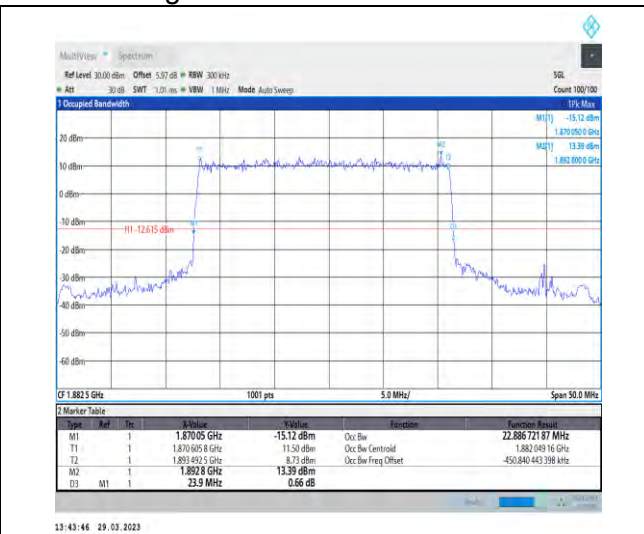
1-N25-15-25-M-1-DFT-QPSK-Outer_Full-128@0-Ant 1-22.887-23.900-≤25-PASS
