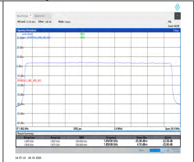
1-N25-15-25-L-3-DFT-PI2BPSK-Outer_Full-128@0-Ant1-1-seegraph-PASS-see graph
