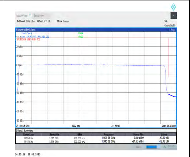
1-N25-15-20-H-6-CP-QPSK-Outer_Full-106@0-Ant1-1-seegraph-PASS-see graph
