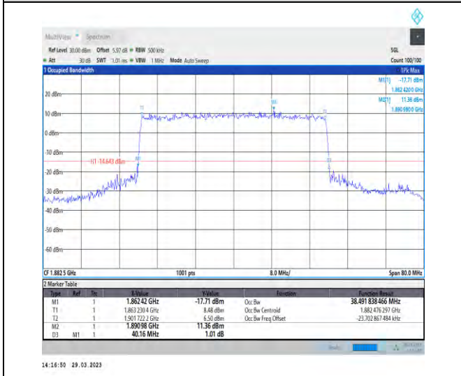
1-N25-15-40-M-8-CP-64QAM-Outer_Full-216@0-Ant1 1-38.492-40.160-≤40-PASS
