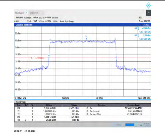
1-N25-15-30-M-4-DFT-64QAM-Outer_Full-160@0-Ant 1-28.543-29.580-≤30-PASS
