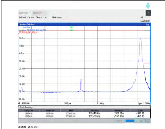
1-N25-15-20-H-5-CP-QPSK-Edge_1RB_Right-1@105-Ant1-1-seegraph-PASS-see graph
