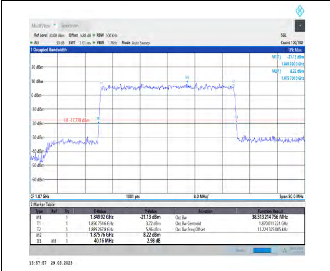
1-N25-15-40-L-9-CP-256QAM-Outer_Full-216@0-Ant t1-38.513-40.160-≤40-PASS
