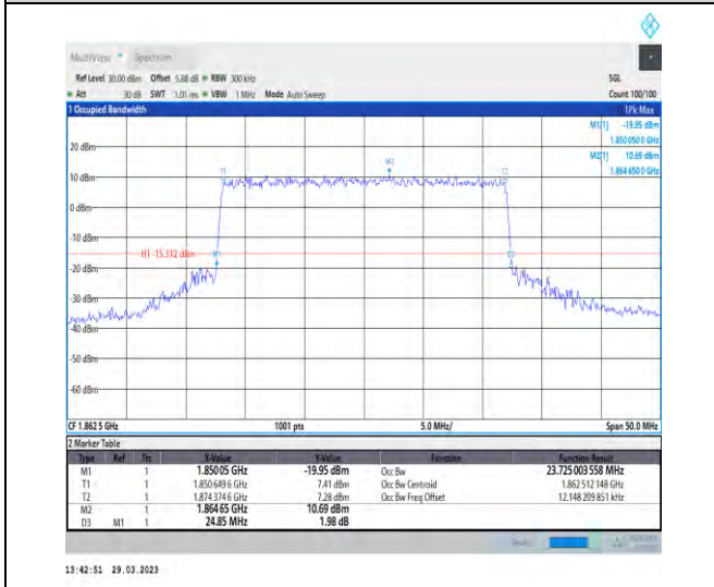
1-N25-15-25-L-7-CP-16QAM-Outer_Full-133@0-Ant 1-23.725-24.850-≤25-PASS
