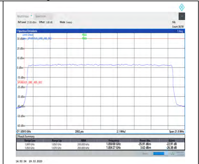
1-N25-15-20-L-3-DFT-PI2BPSK-Outer_Full-100@0-Ant1-1-seegraph-PASS-see graph
