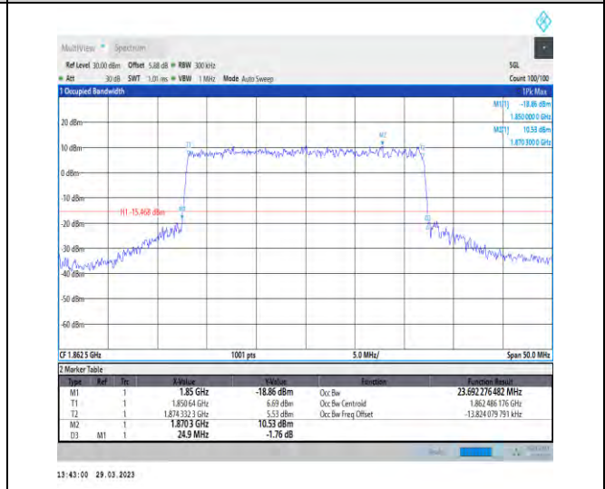
1-N25-15-25-L-8-CP-64QAM-Outer_Full-133@0-Ant 1-23.692-24.900-≤25-PASS
