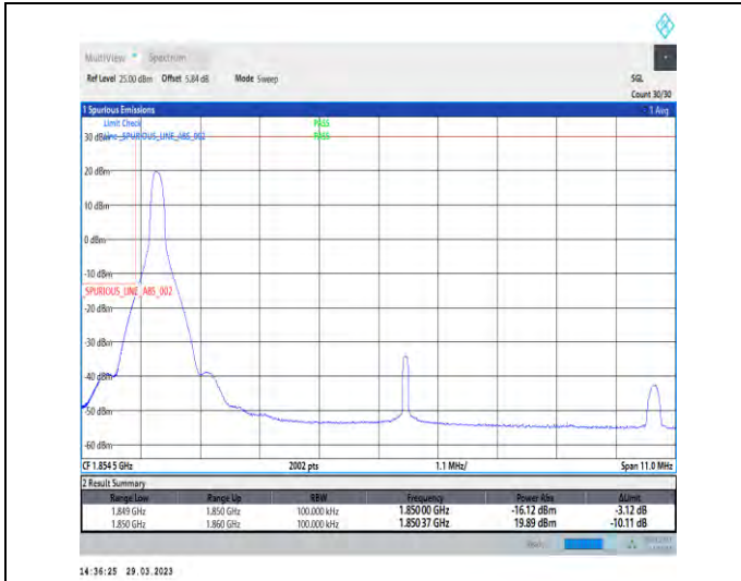
1-N25-15-10-L-1-DFT-PI2BPSK-Edge_1RB_Left-1@0-Ant1-1-seegraph-PASS-see graph
