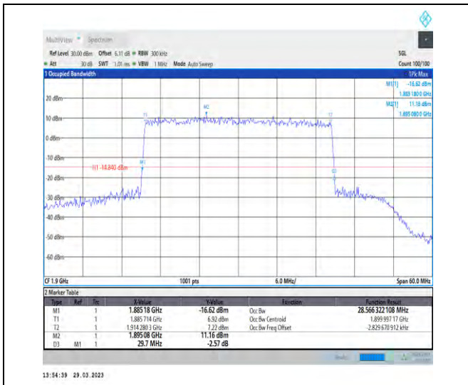
1-N25-15-30-H-4-DFT-64QAM-Outer_Full-160@0-A Ant1-28.566-29.700-≤30-PASS
