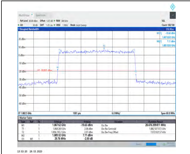
1-N25-15-30-M-9-CP-256QAM-Outer_Full-160@0-A nt1-28.476-29.760-≤30-PASS
