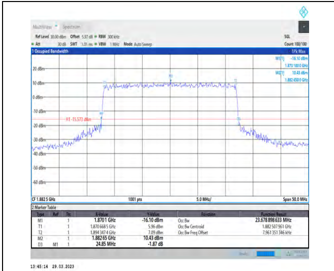
1-N25-15-25-M-8-CP-64QAM-Outer_Full-133@0-Ant 1-23.679-24.850-≤25-PASS
