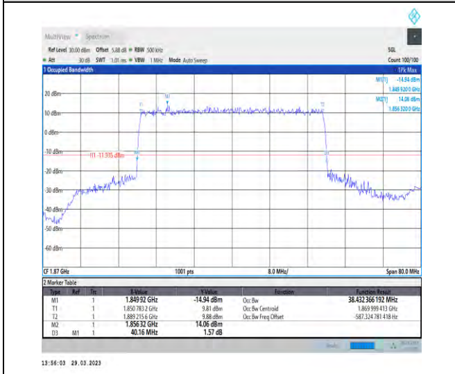
1-N25-15-40-L-1-DFT-QPSK-Outer_Full-216@0-Ant 1-38.432-40.160-≤40-PASS
