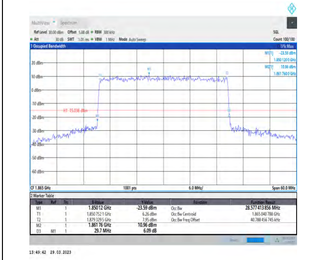
1-N25-15-30-L-4-DFT-64QAM-Outer_Full-160@0-An t1-28.577-29.700-≤30-PASS
