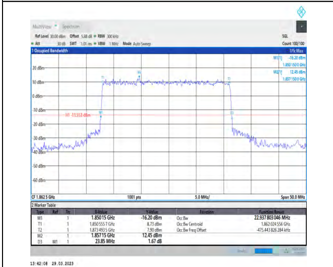
1-N25-15-25-L-3-DFT-16QAM-Outer_Full-128@0-Ant t1-22.938-23.850-≤25-PASS
