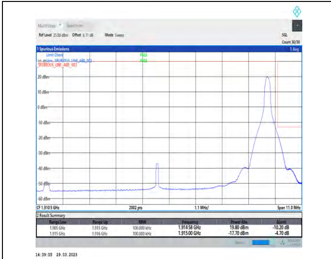
1-N25-15-10-H-2-DFT-PI2BPSK-Edge_1RB_Right-1@51-Ant1-1-seegraph-PASS-see graph
