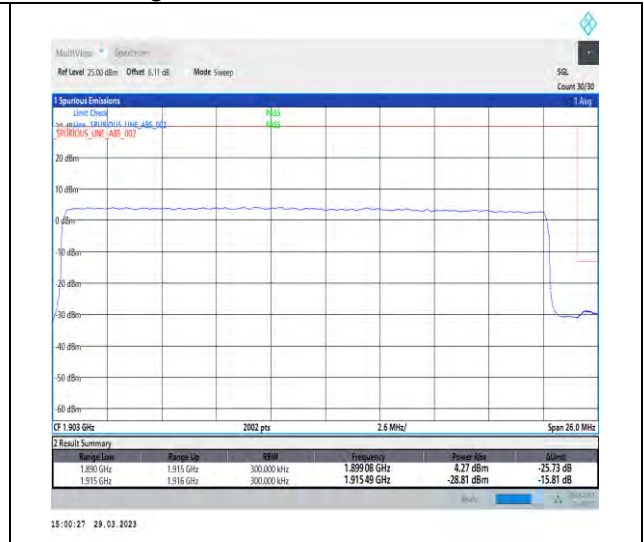
1-N25-15-25-H-3-DFT-PI2BPSK-Outer_Full-128@0-Ant1-1-seegraph-PASS-see graph
