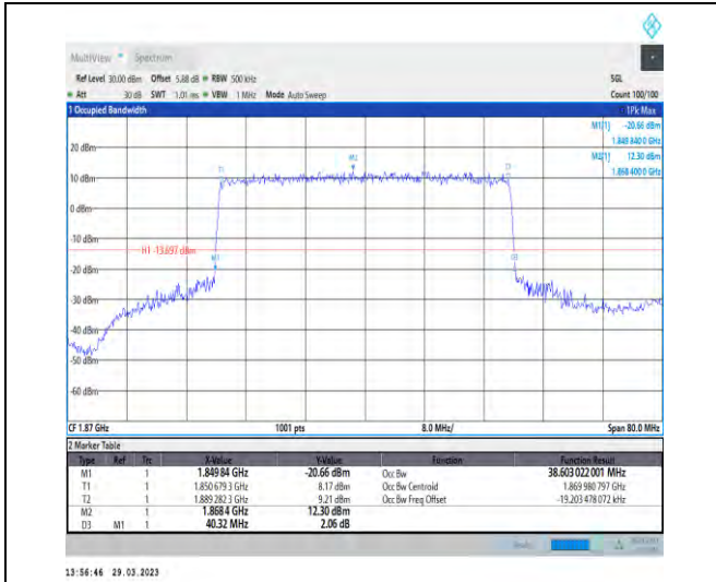
1-N25-15-40-L-3-DFT-16QAM-Outer_Full-216@0-An t1-38.603-40.320-≤40-PASS
