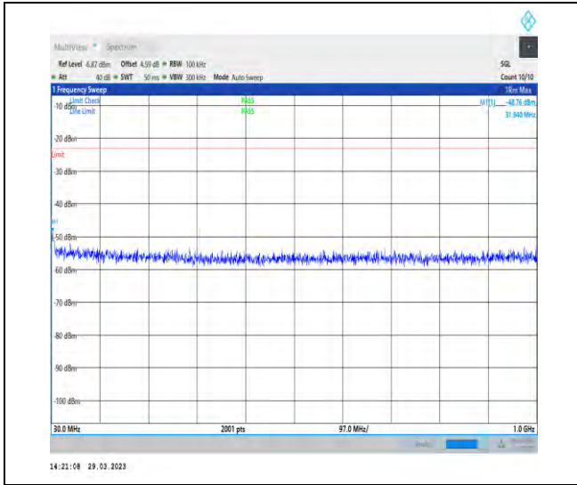
1-N25-15-40-M-1-DFT-PI2BPSK-Inner_1RB_Left-1 @ 1-30-1000-Ant1-31.94--48.76--23-PASS
