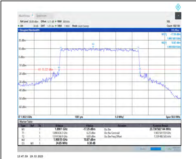
1-N25-15-25-H-7-CP-16QAM-Outer_Full-133@0-Ant 1-23.731-24.850-≤25-PASS
