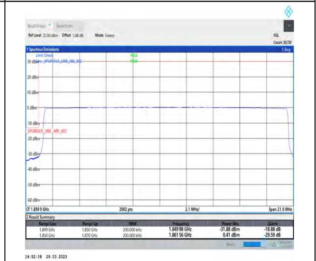
1-N25-15-20-L-6-CP-QPSK-Outer_Full-106@0-Ant1-1-seegraph-PASS-see graph
