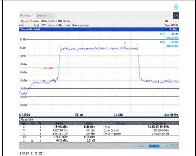
1-N25-15-40-L-6-CP-QPSK-Outer_Full-216@0-Ant1- 38.5-40.160-≤40-PASS
