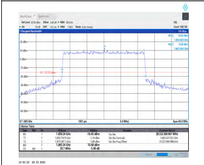
1-N25-15-30-L-8-CP-64QAM-Outer_Full-160@0-Ant 1-28.532-29.700-≤30-PASS
