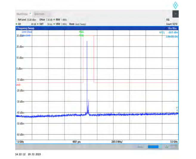
1-N25-15-40-H-1-DFT-PI2BPSK-Inner_1RB_Left-1 @ 1-1000-3000-Ant1-2984.00--38.91--13-PASS
