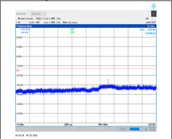
1-N25-15-40-H-1-DFT-PI2BPSK-Inner_1RB_Left-1@ 1-12000-20000-Ant1-17268.00--28.29--13-PASS
