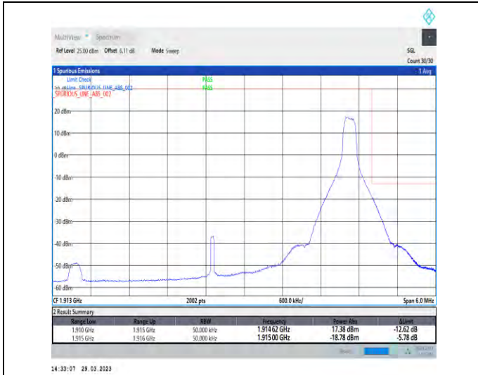
1-N25-15-5-H-2-DFT-PI2BPSK-Edge_1RB_Right-1@2-4-Ant1-1-seegraph-PASS-see graph
