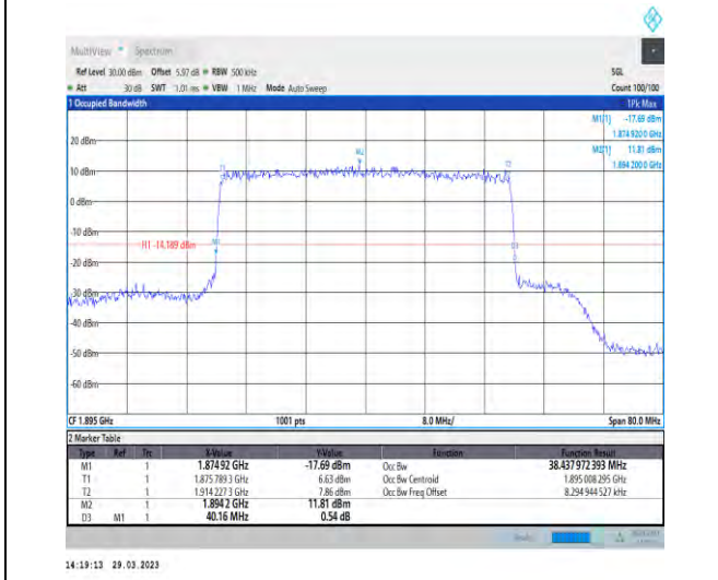
1-N25-15-40-H-7-CP-16QAM-Outer_Full-216@0-Ant1-38.438-40.160-≤40-PASS
