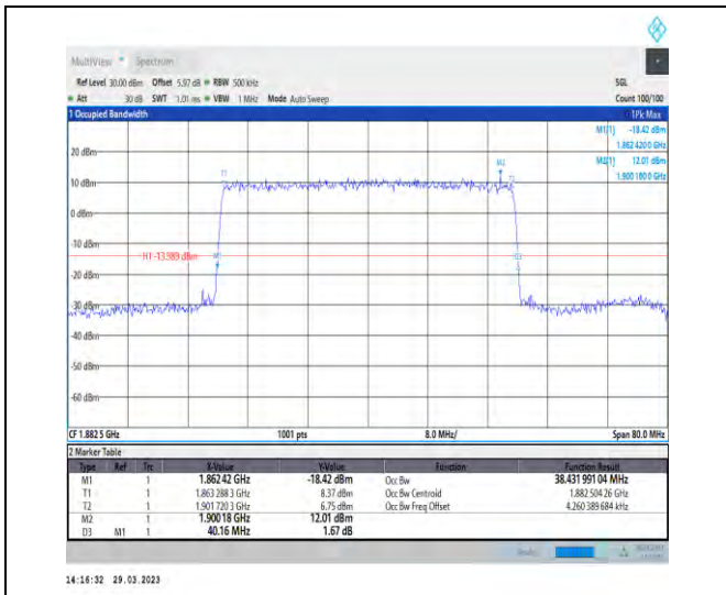
1-N25-15-40-M-6-CP-QPSK-Outer_Full-216@0-Ant1 -1-38.432-40.160-≤40-PASS
