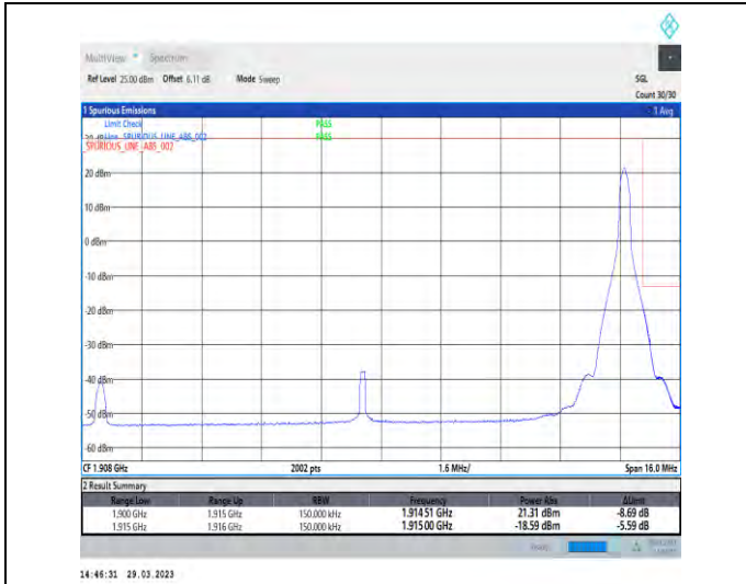
1-N25-15-15-H-2-DFT-PI2BPSK-Edge_1RB_Right-1@78-Ant1-1-seegraph-PASS-see graph
