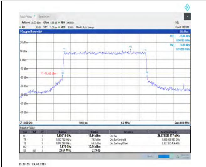
1-N25-15-30-L-6-CP-QPSK-Outer_Full-160@0-Ant-1 28.574-29.640-≤30-PASS
