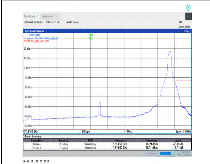
1-N25-15-10-H-5-CP-QPSK-Edge_1RB_Right-1@51-Ant1-1-seegraph-PASS-see graph
