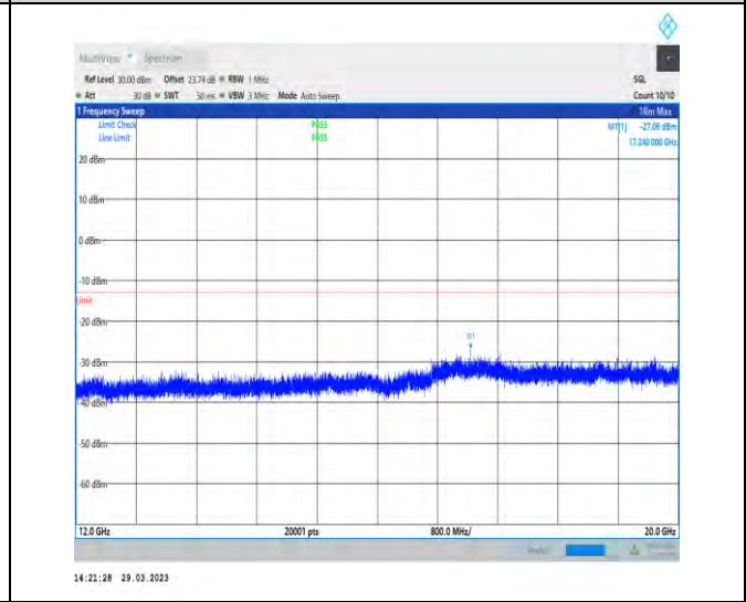
1-N25-15-40-M-1-DFT-PI2BPSK-Inner_1RB_Left-1 @ 1-12000-20000-Ant1-17240.00--27.09--13-PASS
