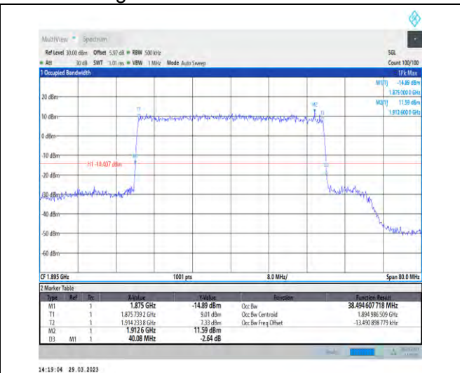
1-N25-15-40-H-6-CP-QPSK-Outer_Full-216@0-Ant1-38.495-40.080-≤40-PASS
