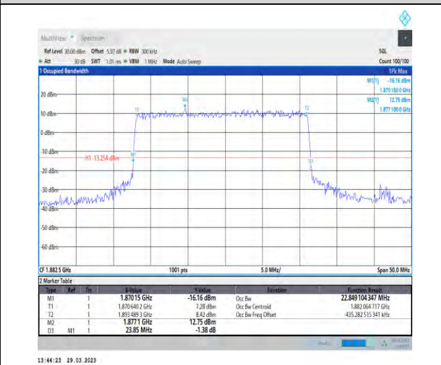
1-N25-15-25-M-3-DFT-16QAM-Outer_Full-128@0-Ant nt1-22.849-23.850-≤25-PASS
