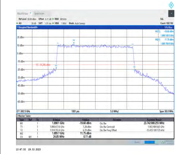
1-N25-15-25-H-6-CP-QPSK-Outer_Full-133@0-Ant1 -23.742-24.850-≤25-PASS
