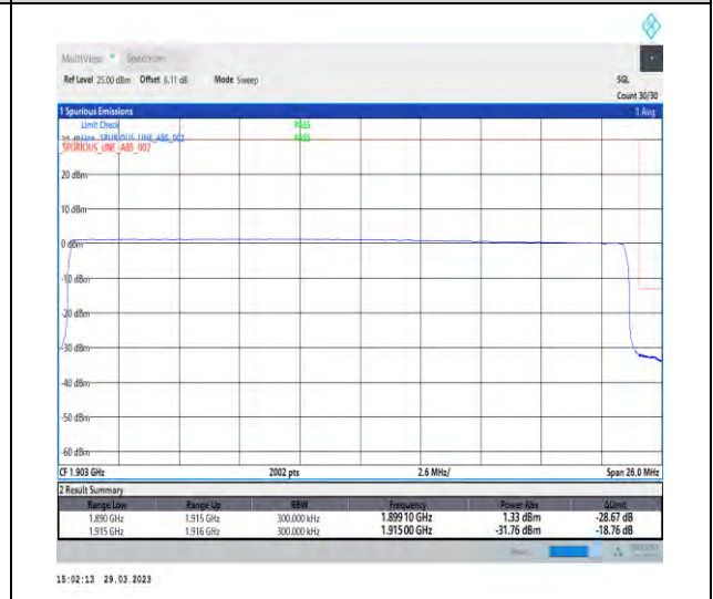
1-N25-15-25-H-6-CP-QPSK-Outer_Full-133@0-Ant1-1-seegraph-PASS-see graph
