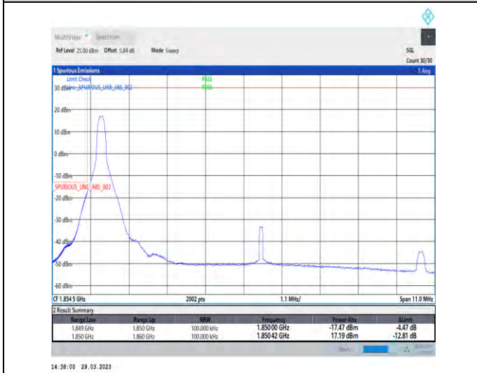
1-N25-15-10-L-4-CP-QPSK-Edge_1RB_Left-1@0-Ant1-1-seegraph-PASS-see graph
