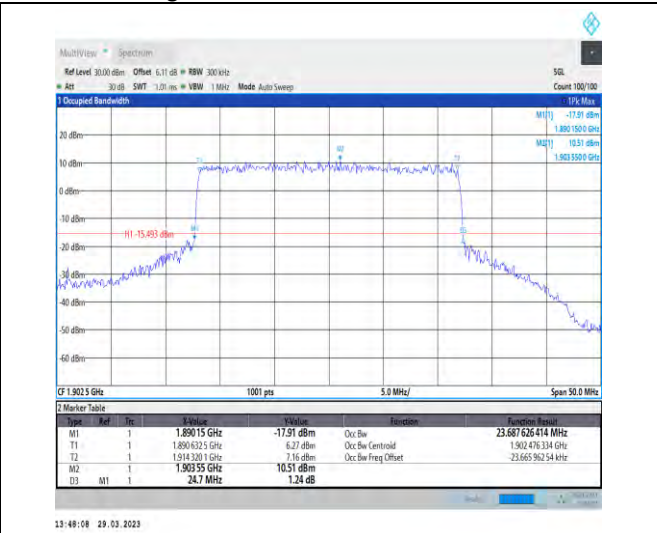
1-N25-15-25-H-8-CP-64QAM-Outer_Full-133@0-Ant 1-23.688-24.700-≤25-PASS
