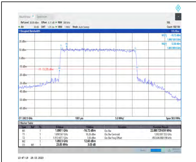
1-N25-15-25-H-3-DFT-16QAM-Outer_Full-128@0-A nt1-22.881-23.850-≤25-PASS
