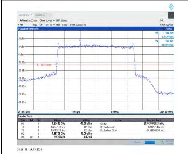
1-N25-15-40-H-3-DFT-16QAM-Outer_Full-216@0-Ant 1-38.443-40.160-≤40-PASS
