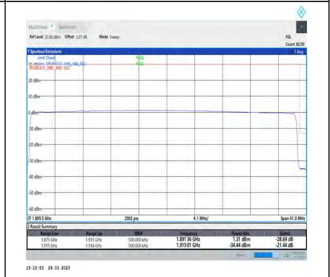
1-N25-15-40-H-6-CP-QPSK-Outer_Full-216@0-Ant1-1-seegraph-PASS-see graph
