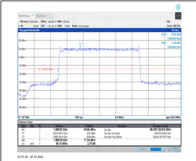
1-N25-15-40-L-7-CP-16QAM-Outer_Full-216@0-Ant 1-38.539-40.160-≤40-PASS
