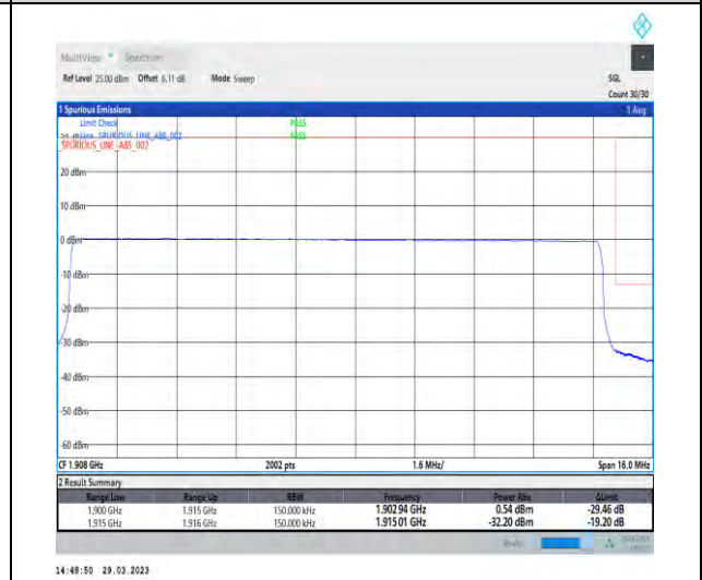
1-N25-15-15-H-6-CP-QPSK-Outer_Full-79@0-Ant1-1-seegraph-PASS-see graph
