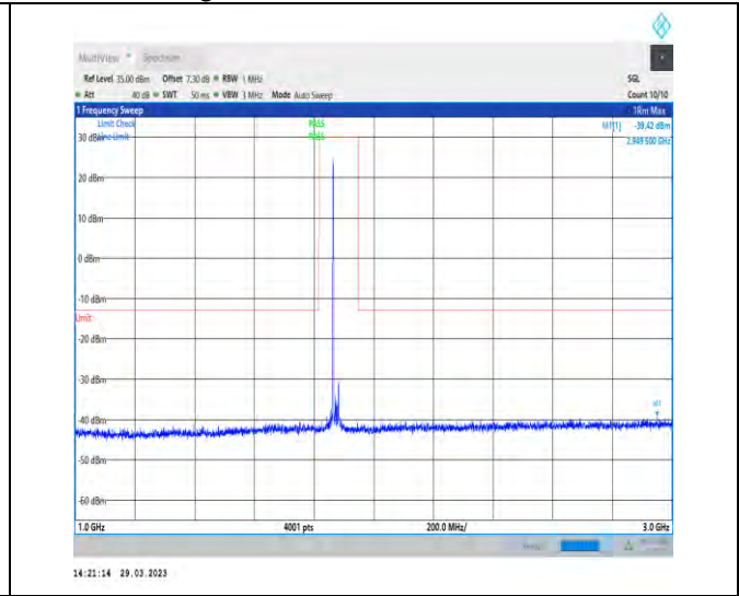
1-N25-15-40-M-1-DFT-PI2BPSK-Inner_1RB_Left-1 @ 1-1000-3000-Ant1-2949.50--39.42--13-PASS
