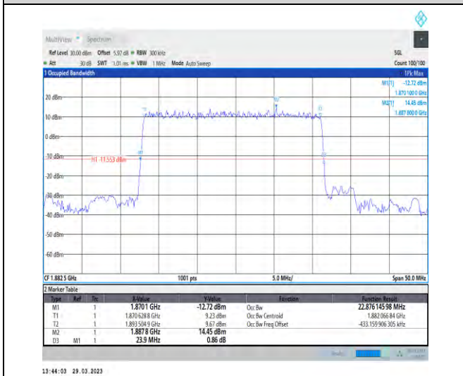
1-N25-15-25-M-2-DFT-PI2BPSK-Outer_Full-128@0-Ant Ant1-22.876-23.900-≤25-PASS
