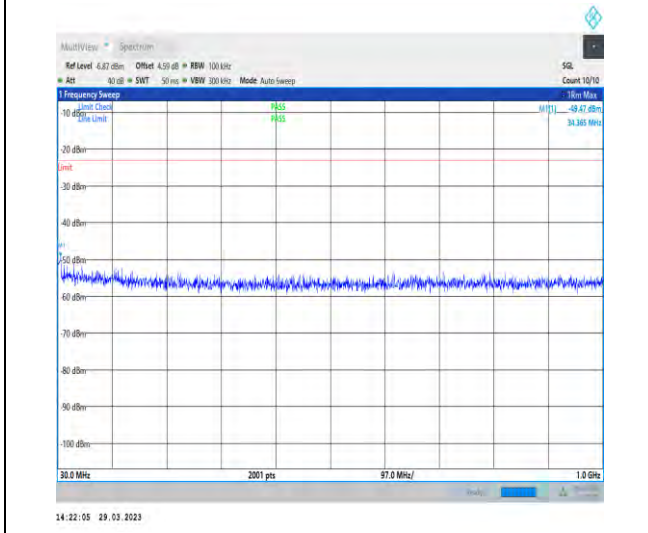
1-N25-15-40-H-1-DFT-PI2BPSK-Inner_1RB_Left-1 @ 1-30-1000-Ant1-34.37--49.47--23-PASS
