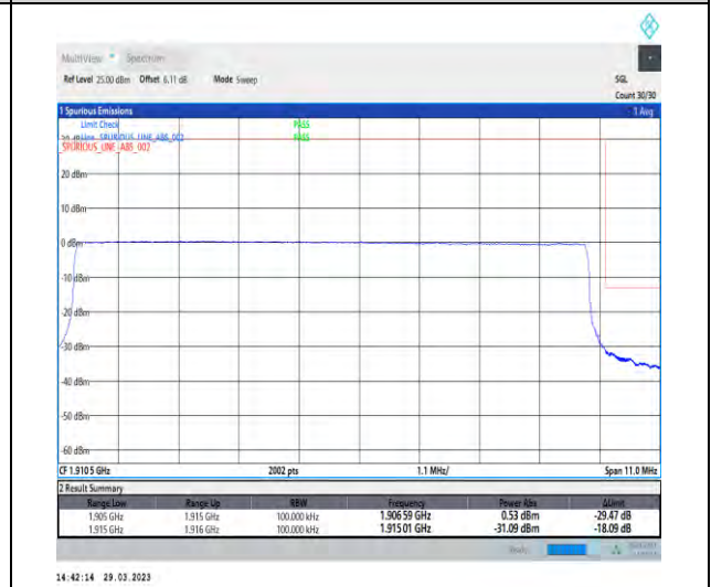
1-N25-15-10-H-6-CP-QPSK-Outer_Full-52@0-Ant1-1-seegraph-PASS-see graph
