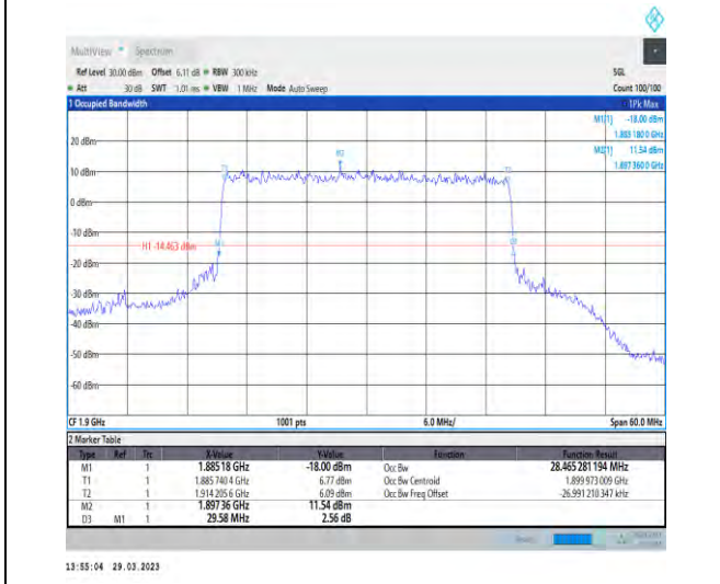
1-N25-15-30-H-6-CP-QPSK-Outer_Full-160@0-Ant1 -28.465-29.580-≤30-PASS
