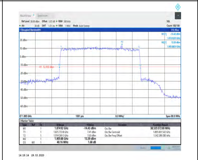
1-N25-15-40-H-4-DFT-64QAM-Outer_Full-216@0-Ant 1-38.536-40.160-≤40-PASS
