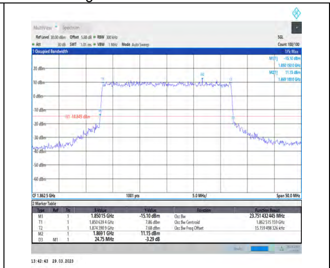
1-N25-15-25-L-6-CP-QPSK-Outer_Full-133@0-Ant1- 23.751-24.750-≤25-PASS
