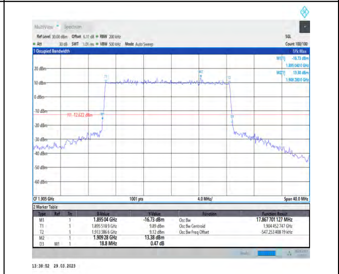
1-N25-15-20-H-1-DFT-QPSK-Outer_Full-100@0-Ant 1-17.868-18.800-≤20-PASS
