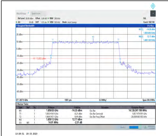
1-N25-15-15-L-7-CP-16QAM-Outer_Full-79@0-Ant1 -14.126-14.910-≤15-PASS
