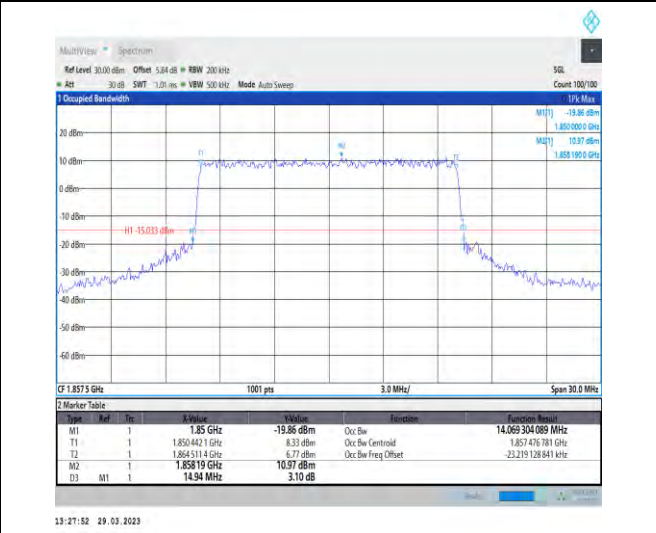
1-N25-15-15-L-6-CP-QPSK-Outer_Full-79@0-Ant1-1 4.069-14.940-≤15-PASS
