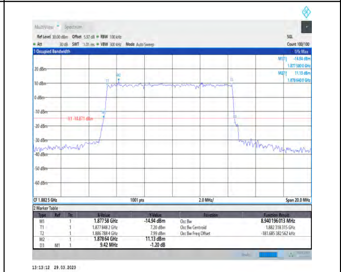
1-N25-15-10-M-4-DFT-64QAM-Outer_Full-50@0-Ant 1-8.94-9.420-≤10-PASS
