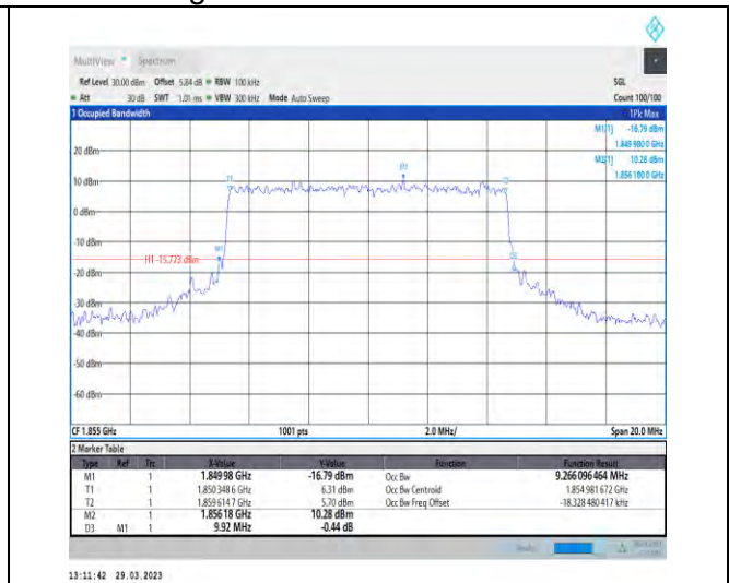
1-N25-15-10-L-7-CP-16QAM-Outer_Full-52@0-Ant1 -9.266-9.920≤10-PASS
