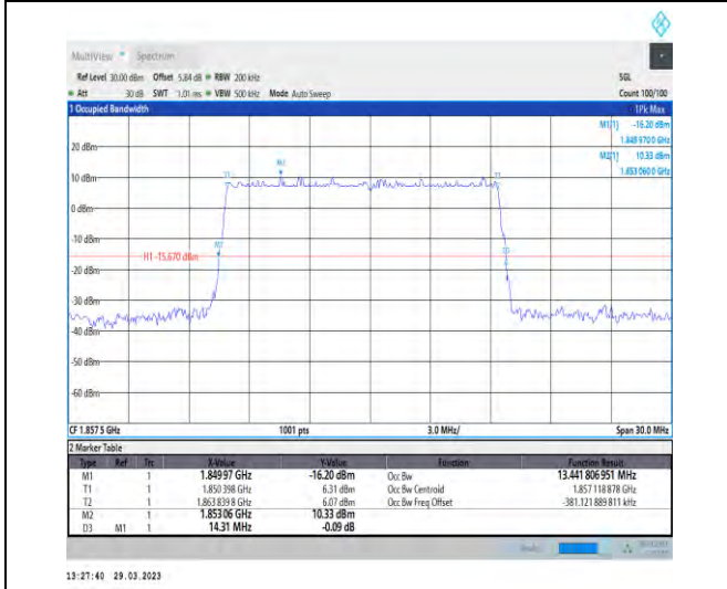
1-N25-15-15-L-5-DFT-256QAM-Outer_Full-75@0-Ant t1-13.442-14.310-≤15-PASS
