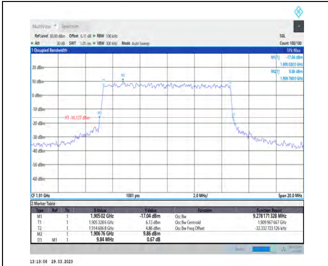
1-N25-15-10-H-8-CP-64QAM-Outer_Full-52@0-Ant1 -9.278-9.840-≤10-PASS
