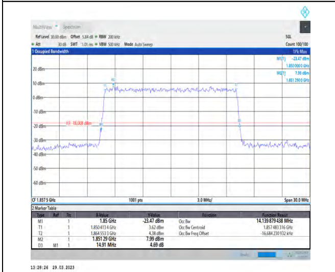
1-N25-15-15-L-9-CP-256QAM-Outer_Full-79@0-Ant 1-14.14-14.910-≤15-PASS
