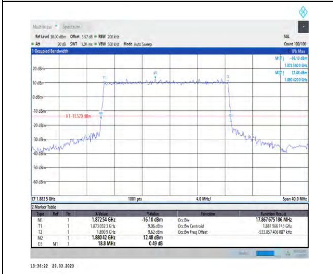
1-N25-15-20-M-1-DFT-QPSK-Outer_Full-100@0-Ant 1-17.868-18.800-≤20-PASS
