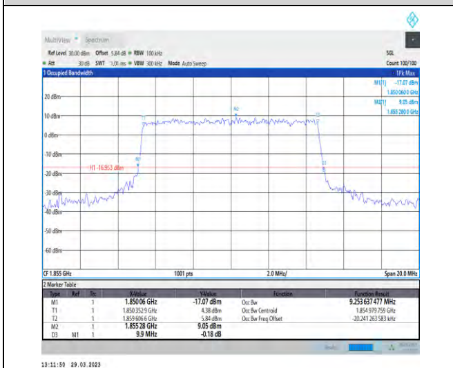
1-N25-15-10-L-8-CP-64QAM-Outer_Full-52@0-Ant1 -9.254-9.900≤10-PASS
