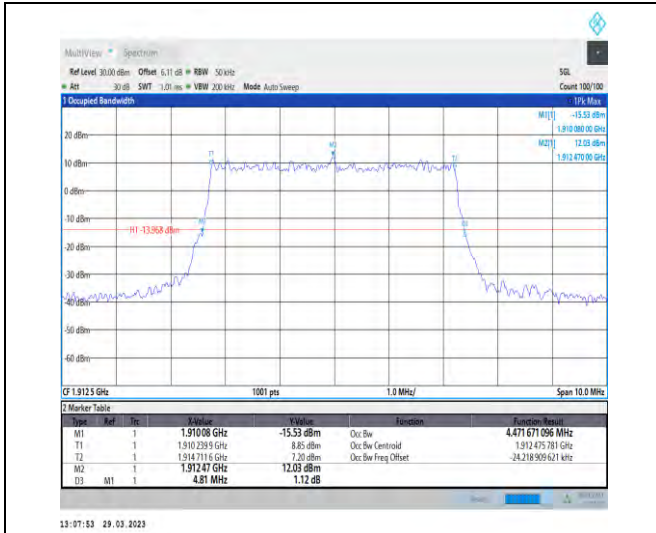
1-N25-15-5-H-3-DFT-16QAM-Outer_Full-25@0-Ant1 -4.472-4.810-≤5-PASS
