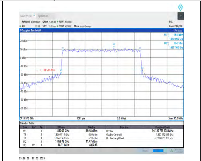
1-N25-15-15-L-8-CP-64QAM-Outer_Full-79@0-Ant1 -14.123-14.910-≤15-PASS
