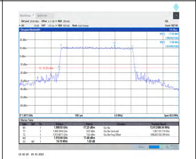
1-N25-15-15-H-4-DFT-64QAM-Outer_Full-75@0-Ant1 1-13.413-14.190-≤15-PASS
