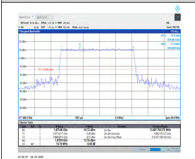
1-N25-15-15-M-4-DFT-64QAM-Outer_Full-75@0-Ant 1-13.408-14.190-≤15-PASS
