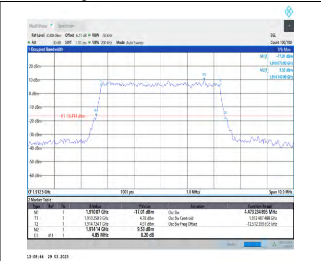
1-N25-15-5-H-8-CP-64QAM-Outer_Full-25@0-Ant1-4.473-4.850-≤5-PASS
