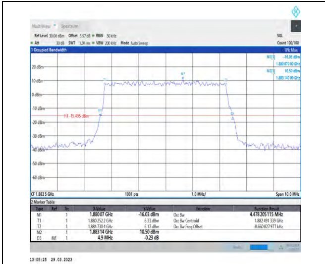
1-N25-15-5-M-4-DFT-64QAM-Outer_Full-25@0-Ant1 -4.478-4.900-≤5-PASS
