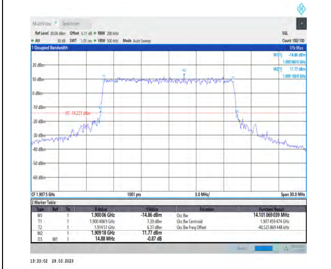
1-N25-15-15-H-7-CP-16QAM-Outer_Full-79@0-Ant1-14.101-14.880-≤15-PASS
