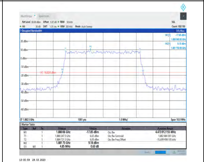
1-N25-15-5-M-7-CP-16QAM-Outer_Full-25@0-Ant1- 4.474-4.850-≤5-PASS
