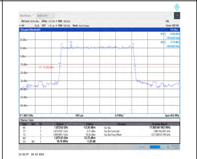
1-N25-15-20-M-2-DFT-PI2BPSK-Outer_Full-100@0-Ant 1-17.866-18.760-≤20-PASS
