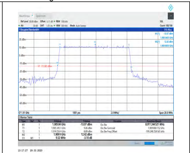
1-N25-15-10-H-1-DFT-QPSK-Outer_Full-50@0-Ant1 -8.911-9.520-≤10-PASS
