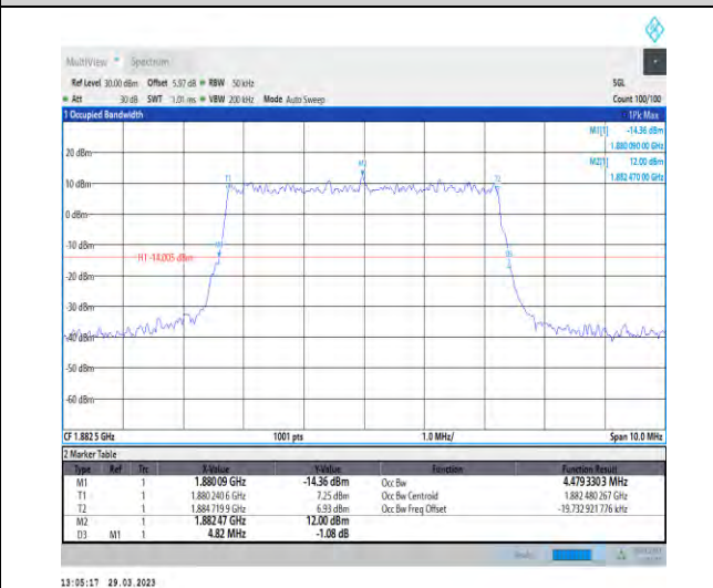
1-N25-15-5-M-3-DFT-16QAM-Outer_Full-25@0-Ant1 -4.479-4.820-≤5-PASS
