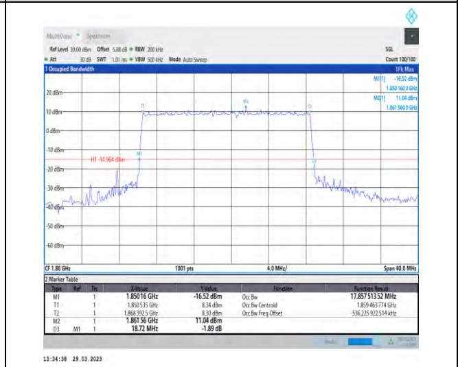
1-N25-15-20-L-3-DFT-16QAM-Outer_Full-100@0-Ant t1-17.858-18.720-≤20-PASS
