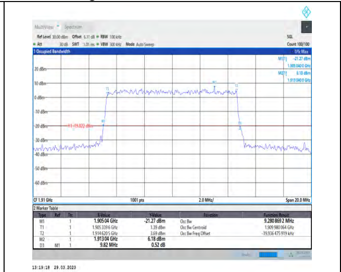
1-N25-15-10-H-9-CP-256QAM-Outer_Full-52@0-Ant 1-9.281-9.820-≤10-PASS
