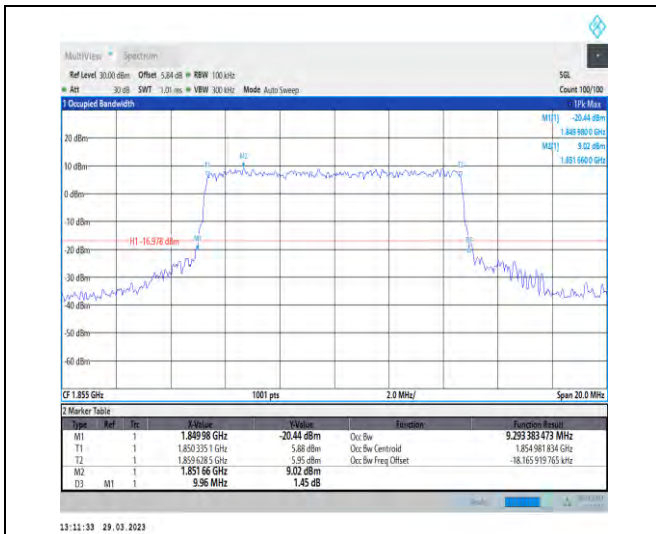
1-N25-15-10-L-6-CP-QPSK-Outer_Full-52@0-Ant1-9 -2.93-9.960≤10-PASS
