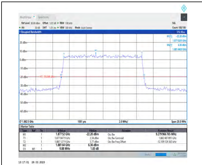
1-N25-15-10-M-9-CP-256QAM-Outer_Full-52@0-Ant 1-9.28-9.880-≤10-PASS
