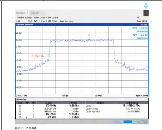
1-N25-15-15-M-7-CP-16QAM-Outer_Full-79@0-Ant1-14.138-14.910-≤15-PASS
