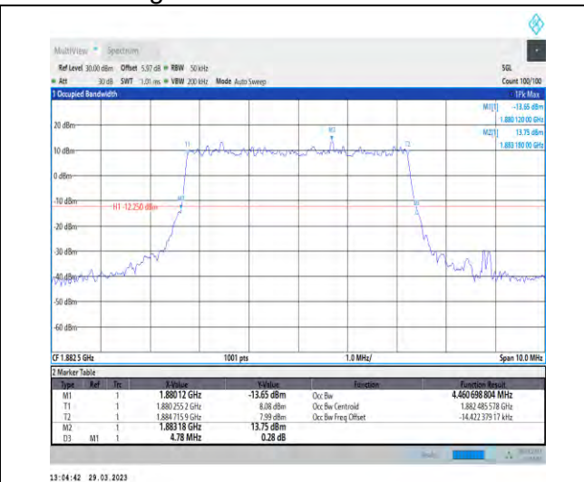
1-N25-15-5-M-1-DFT-QPSK-Outer_Full-25@0-Ant1- 4.461-4.780-≤5-PASS
