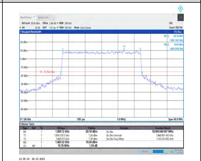
1-N25-15-20-L-7-CP-16QAM-Outer_Full-106@0-Ant 1-18.944-19.760-≤20-PASS
