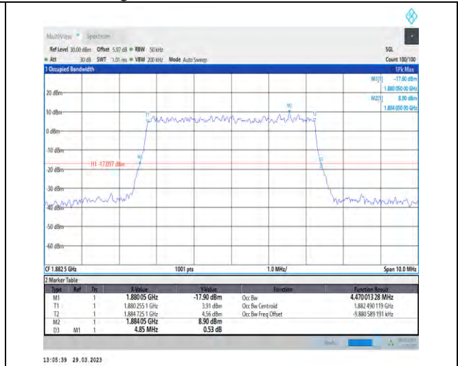
1-N25-15-5-M-5-DFT-256QAM-Outer_Full-25@0-Ant 1-4.47-4.850-≤5-PASS
