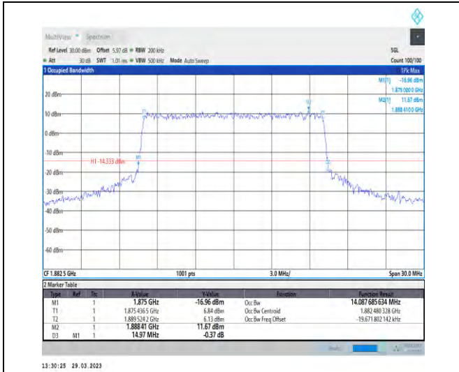
1-N25-15-15-M-6-CP-QPSK-Outer_Full-79@0-Ant1-14.088-14.970-≤15-PASS
