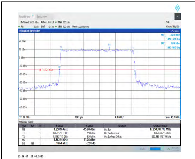
1-N25-15-20-L-4-DFT-64QAM-Outer_Full-100@0-Ant t1-17.85-18.640-≤20-PASS
