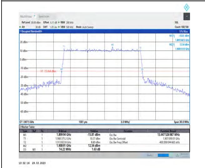
1-N25-15-15-H-3-DFT-16QAM-Outer_Full-75@0-Ant1 1-13.448-14.220-≤15-PASS
