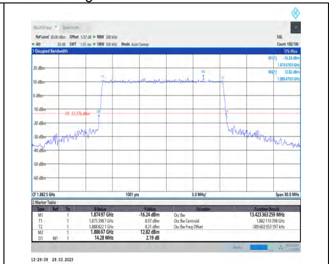
1-N25-15-15-M-3-DFT-16QAM-Outer_Full-75@0-Ant 1-13.423-14.280-≤15-PASS
