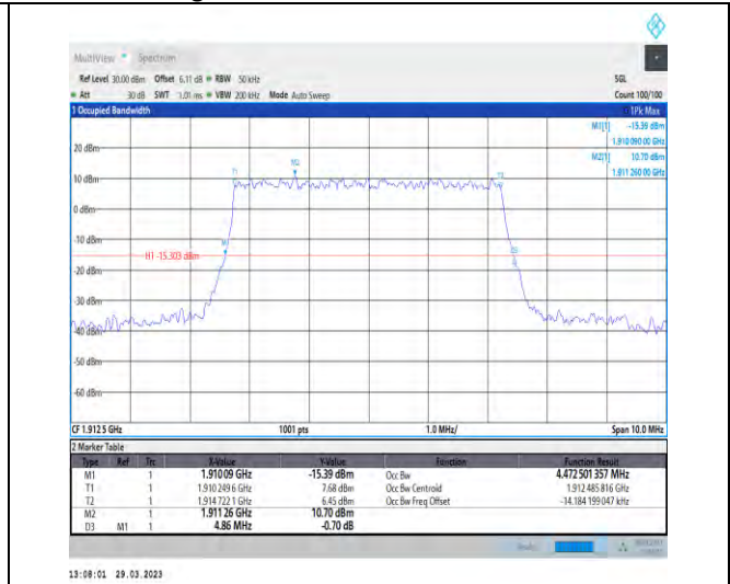
1-N25-15-5-H-4-DFT-64QAM-Outer_Full-25@0-Ant1 -4.473-4.860-≤5-PASS
