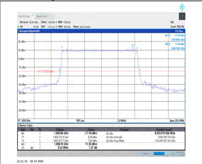
1-N25-15-10-L-3-DFT-16QAM-Outer_Full-50@0-Ant 1-8.936-9.520-≤10-PASS
