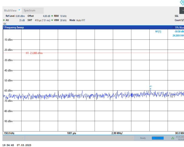
Band17-10MHz-QPSK-23780-1RB#0-Range2:0.15~30MHz
