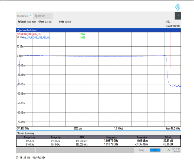
1-DC_5A_n2A-15-15-H-6-CP-QPSK-Outer_Full-79@0-Ant1-1-seegraph-PASS-see graph
