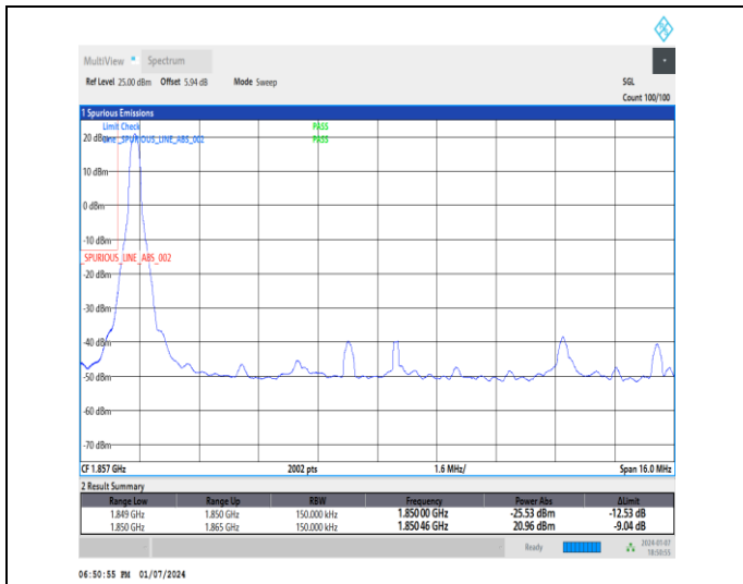
1-DC_5A_n2A-15-15-L-1-DFT-PI2BPSK-Edge_1RB_L eft-1@0-Ant1-1-seegraph-PASS-see graph
