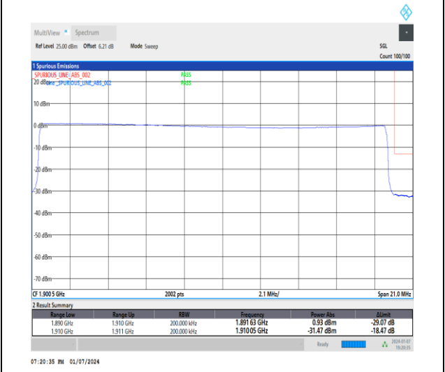
1-DC_5A_n2A-15-20-H-6-CP-QPSK-Outer_Full-106@0-Ant1-1-seegraph-PASS-see graph
