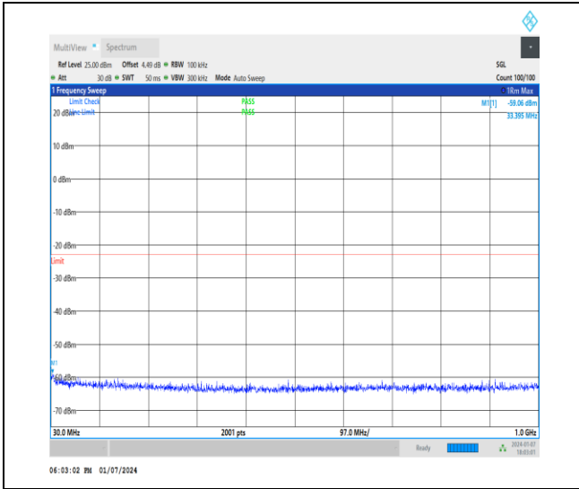
1-DC_5A_n2A-15-20-M-1-DFT-PI2BPSK-Inner_1RB _Left-1@1-30-1000-Ant1-33.40--59.06--23-PASS
