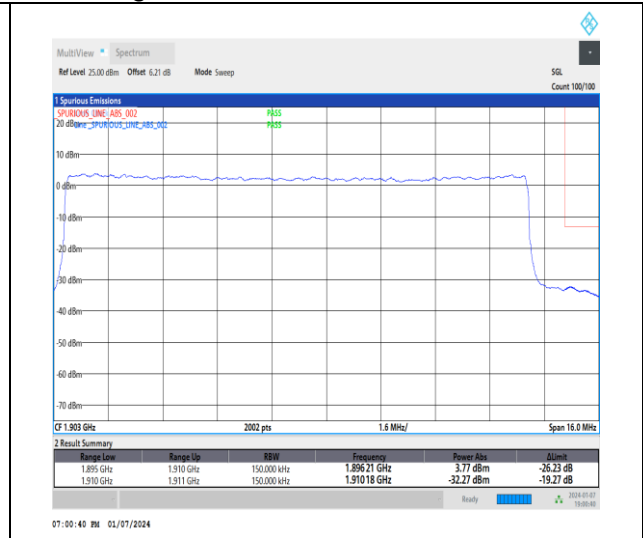
1-DC_5A_n2A-15-15-H-3-DFT-PI2BPSK-Outer_Fu ll-75@0-Ant1-1-seegraph-PASS-see graph
