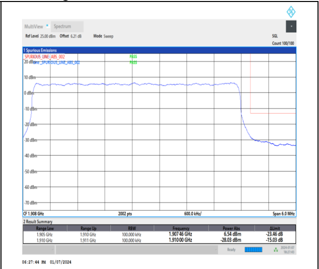
1-DC_5A_n2A-15-5-H-3-DFT-PI2BPSK-Outer_Full-25@0-Ant1-1-seegraph-PASS-see graph
