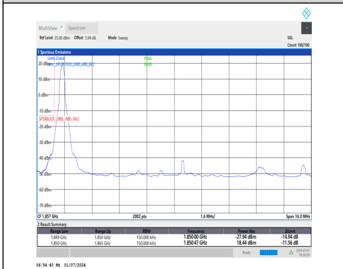
1-DC_5A_n2A-15-15-L-4-CP-QPSK-Edge_1RB_Left-1 @0-Ant1-1-seegraph-PASS-see graph
