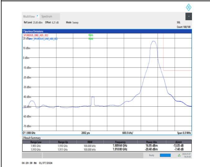
1-DC_5A_n2A-15-5-H-5-CP-QPSK-Edge_1RB_Right-1@24-Ant1-1-seegraph-PASS-see graph
