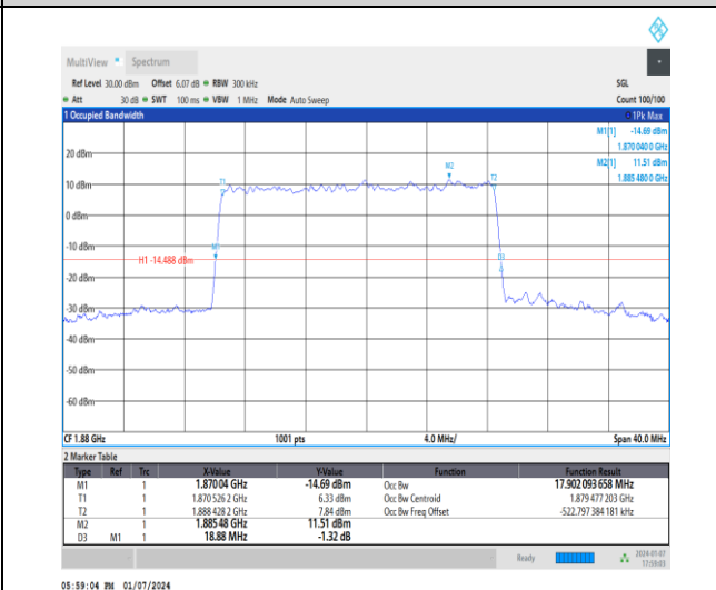
1-DC_5A_n2A-15-20-M-5-DFT-256QAM-Outer_Full-100@0-Ant1-17.902-18.880-≤20-PASS
