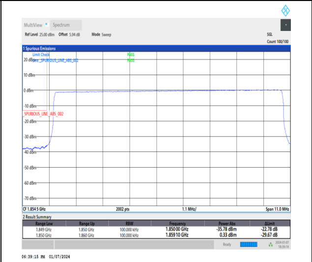
1-DC_5A_n2A-15-10-L-6-CP-QPSK-Outer_Full-52 @0-Ant1-1-seegraph-PASS-see graph
