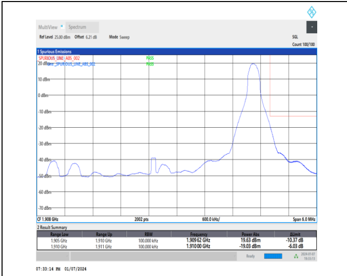
1-DC_5A_n2A-15-5-H-2-DFT-PI2BPSK-Edge_1RB_Right-1@24-Ant1-1-seegraph-PASS-see graph
