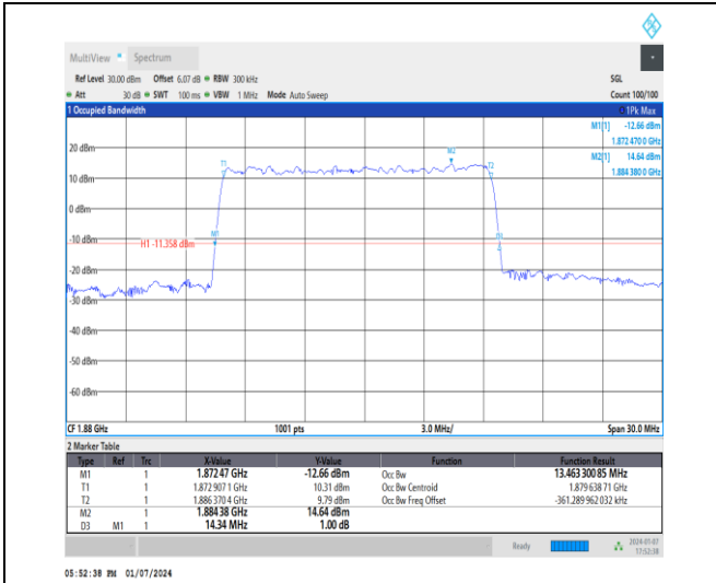
1-DC_5A_n2A-15-15-M-3-DFT-16QAM-Outer_Full-7 5@0-Ant1-13.463-14.340-≤15-PASS
