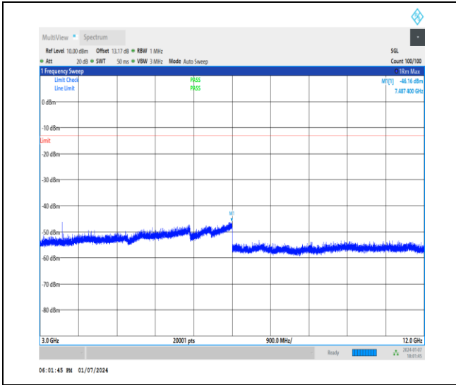
1-DC_5A_n2A-15-20-L-1-DFT-PI2BPSK-Inner_1RB _Left-1@1-3000-12000-Ant1-7487.40--46.16--13-PA SS
