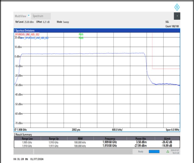
1-DC_5A_n2A-15-5-H-6-CP-QPSK-Outer_Full-25@0-Ant1-1-seegraph-PASS-see graph
