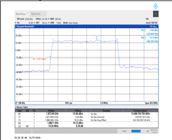
1-DC_5A_n2A-15-15-M-4-DFT-64QAM-Outer_Full-7 5@0-Ant1-13.497-14.340-≤15-PASS
