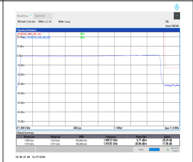
1-DC_5A_n2A-15-10-H-6-CP-QPSK-Outer_Full-52@0-Ant1-1-seegraph-PASS-see graph
