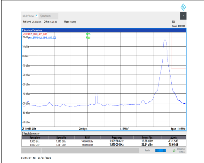
1-DC_5A_n2A-15-10-H-5-CP-QPSK-Edge_1RB_Right-1@51-Ant1-1-seegraph-PASS-see graph
