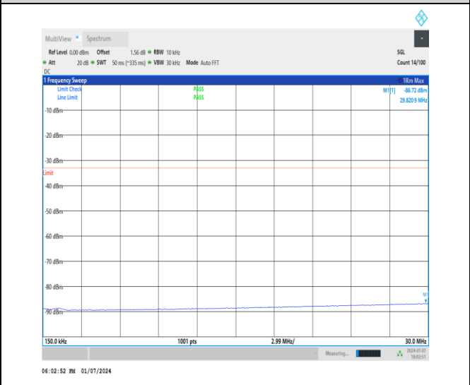
1-DC_5A_n2A-15-20-M-1-DFT-PI2BPSK-Inner_1RB_ Left-1@1-0.15-30-Ant1-29.82--86.72--33-PASS
