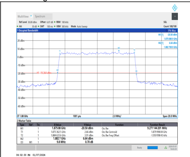
1-DC_5A_n2A-15-10-M-9-CP-256QAM-Outer_Full-5 2@0-Ant1-9.271-9.800-≤10-PASS
