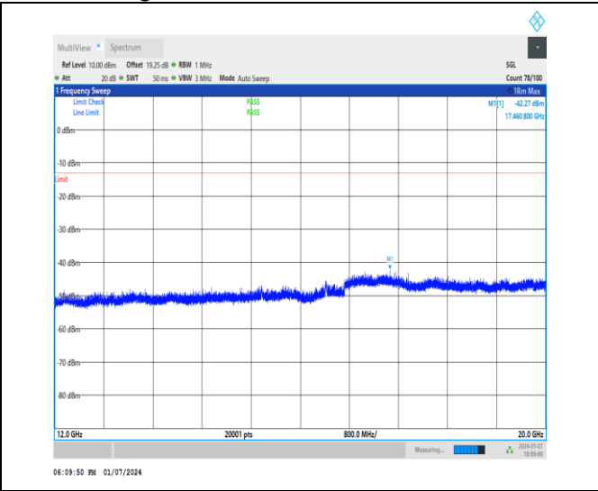
1-DC_5A_n2A-15-20-H-1-DFT-PI2BPSK-Inner_1RB_ Left-1@1-12000-20000-Ant1-17460.80--42.27--13-PA SS
