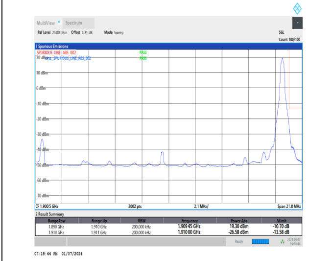
1-DC_5A_n2A-15-20-H-5-CP-QPSK-Edge_1RB_Right-1@105-Ant1-1-seegraph-PASS-see graph
