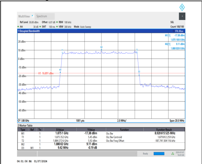
1-DC_5A_n2A-15-10-M-5-DFT-256QAM-Outer_Full-50@0-Ant1-8.921-9.420-≤10-PASS
