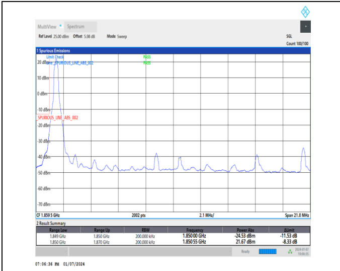
1-DC_5A_n2A-15-20-L-1-DFT-PI2BPSK-Edge_1RB_L eft-1@0-Ant1-1-seegraph-PASS-see graph
