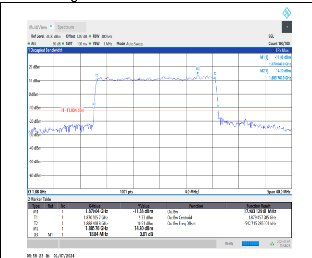
1-DC_5A_n2A-15-20-M-3-DFT-16QAM-Outer_Full-100@0-Ant1-17.903-18.840-≤20-PASS
