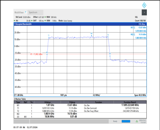
1-DC_5A_n2A-15-20-M-1-DFT-QPSK-Outer_Full-10 0@0-Ant1-17.895-18.960-≤20-PASS
