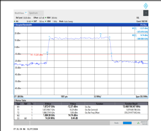
1-DC_5A_n2A-15-15-M-6-CP-QPSK-Outer_Full-79 @0-Ant1-13.468-14.34-≤15-PASS
