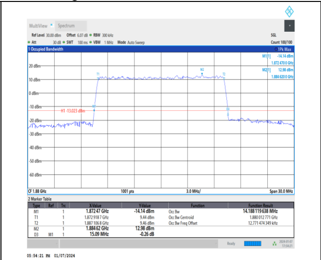
1-DC_5A_n2A-15-15-M-8-CP-64QAM-Outer_Full-79 @0-Ant1-14.188-15.090-≤15-PASS
