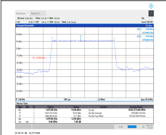
1-DC_5A_n2A-15-10-M-2-DFT-PI2BPSK-Outer_Full-50 @0-Ant1-8.952-9.460-≤10-PASS
