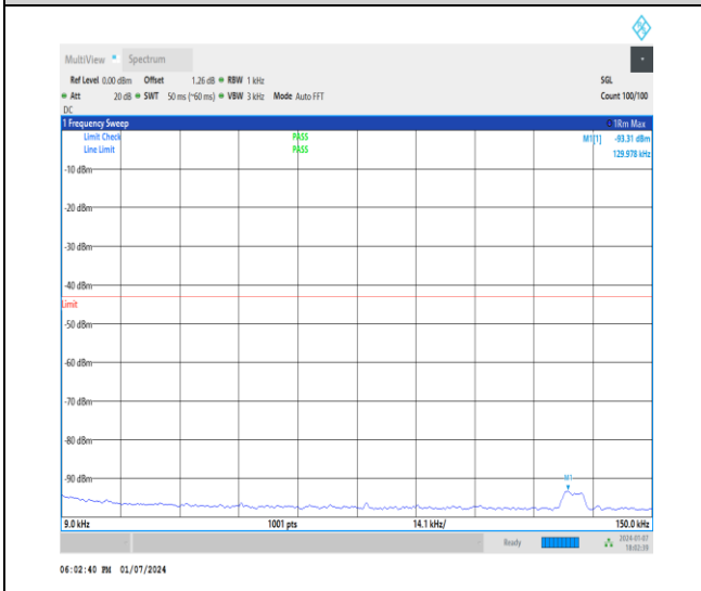
1-DC_5A_n2A-15-20-M-1-DFT-PI2BPSK-Inner_1RB _Left-1@1-0.009-0.15-Ant1-0.13--93.31--43-PASS
