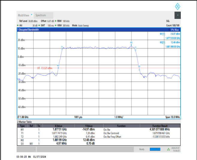
1-DC_5A_n2A-15-5-M-8-CP-64QAM-Outer_Full-25@0-Ant1-4.501-4.970-≤5-PASS
