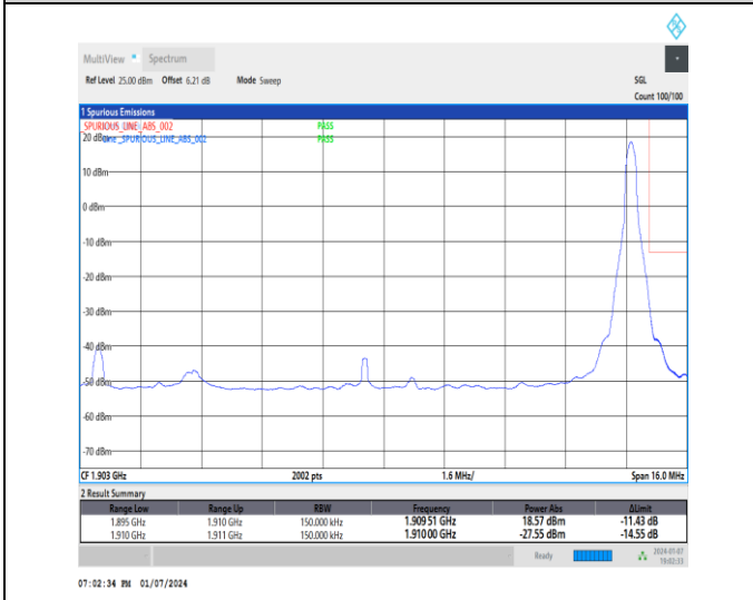
1-DC_5A_n2A-15-15-H-5-CP-QPSK-Edge_1RB_Right-1@78-Ant1-1-seegraph-PASS-see graph
