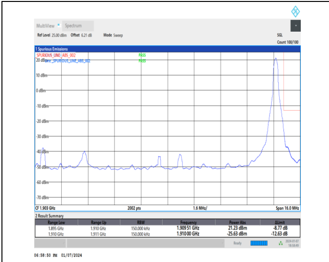
1-DC_5A_n2A-15-15-H-2-DFT-PI2BPSK-Edge_1RB_Right-1@78-Ant1-1-seegraph-PASS-see graph
