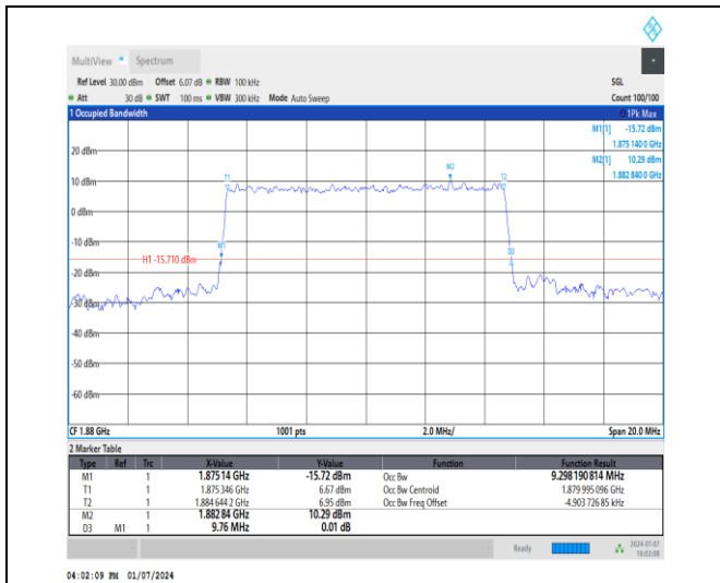
1-DC_5A_n2A-15-10-M-8-CP-64QAM-Outer_Full-52 @0-Ant1-9.298-9.760-≤10-PASS
