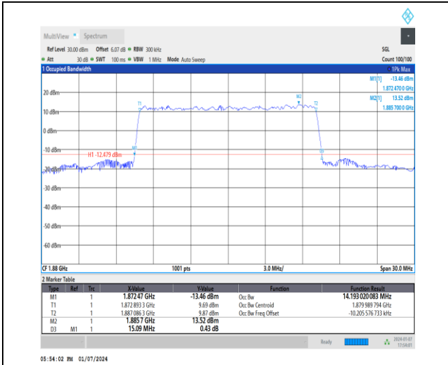
1-DC_5A_n2A-15-15-M-7-CP-16QAM-Outer_Full-79 @0-Ant1-14.193-15.090-≤15-PASS
