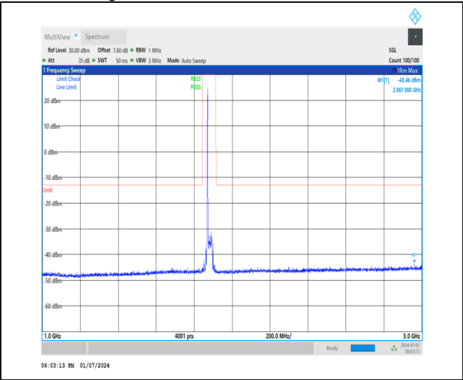
1-DC_5A_n2A-15-20-M-1-DFT-PI2BPSK-Inner_1RB Left-1@1-1000-3000-Ant1-2961.00--43.46--13-PASS
