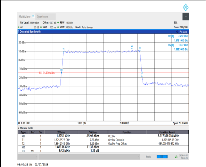
1-DC_5A_n2A-15-10-M-3-DFT-16QAM-Outer_Full-5 @0-Ant1-8.917-9.420-≤10-PASS
