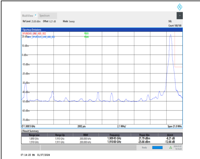
1-DC_5A_n2A-15-20-H-2-DFT-PI2BPSK-Edge_1RB_Right-1@105-Ant1-1-seegraph-PASS-see graph
