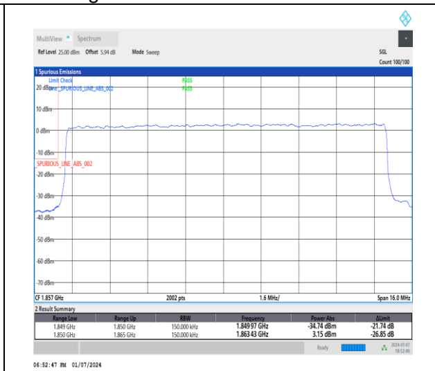
1-DC_5A_n2A-15-15-L-3-DFT-PI2BPSK-Outer_Ful I-75@0-Ant1-1-seegraph-PASS-see graph
