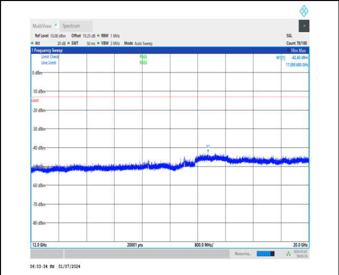
1-DC_5A_n2A-15-20-M-1-DFT-PI2BPSK-Inner_1RB Left-1@1-12000-20000-Ant1-17093.60--42.60--13-PA SS
