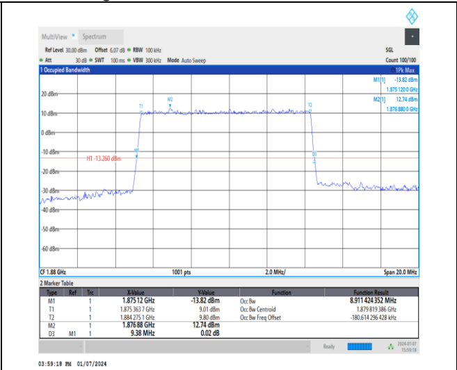
1-DC_5A_n2A-15-10-M-1-DFT-QPSK-Outer_Full-50 @0-Ant1-8.911-9.380-≤10-PASS
