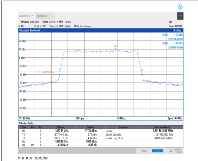
1-DC_5A_n2A-15-5-M-9-CP-256QAM-Outer_Full-25 @0-Ant1-4.492-4.980-≤5-PASS
