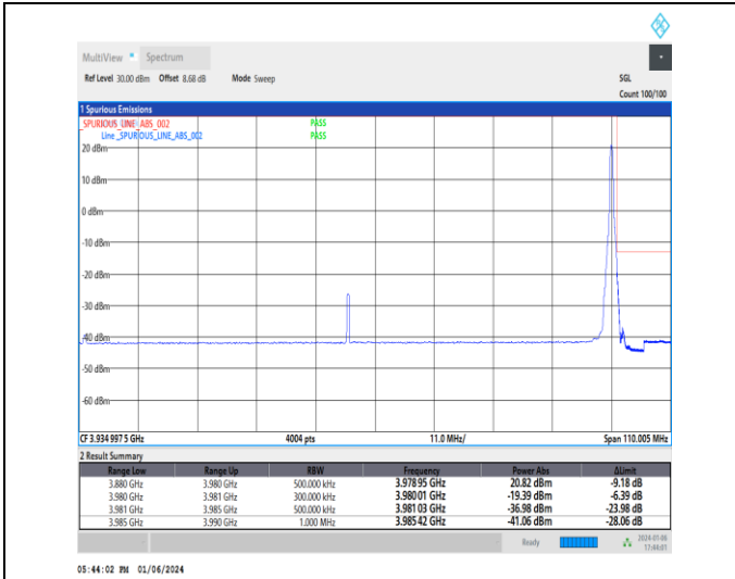
1-N77-3700-3980-30-100-H-2-DFT-PI2BPSK-Edge_1R_B_Right-1@272-Ant2-1--PASS-see graph
