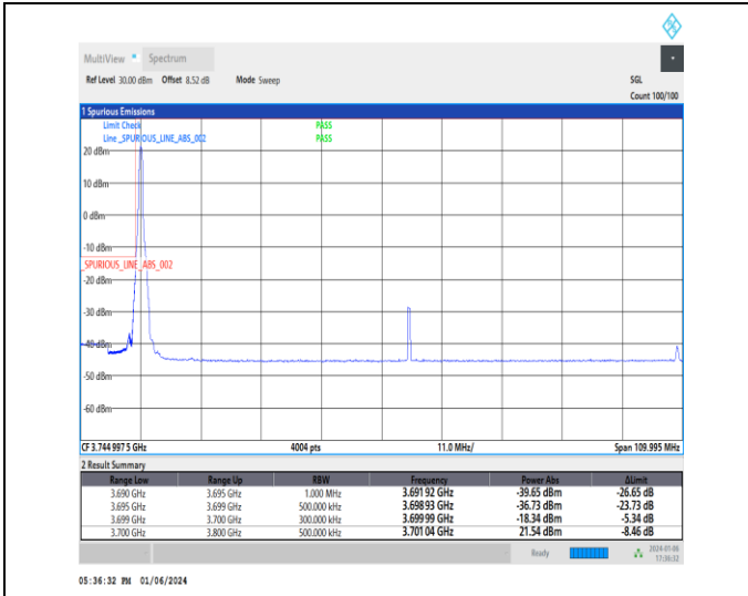
1-N77-3700-3980-30-100-L-1-DFT-PI2BPSK-Edge_1R_B_Left-1@0-Ant2-1--PASS-see graph
