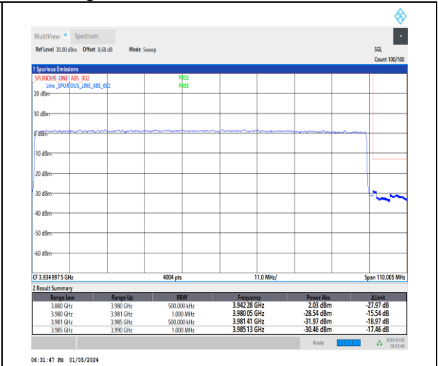
1-N77-3700-3980-30-100-H-3-DFT-PI2BPSK-Outer_Full-270@0-Ant2-1--PASS-see graph
