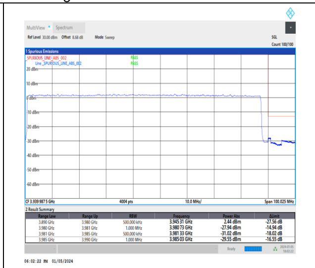
1-N77-3700-3980-30-90-H-3-DFT-PI2BPSK-Outer_Full-240@0-Ant2-1--PASS-see graph
