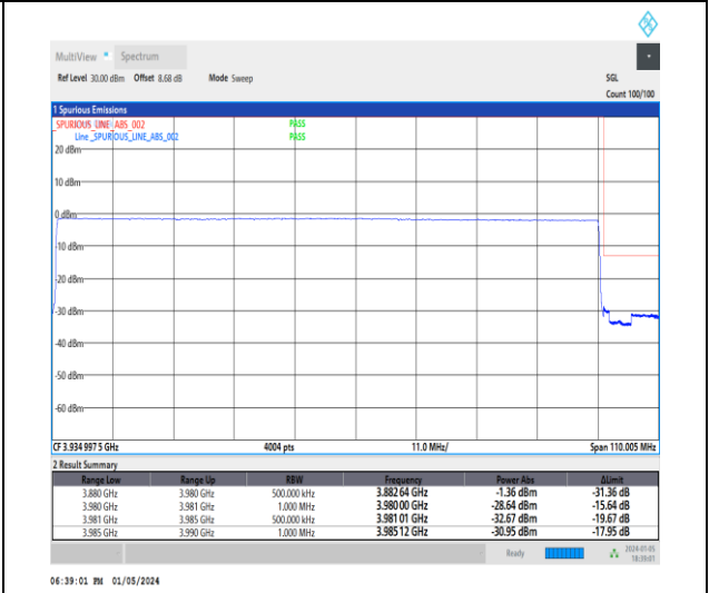
1-N77-3700-3980-30-100-H-6-CP-QPSK-Outer_Full-273@0-Ant2-1--PASS-see graph
