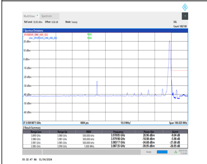
1-N77-3700-3980-30-90-H-5-CP-QPSK-Edge_1RB_Right-1@244-Ant2-1--PASS-see graph
