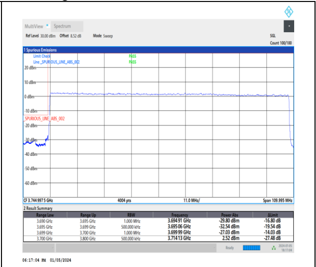
1-N77-3700-3980-30-100-L-3-DFT-PI2BPSK-Outer_Full-270@0-Ant2-1--PASS-see graph
