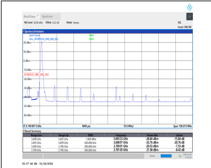
1-N77-3700-3980-30-90-L-1-DFT-PI2BPSK-Edge_1RB _Left-1@0-Ant2-1--PASS-see graph
