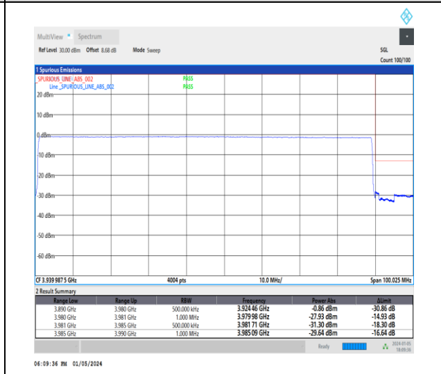
1-N77-3700-3980-30-90-H-6-CP-QPSK-Outer_Full-245@0-Ant2-1--PASS-see graph
