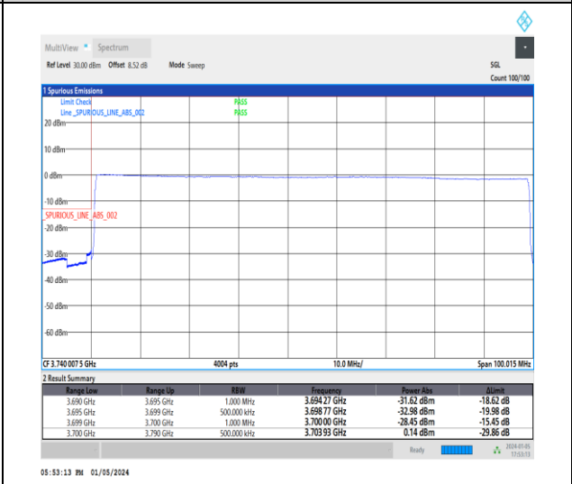
1-N77-3700-3980-30-90-L-6-CP-QPSK-Outer_Full -245@0-Ant2-1--PASS-see graph
