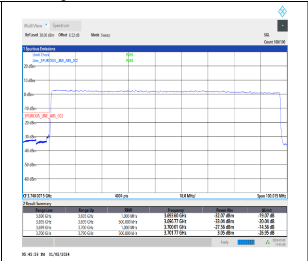
1-N77-3700-3980-30-90-L-3-DFT-PI2BPSK-Outer _Full-240@0-Ant2-1--PASS-see graph
