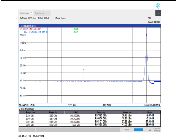
1-N77-3700-3980-30-100-H-5-CP-QPSK-Edge_1RB_Right-1@272-Ant2-1--PASS-see graph
