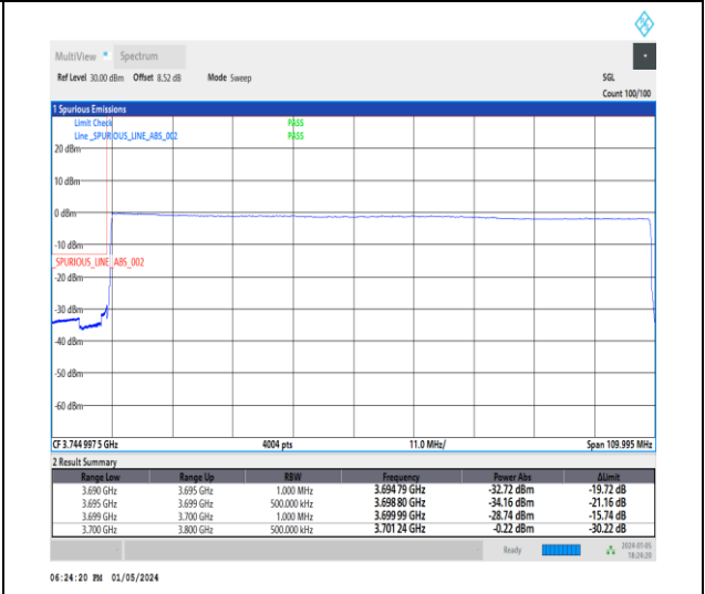
1-N77-3700-3980-30-100-L-6-CP-QPSK-Outer_Full-273@0-Ant2-1--PASS-see graph
