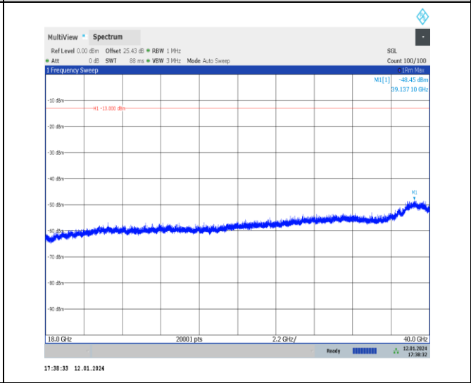
1-N77-3700-3980-30-100-M-1-DFT-PI2BPSK-Inner_1RB_Left-1@1-18000-40000-Ant2-18000.00--48.45--1 3-PASS
