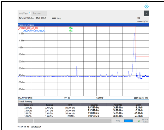
1-N77-3700-3980-30-90-H-2-DFT-PI2BPSK-Edge_1R_B_Right-1@244-Ant2-1--PASS-see graph
