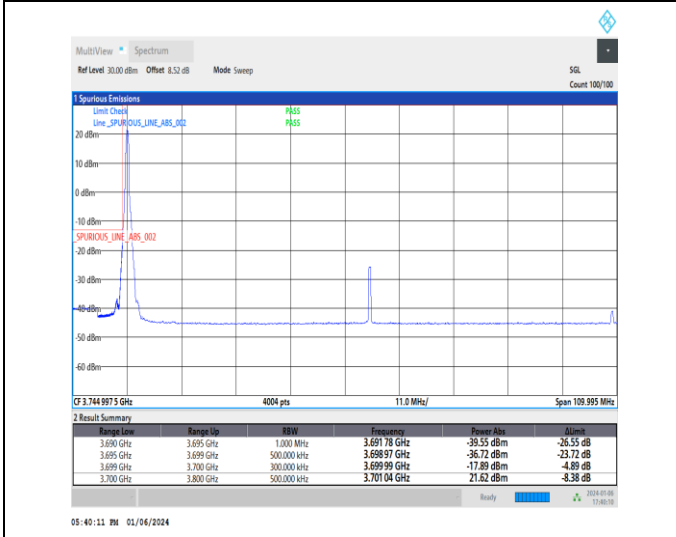
1-N77-3700-3980-30-100-L-4-CP-QPSK-Edge_1RB_Left-1@0-Ant2-1--PASS-see graph
