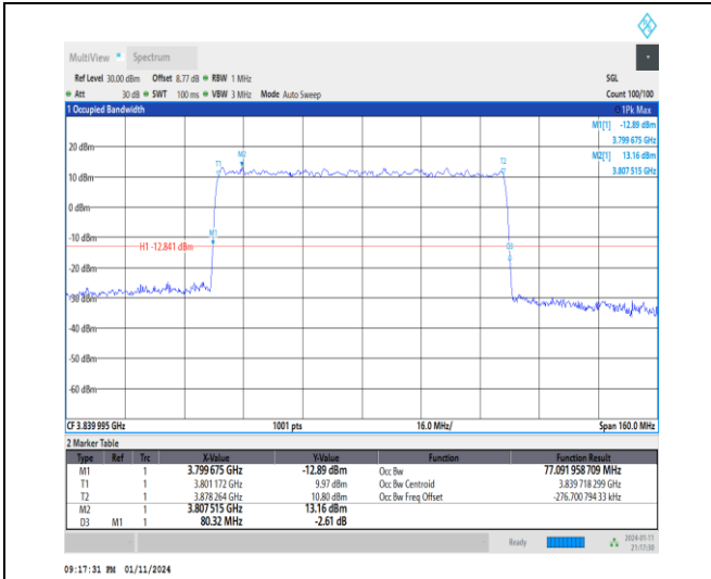
1-N77-3700-3980-30-80-M-4-DFT-64QAM-Outer_Full I-216@0-Ant2-77.092-80.320-≤80-PASS
