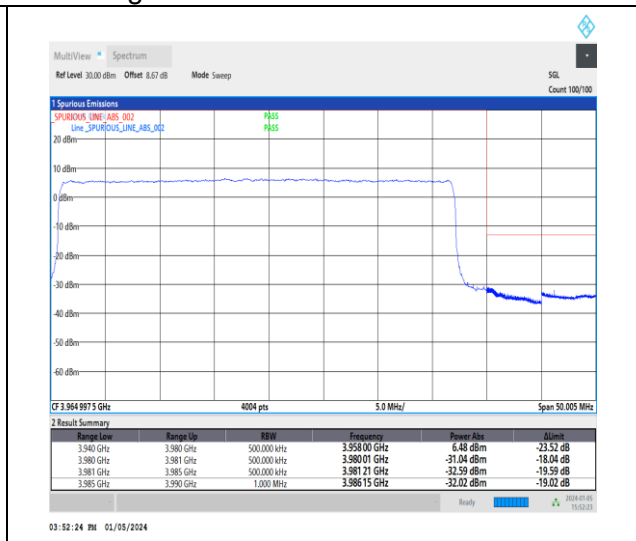
1-N77-3700-3980-30-40-H-3-DFT-PI2BPSK-Outer_Full-100@0-Ant2-1--PASS-see graph
