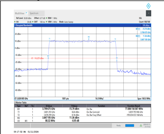
1-N77-3700-3980-30-80-M-5-DFT-256QAM-Outer_Full ull-216@0-Ant2-77.006-80.320-≤80-PASS
