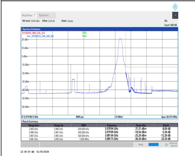
1-N77-3700-3980-30-20-H-5-CP-QPSK-Edge_1RB_Right-1@50-Ant2-1--PASS-see graph
