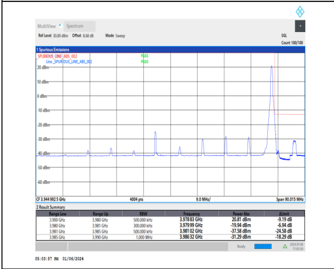
1-N77-3700-3980-30-80-H-5-CP-QPSK-Edge_1RB_Right-1@216-Ant2-1--PASS-see graph
