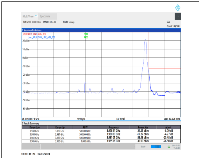
1-N77-3700-3980-30-40-H-2-DFT-PI2BPSK-Edge_1R_B_Right-1@105-Ant2-1--PASS-see graph
