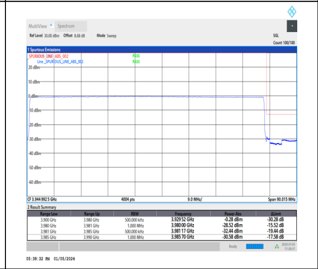
1-N77-3700-3980-30-80-H-6-CP-QPSK-Outer_Full-217@0-Ant2-1--PASS-see graph
