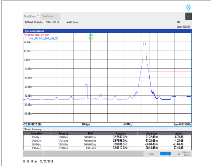
1-N77-3700-3980-30-30-H-5-CP-QPSK-Edge_1RB_Right-1@77-Ant2-1--PASS-see graph
