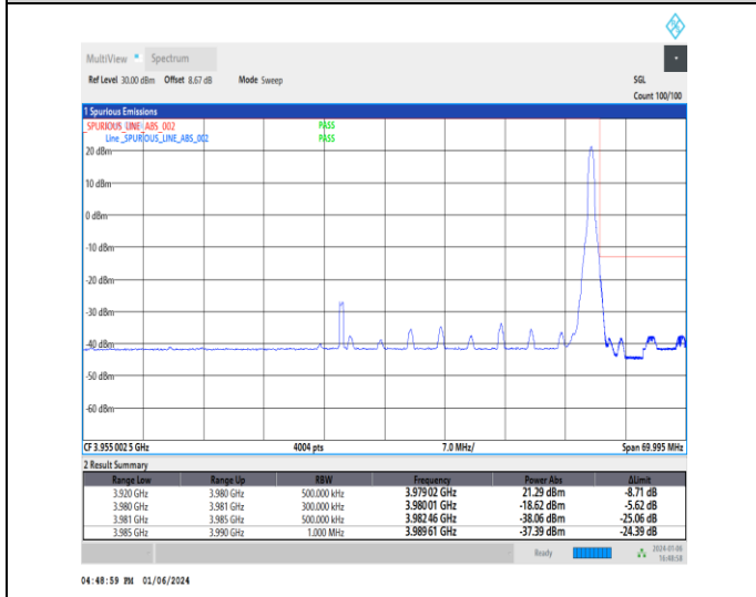
1-N77-3700-3980-30-60-H-5-CP-QPSK-Edge_1RB_Right-1@161-Ant2-1--PASS-see graph
