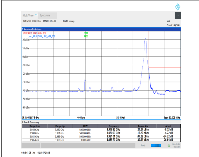
1-N77-3700-3980-30-40-H-5-CP-QPSK-Edge_1RB_Right-1@105-Ant2-1--PASS-see graph
