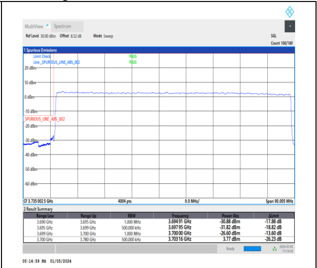
1-N77-3700-3980-30-80-L-3-DFT-PI2BPSK-Outer_Full-216@0-Ant2-1--PASS-see graph
