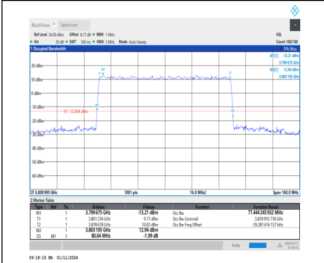
1-N77-3700-3980-30-80-M-6-CP-QPSK-Outer_Full-2 17@0-Ant2-77.444-80.640-≤80-PASS
