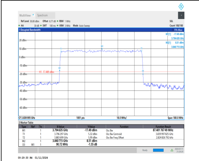
1-N77-3700-3980-30-90-M-9-CP-256QAM-Outer_Ful-1-245@0-Ant2-87.402-90.720-≤90-PASS
