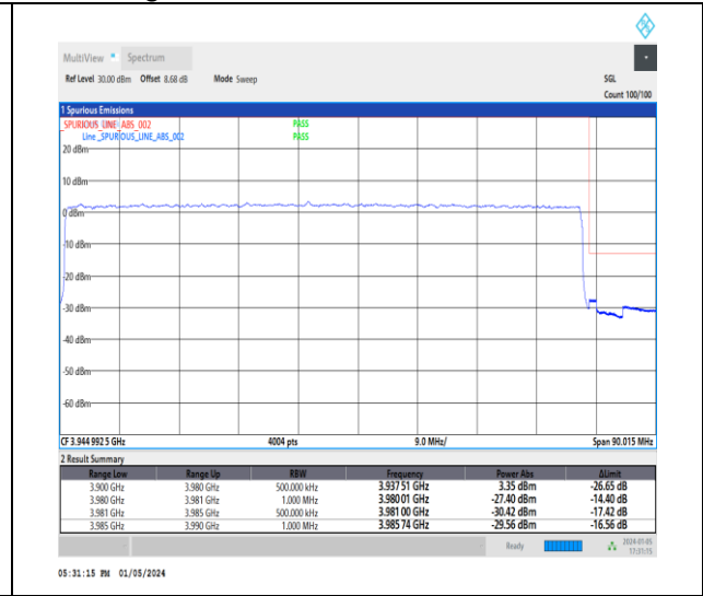
1-N77-3700-3980-30-80-H-3-DFT-PI2BPSK-Outer_Full-216@0-Ant2-1--PASS-see graph
