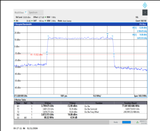
1-N77-3700-3980-30-80-M-3-DFT-16QAM-Outer_Full-216@0-Ant2-77.042-80.320-≤80-PASS
