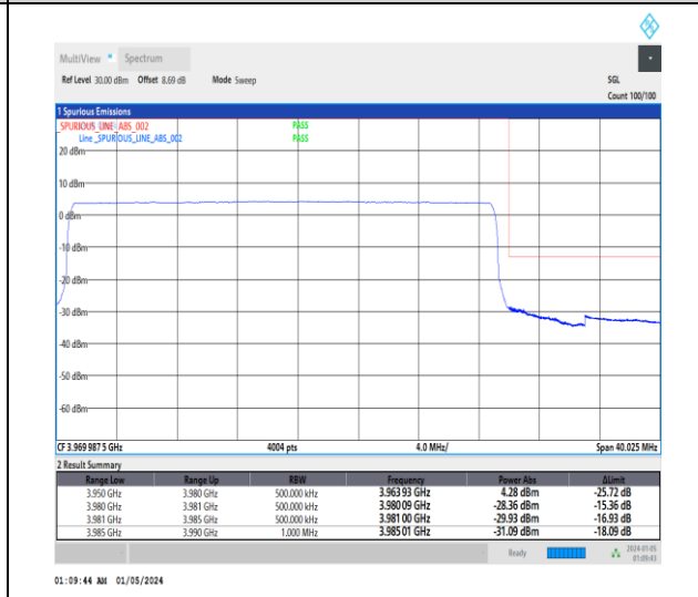
1-N77-3700-3980-30-30-H-6-CP-QPSK-Outer_Full-78@0-Ant2-1--PASS-see graph
