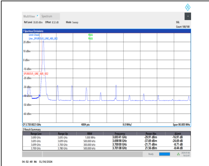
1-N77-3700-3980-30-80-L-1-DFT-PI2BPSK-Edge_1RB_Left-1@0-Ant2-1--PASS-see graph
