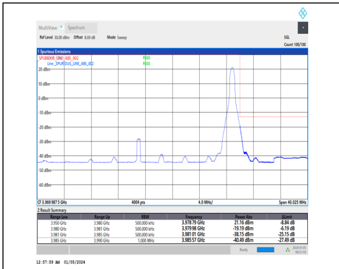
1-N77-3700-3980-30-30-H-2-DFT-PI2BPSK-Edge_1R_B_Right-1@77-Ant2-1--PASS-see graph
