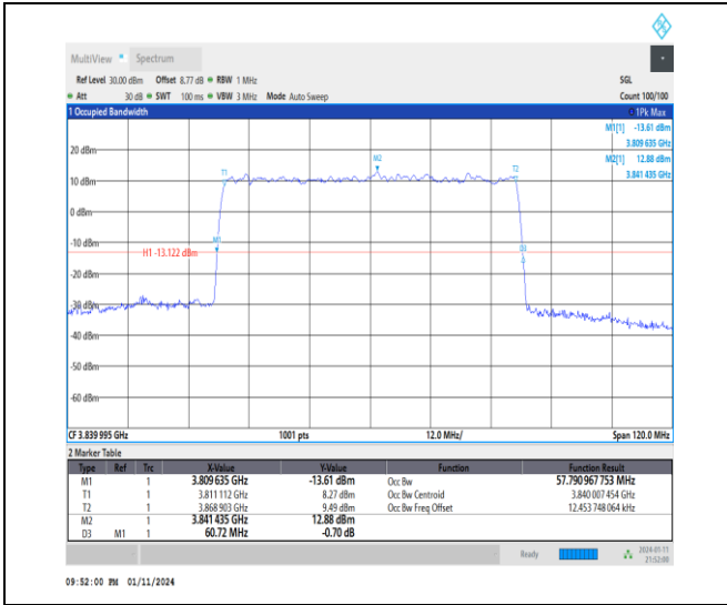
1-N77-3700-3980-30-60-M-5-DFT-256QAM-Outer_Full-162@0-Ant2-57.791-60.720-≤60-PASS
