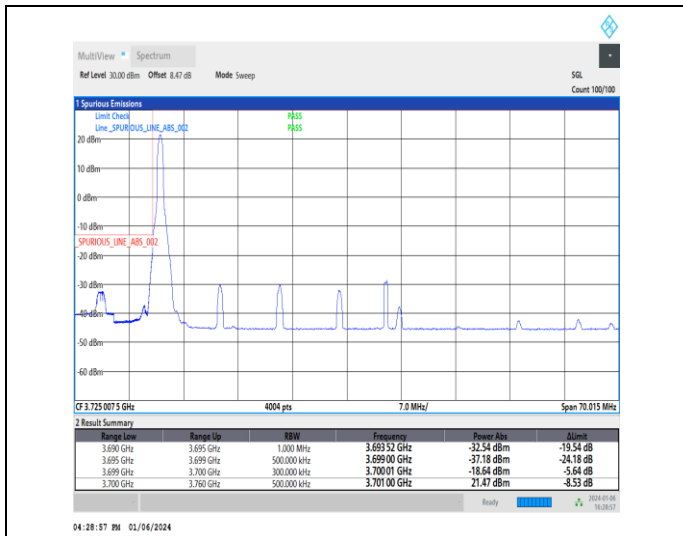
1-N77-3700-3980-30-60-L-1-DFT-PI2BPSK-Edge_1RB_Left-1@0-Ant2-1--PASS-see graph
