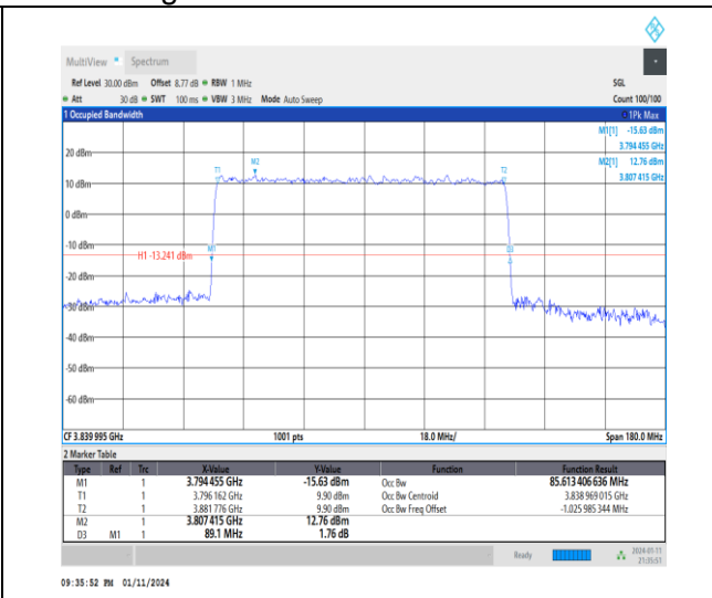
1-N77-3700-3980-30-90-M-4-DFT-64QAM-Outer_Fu II-240@0-Ant2-85.613-89.100-≤90-PASS
