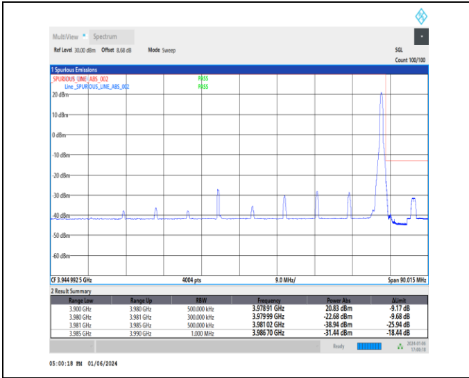
1-N77-3700-3980-30-80-H-2-DFT-PI2BPSK-Edge_1R_B_Right-1@216-Ant2-1--PASS-see graph
