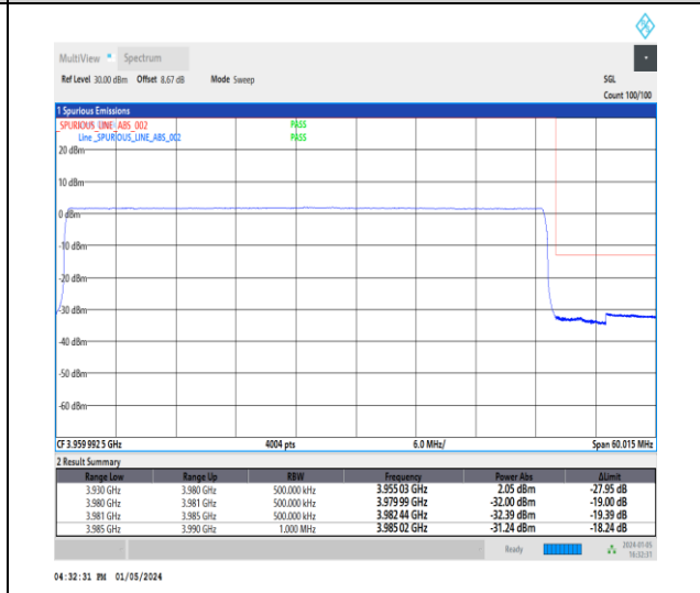
1-N77-3700-3980-30-50-H-6-CP-QPSK-Outer_Full-133@0-Ant2-1--PASS-see graph
