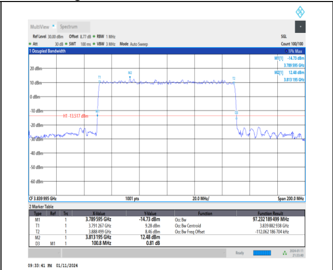
1-N77-3700-3980-30-100-M-7-CP-16QAM-Outer_FuII-273@0-Ant2-97.232-100.800-≤100-PASS
