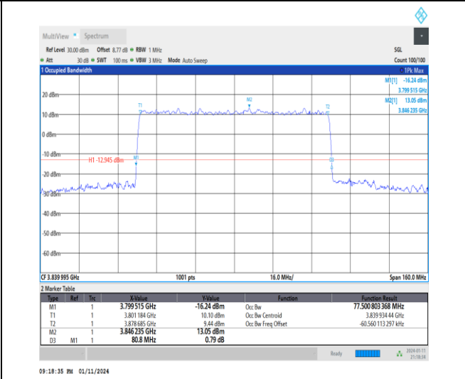
1-N77-3700-3980-30-80-M-7-CP-16QAM-Outer_Full -217@0-Ant2-77.501-80.800-≤80-PASS
