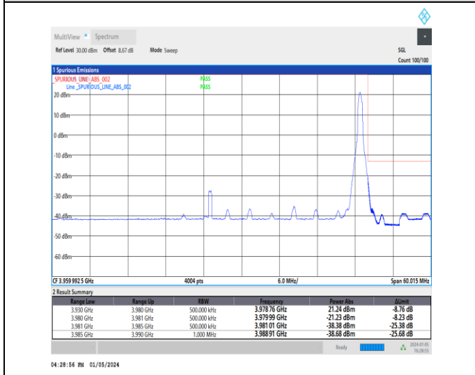
1-N77-3700-3980-30-50-H-5-CP-QPSK-Edge_1RB_Right-1@132-Ant2-1--PASS-see graph
