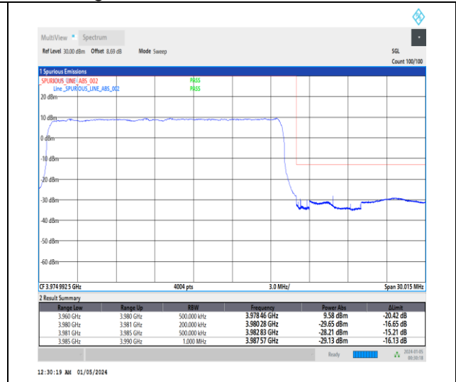
1-N77-3700-3980-30-20-H-3-DFT-PI2BPSK-Outer_Full-50@0-Ant2-1--PASS-see graph
