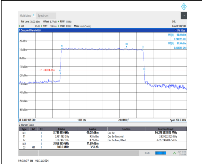
1-N77-3700-3980-30-100-M-4-DFT-64QAM-Outer_Full-270@0-Ant2-96.279-100.000-≤100-PASS
