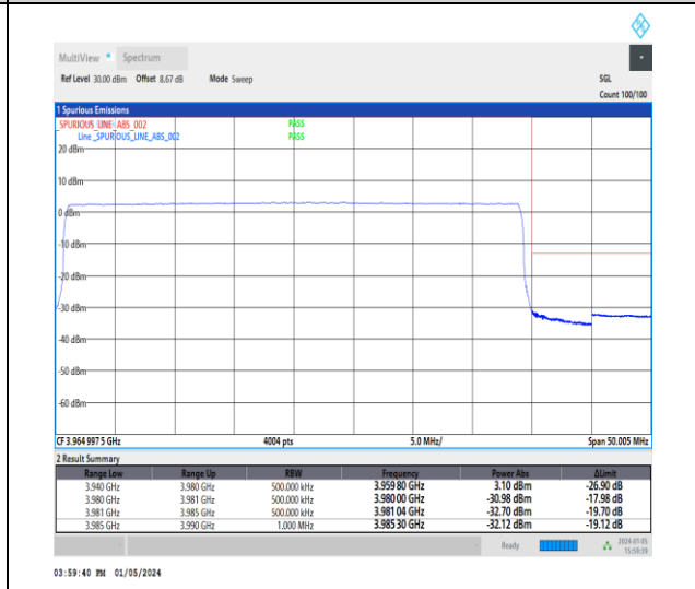
1-N77-3700-3980-30-40-H-6-CP-QPSK-Outer_Full-106@0-Ant2-1--PASS-see graph
