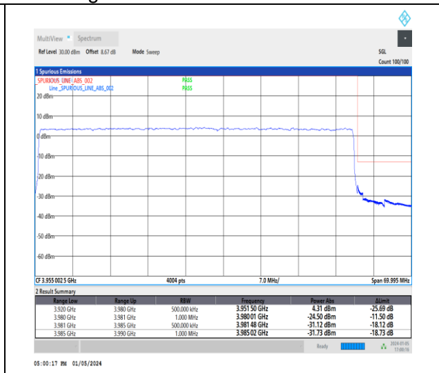
1-N77-3700-3980-30-60-H-3-DFT-PI2BPSK-Outer_Full-162@0-Ant2-1--PASS-see graph
