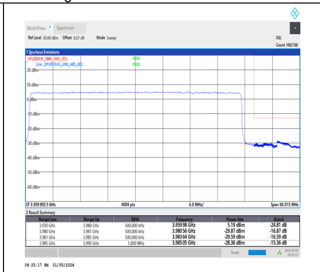
1-N77-3700-3980-30-50-H-3-DFT-PI2BPSK-Outer_Full-128@0-Ant2-1--PASS-see graph
