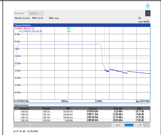
1-N77-3700-3980-30-20-H-6-CP-QPSK-Outer_Full-51@0-Ant2-1--PASS-see graph
