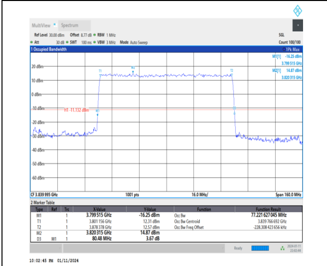
1-N77-3700-3980-30-80-M-2-DFT-PI2BPSK-Outer_Full-216@0-Ant2-77.222-80.480-≤80-PASS
