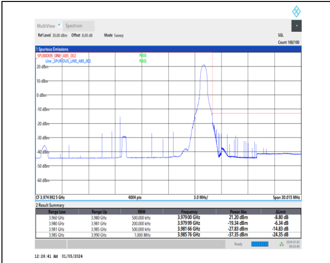
1-N77-3700-3980-30-20-H-2-DFT-PI2BPSK-Edge_1R_B_Right-1@50-Ant2-1--PASS-see graph
