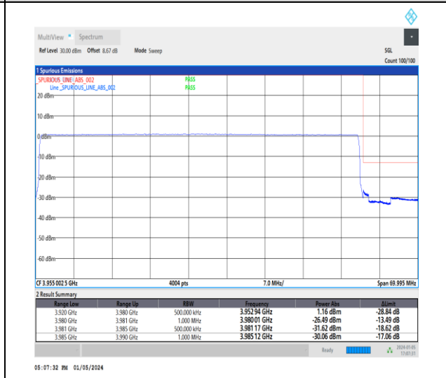
1-N77-3700-3980-30-60-H-6-CP-QPSK-Outer_Full-162@0-Ant2-1--PASS-see graph
