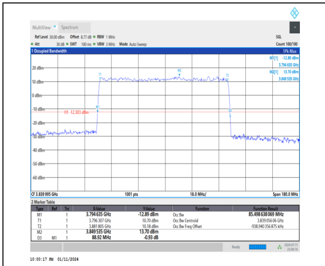
1-N77-3700-3980-30-90-M-3-DFT-16QAM-Outer_Ful I-240@0-Ant2-85.499-88.920-≤90-PASS
