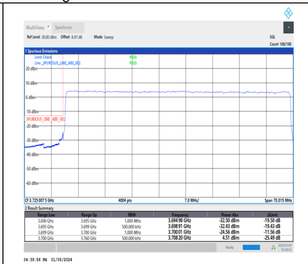
1-N77-3700-3980-30-60-L-3-DFT-PI2BPSK-Outer_Full-162@0-Ant2-1--PASS-see graph
