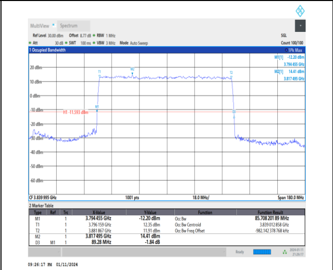
1-N77-3700-3980-30-90-M-2-DFT-PI2BPSK-Outer_Full-240@0-Ant2-85.708-89.280-<math>\leq 90</math>-PASS
