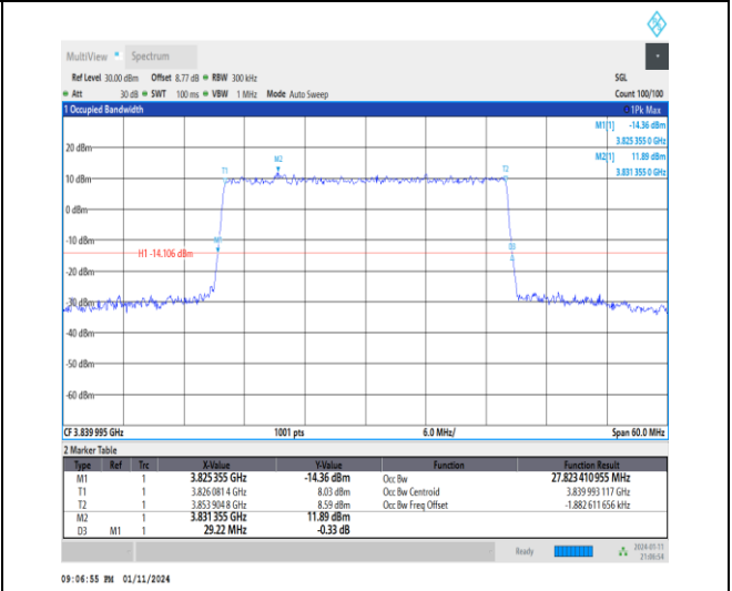
1-N77-3700-3980-30-30-M-7-CP-16QAM-Outer_Full -78@0-Ant2-27.823-29.220-≤30-PASS
