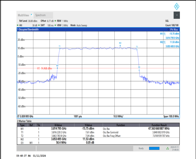
1-N77-3700-3980-30-50-M-9-CP-256QAM-Outer_Full-1 133@0-Ant2-47.564-50.400-≤50-PASS
