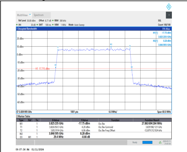
1-N77-3700-3980-30-30-M-9-CP-256QAM-Outer_Fu II-78@0-Ant2-27.864-29.400-≤30-PASS
