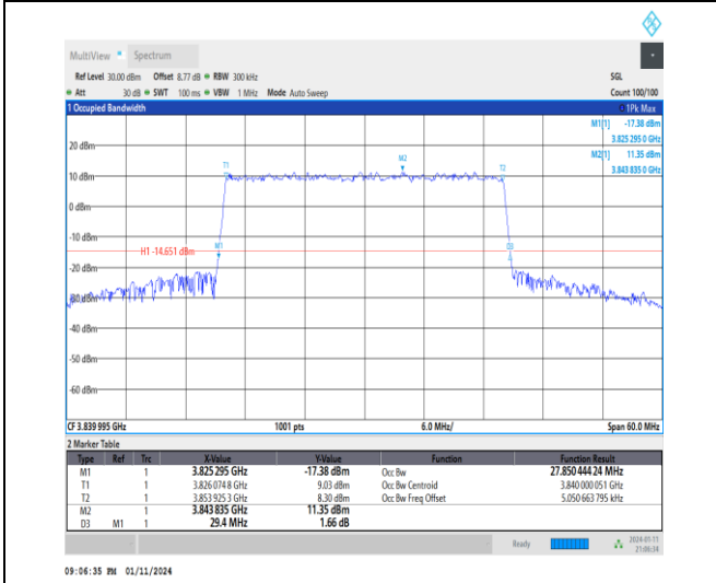
1-N77-3700-3980-30-30-M-6-CP-QPSK-Outer_Full-7 8@0-Ant2-27.85-29.400-≤30-PASS
