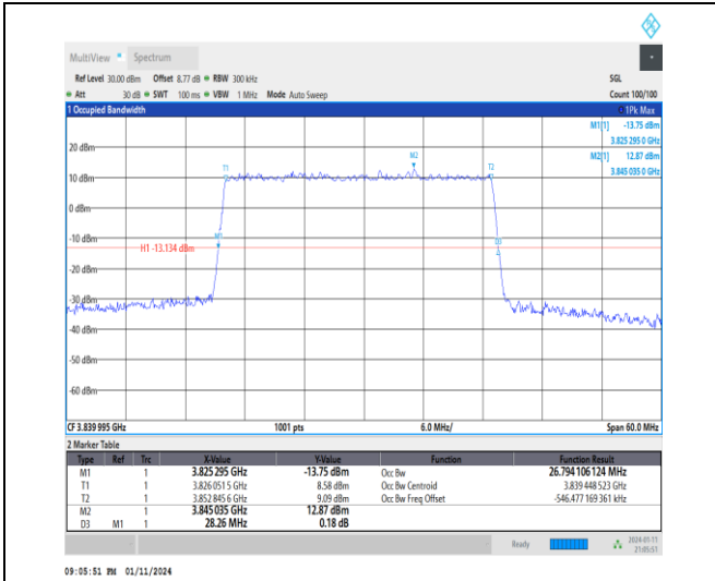
1-N77-3700-3980-30-30-M-4-DFT-64QAM-Outer_Ful I-75@0-Ant2-26.794-28.260-≤30-PASS
