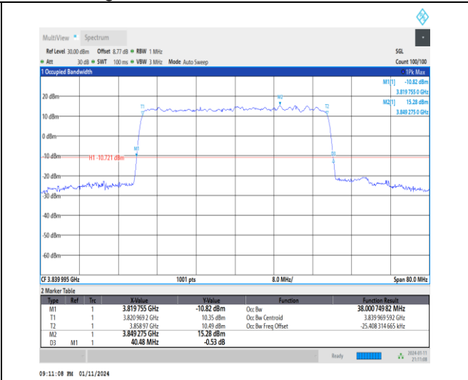
1-N77-3700-3980-30-40-M-8-CP-64QAM-Outer_Full-106@0-Ant2-38.001-40.480-≤40-PASS
