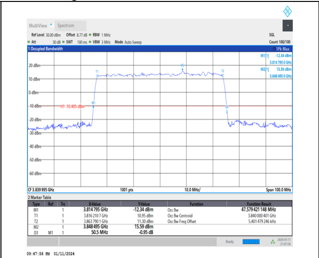
1-N77-3700-3980-30-50-M-7-CP-16QAM-Outer_Full -133@0-Ant2-47.579-50.500-≤50-PASS
