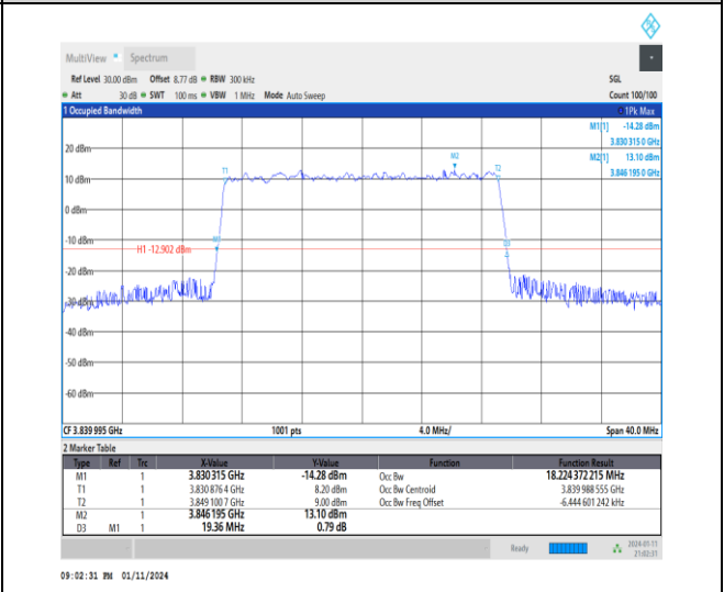
1-N77-3700-3980-30-20-M-8-CP-64QAM-Outer_Full-51@0-Ant2-18.224-19.360-≤20-PASS
