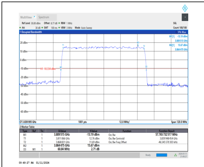
1-N77-3700-3980-30-60-M-1-DFT-QPSK-Outer_Full-162@0-Ant2-57.766-60.840-≤60-PASS
