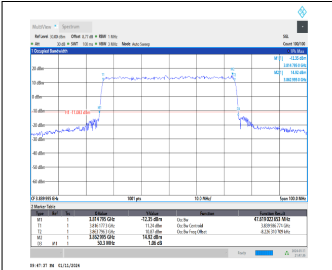
1-N77-3700-3980-30-50-M-6-CP-QPSK-Outer_Full-1 33@0-Ant2-47.619-50.300-≤50-PASS
