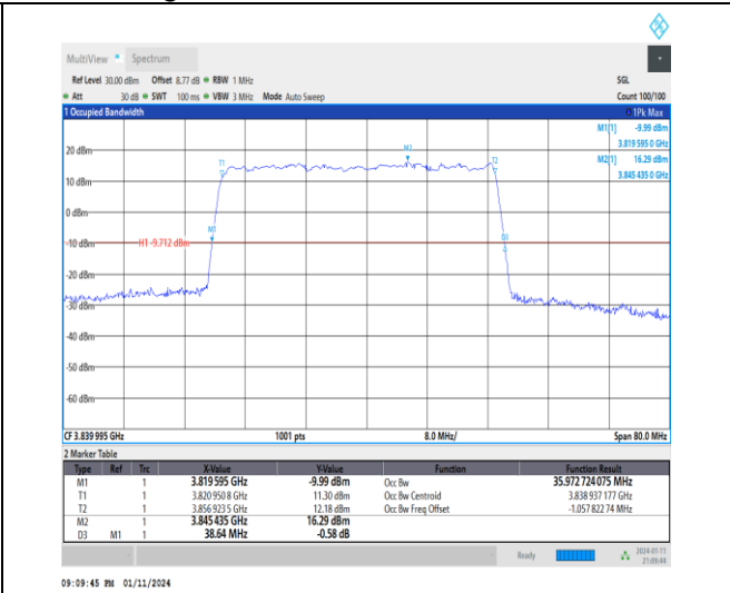
1-N77-3700-3980-30-40-M-4-DFT-64QAM-Outer_Fu II-100@0-Ant2-35.973-38.640-≤40-PASS
