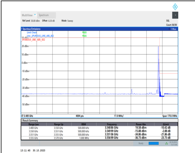
1-N77-3450-3550-30-60-H-2-DFT-PI2BPSK-Edge_1R_B_Right-1@161-Ant2-1--PASS-see graph
