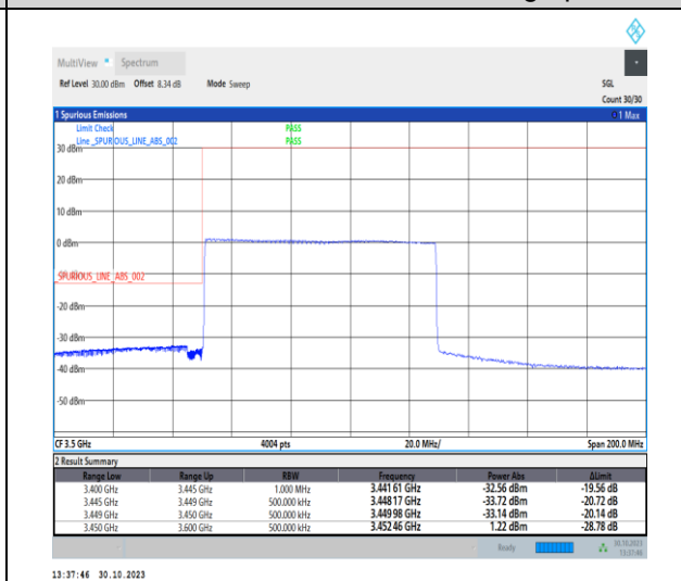
1-N77-3450-3550-30-80-L-6-CP-QPSK-Outer_Full -217@0-Ant2-1--PASS-see graph
