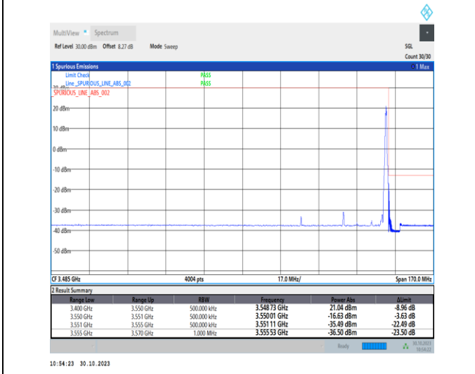
1-N77-3450-3550-30-40-H-5-CP-QPSK-Edge_1RB_Right-1@105-Ant2-1--PASS-see graph
