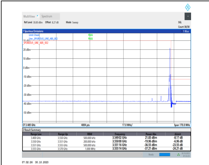
1-N77-3450-3550-30-20-H-2-DFT-PI2BPSK-Edge_1R_B_Right-1@50-Ant2-1--PASS-see graph
