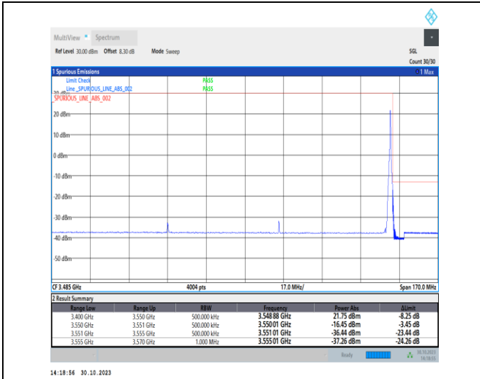
1-N77-3450-3550-30-100-H-2-DFT-PI2BPSK-Edge_1R_B_Right-1@272-Ant2-1--PASS-see graph
