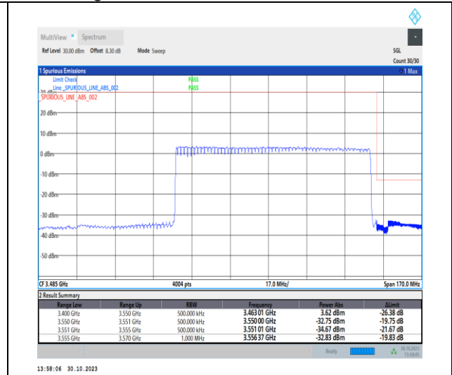
1-N77-3450-3550-30-90-H-3-DFT-PI2BPSK-Outer_Full-240@0-Ant2-1--PASS-see graph
