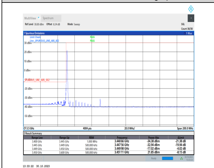
1-N77-3450-3550-30-80-L-4-CP-QPSK-Edge_1RB_Lef t-1@0-Ant2-1--PASS-see graph
