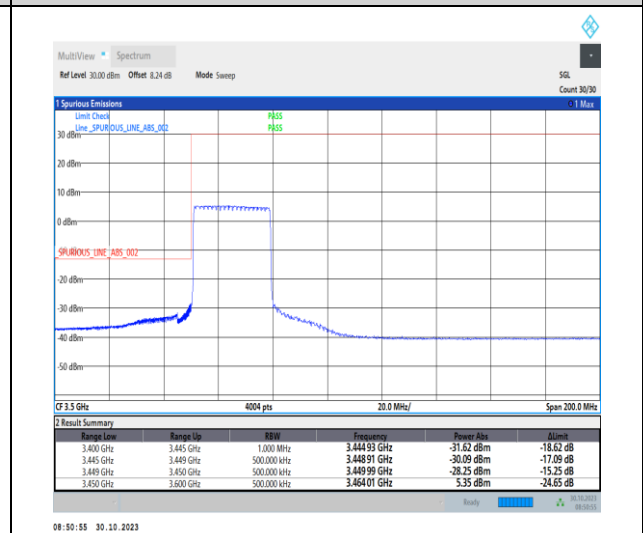
1-N77-3450-3550-30-30-L-6-CP-QPSK-Outer_Full -78@0-Ant2-1--PASS-see graph
