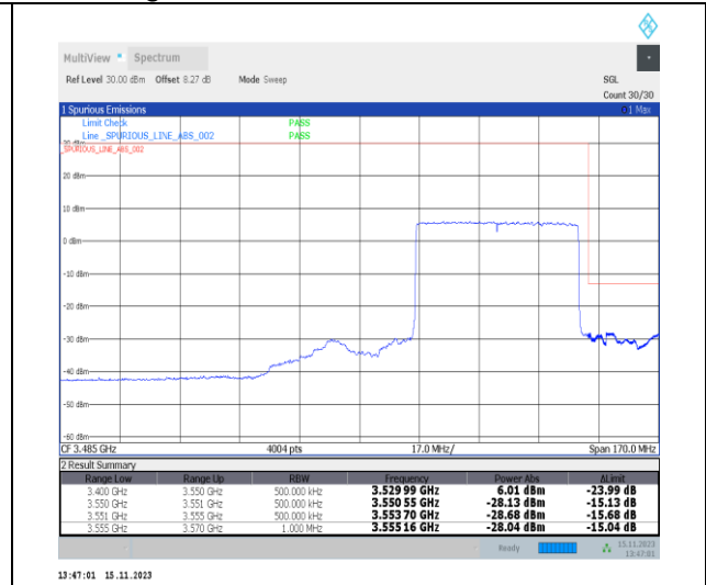
1-N77-3450-3550-30-50-H-3-DFT-PI2BPSK-Outer_Full-128@0-Ant2-1--PASS-see graph
