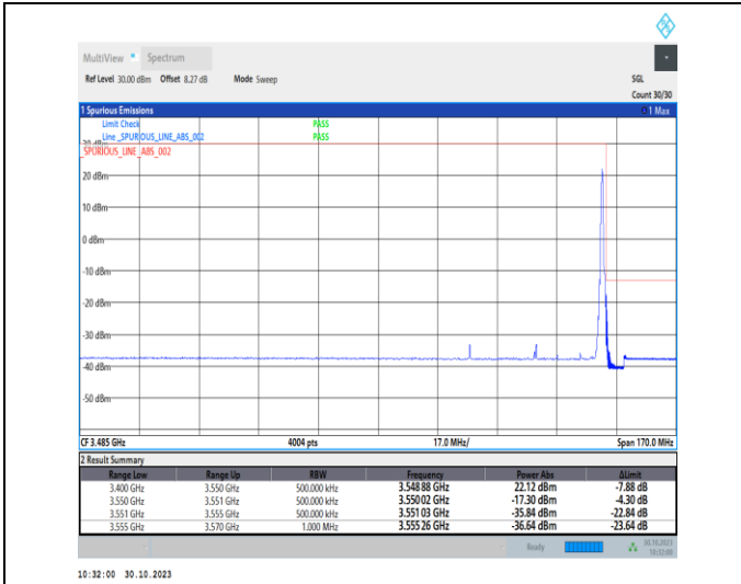
1-N77-3450-3550-30-40-H-2-DFT-PI2BPSK-Edge_1R_B_Right-1@105-Ant2-1--PASS-see graph
