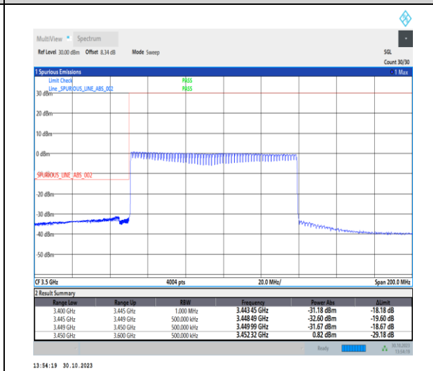
1-N77-3450-3550-30-90-L-6-CP-QPSK-Outer_Full -245@0-Ant2-1--PASS-see graph
