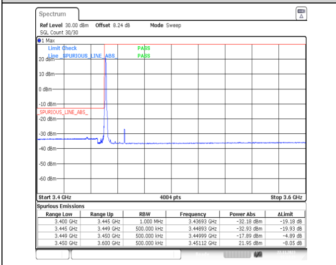
1-N77-3450-3550-30-30-L-4-CP-QPSK-Edge_1RB_Lef t-1@0-Ant2-1--PASS-see graph
