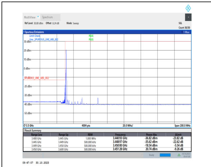
1-N77-3450-3550-30-40-L-1-DFT-PI2BPSK-Edge_1RB _Left-1@0-Ant2-1--PASS-see graph
