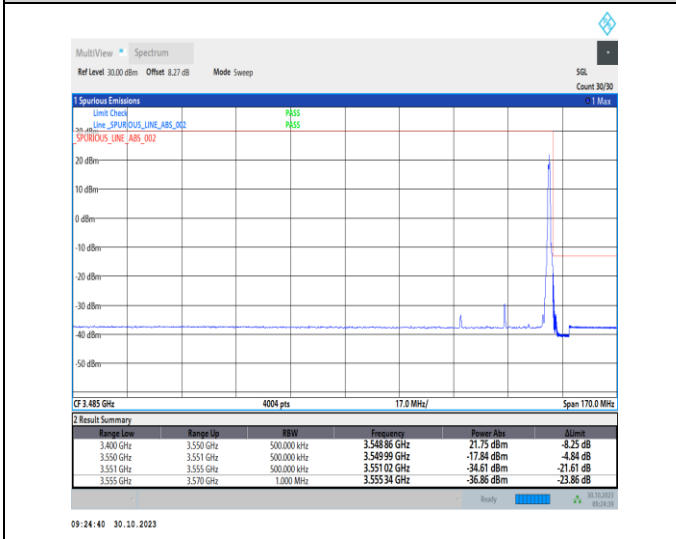
1-N77-3450-3550-30-30-H-5-CP-QPSK-Edge_1RB_Right-1@77-Ant2-1--PASS-see graph
