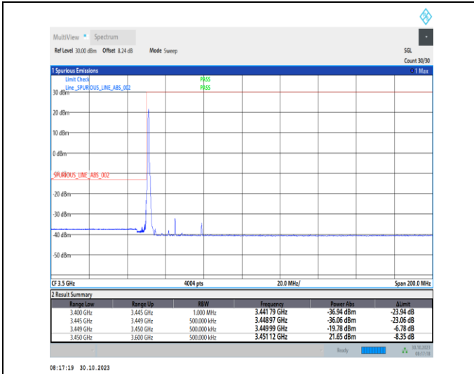
1-N77-3450-3550-30-30-L-1-DFT-PI2BPSK-Edge_1RB _Left-1@0-Ant2-1--PASS-see graph
