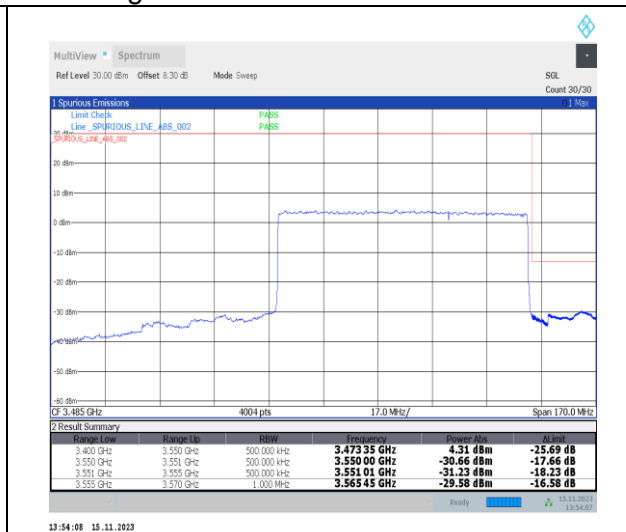
1-N77-3450-3550-30-80-H-3-DFT-PI2BPSK-Outer_Full-216@0-Ant2-1--PASS-see graph
