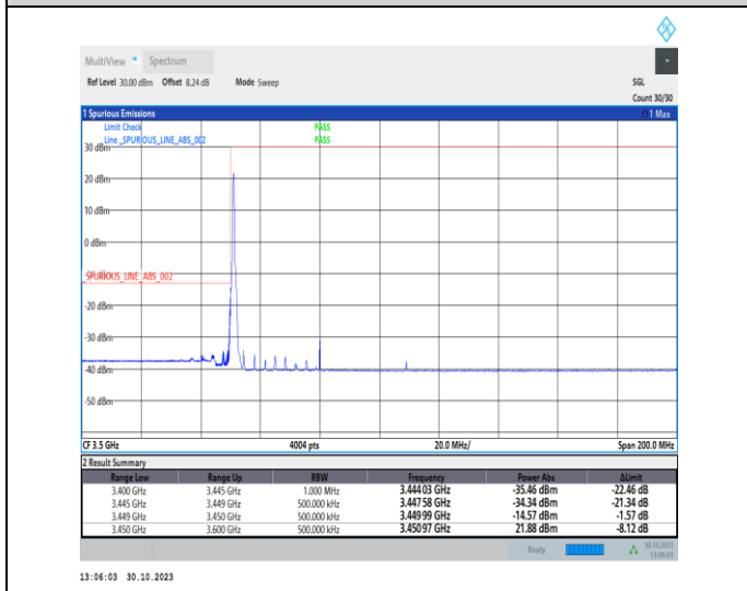
1-N77-3450-3550-30-60-L-4-CP-QPSK-Edge_1RB_Lef t-1@0-Ant2-1--PASS-see graph
