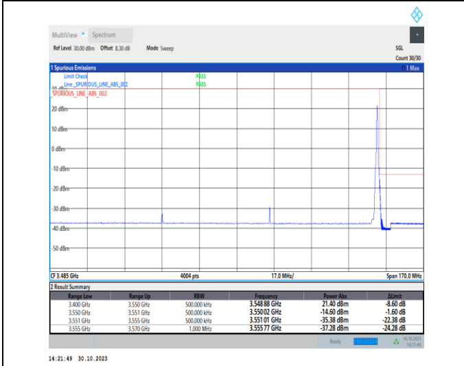
1-N77-3450-3550-30-100-H-5-CP-QPSK-Edge_1RB_Right-1@272-Ant2-1--PASS-see graph
