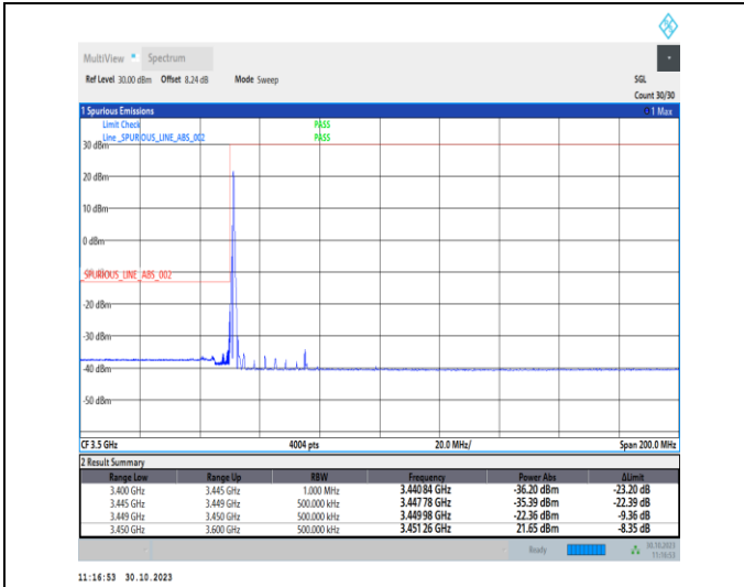
1-N77-3450-3550-30-50-L-1-DFT-PI2BPSK-Edge_1RB _Left-1@0-Ant2-1--PASS-see graph
