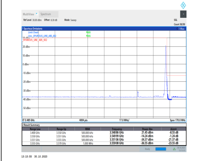
1-N77-3450-3550-30-60-H-5-CP-QPSK-Edge_1RB_Right-1@161-Ant2-1--PASS-see graph
