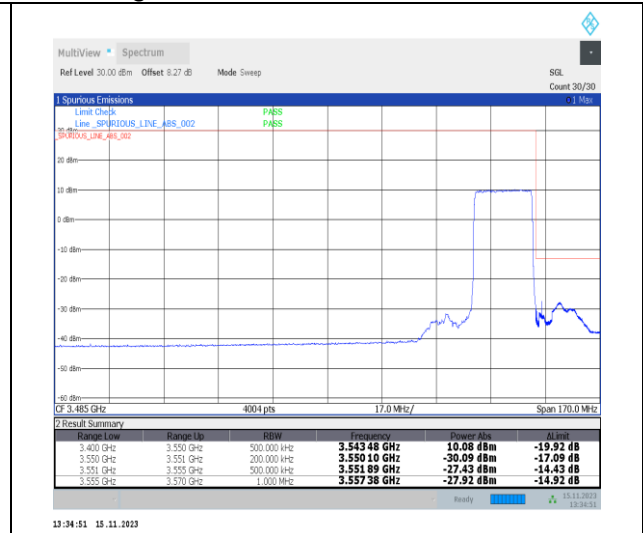
1-N77-3450-3550-30-20-H-3-DFT-PI2BPSK-Outer_Full-50@0-Ant2-1--PASS-see graph
