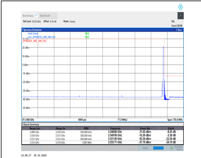
1-N77-3450-3550-30-90-H-2-DFT-PI2BPSK-Edge_1R B_Right-1@244-Ant2-1--PASS-see graph
