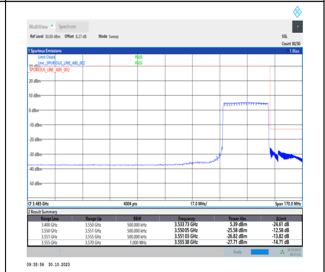
1-N77-3450-3550-30-30-H-6-CP-QPSK-Outer_Full-78@0-Ant2-1--PASS-see graph
