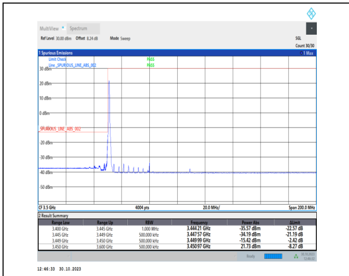
1-N77-3450-3550-30-60-L-1-DFT-PI2BPSK-Edge_1RB _Left-1@0-Ant2-1--PASS-see graph
