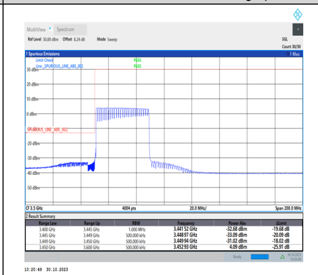
1-N77-3450-3550-30-40-L-6-CP-QPSK-Outer_Full -106@0-Ant2-1--PASS-see graph
