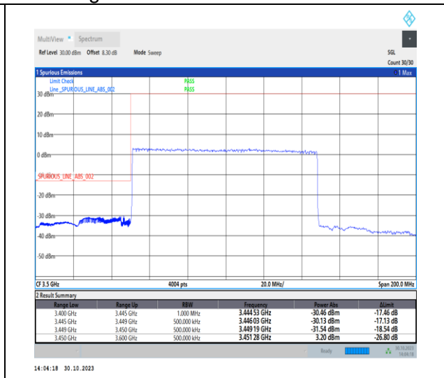
1-N77-3450-3550-30-100-L-3-DFT-PI2BPSK-Outer_Full-270@0-Ant2-1--PASS-see graph
