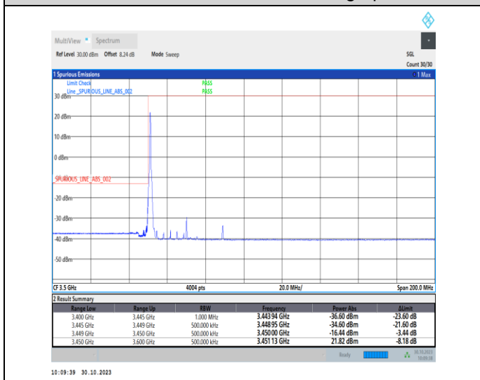
1-N77-3450-3550-30-40-L-4-CP-QPSK-Edge_1RB_Lef t-1@0-Ant2-1--PASS-see graph
