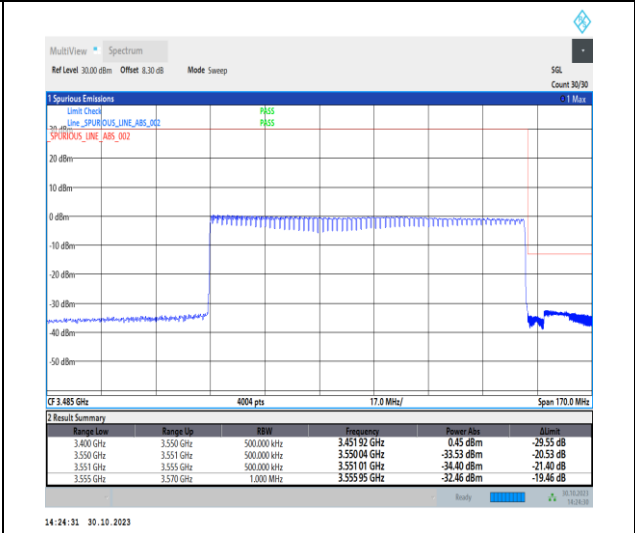
1-N77-3450-3550-30-100-H-6-CP-QPSK-Outer_Full-273@0-Ant2-1--PASS-see graph
