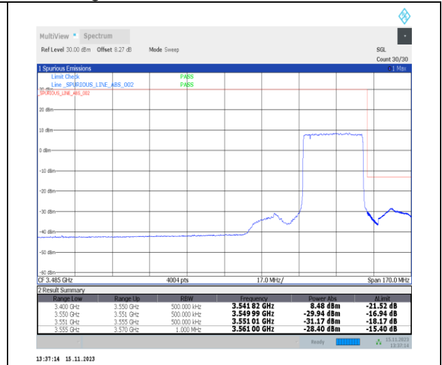
1-N77-3450-3550-30-30-H-3-DFT-PI2BPSK-Outer_Full-75@0-Ant2-1--PASS-see graph
