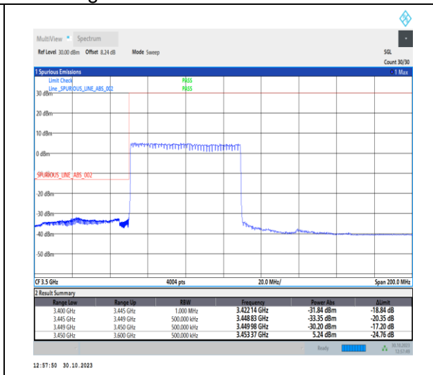
1-N77-3450-3550-30-60-L-3-DFT-PI2BPSK-Outer _Full-162@0-Ant2-1--PASS-see graph
