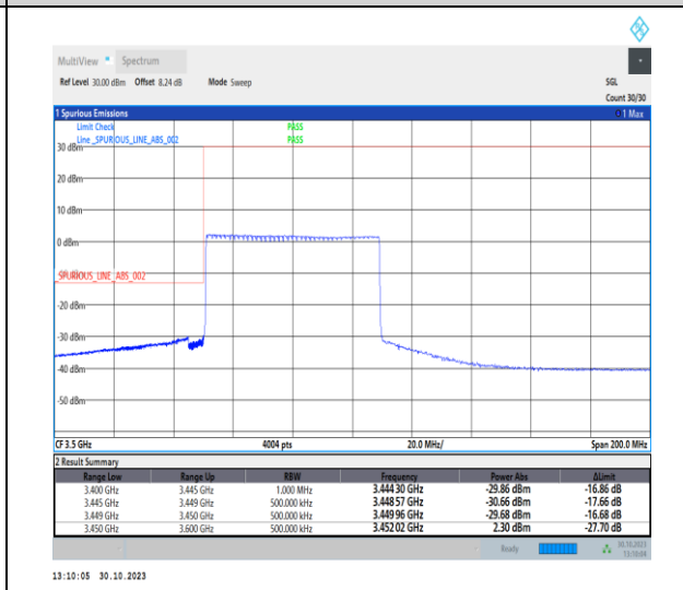
1-N77-3450-3550-30-60-L-6-CP-QPSK-Outer_Full -162@0-Ant2-1--PASS-see graph
