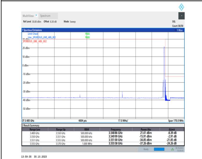
1-N77-3450-3550-30-90-H-5-CP-QPSK-Edge_1RB_Right-1@244-Ant2-1--PASS-see graph
