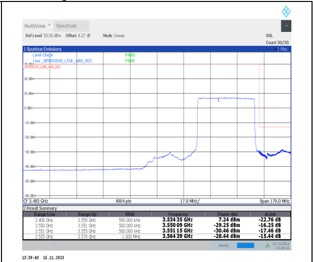
1-N77-3450-3550-30-40-H-3-DFT-PI2BPSK-Outer_Full-100@0-Ant2-1--PASS-see graph
