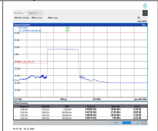
1-N77-3450-3550-30-50-L-3-DFT-PI2BPSK-Outer _Full-128@0-Ant2-1--PASS-see graph
