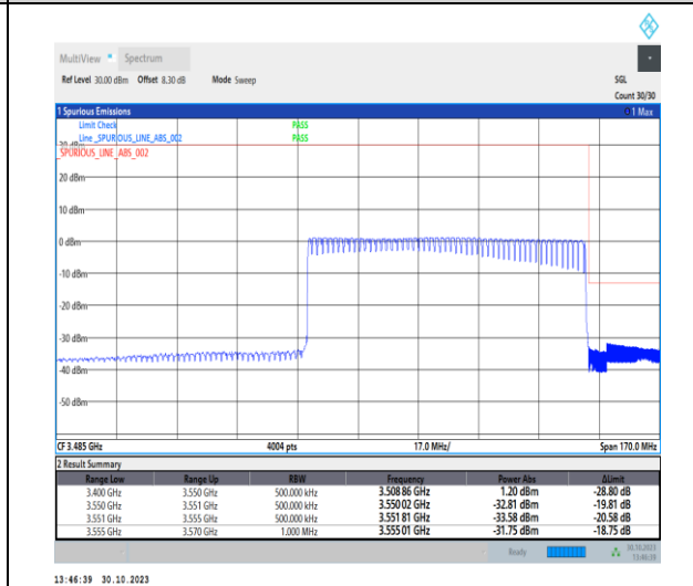
1-N77-3450-3550-30-80-H-6-CP-QPSK-Outer_Full-217@0-Ant2-1--PASS-see graph
