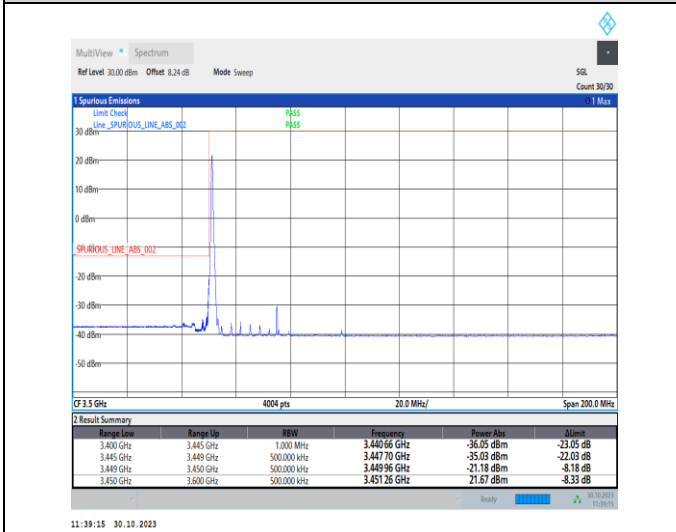
1-N77-3450-3550-30-50-L-4-CP-QPSK-Edge_1RB_Lef t-1@0-Ant2-1--PASS-see graph
