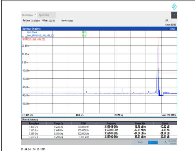
1-N77-3450-3550-30-80-H-5-CP-QPSK-Edge_1RB_Right-1@216-Ant2-1--PASS-see graph
