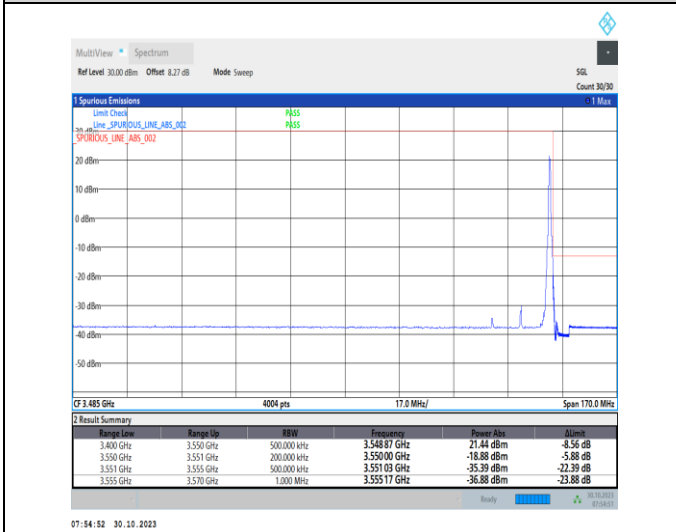
1-N77-3450-3550-30-20-H-5-CP-QPSK-Edge_1RB_Right-1@50-Ant2-1--PASS-see graph
