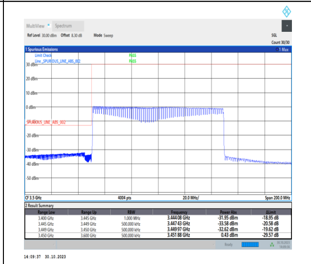
1-N77-3450-3550-30-100-L-6-CP-QPSK-Outer_Full-273@0-Ant2-1--PASS-see graph
