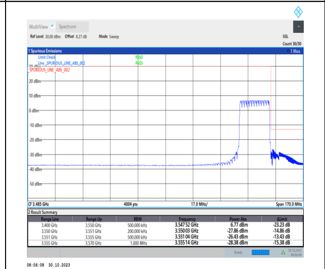
1-N77-3450-3550-30-20-H-6-CP-QPSK-Outer_Full-51@0-Ant2-1--PASS-see graph
