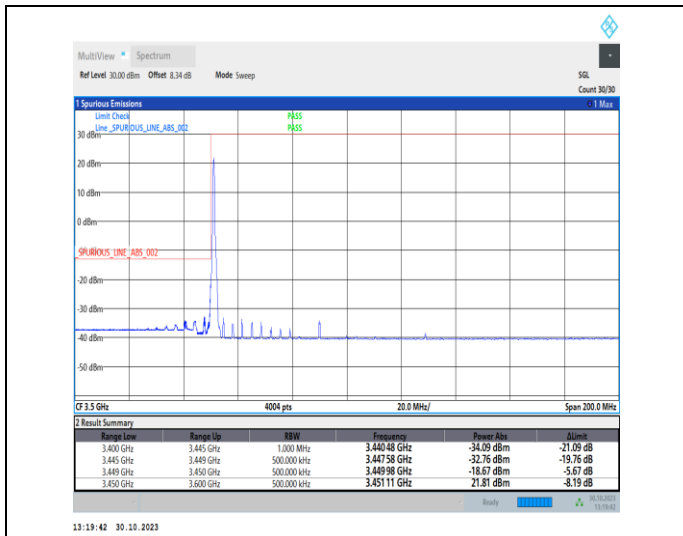
1-N77-3450-3550-30-80-L-1-DFT-PI2BPSK-Edge_1RB _Left-1@0-Ant2-1--PASS-see graph
