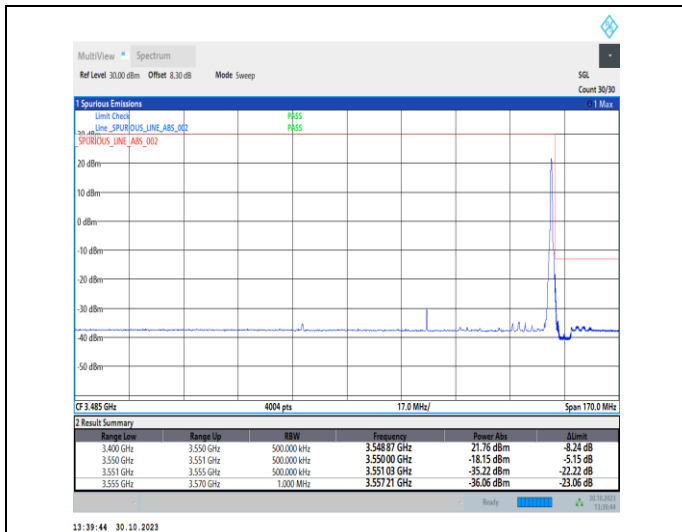
1-N77-3450-3550-30-80-H-2-DFT-PI2BPSK-Edge_1R_B_Right-1@216-Ant2-1--PASS-see graph
