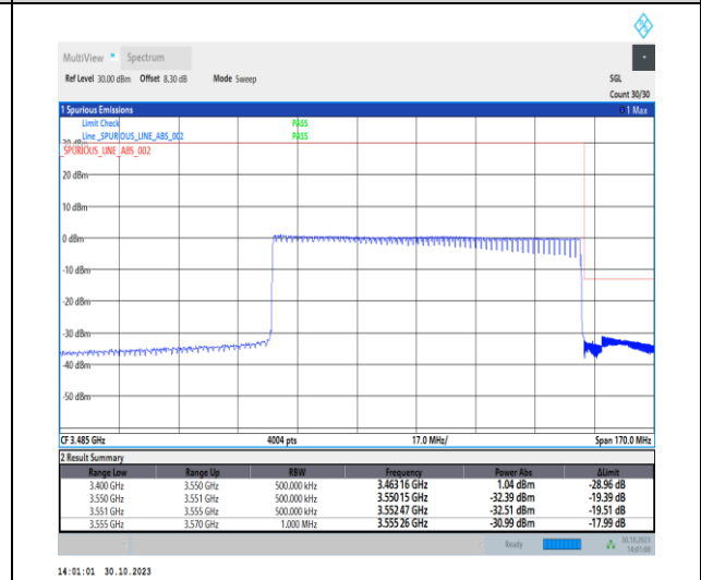
1-N77-3450-3550-30-90-H-6-CP-QPSK-Outer_Full-245@0-Ant2-1--PASS-see graph
