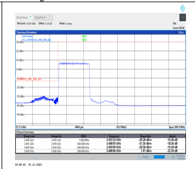
1-N77-3450-3550-30-40-L-3-DFT-PI2BPSK-Outer _Full-100@0-Ant2-1--PASS-see graph
