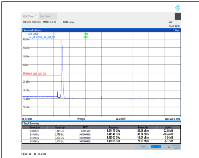
1-N77-3450-3550-30-100-L-1-DFT-PI2BPSK-Edge_1R_B_Left-1@0-Ant2-1--PASS-see graph
