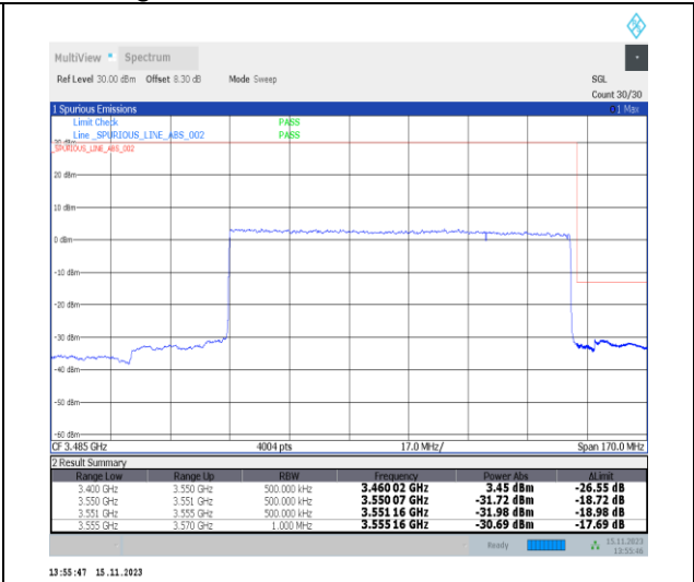
1-N77-3450-3550-30-100-H-3-DFT-PI2BPSK-Outer_Full-270@0-Ant2-1--PASS-see graph
