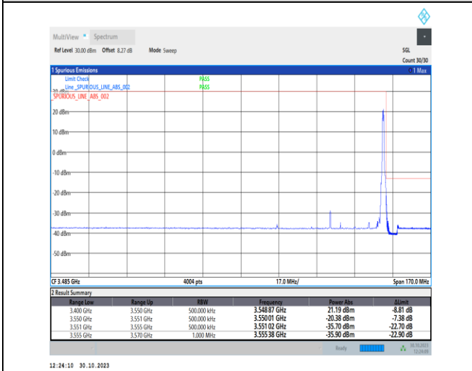
1-N77-3450-3550-30-50-H-5-CP-QPSK-Edge_1RB_Right-1@132-Ant2-1--PASS-see graph
