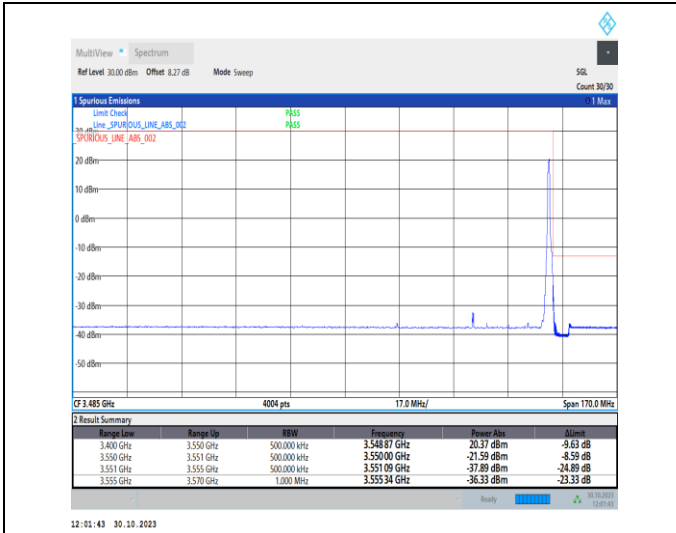
1-N77-3450-3550-30-50-H-2-DFT-PI2BPSK-Edge_1R_B_Right-1@132-Ant2-1--PASS-see graph
