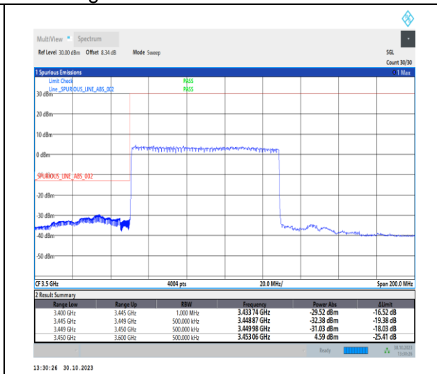
1-N77-3450-3550-30-80-L-3-DFT-PI2BPSK-Outer _Full-216@0-Ant2-1--PASS-see graph
