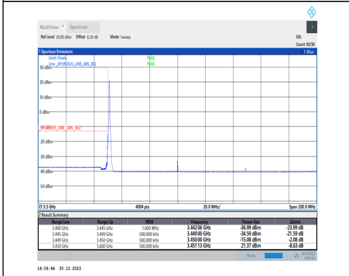
1-N77-3450-3550-30-100-L-4-CP-QPSK-Edge_1RB_Left-1@0-Ant2-1--PASS-see graph
