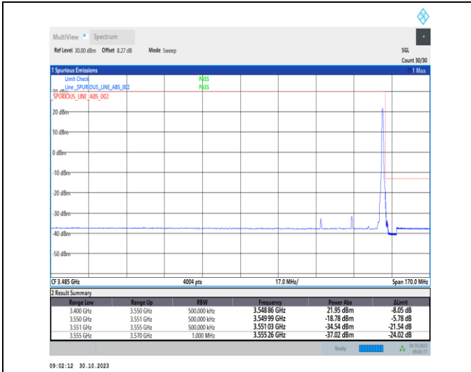
1-N77-3450-3550-30-30-H-2-DFT-PI2BPSK-Edge_1R_B_Right-1@77-Ant2-1--PASS-see graph
