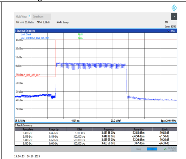
1-N77-3450-3550-30-90-L-3-DFT-PI2BPSK-Outer _Full-240@0-Ant2-1--PASS-see graph
