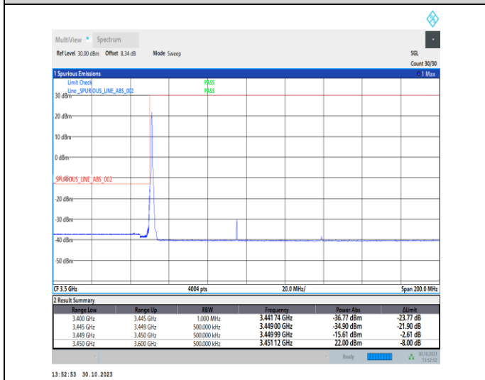
1-N77-3450-3550-30-90-L-4-CP-QPSK-Edge_1RB_Lef t-1@0-Ant2-1--PASS-see graph
