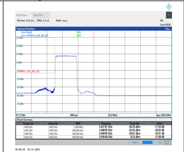
1-N77-3450-3550-30-30-L-3-DFT-PI2BPSK-Outer _Full-75@0-Ant2-1--PASS-see graph
