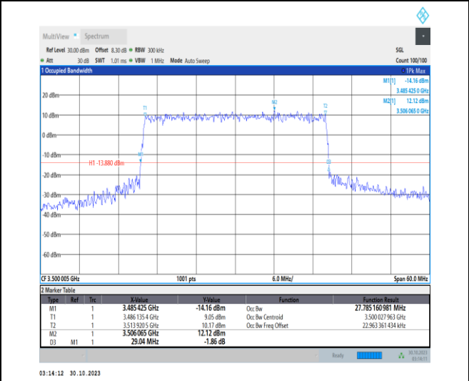
1-N77-3450-3550-30-30-M-7-CP-16QAM-Outer_Full-78 -78@0-Ant2-27.785-29.040-≤30-PASS
