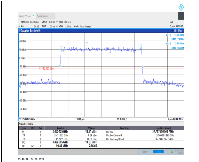
1-N77-3450-3550-30-60-M-1-DFT-QPSK-Outer_Full-162@0-Ant2-57.718-59.880-≤60-PASS
