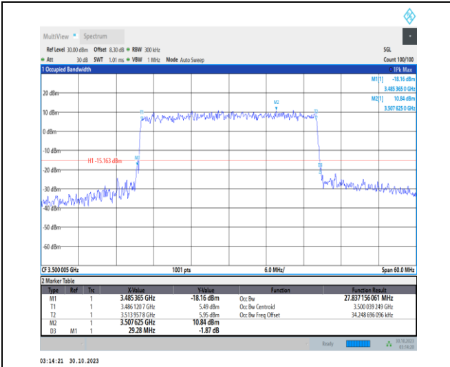
1-N77-3450-3550-30-30-M-8-CP-64QAM-Outer_Full-78@0-Ant2-27.837-29.280-≤30-PASS
