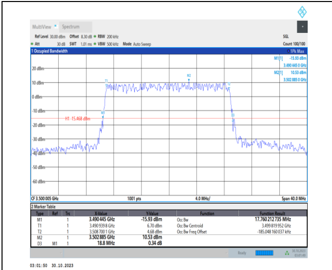
1-N77-3450-3550-30-20-M-5-DFT-256QAM-Outer_Full-50@0-Ant2-17.76-18.800-≤20-PASS
