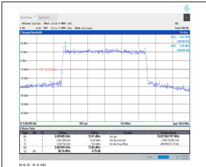
1-N77-3450-3550-30-80-M-4-DFT-64QAM-Outer_Ful I-216@0-Ant2-76.873-80.160-≤80-PASS
