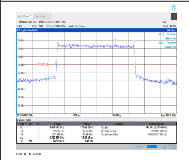
1-N77-3450-3550-30-90-M-2-DFT-PI2BPSK-Outer_Full-240@0-Ant2-85.518-88.920-≤90-PASS
