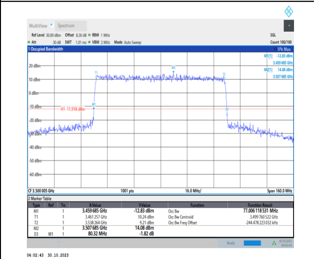
1-N77-3450-3550-30-80-M-3-DFT-16QAM-Outer_Full-216@0-Ant2-77.006-80.320-≤80-PASS
