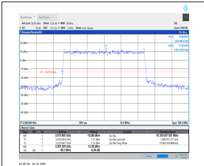
1-N77-3450-3550-30-50-M-6-CP-QPSK-Outer_Full-1 33@0-Ant2-47.335-49.500-≤50-PASS
