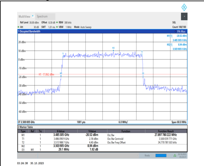
1-N77-3450-3550-30-30-M-9-CP-256QAM-Outer_Fu II-78@0-Ant2-27.898-29.100-≤30-PASS
