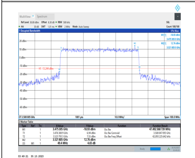
1-N77-3450-3550-30-50-M-8-CP-64QAM-Outer_Full-133@0-Ant2-47.492-49.400-≤50-PASS
