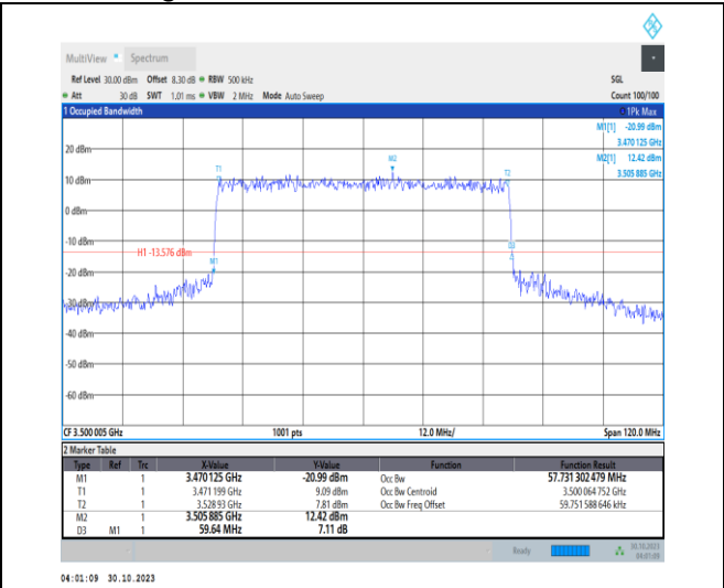
1-N77-3450-3550-30-60-M-6-CP-QPSK-Outer_Full-162@0-Ant2-57.731-59.640-≤60-PASS
