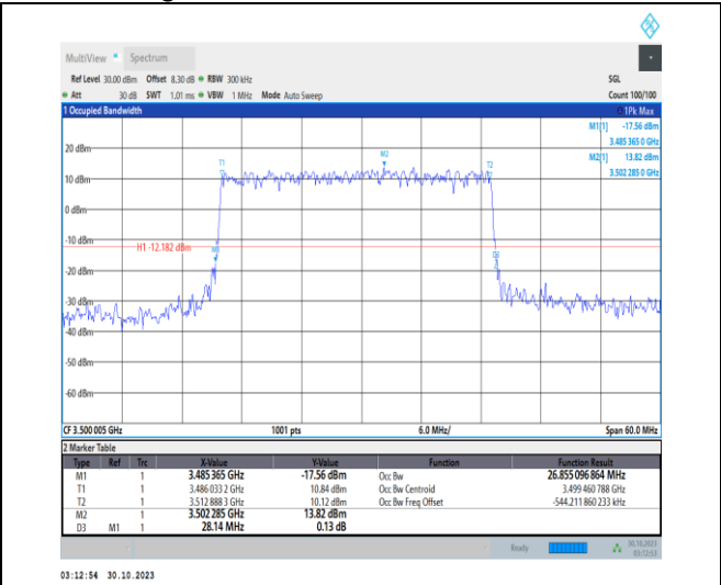
1-N77-3450-3550-30-30-M-1-DFT-QPSK-Outer_Full-75@0-Ant2-26.855-28.140-<=30-PASS
