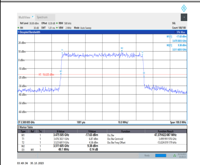
1-N77-3450-3550-30-50-M-9-CP-256QAM-Outer_Full-133@0-Ant2-47.38-49.100-≤50-PASS
