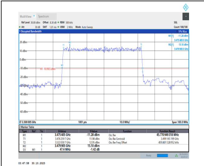
1-N77-3450-3550-30-50-M-2-DFT-PI2BPSK-Outer_Full-128@0-Ant2-45.771-47.400-≤50-PASS
