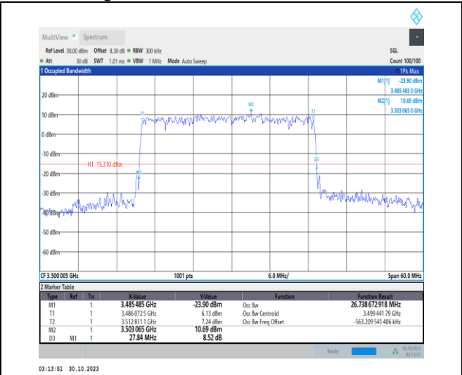
1-N77-3450-3550-30-30-M-5-DFT-256QAM-Outer_Full ull-75@0-Ant2-26.739-27.840-≤30-PASS
