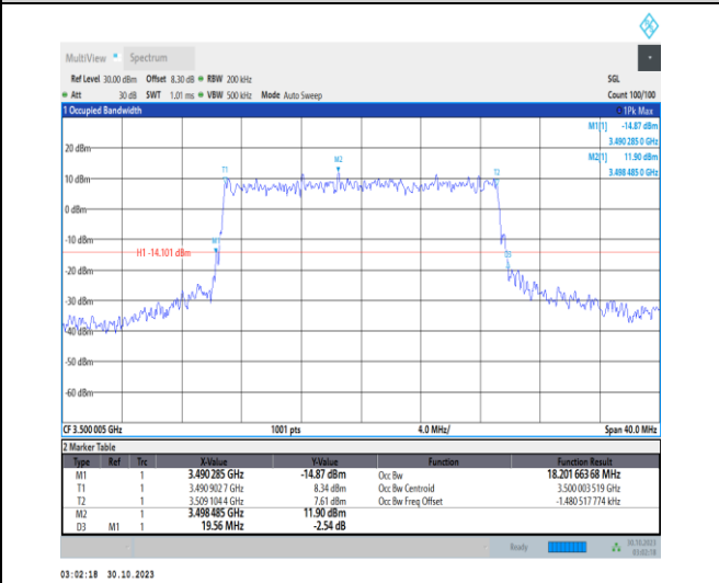
1-N77-3450-3550-30-20-M-8-CP-64QAM-Outer_Full-51@0-Ant2-18.202-19.560-≤20-PASS
