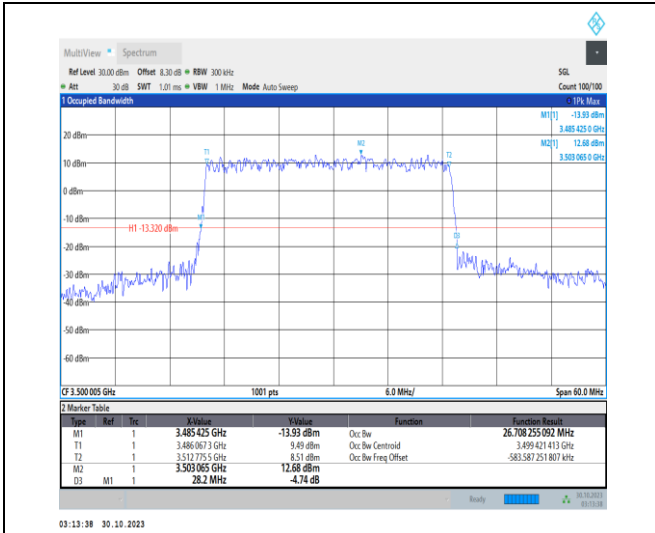
1-N77-3450-3550-30-30-M-4-DFT-64QAM-Outer_Full I-75@0-Ant2-26.708-28.200-≤30-PASS
