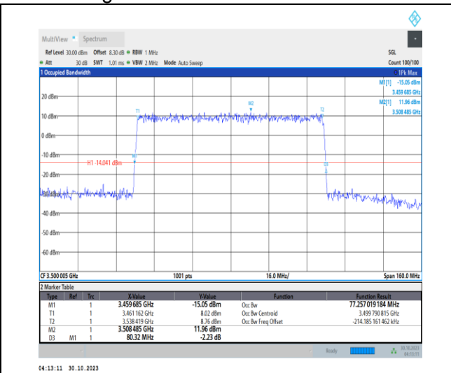
1-N77-3450-3550-30-80-M-5-DFT-256QAM-Outer_Full-216@0-Ant2-77.257-80.320-≤80-PASS
