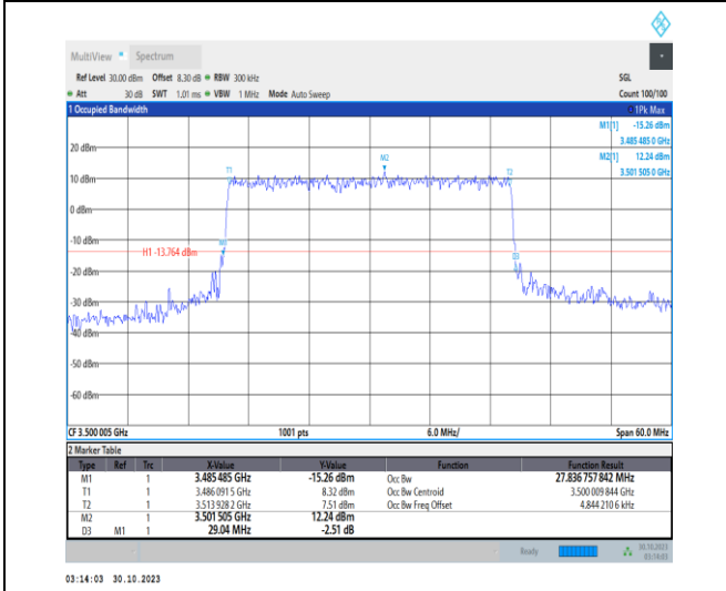
1-N77-3450-3550-30-30-M-6-CP-QPSK-Outer_Full-7 8@0-Ant2-27.837-29.040-≤30-PASS
