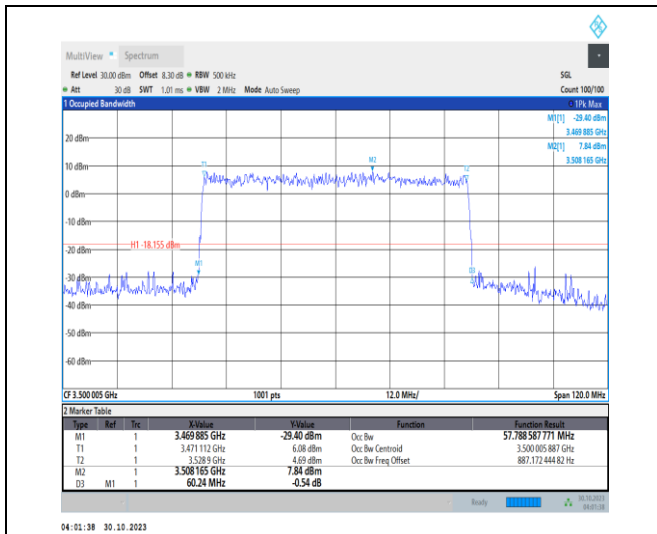
1-N77-3450-3550-30-60-M-9-CP-256QAM-Outer_Ful I-162@0-Ant2-57.789-60.240-≤60-PASS
