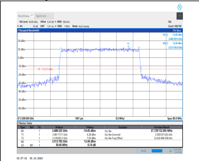
1-N77-3450-3550-30-40-M-8-CP-64QAM-Outer_Full-106@0-Ant2-37.729-39.440-≤40-PASS
