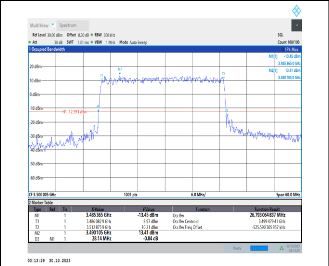
1-N77-3450-3550-30-30-M-3-DFT-16QAM-Outer_Full-75@0-Ant2-26.793-28.140-<=30-PASS
