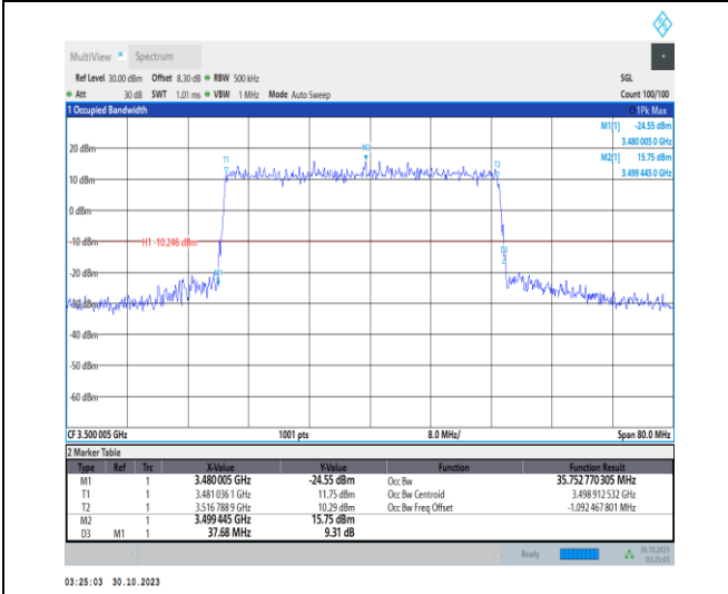
1-N77-3450-3550-30-40-M-1-DFT-QPSK-Outer_Full-100@0-Ant2-35.753-37.680-≤40-PASS
