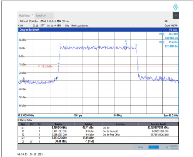
1-N77-3450-3550-30-40-M-7-CP-16QAM-Outer_Full-106@0-Ant2-37.74-39.440-≤40-PASS
