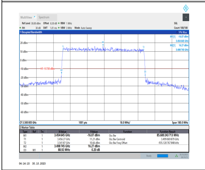
1-N77-3450-3550-30-90-M-1-DFT-QPSK-Outer_Full-240@0-Ant2-85.6-88.920-≤90-PASS
