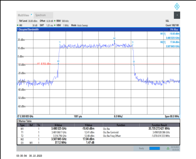
1-N77-3450-3550-30-40-M-2-DFT-PI2BPSK-Outer_Full-100@0-Ant2-35.735-37.120-≤40-PASS
