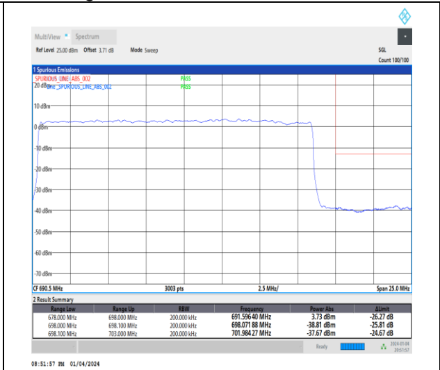
1-N71-15-20-H-3-DFT-PI2BPSK-Outer_Full-100@0-Ant1-1--PASS-see graph
