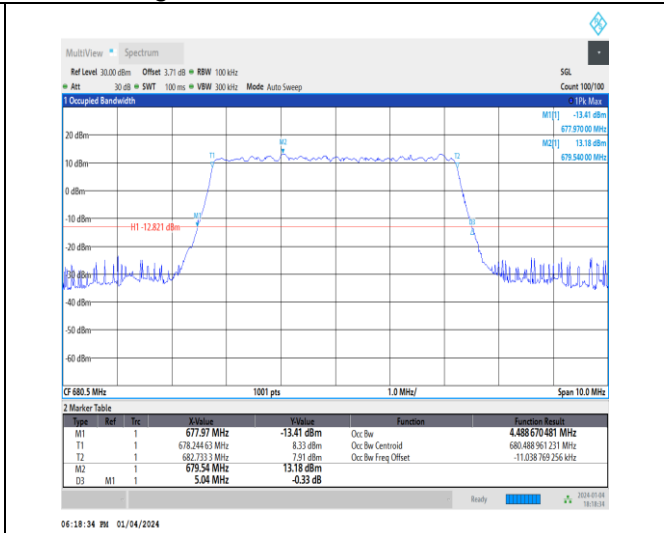
1-N71-15-5-M-6-CP-QPSK-Outer_Full-25@0-Ant1-4. 489-5.040-≤5-PASS
