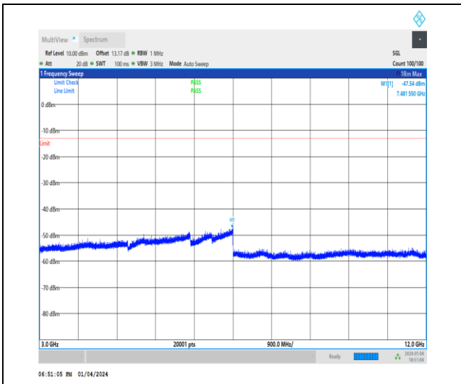
1-N71-15-20-H-1-DFT-PI2BPSK-Inner_1RB_Left-1 @ 1-3000-12000-Ant1-7481.55--47.54--13-PASS
