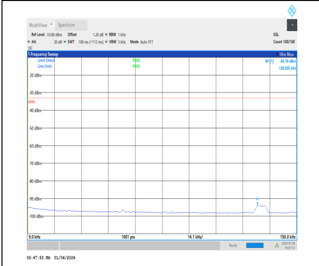
1-N71-15-20-M-1-DFT-PI2BPSK-Inner_1RB_Left-1 @ 1-0.009-0.15-Ant1-0.13--93.76--33-PASS
