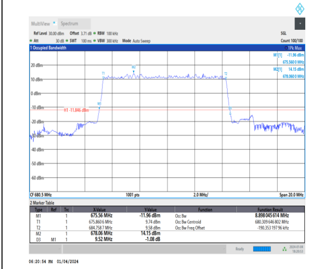
1-N71-15-10-M-2-DFT-PI2BPSK-Outer_Full-50@0-A nt1-8.898-9.520-≤10-PASS
