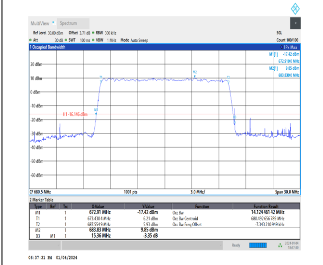
1-N71-15-15-M-9-CP-256QAM-Outer_Full-79@0-Ant t1-14.124-15.360-≤15-PASS
