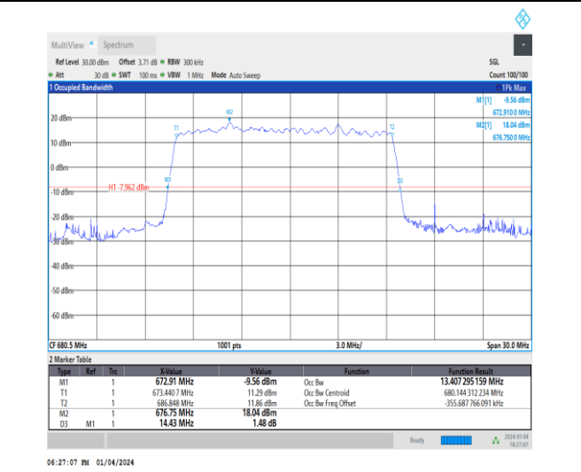
1-N71-15-15-M-2-DFT-PI2BPSK-Outer_Full-75@0-Ant1 nt1-13.407-14.430≤15-PASS
