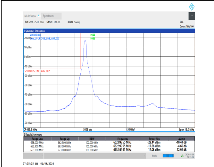
1-N71-15-10-L-4-CP-QPSK-Edge_1RB_Left-1@0-Ant1-1--PASS-see graph
