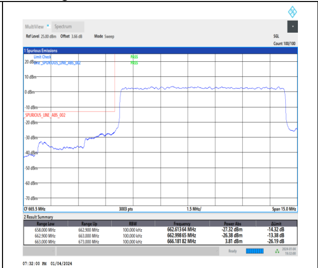
1-N71-15-10-L-3-DFT-PI2BPSK-Outer_Full-50@0-Ant1-1--PASS-see graph
