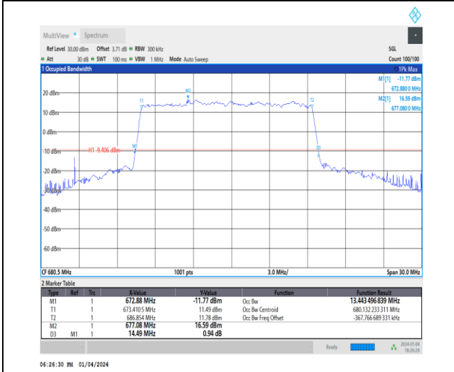
1-N71-15-15-M-1-DFT-QPSK-Outer_Full-75@0-Ant1 -13.443-14.490≤15-PASS
