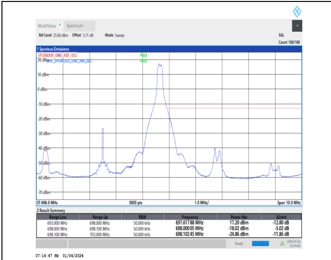
1-N71-15-5-H-2-DFT-PI2BPSK-Edge_1RB_Right-1@2 4-Ant1-1--PASS-see graph
