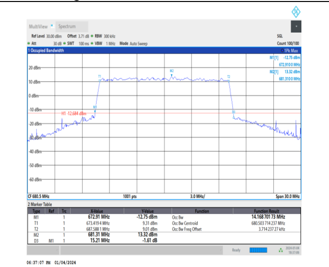
1-N71-15-15-M-8-CP-64QAM-Outer_Full-79@0-Ant1 -14.169-15.210-≤15-PASS
