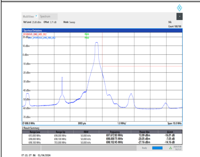
1-N71-15-5-H-5-CP-QPSK-Edge_1RB_Right-1@24-Ant1-1--PASS-see graph
