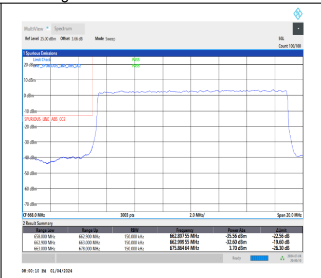
1-N71-15-15-L-3-DFT-PI2BPSK-Outer_Full-75@0-Ant1-1--PASS-see graph
