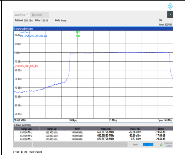
1-N71-15-10-L-6-CP-QPSK-Outer_Full-52@0-Ant1-1--PASS-see graph
