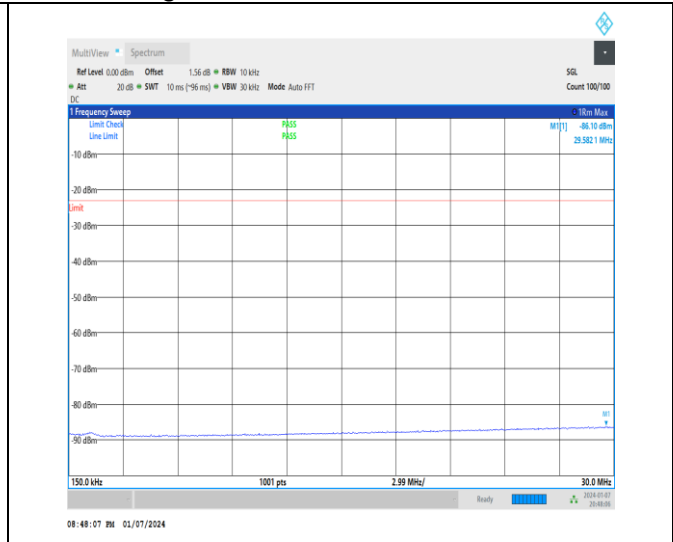
1-N71-15-20-H-1-DFT-PI2BPSK-Inner_1RB_Left-1 @ 1-0.15-30-Ant1-30.00--86.10--23-PASS
