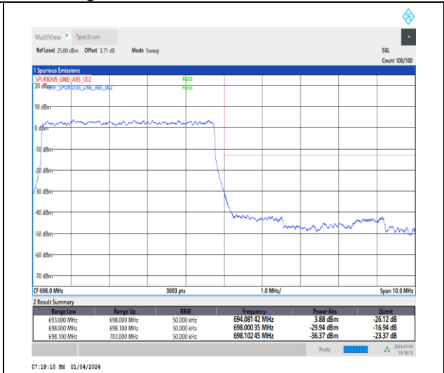
1-N71-15-5-H-3-DFT-PI2BPSK-Outer_Full-25@0-Ant1-1--PASS-see graph
