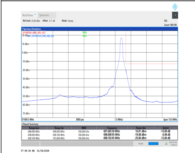
1-N71-15-10-H-5-CP-QPSK-Edge_1RB_Right-1@51-Ant1-1--PASS-see graph
