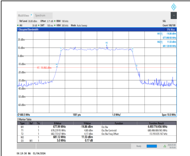
1-N71-15-5-M-9-CP-256QAM-Outer_Full-25@0-Ant 1-4.494-5.000-≤5-PASS
