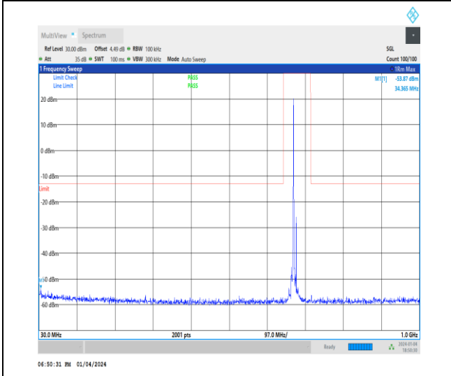
1-N71-15-20-H-1-DFT-PI2BPSK-Inner_1RB_Left-1 @ 1-30-1000-Ant1-34.37--53.87--13-PASS
