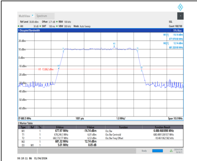
1-N71-15-5-M-5-DFT-256QAM-Outer_Full-25@0-An t1-4.486-5.010-≤5-PASS
