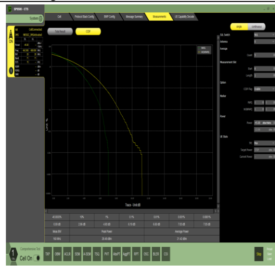
1-N71-PC3-15-20-H-15-NS_01-CP-256QAM-Outer_ Full-100@0-6.10
