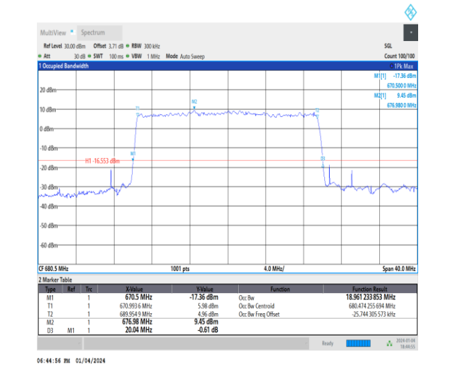
1-N71-15-20-M-9-CP-256QAM-Outer_Full-106@0-Ant nt1-18.961-20.040-≤20-PASS
