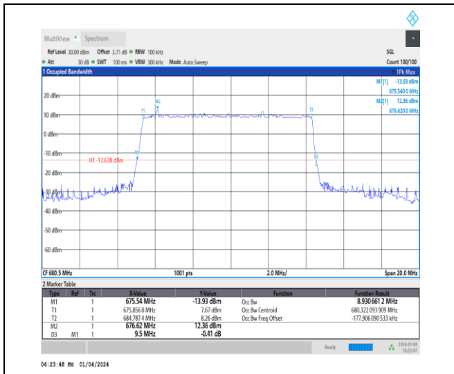
1-N71-15-10-M-4-DFT-64QAM-Outer_Full-50@0-An t1-8.931-9.500-≤10-PASS
