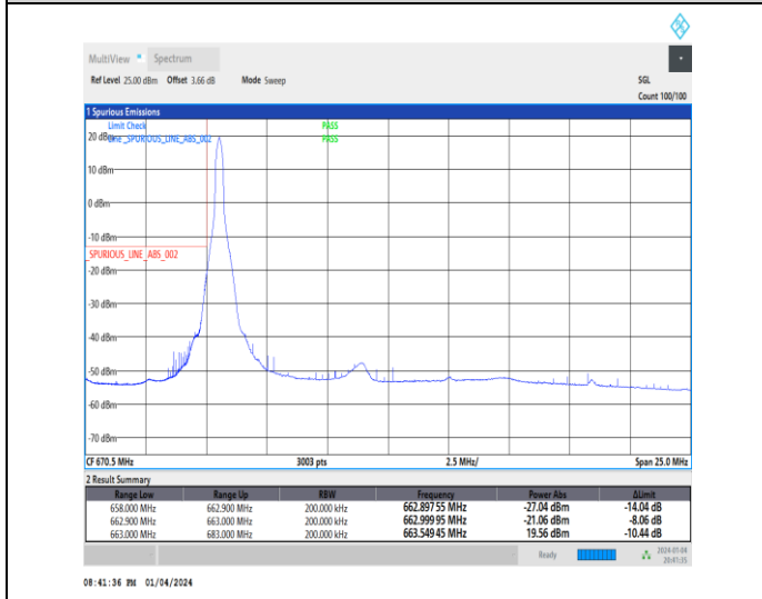
1-N71-15-20-L-4-CP-QPSK-Edge_1RB_Left-1@0-Ant1-1--PASS-see graph
