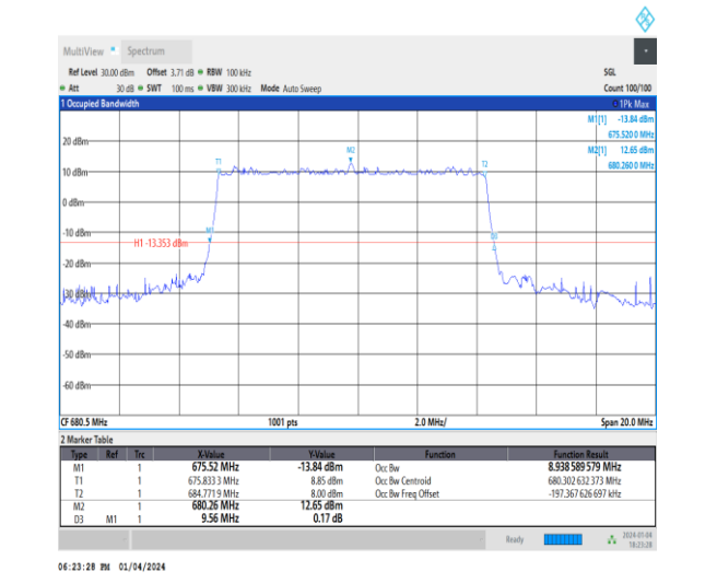
1-N71-15-10-M-3-DFT-16QAM-Outer_Full-50@0-Ant 1-8.939-9.560-≤10-PASS
