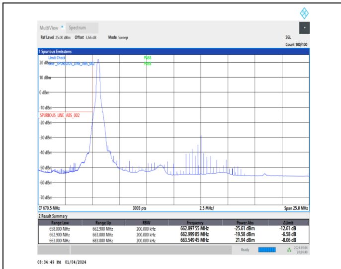
1-N71-15-20-L-1-DFT-PI2BPSK-Edge_1RB_Left-1@0-Ant1-1--PASS-see graph
