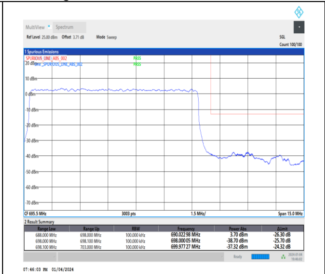
1-N71-15-10-H-3-DFT-PI2BPSK-Outer_Full-50@0-Ant1-1--PASS-see graph
