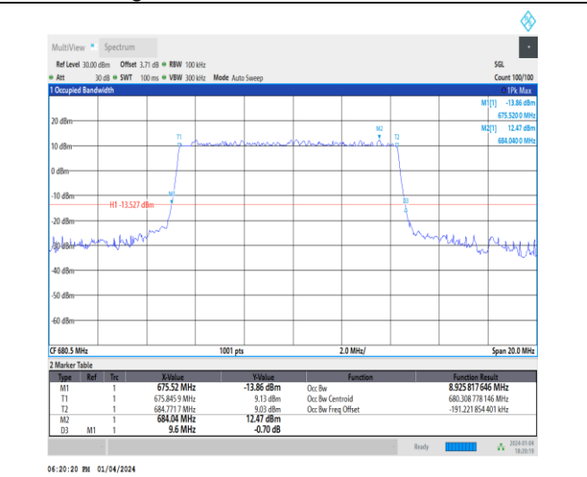
1-N71-15-10-M-1-DFT-QPSK-Outer_Full-50@0-Ant1 -8.926-9.600-≤10-PASS
