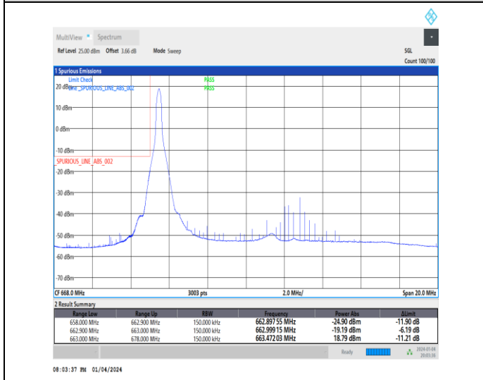
1-N71-15-15-L-4-CP-QPSK-Edge_1RB_Left-1@0-Ant1-1--PASS-see graph
