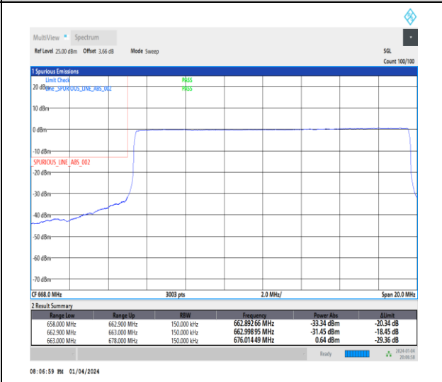
1-N71-15-15-L-6-CP-QPSK-Outer_Full-79@0-Ant1-1--PASS-see graph
