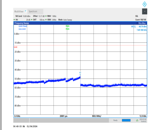
1-N71-15-20-M-1-DFT-PI2BPSK-Inner_1RB_Left-1 @ 1-3000-12000-Ant1-7491.90--46.79--13-PASS
