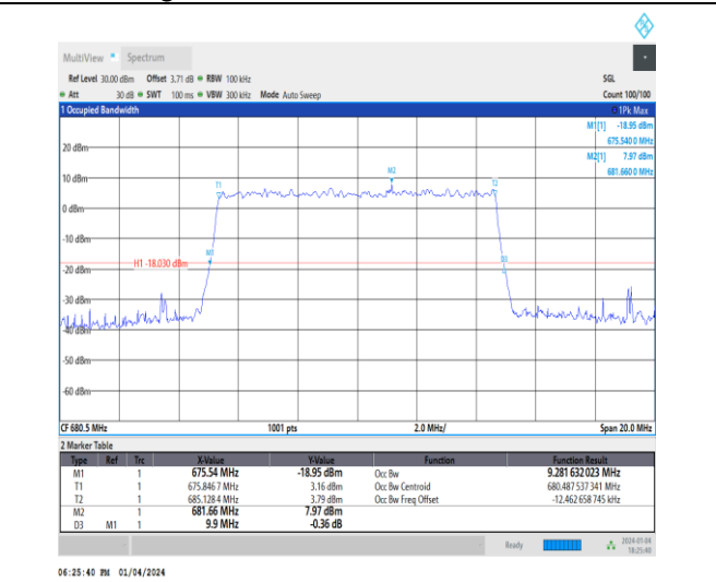
1-N71-15-10-M-9-CP-256QAM-Outer_Full-52@0-Ant 1-9.282-9.900≤10-PASS
