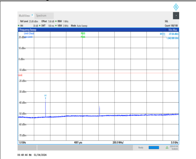
1-N71-15-20-M-1-DFT-PI2BPSK-Inner_1RB_Left-1 @ 1-1000-3000-Ant1-1342.00--37.04--13-PASS
