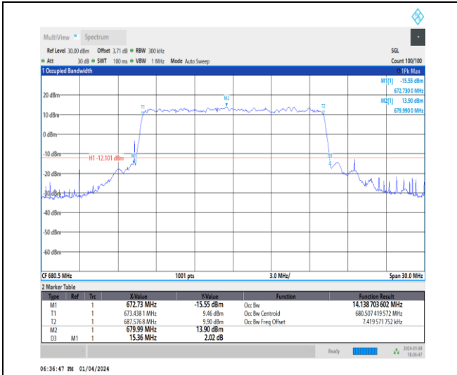
1-N71-15-15-M-7-CP-16QAM-Outer_Full-79@0-Ant 1-14.139-15.360-≤15-PASS
