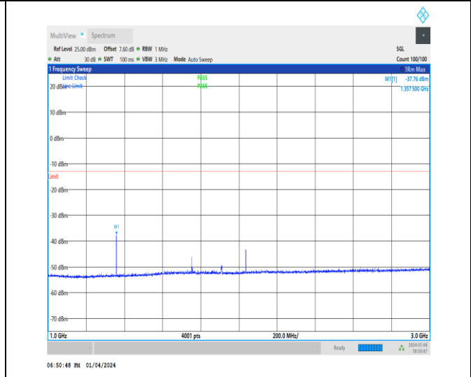
1-N71-15-20-H-1-DFT-PI2BPSK-Inner_1RB_Left-1 @ 1-1000-3000-Ant1-1357.50--37.76--13-PASS
