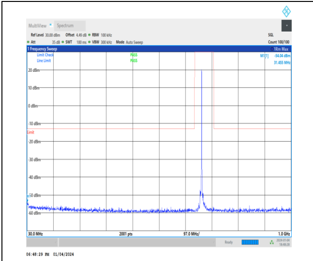
1-N71-15-20-M-1-DFT-PI2BPSK-Inner_1RB_Left-1 @ 1-30-1000-Ant1-31.46--54.04--13-PASS
