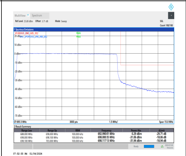
1-N71-15-10-H-6-CP-QPSK-Outer_Full-52@0-Ant1-1--PASS-see graph
