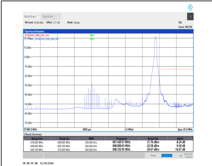
1-N71-15-20-H-2-DFT-PI2BPSK-Edge_1RB_Right-1@105-Ant1-1--PASS-see graph
