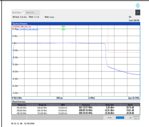
1-N71-15-15-H-6-CP-QPSK-Outer_Full-79@0-Ant1-1--PASS-see graph
