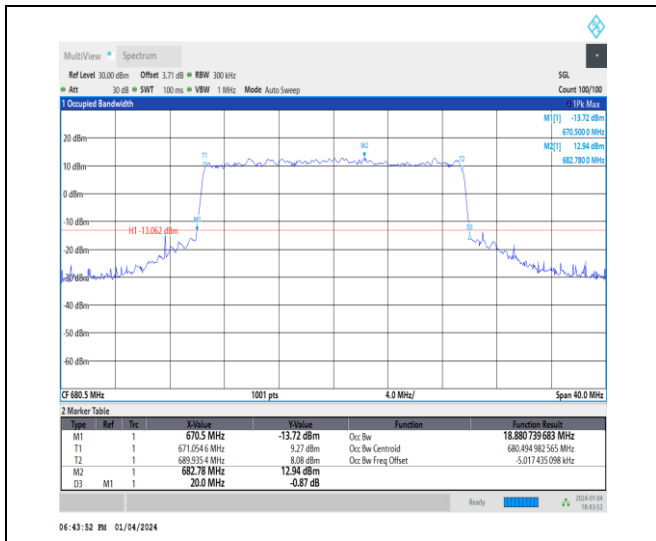
1-N71-15-20-M-6-CP-QPSK-Outer_Full-106@0-Ant 1-18.881-20.000-≤20-PASS
