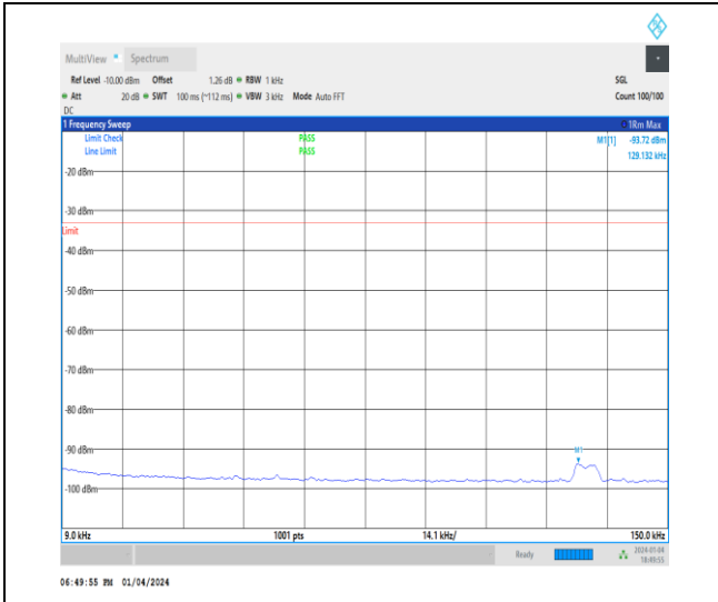
1-N71-15-20-H-1-DFT-PI2BPSK-Inner_1RB_Left-1 @ 1-0.009-0.15-Ant1-0.13--93.72--33-PASS
