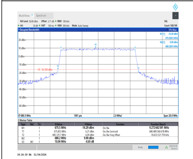
1-N71-15-10-M-6-CP-QPSK-Outer_Full-52@0-Ant1- 9.273-10.040-≤10-PASS
