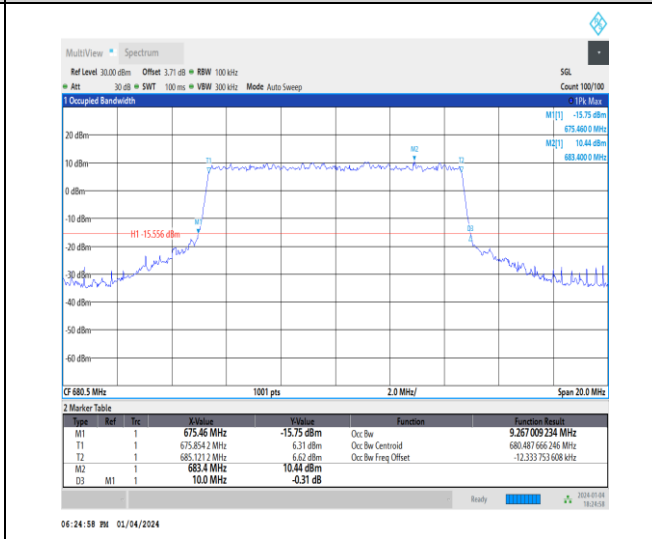
1-N71-15-10-M-7-CP-16QAM-Outer_Full-52@0-Ant1 -9.267-10.000-≤10-PASS
