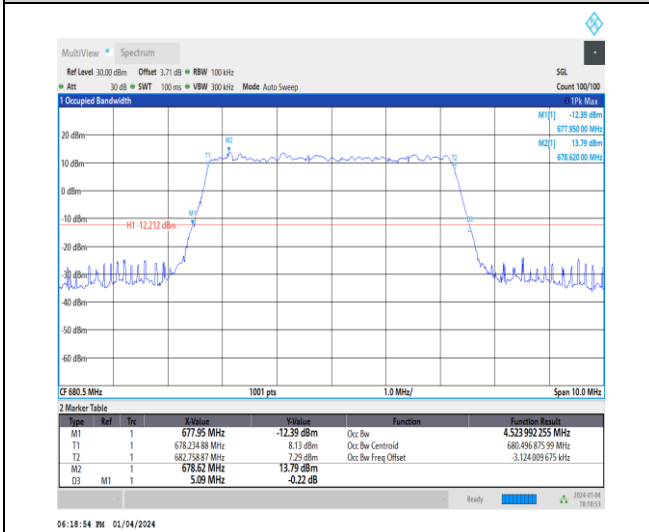
1-N71-15-5-M-7-CP-16QAM-Outer_Full-25@0-Ant1-4.524-5.090-≤5-PASS
