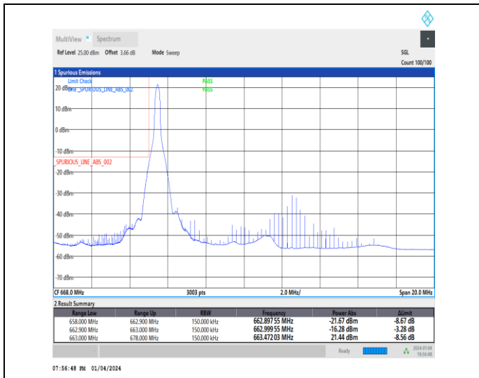
1-N71-15-15-L-1-DFT-PI2BPSK-Edge_1RB_Left-1@0-Ant1-1--PASS-see graph
