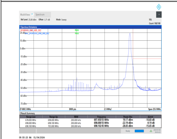
1-N71-15-20-H-5-CP-QPSK-Edge_1RB_Right-1@105-Ant1-1--PASS-see graph
