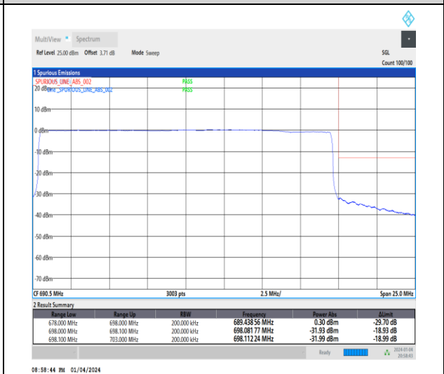
1-N71-15-20-H-6-CP-QPSK-Outer_Full-106@0-Ant1-1--PASS-see graph
