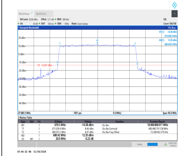
1-N71-15-20-M-8-CP-64QAM-Outer_Full-106@0-Ant t1-18.901-20.000-≤20-PASS
