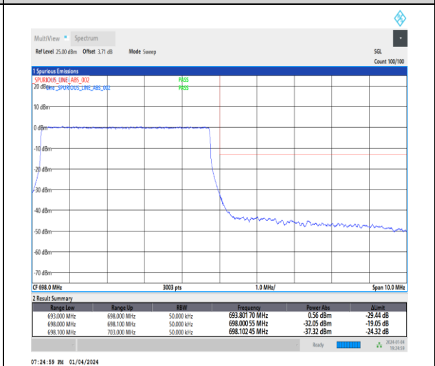
1-N71-15-5-H-6-CP-QPSK-Outer_Full-25@0-Ant1-1--PASS-see graph
