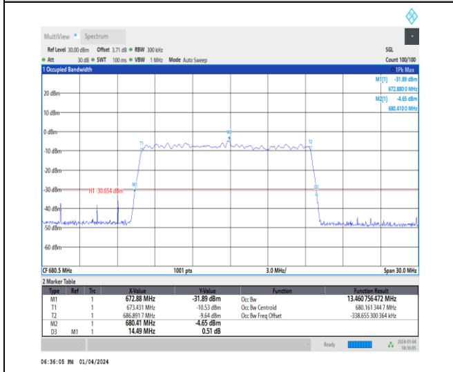
1-N71-15-15-M-5-DFT-256QAM-Outer_Full-75@0-Ant1-13.461-14.490-≤15-PASS
