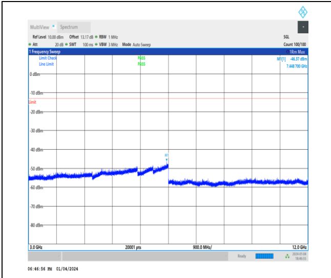
1-N71-15-20-L-1-DFT-PI2BPSK-Inner_1RB_Left-1 @ 1-3000-12000-Ant1-7448.70--46.37--13-PASS
