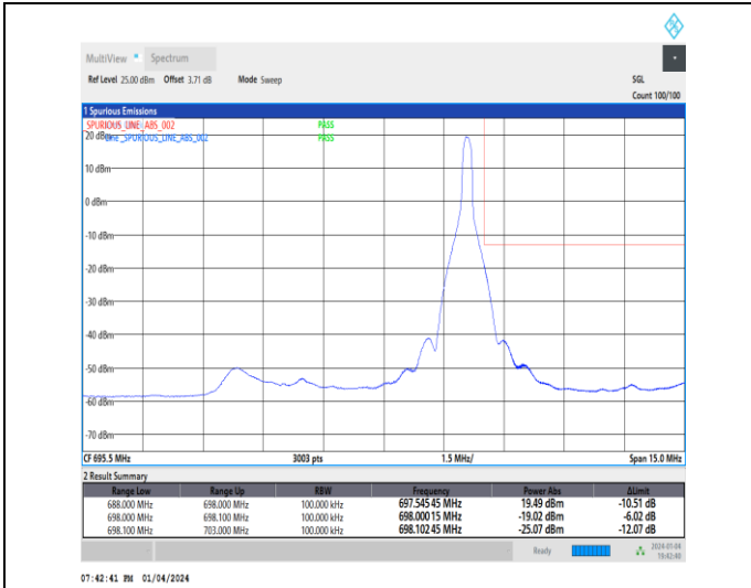
1-N71-15-10-H-2-DFT-PI2BPSK-Edge_1RB_Right-1@51-Ant1-1--PASS-see graph
