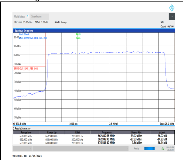
1-N71-15-20-L-3-DFT-PI2BPSK-Outer_Full-100@0-Ant1-1--PASS-see graph
