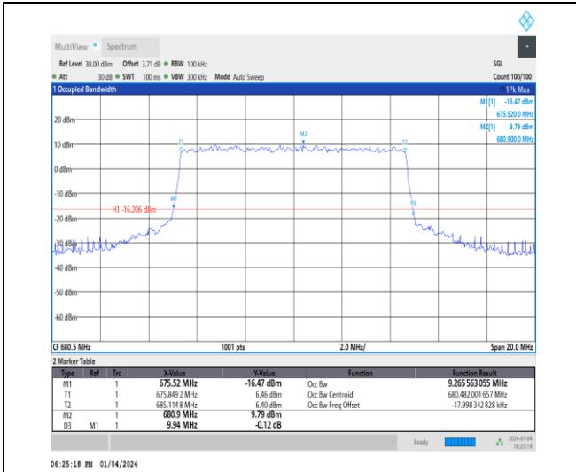
1-N71-15-10-M-8-CP-64QAM-Outer_Full-52@0-Ant 1-9.266-9.940≤10-PASS
