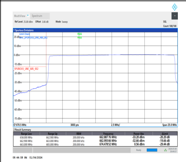
1-N71-15-20-L-6-CP-QPSK-Outer_Full-106@0-Ant1-1--PASS-see graph
