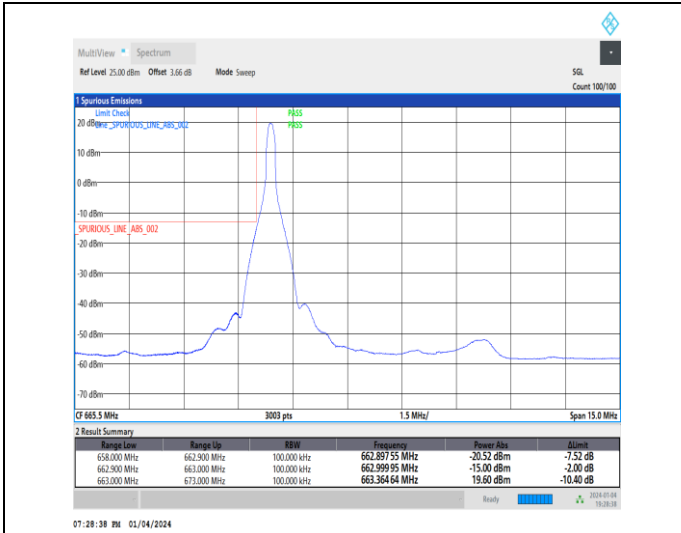
1-N71-15-10-L-1-DFT-PI2BPSK-Edge_1RB_Left-1@0-Ant1-1--PASS-see graph
