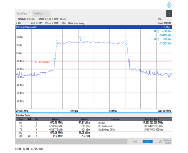
1-N71-15-20-M-1-DFT-QPSK-Outer_Full-100@0-Ant 1-17.827-19.200-≤20-PASS
