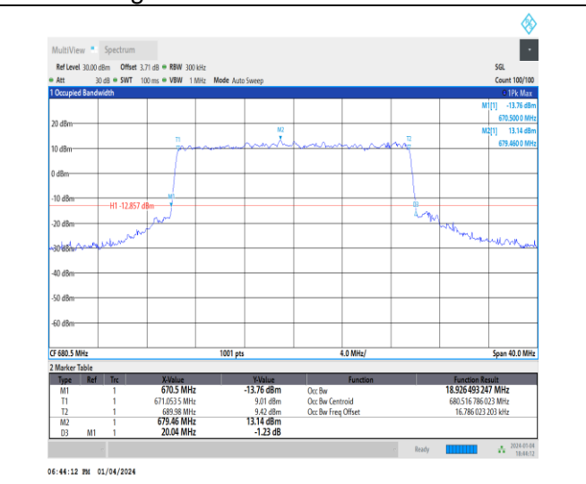
1-N71-15-20-M-7-CP-16QAM-Outer_Full-106@0-Ant 1-18.926-20.040-≤20-PASS
