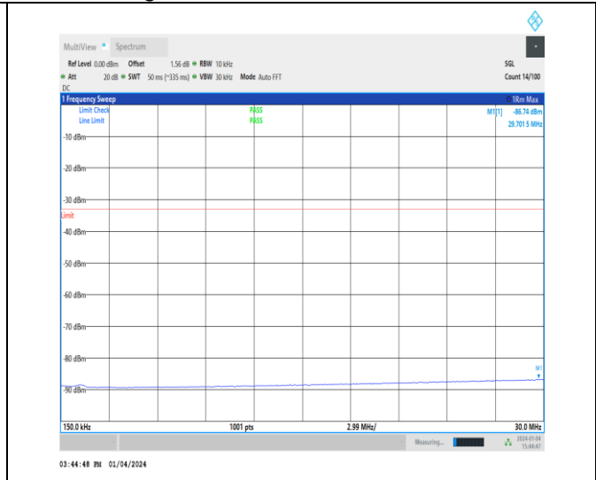
1-N66-15-40-H-1-DFT-PI2BPSK-Inner_1RB_Left-1 @ 1-0.15-30-Ant1-29.70--86.74--33-PASS
