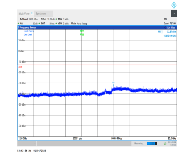
1-N66-15-40-M-1-DFT-PI2BPSK-Inner_1RB_Left-1 @ 1-12000-20000-Ant1-16813.60--32.87--13-PASS
