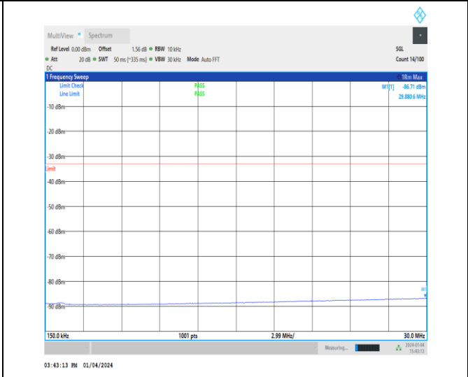
1-N66-15-40-M-1-DFT-PI2BPSK-Inner_1RB_Left-1 @ 1-0.15-30-Ant1-29.88--86.71--33-PASS
