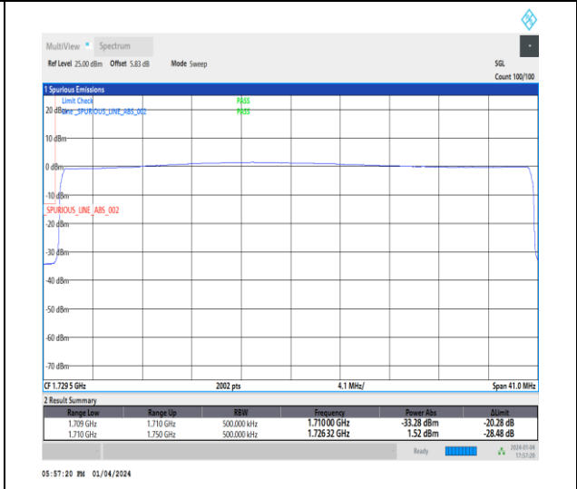
1-N66-15-40-L-6-CP-QPSK-Outer_Full-216@0-Ant1-1-seegraph-PASS-see graph
