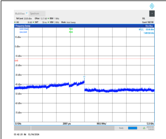
1-N66-15-40-L-1-DFT-PI2BPSK-Inner_1RB_Left-1 @ 1-3000-12000-Ant1-7499.55--35.46--13-PASS
