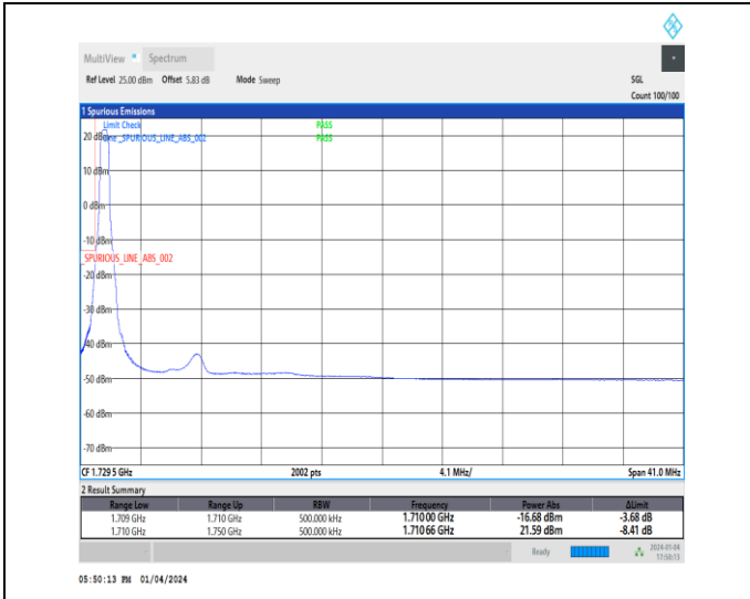
1-N66-15-40-L-1-DFT-PI2BPSK-Edge_1RB_Left-1@0-Ant1-1-seegraph-PASS-see graph
