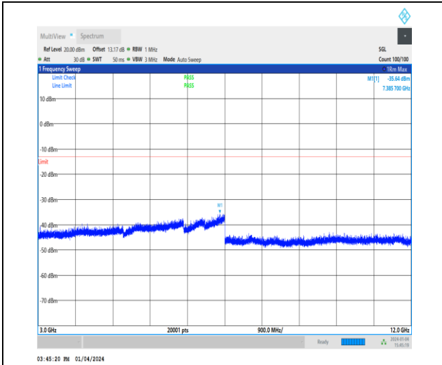
1-N66-15-40-H-1-DFT-PI2BPSK-Inner_1RB_Left-1 @ 1-3000-12000-Ant1-7385.70--35.64--13-PASS
