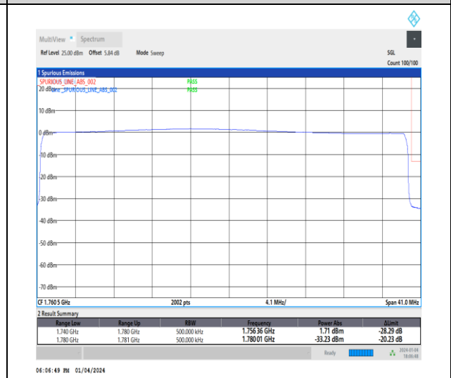
1-N66-15-40-H-6-CP-QPSK-Outer_Full-216@0-Ant1-1-seegraph-PASS-see graph
