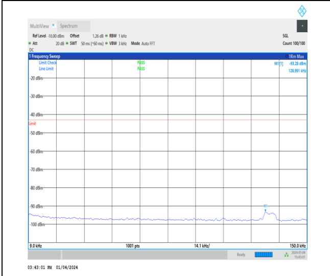
1-N66-15-40-M-1-DFT-PI2BPSK-Inner_1RB_Left-1 @ 1-0.009-0.15-Ant1-0.13--93.28--43-PASS
