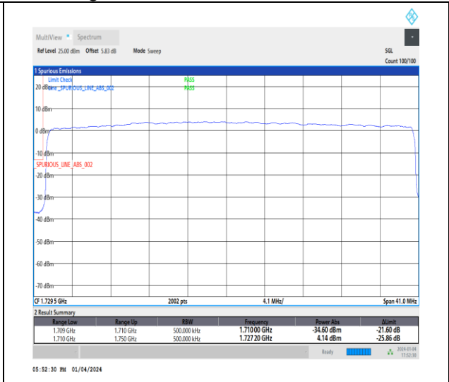
1-N66-15-40-L-3-DFT-PI2BPSK-Outer_Full-216@0-Ant1-1-seegraph-PASS-see graph
