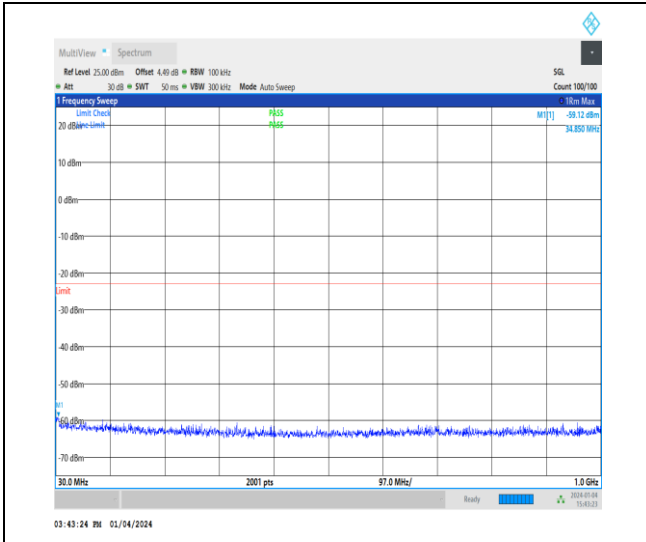
1-N66-15-40-M-1-DFT-PI2BPSK-Inner_1RB_Left-1 @ 1-30-1000-Ant1-34.85--59.12--23-PASS
