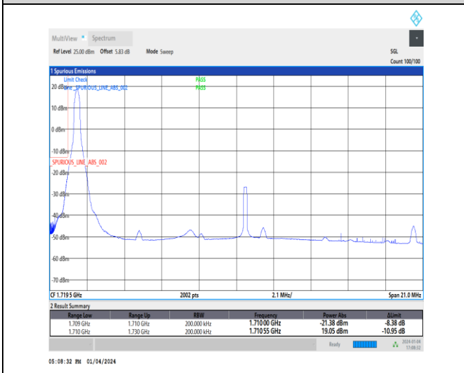
1-N66-15-20-L-4-CP-QPSK-Edge_1RB_Left-1@0-Ant1-1-seegraph-PASS-see graph
