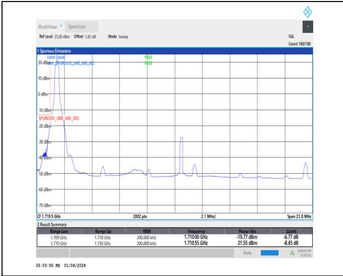
1-N66-15-20-L-1-DFT-PI2BPSK-Edge_1RB_Left-1@0-Ant1-1-seegraph-PASS-see graph
