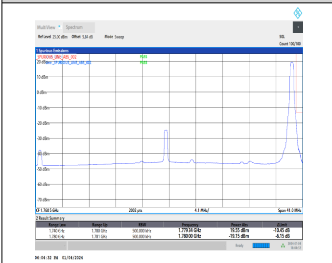
1-N66-15-40-H-5-CP-QPSK-Edge_1RB_Right-1@215-Ant1-1-seegraph-PASS-see graph
