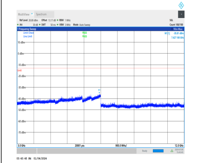
1-N66-15-40-M-1-DFT-PI2BPSK-Inner_1RB_Left-1 @ 1-3000-12000-Ant1-7427.10--35.81--13-PASS
