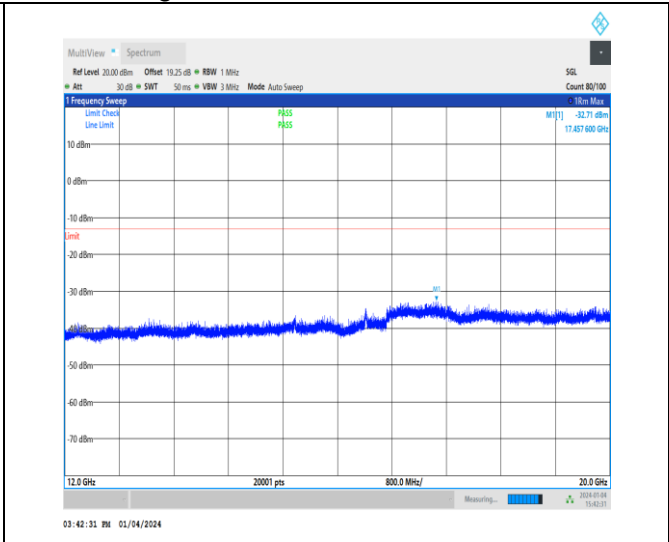
1-N66-15-40-L-1-DFT-PI2BPSK-Inner_1RB_Left-1 @ 1-12000-20000-Ant1-17457.60--32.71--13-PASS
