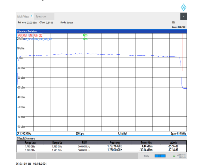
1-N66-15-40-H-3-DFT-PI2BPSK-Outer_Full-216@0-Ant1-1-seegraph-PASS-see graph
