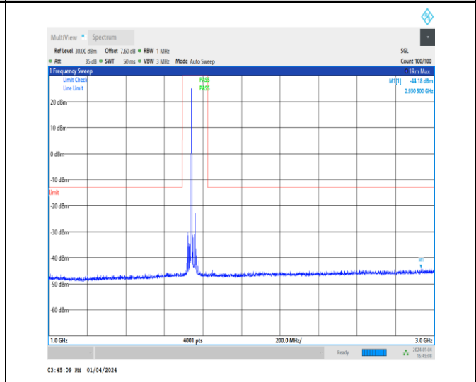
1-N66-15-40-H-1-DFT-PI2BPSK-Inner_1RB_Left-1 @ 1-1000-3000-Ant1-2930.50--44.18--13-PASS
