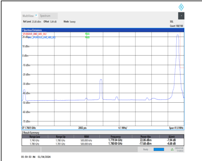
1-N66-15-40-H-2-DFT-PI2BPSK-Edge_1RB_Right-1@215-Ant1-1-seegraph-PASS-see graph
