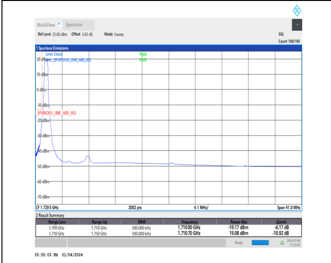
1-N66-15-40-L-4-CP-QPSK-Edge_1RB_Left-1@0-Ant1-1-seegraph-PASS-see graph
