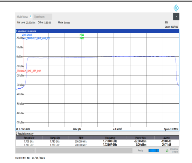
1-N66-15-20-L-6-CP-QPSK-Outer_Full-106@0-Ant1-1-seegraph-PASS-see graph
