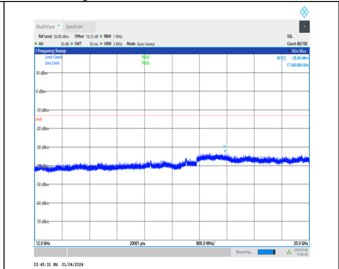
1-N66-15-40-H-1-DFT-PI2BPSK-Inner_1RB_Left-1 @ 1-12000-20000-Ant1-17540.00--33.04--13-PASS
