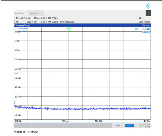
1-N66-15-40-H-1-DFT-PI2BPSK-Inner_1RB_Left-1 @ 1-30-1000-Ant1-34.37--58.94--23-PASS
