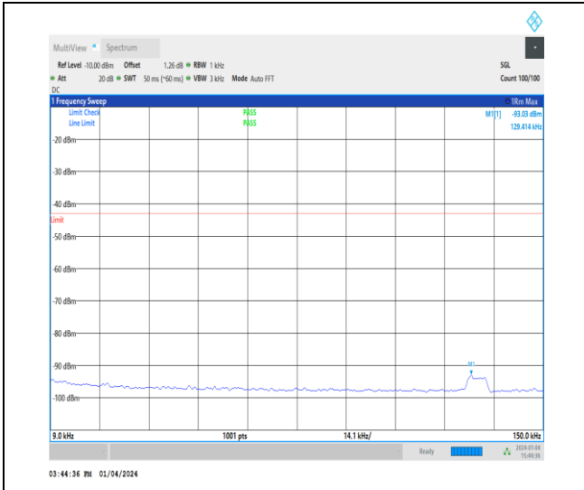
1-N66-15-40-H-1-DFT-PI2BPSK-Inner_1RB_Left-1 @ 1-0.009-0.15-Ant1-0.13--93.03--43-PASS
