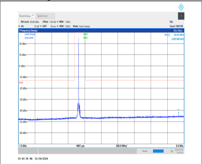
1-N66-15-40-M-1-DFT-PI2BPSK-Inner_1RB_Left-1 @ 1-1000-3000-Ant1-2933.50--42.92--13-PASS
