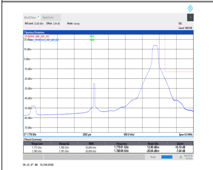
1-N66-15-5-H-5-CP-QPSK-Edge_1RB_Right-1@24-Ant1-1-seegraph-PASS-see graph
