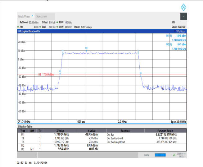
1-N66-15-10-M-5-DFT-256QAM-Outer_Full-50@0-A nt1-8.922-9.540-≤10-PASS
