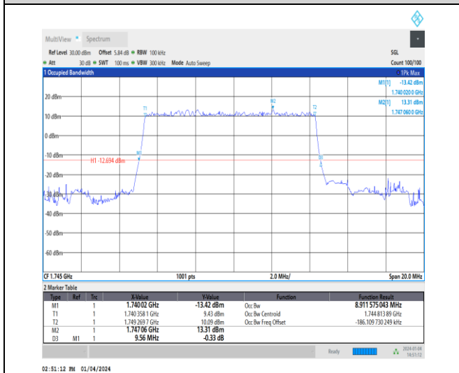
1-N66-15-10-M-2-DFT-PI2BPSK-Outer_Full-50@0-Ant1 -8.912-9.560-≤10-PASS
