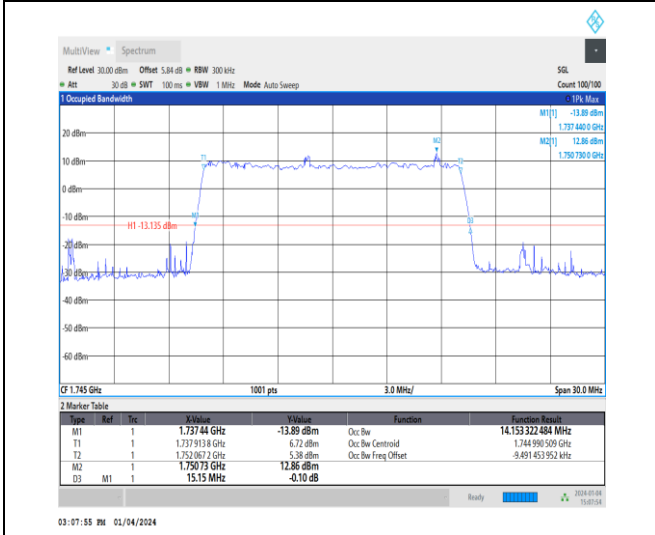
1-N66-15-15-M-9-CP-256QAM-Outer_Full-79@0-Ant 1-14.153-15.150≤15-PASS
