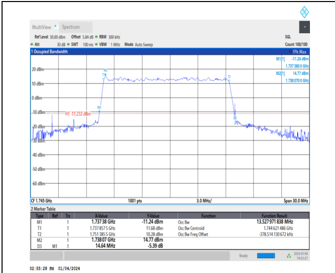
1-N66-15-15-M-3-DFT-16QAM-Outer_Full-75@0-Ant 1-13.528-14.640-≤15-PASS
