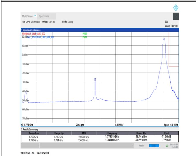
1-N66-15-15-H-5-CP-QPSK-Edge_1RB_Right-1@78-Ant1-1-seegraph-PASS-see graph
