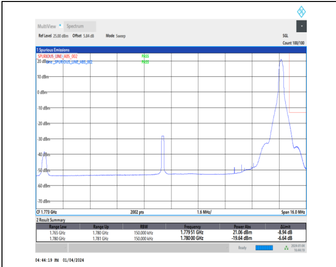
1-N66-15-15-H-2-DFT-PI2BPSK-Edge_1RB_Right-1@78-Ant1-1-seegraph-PASS-see graph
