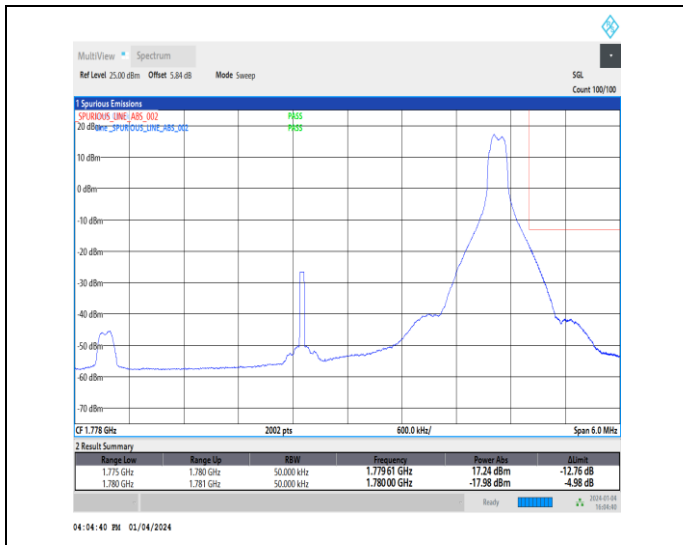
1-N66-15-5-H-2-DFT-PI2BPSK-Edge_1RB_Right-1@2-4-Ant1-1-seegraph-PASS-see graph
