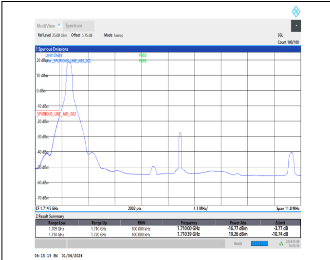
1-N66-15-10-L-1-DFT-PI2BPSK-Edge_1RB_Left-1@0-Ant1-1-seegraph-PASS-see graph
