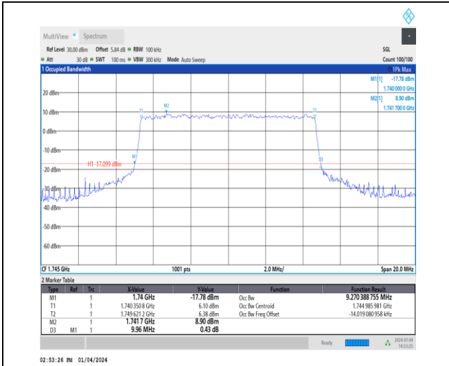
1-N66-15-10-M-8-CP-64QAM-Outer_Full-52@0-Ant1 -9.27-9.960-≤10-PASS
