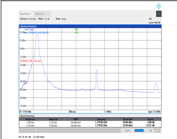
1-N66-15-10-L-4-CP-QPSK-Edge_1RB_Left-1@0-Ant1-1-seegraph-PASS-see graph
