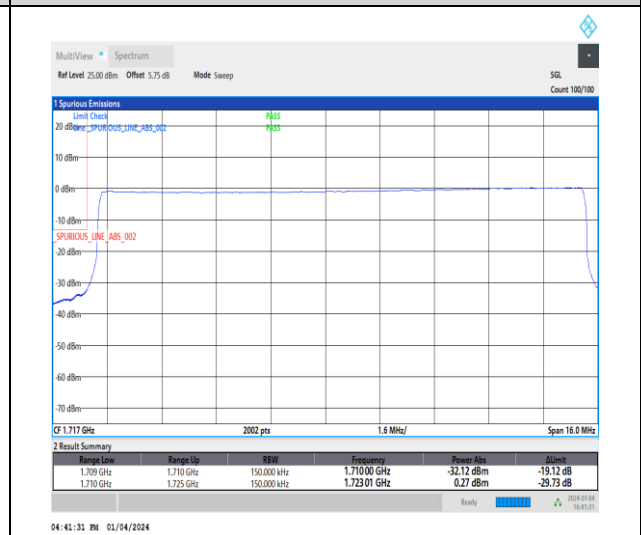
1-N66-15-15-L-6-CP-QPSK-Outer_Full-79@0-Ant1-1-seegraph-PASS-see graph
