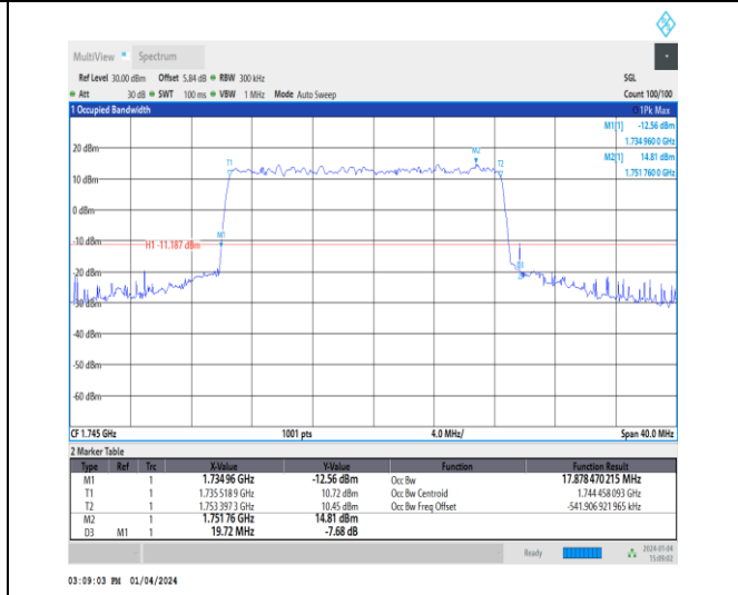
1-N66-15-20-M-1-DFT-QPSK-Outer_Full-100@0-Ant 1-17.878-19.720≤20-PASS
