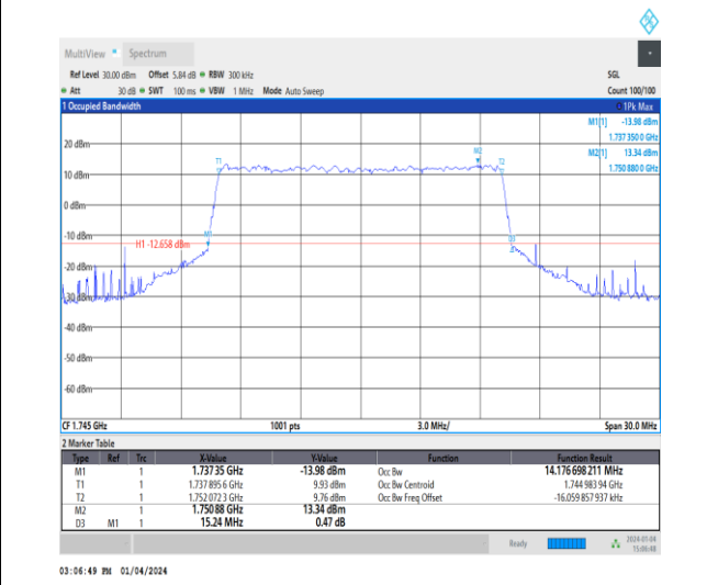
1-N66-15-15-M-6-CP-QPSK-Outer_Full-79@0-Ant1 14.177-15.240-≤15-PASS
