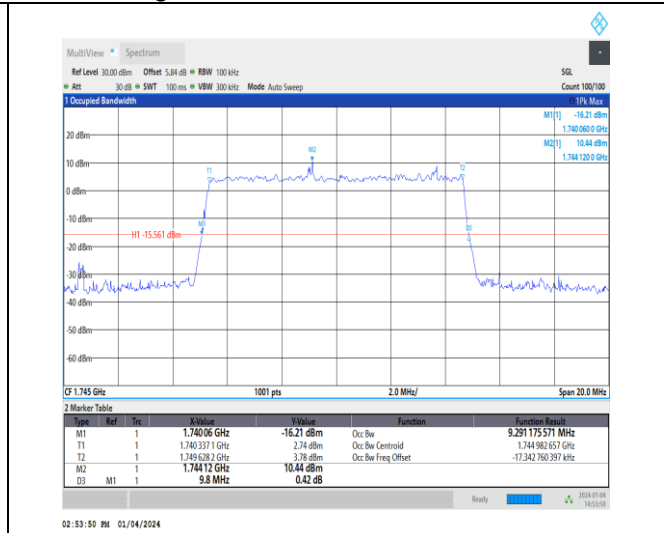
1-N66-15-10-M-9-CP-256QAM-Outer_Full-52@0-Ant 1-9.291-9.800-≤10-PASS
