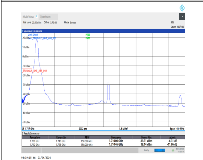
1-N66-15-15-L-4-CP-QPSK-Edge_1RB_Left-1@0-Ant1-1-seegraph-PASS-see graph
