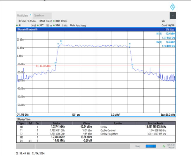
1-N66-15-15-M-4-DFT-64QAM-Outer_Full-75@0-Ant 1-13.451-14.460-≤15-PASS
