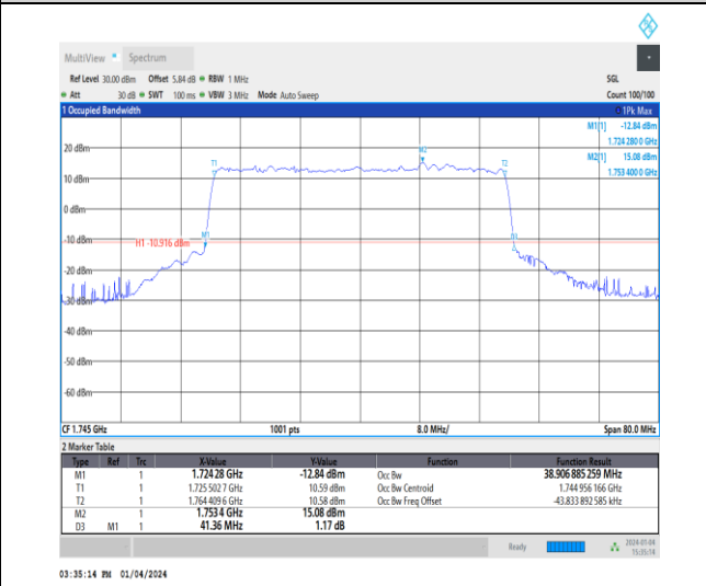
1-N66-15-40-M-8-CP-64QAM-Outer_Full-216@0-Ant1-38.907-41.360-≤40-PASS
