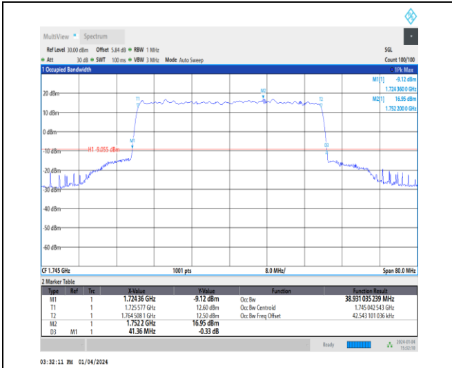
1-N66-15-40-M-1-DFT-QPSK-Outer_Full-216@0-Ant 1-38.931-41.360-≤40-PASS
