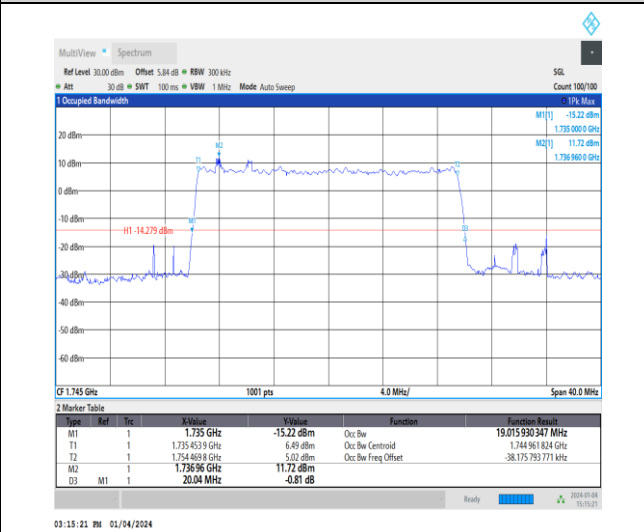
1-N66-15-20-M-9-CP-256QAM-Outer_Full-106@0-A nt1-19.016-20.040-≤20-PASS
