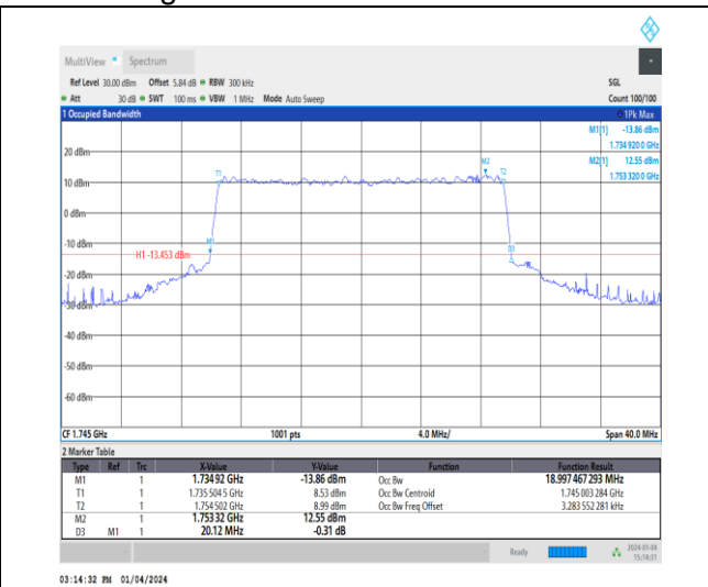
1-N66-15-20-M-7-CP-16QAM-Outer_Full-106@0-Ant 1-18.997-20.120-≤20-PASS
