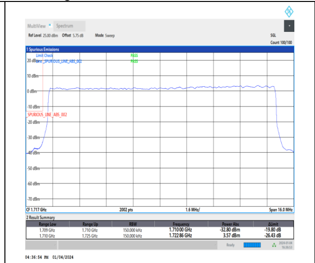
1-N66-15-15-L-3-DFT-PI2BPSK-Outer_Full-75@0-Ant1-1-seegraph-PASS-see graph
