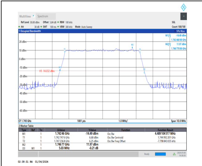
1-N66-15-5-M-5-DFT-256QAM-Outer_Full-25@0-Ant 1-4.489-5.030-≤5-PASS
