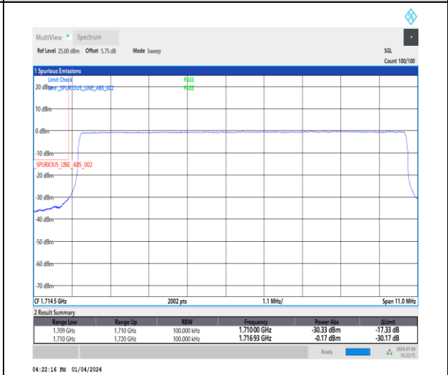
1-N66-15-10-L-6-CP-QPSK-Outer_Full-52@0-Ant1-1-seegraph-PASS-see graph
