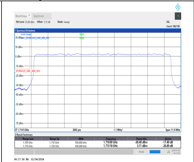
1-N66-15-10-L-3-DFT-PI2BPSK-Outer_Full-50@0-Ant1-1-seegraph-PASS-see graph
