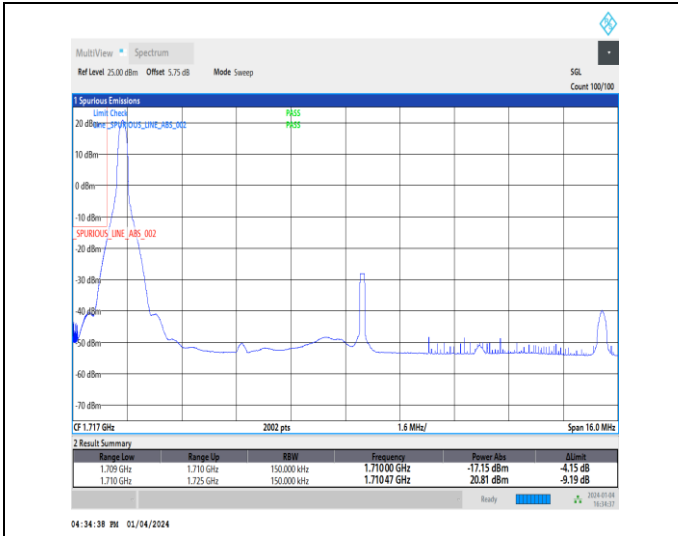
1-N66-15-15-L-1-DFT-PI2BPSK-Edge_1RB_Left-1@0-Ant1-1-seegraph-PASS-see graph
