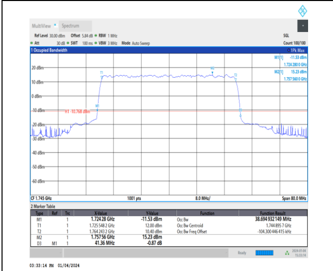
1-N66-15-40-M-3-DFT-16QAM-Outer_Full-216@0-Ant 1-38.695-41.360-≤40-PASS
