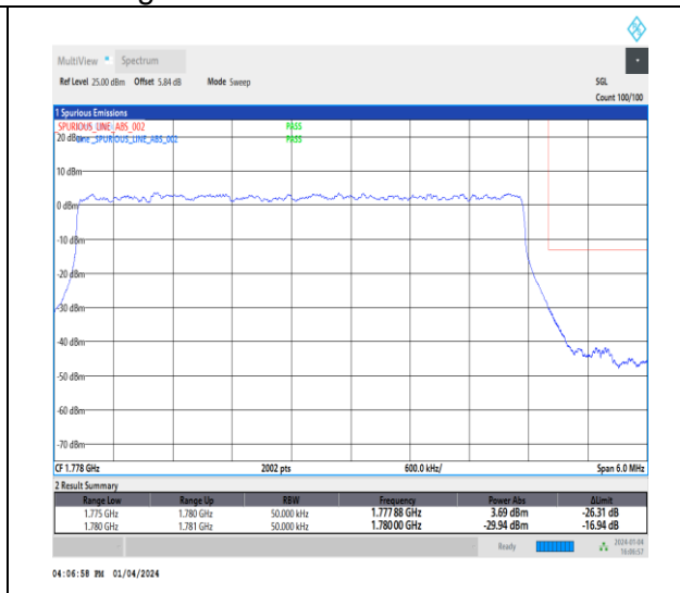
1-N66-15-5-H-3-DFT-PI2BPSK-Outer_Full-25@0-Ant1-1-seegraph-PASS-see graph
