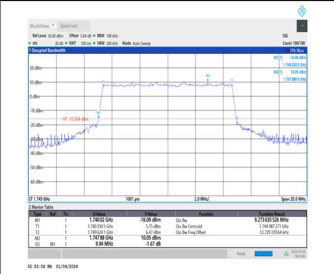
1-N66-15-10-M-7-CP-16QAM-Outer_Full-52@0-Ant1 -9.274-9.940-≤10-PASS
