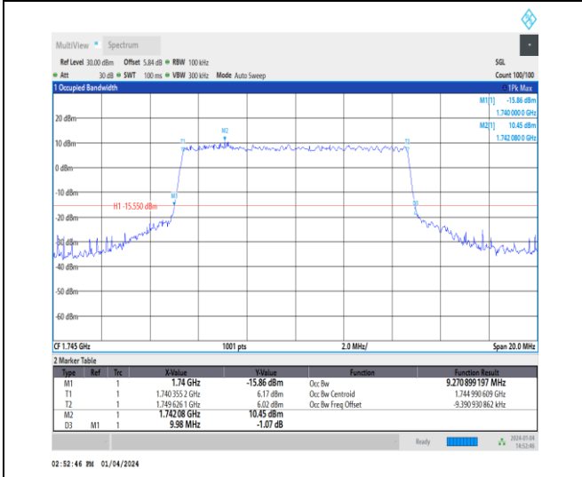
1-N66-15-10-M-6-CP-QPSK-Outer_Full-52@0-Ant1 9.271-9.980-≤10-PASS
