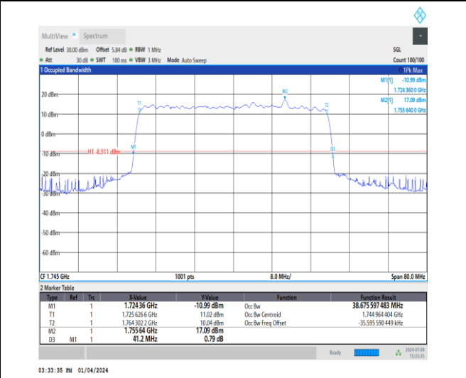
1-N66-15-40-M-4-DFT-64QAM-Outer_Full-216@0-Ant 1-38.676-41.200-≤40-PASS
