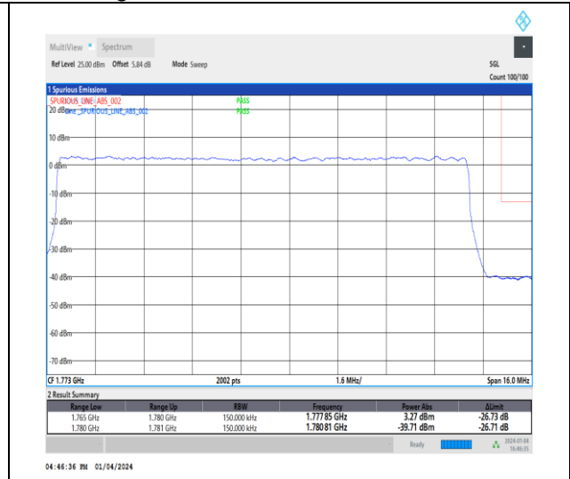
1-N66-15-15-H-3-DFT-PI2BPSK-Outer_Full-75@0-Ant1-1-seegraph-PASS-see graph
