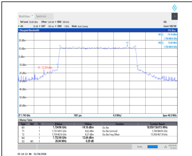
1-N66-15-20-M-6-CP-QPSK-Outer_Full-106@0-Ant1 -18.959-20.040-≤20-PASS
