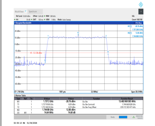
1-N66-15-15-M-5-DFT-256QAM-Outer_Full-75@0-A nt1-13.484-14.640-≤15-PASS
