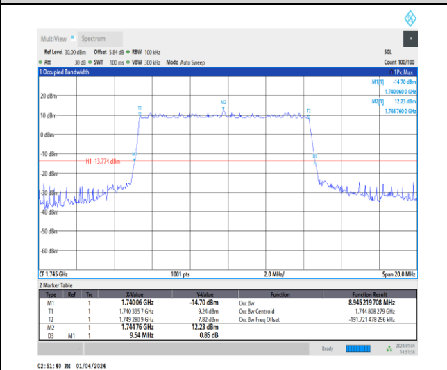
1-N66-15-10-M-3-DFT-16QAM-Outer_Full-50@0-Ant1 1-8.945-9.540-≤10-PASS
