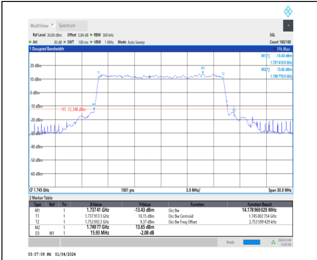
1-N66-15-15-M-7-CP-16QAM-Outer_Full-79@0-Ant1 -14.179-15.930≤15-PASS
