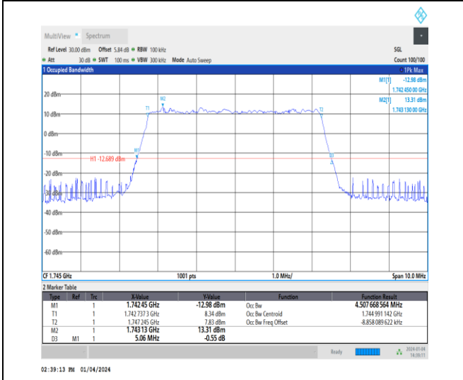
1-N66-15-5-M-7-CP-16QAM-Outer_Full-25@0-Ant1- 4.508-5.060-≤5-PASS
