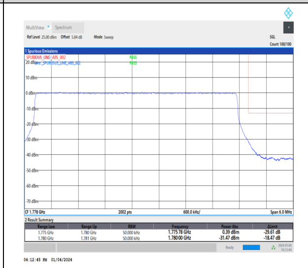
1-N66-15-5-H-6-CP-QPSK-Outer_Full-25@0-Ant1-1-seegraph-PASS-see graph
