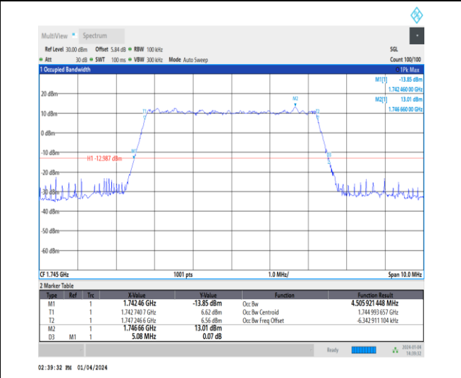
1-N66-15-5-M-8-CP-64QAM-Outer_Full-25@0-Ant1- 4.506-5.080-≤5-PASS
