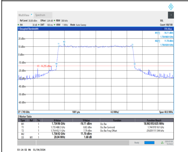
1-N66-15-20-M-8-CP-64QAM-Outer_Full-106@0-Ant 1-18.964-20.040-≤20-PASS
