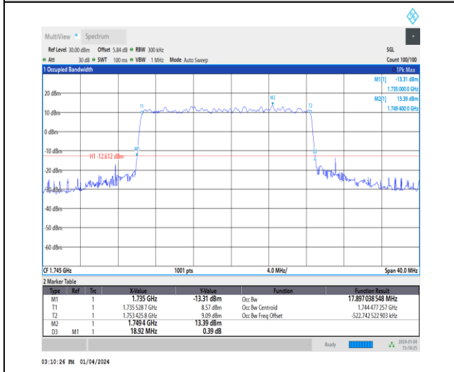
1-N66-15-20-M-4-DFT-64QAM-Outer_Full-100@0-Ant1-17.897-18.920-≤20-PASS
