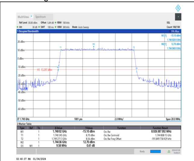
1-N66-15-10-M-1-DFT-QPSK-Outer_Full-50@0-Ant1 -8.926-9.580-≤10-PASS
