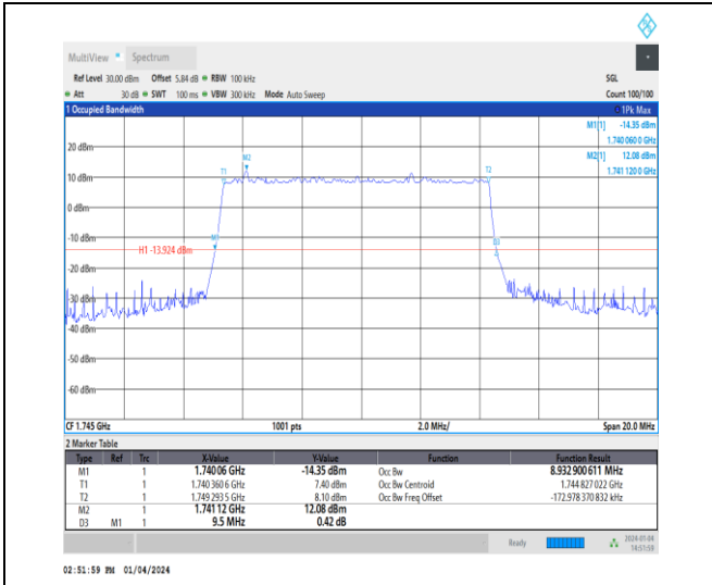
1-N66-15-10-M-4-DFT-64QAM-Outer_Full-50@0-Ant 1-8.933-9.500-≤10-PASS
