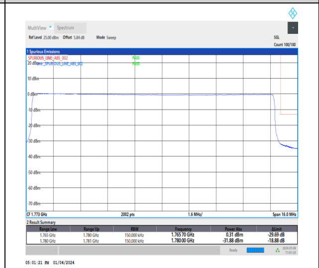
1-N66-15-15-H-6-CP-QPSK-Outer_Full-79@0-Ant1-1-seegraph-PASS-see graph
