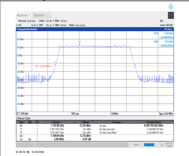
1-N66-15-5-M-6-CP-QPSK-Outer_Full-25@0-Ant1-4. 506-5.060-≤5-PASS
