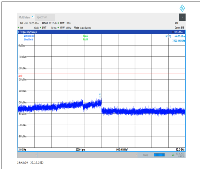
1-N41-30-100-H-1-DFT-PI2BPSK-Inner_1RB_Left-1 @ 1-3000-12000-Ant1-7376.25--46.50--25-PASS
