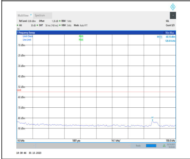
1-N41-30-100-M-1-DFT-PI2BPSK-Inner_1RB_Left-1 @ 1-0.009-0.15-Ant1-0.13--83.10--55-PASS
