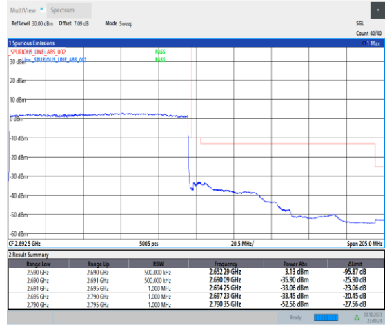
1-N41-30-100-H-3-DFT-PI2BPSK-Outer_Full-270 @0-Ant1-1--PASS-see graph
