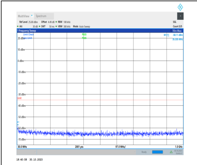
1-N41-30-100-M-1-DFT-PI2BPSK-Inner_1RB_Left-1 @ 1-30-1000-Ant1-79.47--58.11--35-PASS
