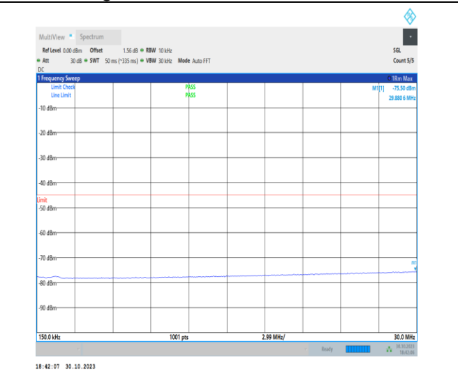
1-N41-30-100-H-1-DFT-PI2BPSK-Inner_1RB_Left-1 @ 1-0.15-30-Ant1-29.07--75.50--45-PASS
