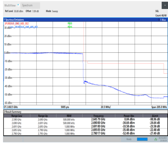
1-N41-30-100-H-6-CP-QPSK-Outer_Full-273 @0-Ant1-1--PASS-see graph
