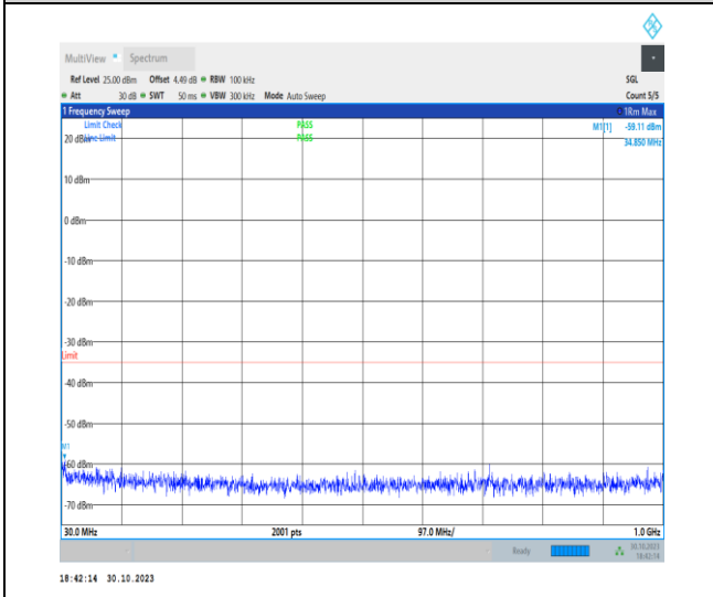
1-N41-30-100-H-1-DFT-PI2BPSK-Inner_1RB_Left-1 @ 1-30-1000-Ant1-32.91--59.11--35-PASS
