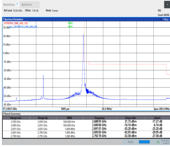
1-N41-30-100-H-2-DFT-PI2BPSK-Edge_1RB_Right-1 @272-Ant1-1--PASS-see graph
