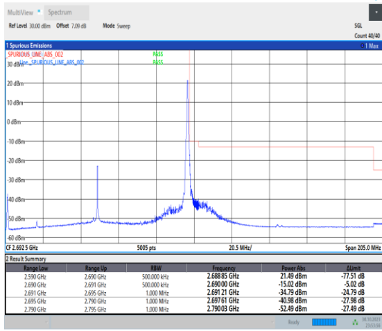
1-N41-30-100-H-5-CP-QPSK-Edge_1RB_Right-1 @272 -Ant1-1--PASS-see graph
