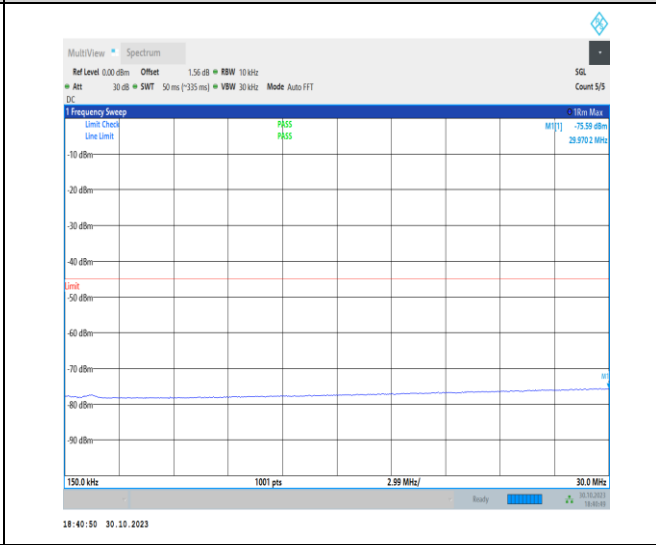
1-N41-30-100-M-1-DFT-PI2BPSK-Inner_1RB_Left-1 @ 1-0.15-30-Ant1-29.97--75.59--45-PASS
