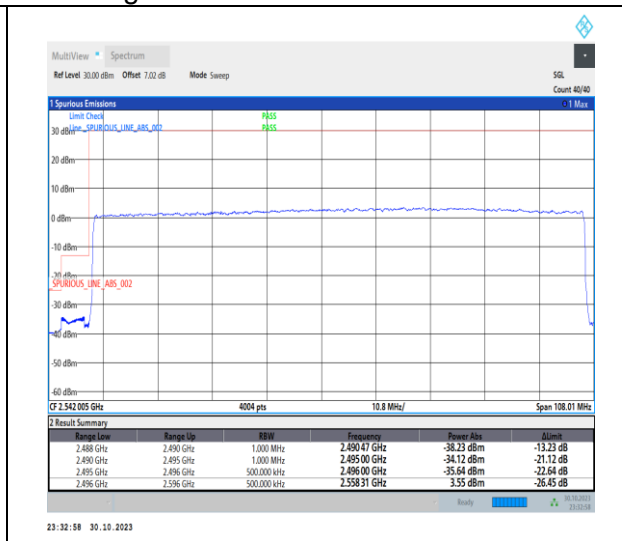
1-N41-30-100-L-3-DFT-PI2BPSK-Outer_Full-270@0-Ant1-1--PASS-see graph
