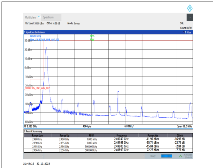
1-N41-30-60-L-1-DFT-PI2BPSK-Edge_1RB_Left-1@0-Ant1-1--PASS-see graph
