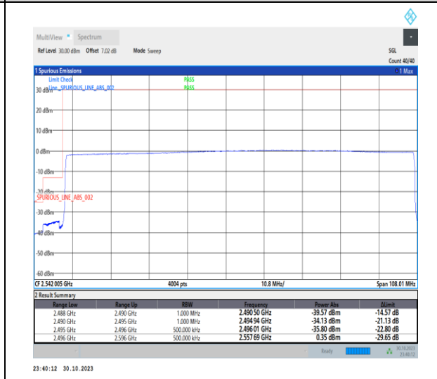
1-N41-30-100-L-6-CP-QPSK-Outer_Full-273@0-Ant1-1--PASS-see graph
