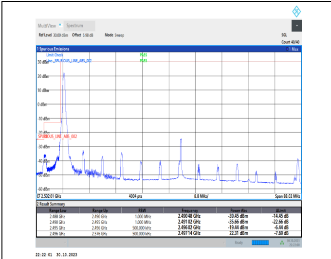
1-N41-30-80-L-1-DFT-PI2BPSK-Edge_1RB_Left-1@0-Ant1-1--PASS-see graph
