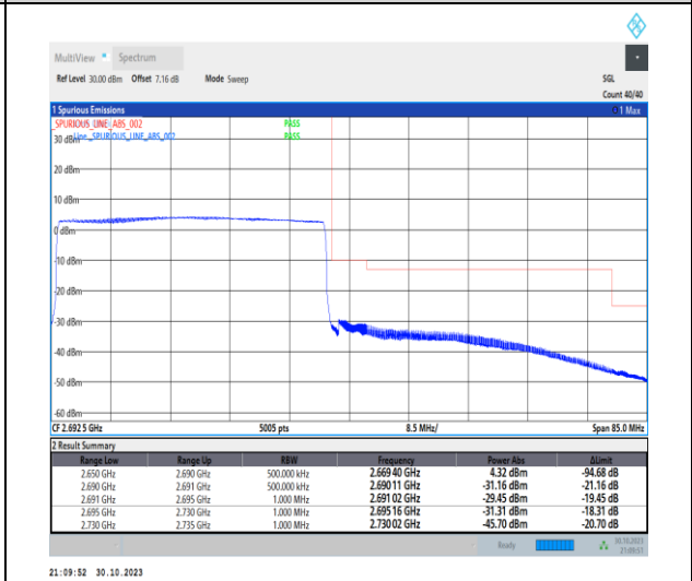
1-N41-30-40-H-6-CP-QPSK-Outer_Full-106 @ 0-Ant1-1--PASS-see graph
