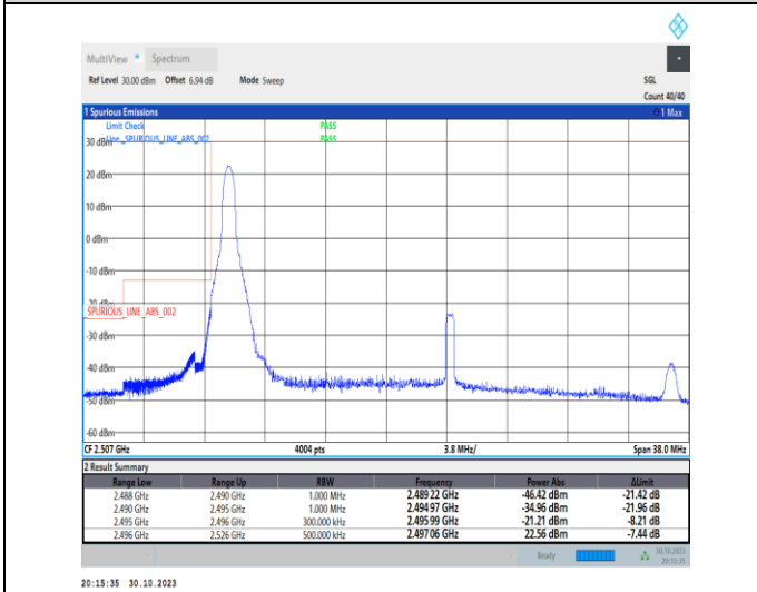
1-N41-30-30-L-4-CP-QPSK-Edge_1RB_Left-1@0-Ant1-1--PASS-see graph
