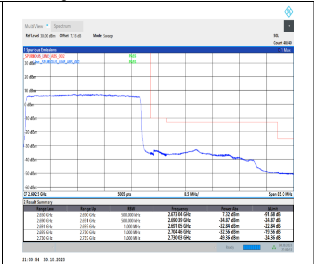
1-N41-30-40-H-3-DFT-PI2BPSK-Outer_Full-100 @ 0-Ant1-1--PASS-see graph
