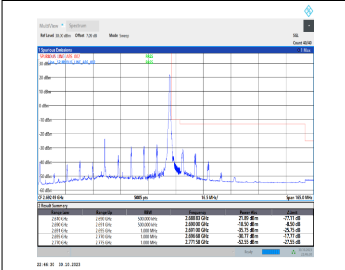
1-N41-30-80-H-5-CP-QPSK-Edge_1RB_Right-1@216-Ant1-1--PASS-see graph
