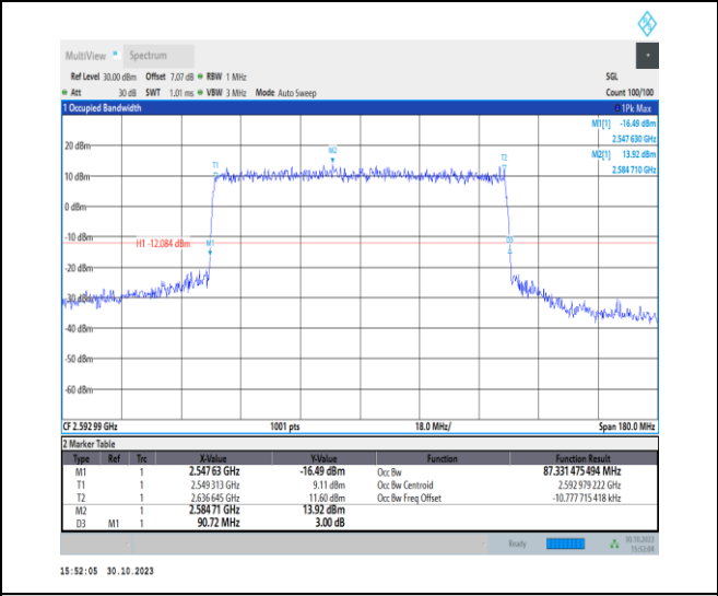
1-N41-30-90-M-6-CP-QPSK-Outer_Full-245@0-Ant1 -87.331-90.720-≤90-PASS
