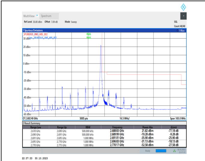
1-N41-30-80-H-2-DFT-PI2BPSK-Edge_1RB_Right-1@216-Ant1-1--PASS-see graph
