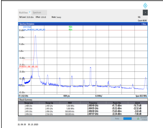
1-N41-30-60-L-4-CP-QPSK-Edge_1RB_Left-1@0-Ant1-1--PASS-see graph
