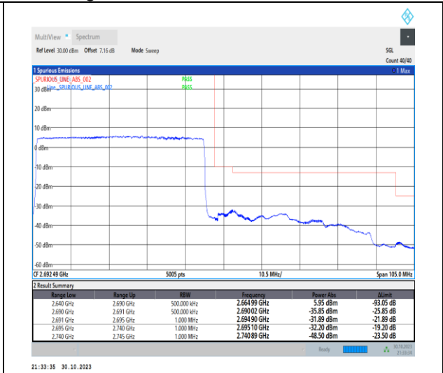
1-N41-30-50-H-3-DFT-PI2BPSK-Outer_Full-128@0-Ant1-1--PASS-see graph
