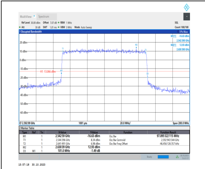
1-N41-30-100-M-6-CP-QPSK-Outer_Full-273@0-Ant 1-97.096-101.000≤100-PASS
