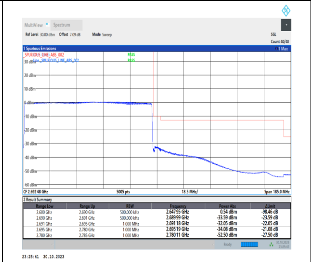
1-N41-30-90-H-6-CP-QPSK-Outer_Full-245@0-Ant1-1--PASS-see graph
