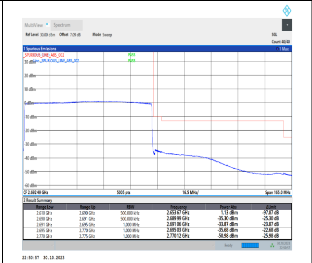
1-N41-30-80-H-6-CP-QPSK-Outer_Full-217@0-Ant1-1--PASS-see graph
