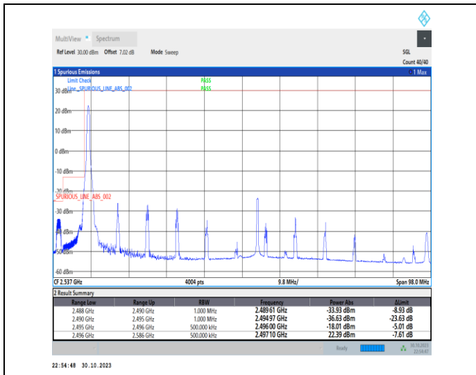
1-N41-30-90-L-1-DFT-PI2BPSK-Edge_1RB_Left-1@0-Ant1-1--PASS-see graph
