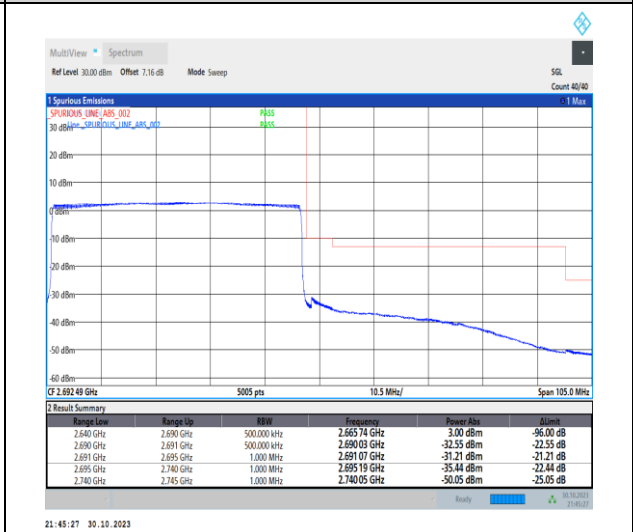
1-N41-30-50-H-6-CP-QPSK-Outer_Full-133@0-Ant1-1--PASS-see graph
