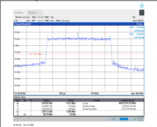
1-N41-30-90-M-8-CP-64QAM-Outer_Full-245@0-An t1-86.873-90.720-≤90-PASS
