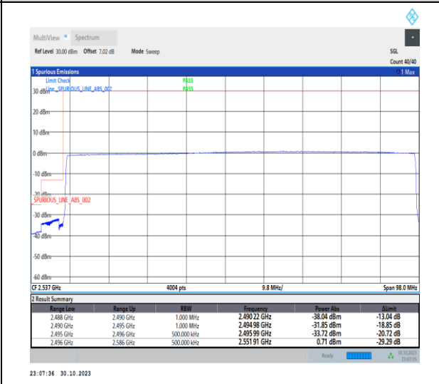
1-N41-30-90-L-6-CP-QPSK-Outer_Full-245@0-Ant1-1--PASS-see graph
