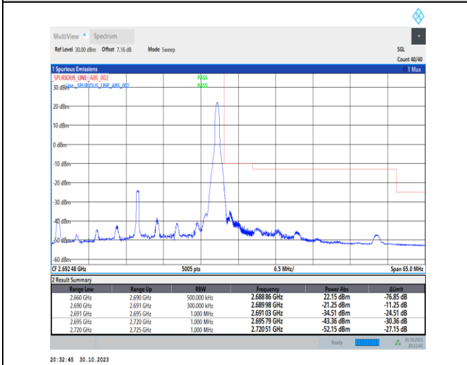
1-N41-30-30-H-5-CP-QPSK-Edge_1RB_Right-1@77-Ant1-1--PASS-see graph
