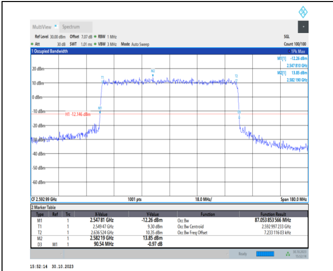
1-N41-30-90-M-7-CP-16QAM-Outer_Full-245@0-Ant 1-87.054-90.540-≤90-PASS
