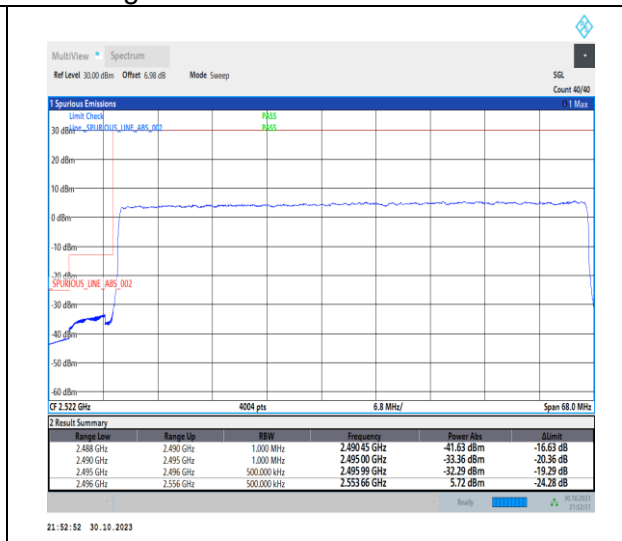
1-N41-30-60-L-3-DFT-PI2BPSK-Outer_Full-162@0-Ant1-1--PASS-see graph
