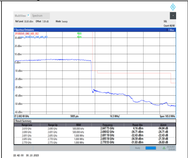
1-N41-30-80-H-3-DFT-PI2BPSK-Outer_Full-216@0-Ant1-1--PASS-see graph
