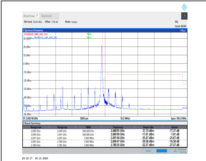
1-N41-30-90-H-2-DFT-PI2BPSK-Edge_1RB_Right-1@244-Ant1-1--PASS-see graph
