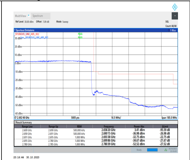
1-N41-30-90-H-3-DFT-PI2BPSK-Outer_Full-240@0-Ant1-1--PASS-see graph
