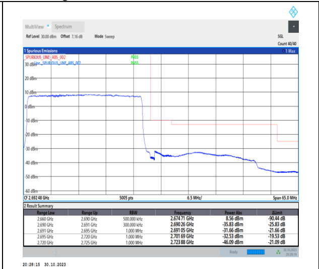
1-N41-30-30-H-3-DFT-PI2BPSK-Outer_Full-75@0-Ant1-1--PASS-see graph
