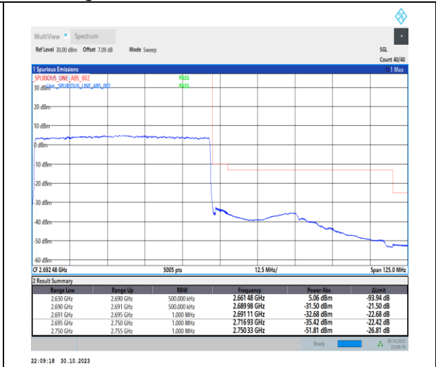
1-N41-30-60-H-3-DFT-PI2BPSK-Outer_Full-162 @ 0-Ant1-1--PASS-see graph
