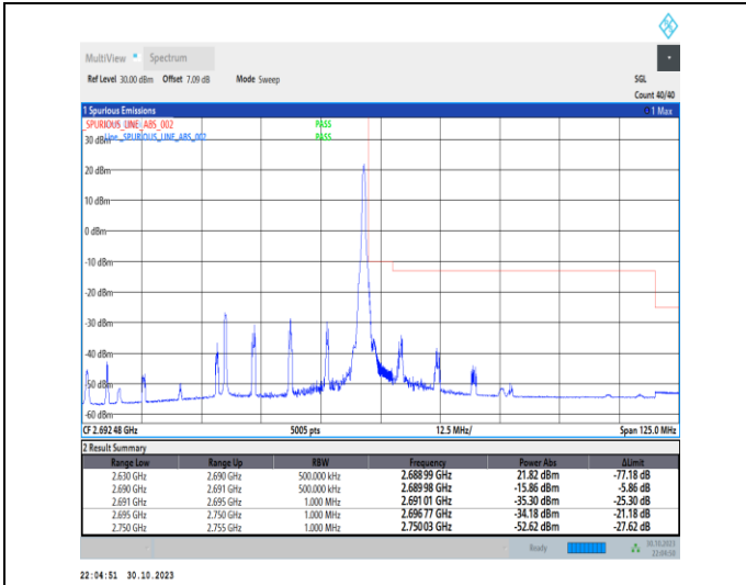
1-N41-30-60-H-2-DFT-PI2BPSK-Edge_1RB_Right-1 @ 161-Ant1-1--PASS-see graph
