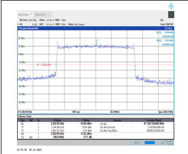
1-N41-30-100-M-8-CP-64QAM-Outer_Full-273@0-A nt1-97.167-100.800≤100-PASS
