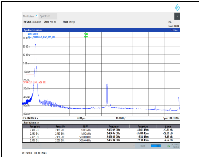
1-N41-30-100-L-1-DFT-PI2BPSK-Edge_1RB_Left-1@0-Ant1-1--PASS-see graph
