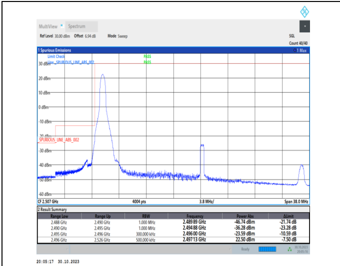
1-N41-30-30-L-1-DFT-PI2BPSK-Edge_1RB_Left-1@0-Ant1-1--PASS-see graph
