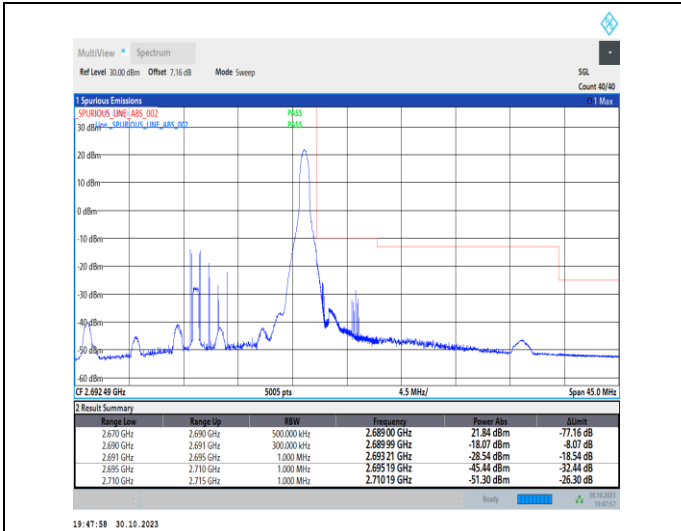
1-N41-30-20-H-2-DFT-PI2BPSK-Edge_1RB_Right-1@50-Ant1-1--PASS-see graph
