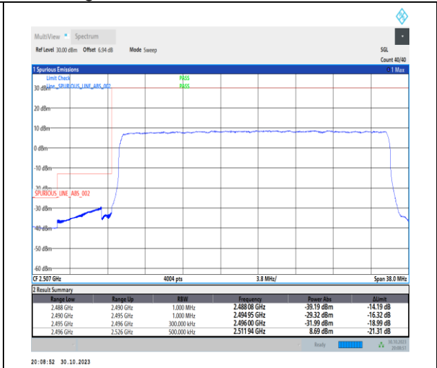
1-N41-30-30-L-3-DFT-PI2BPSK-Outer_Full-75@0-Ant1-1--PASS-see graph
