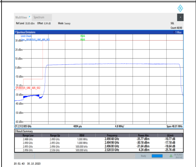
1-N41-30-40-L-6-CP-QPSK-Outer_Full-106@0-Ant1-1--PASS-see graph
