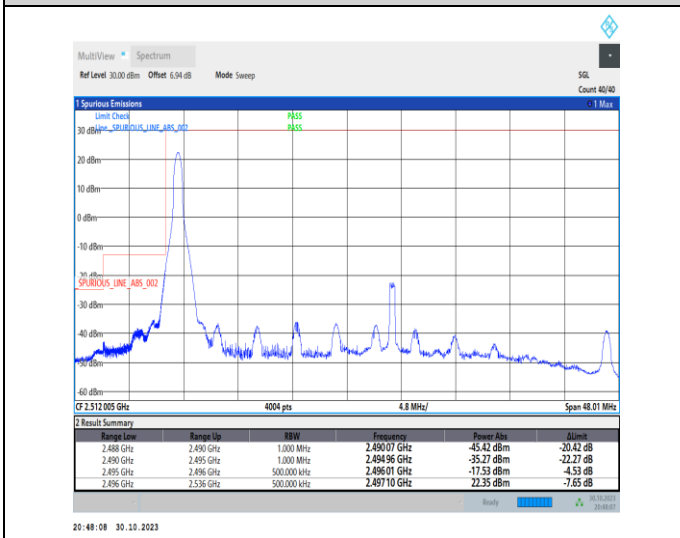
1-N41-30-40-L-4-CP-QPSK-Edge_1RB_Left-1@0-Ant1-1--PASS-see graph
