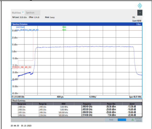
1-N41-30-40-L-3-DFT-PI2BPSK-Outer_Full-100@0-Ant1-1--PASS-see graph
