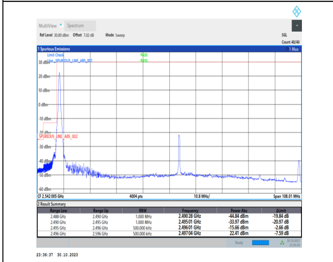
1-N41-30-100-L-4-CP-QPSK-Edge_1RB_Left-1@0-Ant1-1--PASS-see graph
