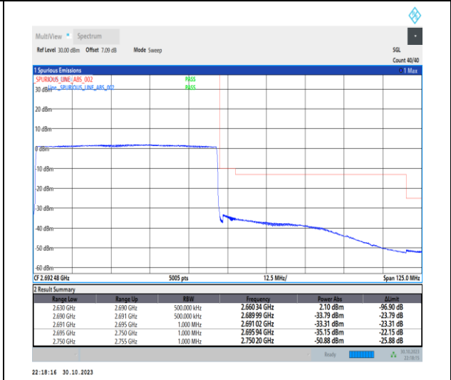
1-N41-30-60-H-6-CP-QPSK-Outer_Full-162 @ 0-Ant1-1--PASS-see graph
