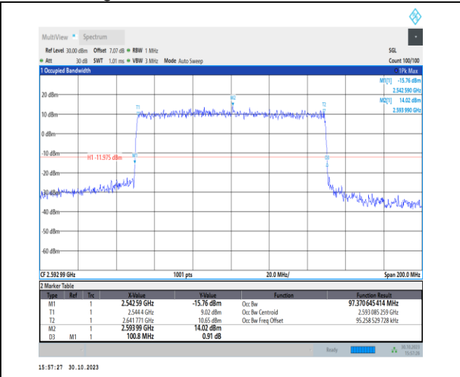
1-N41-30-100-M-7-CP-16QAM-Outer_Full-273@0-A nt1-97.371-100.800≤100-PASS
