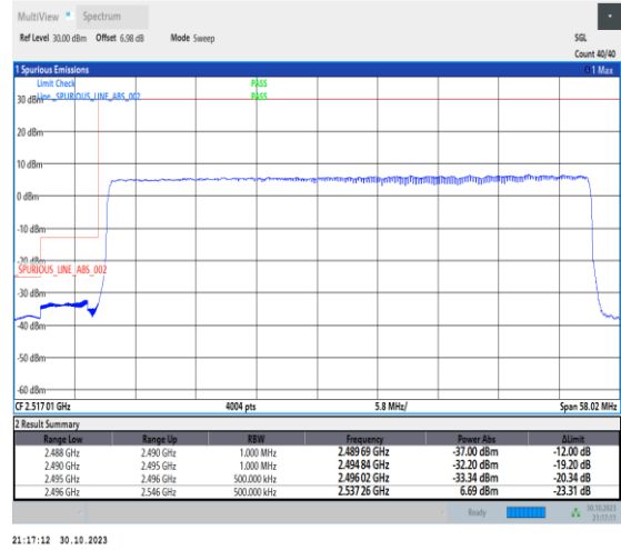
1-N41-30-50-L-3-DFT-PI2BPSK-Outer_Full-128@0-Ant1-1--PASS-see graph
