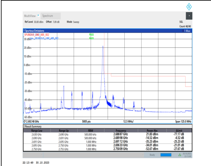
1-N41-30-60-H-5-CP-QPSK-Edge_1RB_Right-1 @ 161-Ant1-1--PASS-see graph
