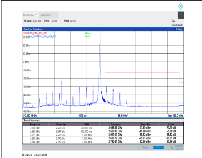
1-N41-30-90-H-5-CP-QPSK-Edge_1RB_Right-1@244-Ant1-1--PASS-see graph
