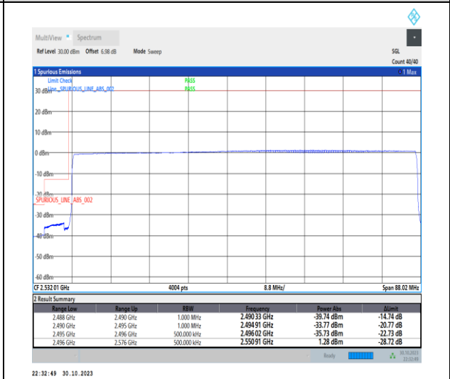
1-N41-30-80-L-6-CP-QPSK-Outer_Full-217@0-Ant1-1--PASS-see graph
