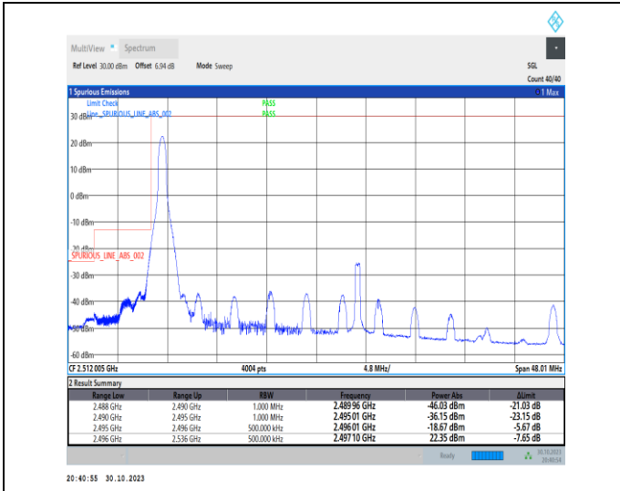
1-N41-30-40-L-1-DFT-PI2BPSK-Edge_1RB_Left-1@0-Ant1-1--PASS-see graph
