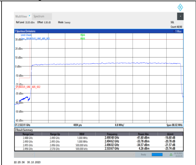
1-N41-30-80-L-3-DFT-PI2BPSK-Outer_Full-216@0-Ant1-1--PASS-see graph
