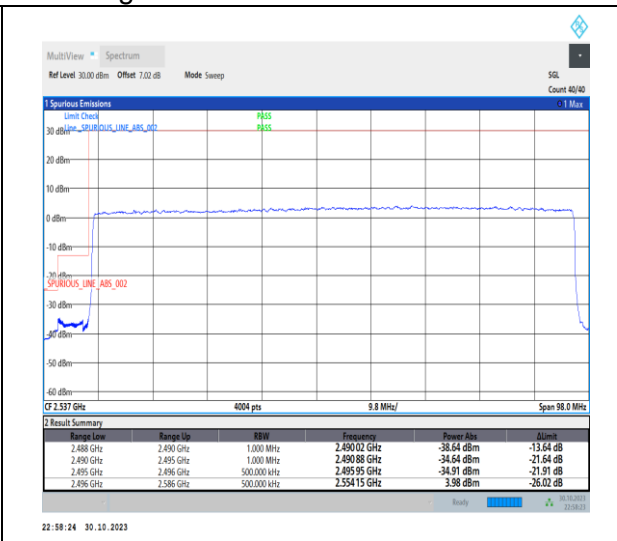
1-N41-30-90-L-3-DFT-PI2BPSK-Outer_Full-240@0-Ant1-1--PASS-see graph
