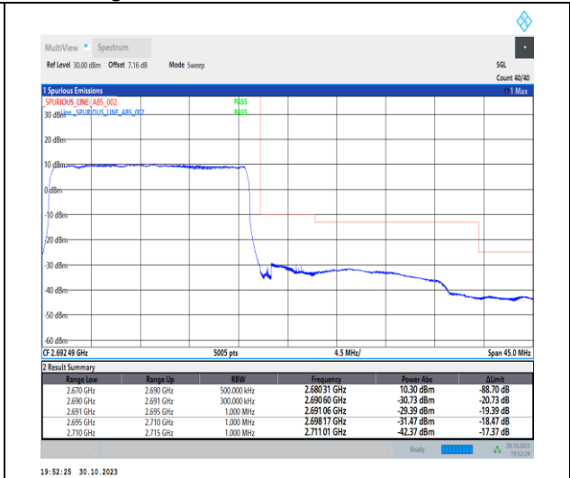
1-N41-30-20-H-3-DFT-PI2BPSK-Outer_Full-50@0-Ant1-1--PASS-see graph
