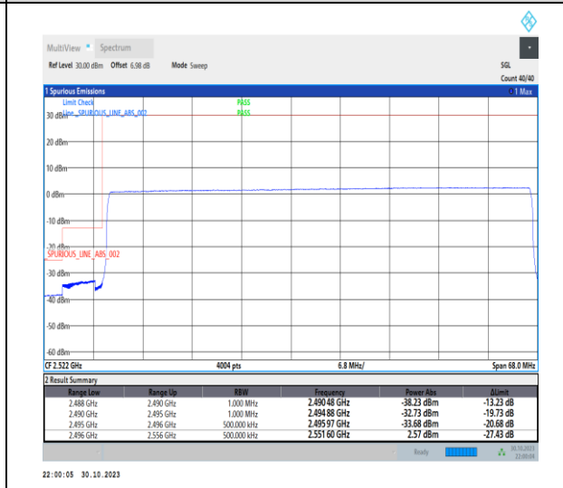
1-N41-30-60-L-6-CP-QPSK-Outer_Full-162@0-Ant1-1--PASS-see graph
