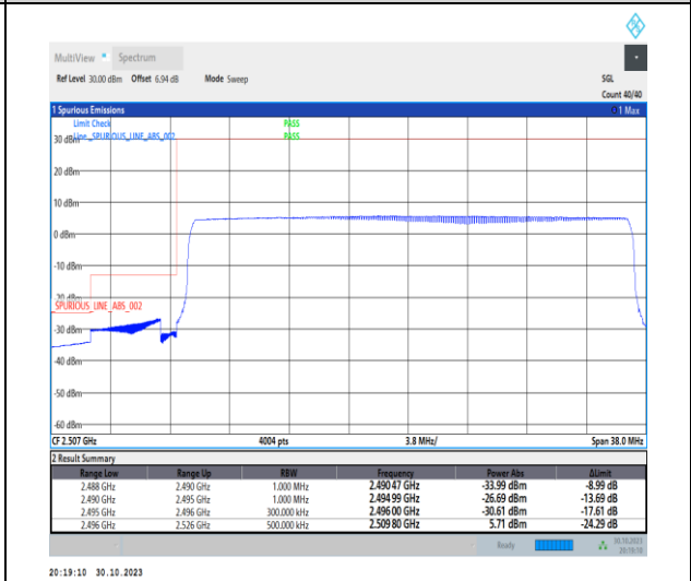
1-N41-30-30-L-6-CP-QPSK-Outer_Full-78@0-Ant1-1--PASS-see graph
