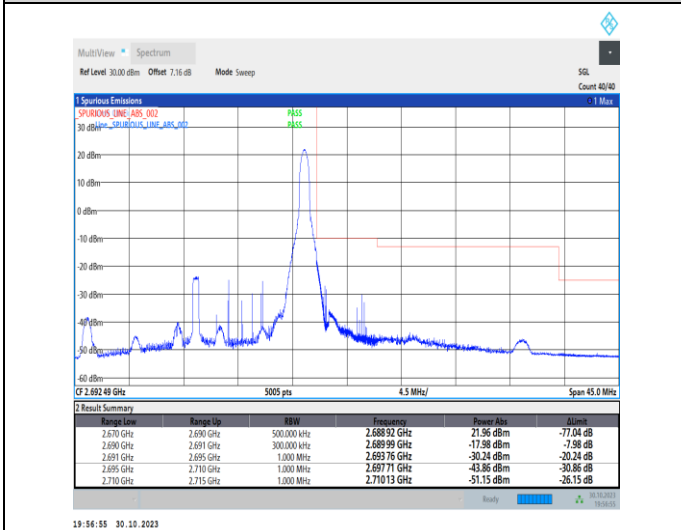
1-N41-30-20-H-5-CP-QPSK-Edge_1RB_Right-1@50-Ant1-1--PASS-see graph
