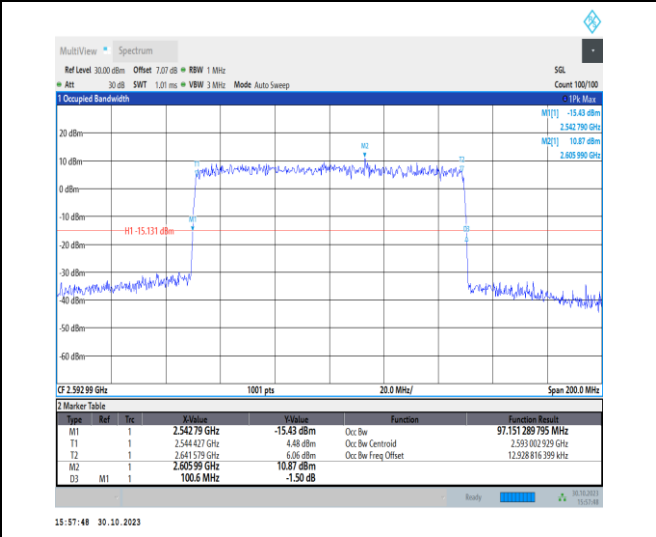
1-N41-30-100-M-9-CP-256QAM-Outer_Full-273@0-A Ant1-97.151-100.600≤100-PASS
