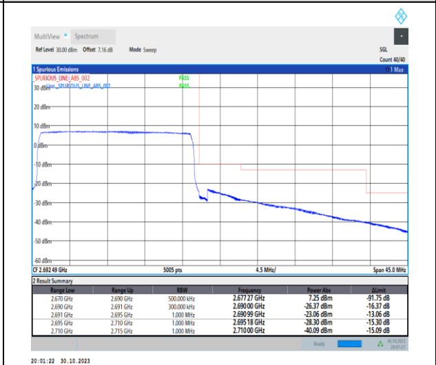
1-N41-30-20-H-6-CP-QPSK-Outer_Full-51@0-Ant1-1--PASS-see graph
