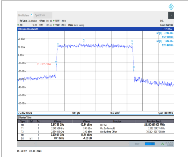
1-N41-30-90-M-3-DFT-16QAM-Outer_Full-240@0-A nt1-85.39-89.100-≤90-PASS
