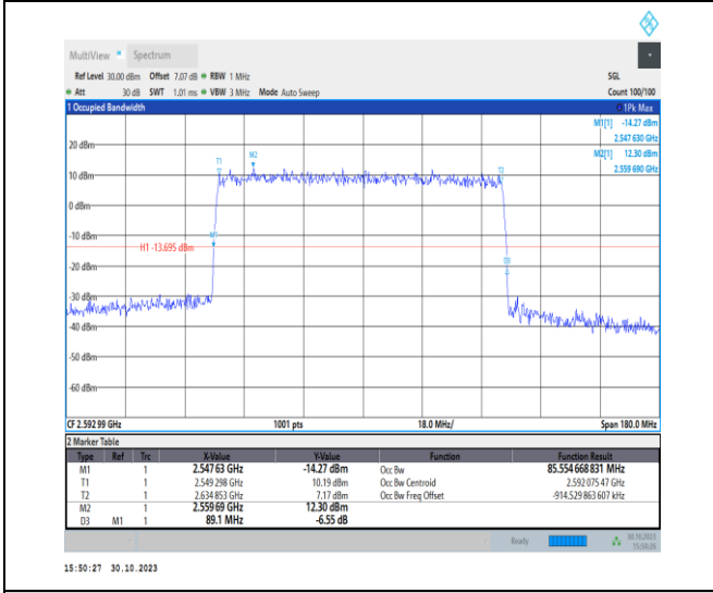
1-N41-30-90-M-5-DFT-256QAM-Outer_Full-240@0-A Ant1-85.555-89.100-≤90-PASS
