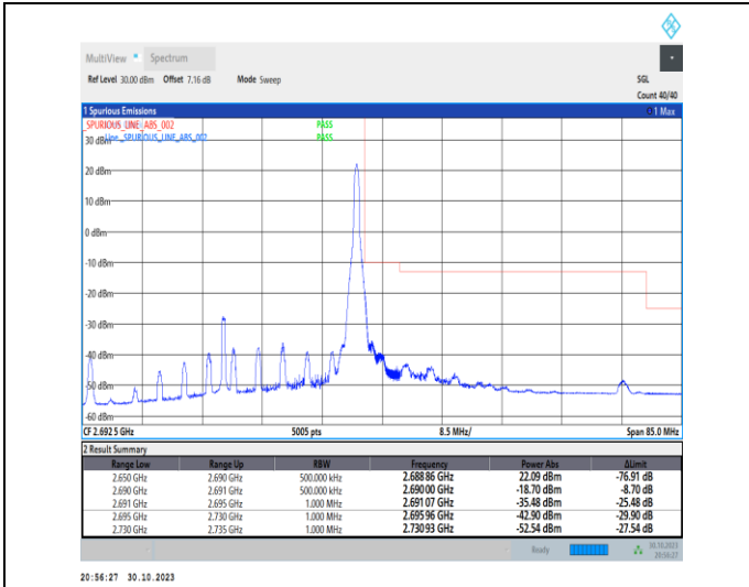
1-N41-30-40-H-2-DFT-PI2BPSK-Edge_1RB_Right-1 @ 105-Ant1-1--PASS-see graph
