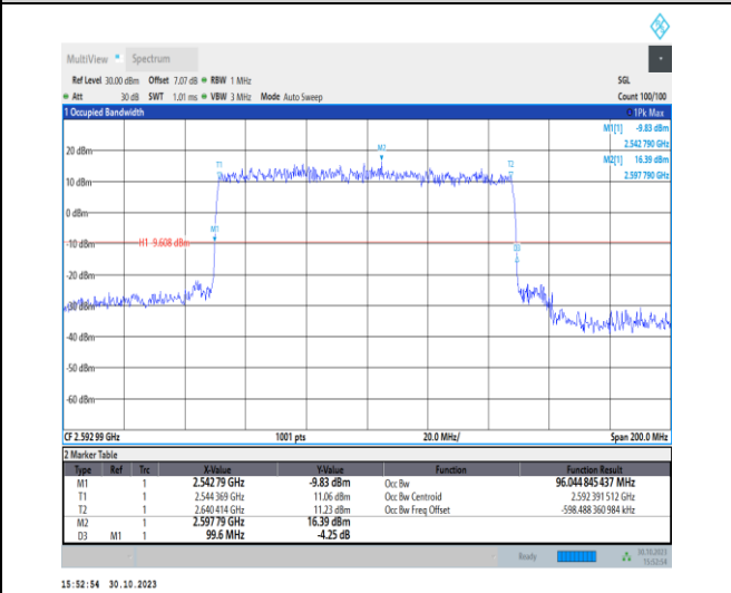
1-N41-30-100-M-1-DFT-QPSK-Outer_Full-270@0-A nt1-96.045-99.600-≤100-PASS
