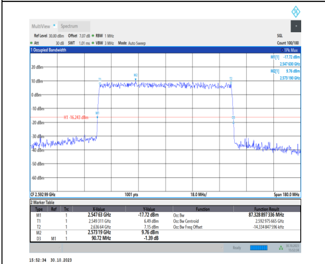
1-N41-30-90-M-9-CP-256QAM-Outer_Full-245@0-A nt1-87.329-90.720-≤90-PASS
