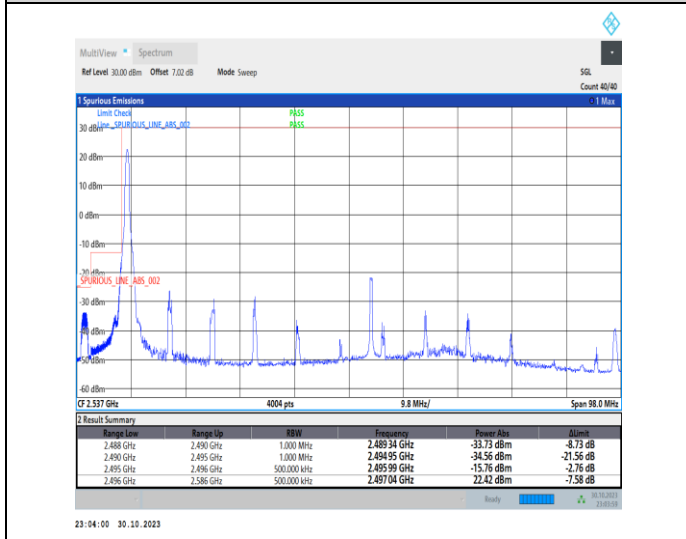
1-N41-30-90-L-4-CP-QPSK-Edge_1RB_Left-1@0-Ant1-1--PASS-see graph
