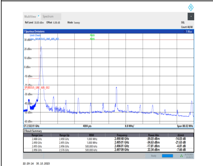
1-N41-30-80-L-4-CP-QPSK-Edge_1RB_Left-1@0-Ant1-1--PASS-see graph
