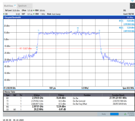
1-N41-30-30-M-7-CP-16QAM-Outer_Full-78@0-Ant 1-27.791-29.220-≤30-PASS
