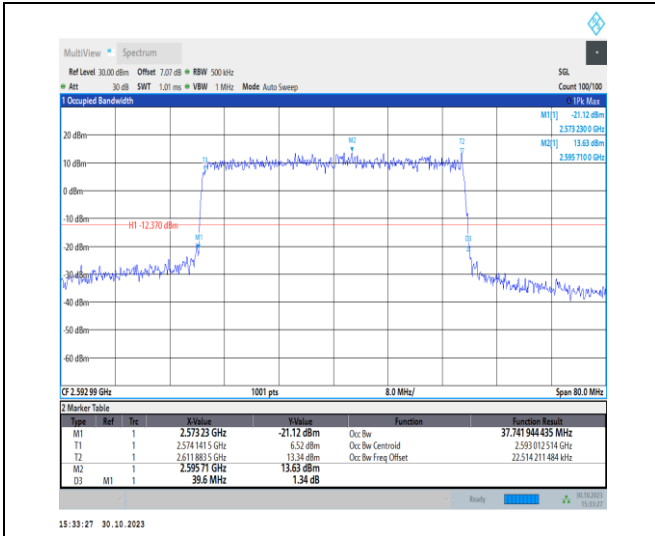
1-N41-30-40-M-7-CP-16QAM-Outer_Full-106@0-Ant 1-37.742-39.600-≤40-PASS
