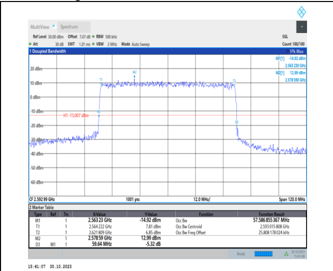
1-N41-30-60-M-6-CP-QPSK-Outer_Full-162@0-Ant1-57.587-59.640-≤60-PASS
