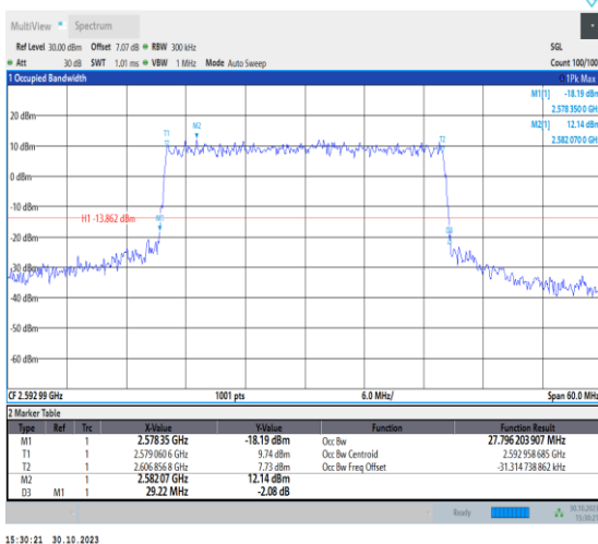
1-N41-30-30-M-6-CP-QPSK-Outer_Full-78@0-Ant1 27.796-29.220-≤30-PASS
