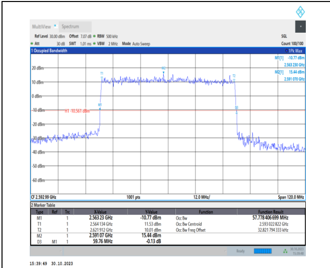
1-N41-30-60-M-1-DFT-QPSK-Outer_Full-162@0-Ant 1-57.778-59.760-≤60-PASS
