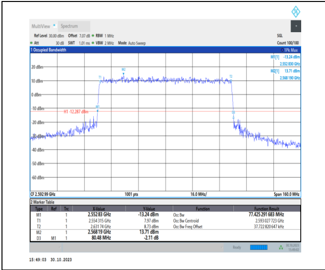
1-N41-30-80-M-8-CP-64QAM-Outer_Full-217@0-Ant 1-77.425-80.480-≤80-PASS
