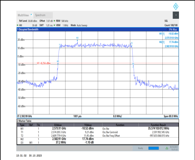
1-N41-30-40-M-2-DFT-PI2BPSK-Outer_Full-100@0-Ant1 -35.574-37.200-≤40-PASS
