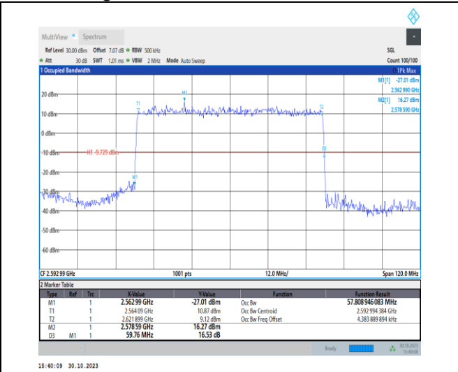
1-N41-30-60-M-2-DFT-PI2BPSK-Outer_Full-162@0-Ant 1-57.809-59.760-≤60-PASS
