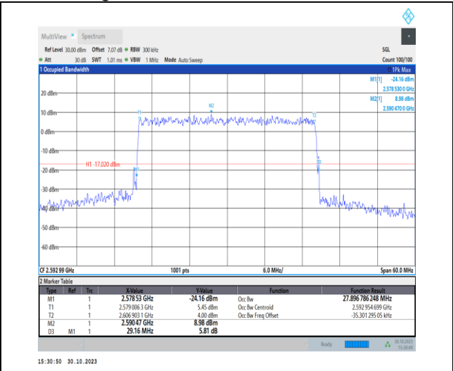
1-N41-30-30-M-9-CP-256QAM-Outer_Full-78@0-Ant1 -27.897-29.160-≤30-PASS
