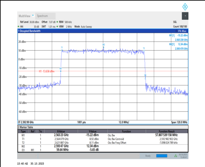
1-N41-30-60-M-4-DFT-64QAM-Outer_Full-162@0-Ant 1-57.808-59.640-≤60-PASS
