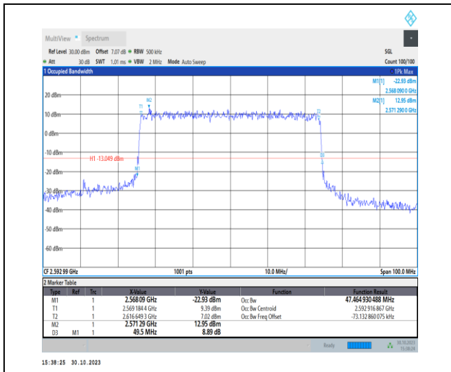
1-N41-30-50-M-6-CP-QPSK-Outer_Full-133@0-Ant1 -47.465-49.500-≤50-PASS
