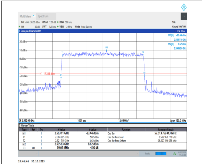
1-N41-30-60-M-9-CP-256QAM-Outer_Full-162@0-A nt1-57.514-59.640-≤60-PASS
