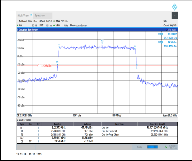
1-N41-30-40-M-6-CP-QPSK-Outer_Full-106@0-Ant1 -37.751-39.520-≤40-PASS
