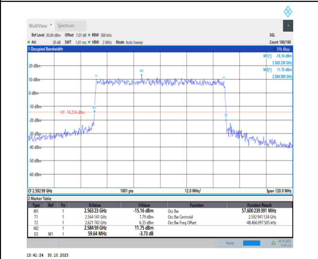
1-N41-30-60-M-8-CP-64QAM-Outer_Full-162@0-Ant1-57.6-59.640-≤60-PASS
