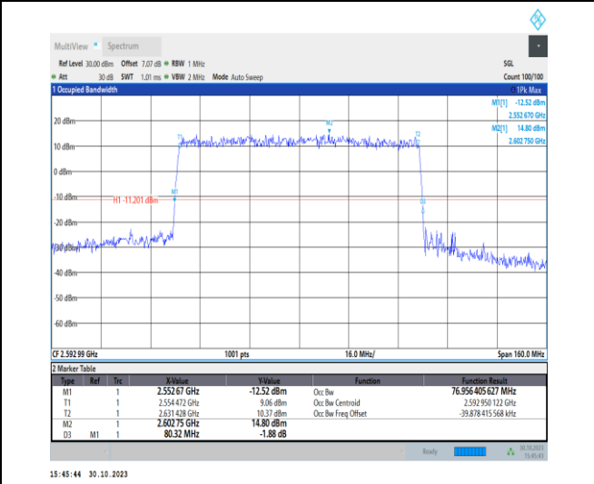
1-N41-30-80-M-3-DFT-16QAM-Outer_Full-216@0-A nt1-76.956-80.320-≤80-PASS
