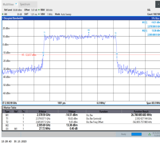
1-N41-30-30-M-4-DFT-64QAM-Outer_Full-75@0-Ant 1-26.78-27.720-≤30-PASS
