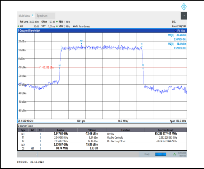
1-N41-30-90-M-2-DFT-PI2BPSK-Outer_Full-240@0-Ant 1-85.287-88.740-≤90-PASS
