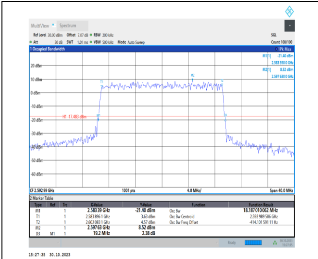
1-N41-30-20-M-9-CP-256QAM-Outer_Full-51@0-Ant 1-18.187-19.200-≤20-PASS
