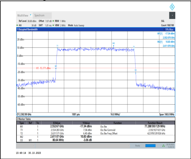
1-N41-30-80-M-9-CP-256QAM-Outer_Full-217@0-A nt1-77.289-80.640-≤80-PASS
