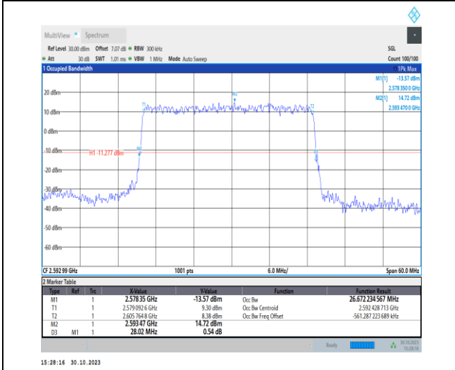
1-N41-30-30-M-2-DFT-PI2BPSK-Outer_Full-75@0-A nt1-26.672-28.020-≤30-PASS
