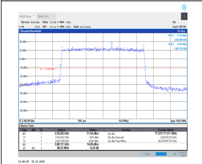
1-N41-30-80-M-6-CP-QPSK-Outer_Full-217@0-Ant1 -77.372-80.320-≤80-PASS
