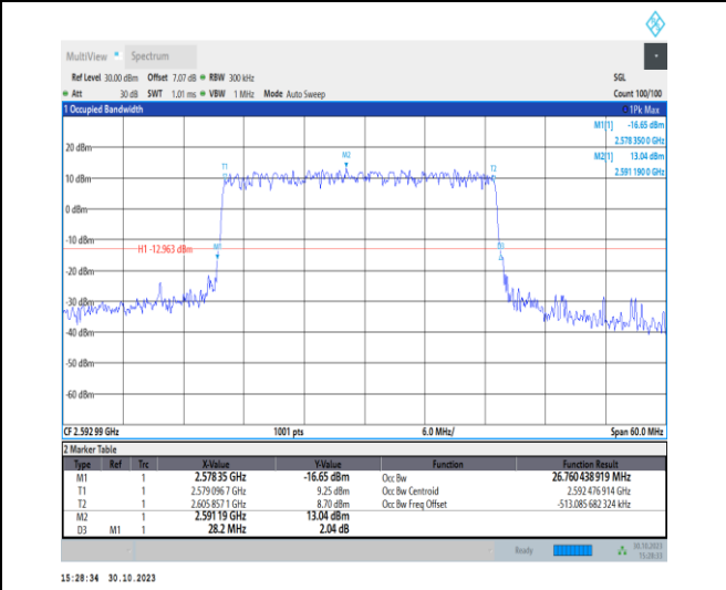
1-N41-30-30-M-3-DFT-16QAM-Outer_Full-75@0-Ant 1-26.76-28.200-≤30-PASS
