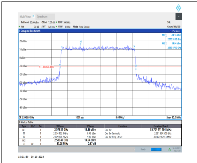
1-N41-30-40-M-3-DFT-16QAM-Outer_Full-100@0-A nt1-35.704-37.280-≤40-PASS
