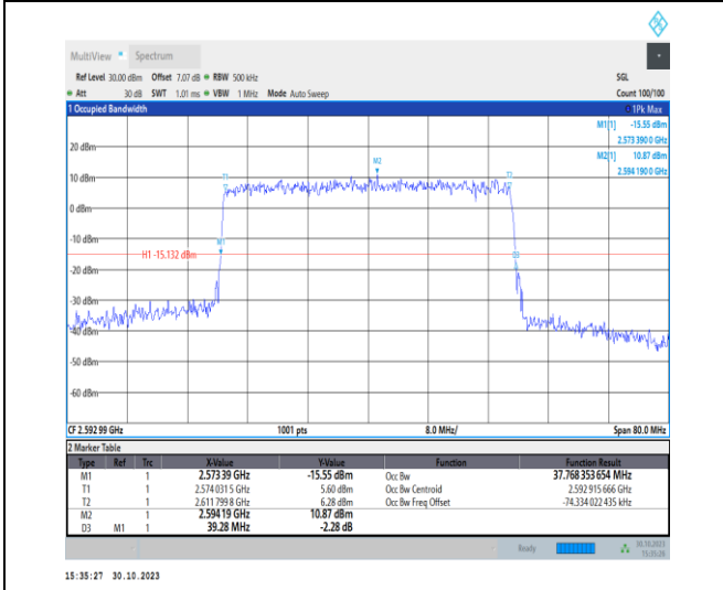
1-N41-30-40-M-9-CP-256QAM-Outer_Full-106@0-A nt1-37.768-39.280-≤40-PASS
