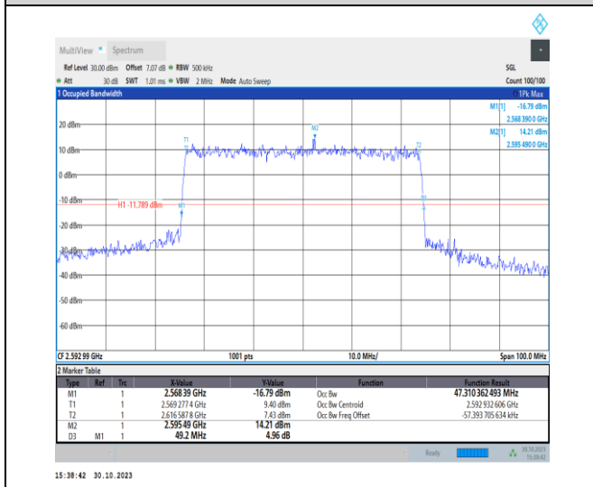
1-N41-30-50-M-8-CP-64QAM-Outer_Full-133@0-Ant1 1-47.31-49.200-≤50-PASS
