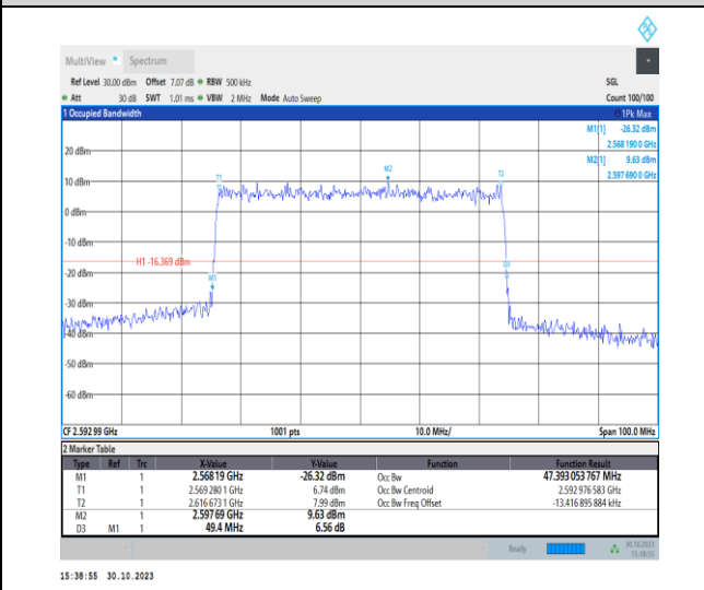
1-N41-30-50-M-9-CP-256QAM-Outer_Full-133@0-Ant1 -47.393-49.400-≤50-PASS
