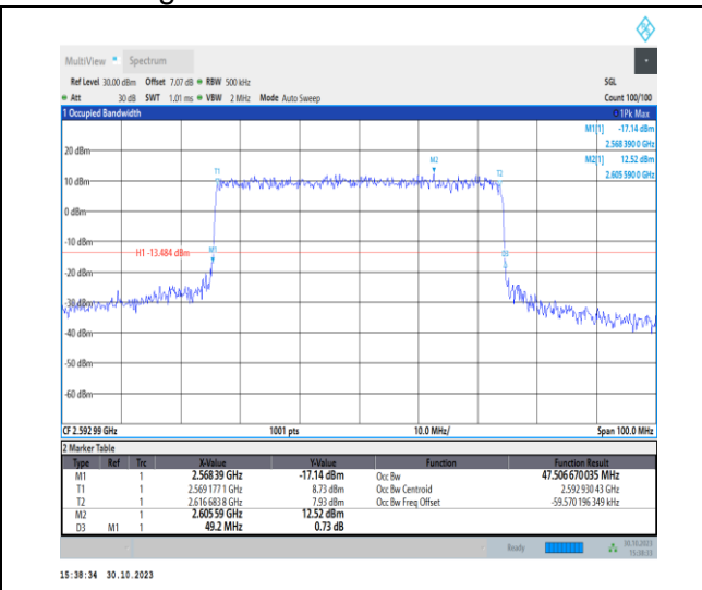
1-N41-30-50-M-7-CP-16QAM-Outer_Full-133@0-Ant1 -47.507-49.200-≤50-PASS
