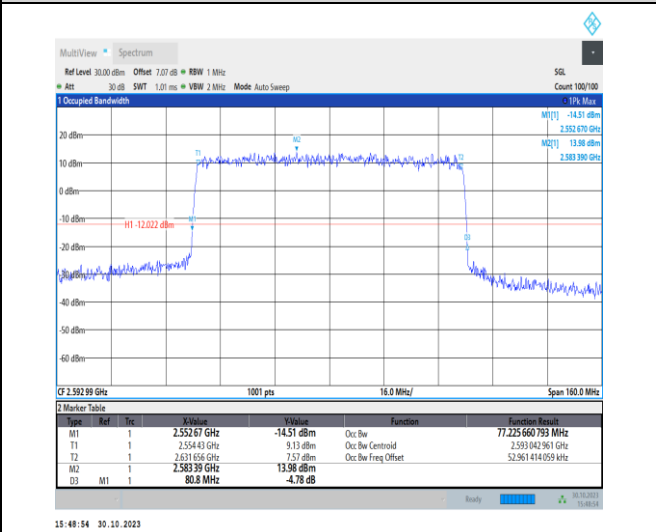
1-N41-30-80-M-7-CP-16QAM-Outer_Full-217@0-Ant1 t1-77.226-80.800-≤80-PASS
