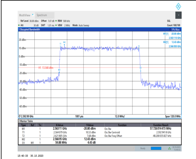
1-N41-30-60-M-3-DFT-16QAM-Outer_Full-162@0-Ant 1-57.726-59.880-≤60-PASS
