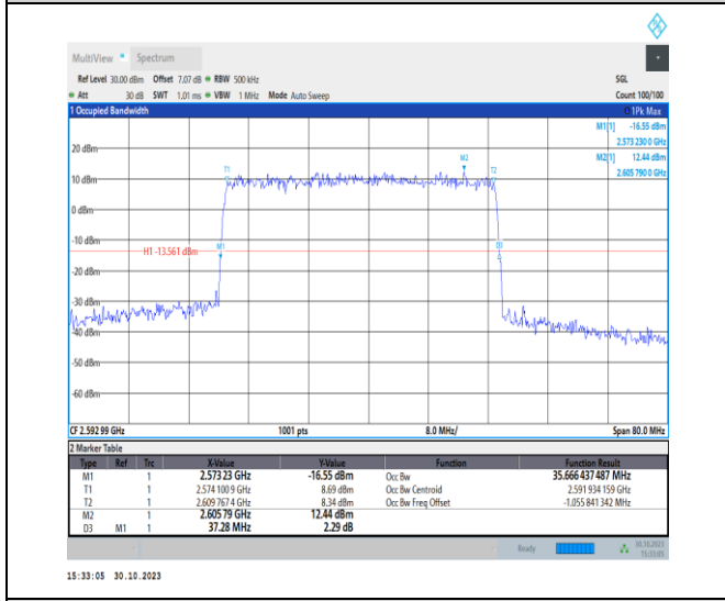
1-N41-30-40-M-5-DFT-256QAM-Outer_Full-100@0-A Ant1-35.666-37.280-≤40-PASS
