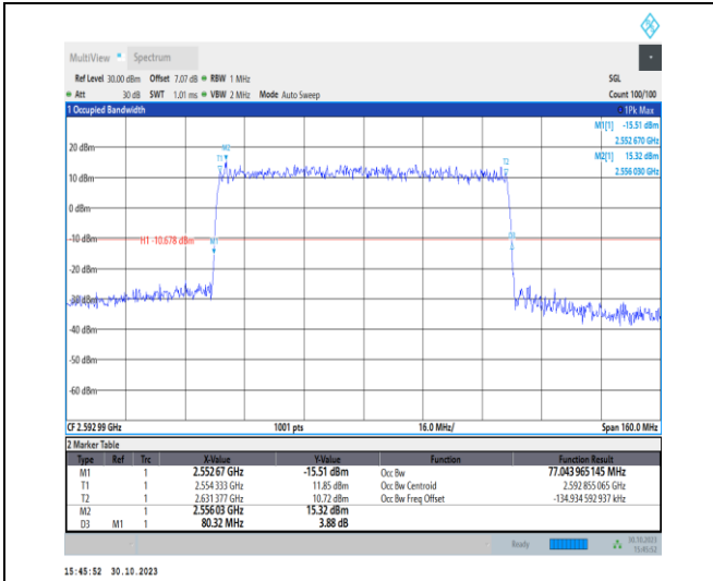
1-N41-30-80-M-4-DFT-64QAM-Outer_Full-216@0-A nt1-77.044-80.320-≤80-PASS
