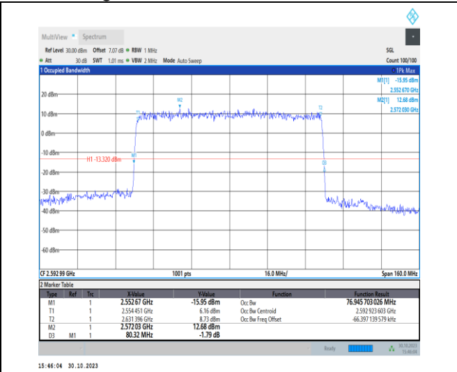
1-N41-30-80-M-5-DFT-256QAM-Outer_Full-216@0-A Ant1-76.946-80.320-≤80-PASS
