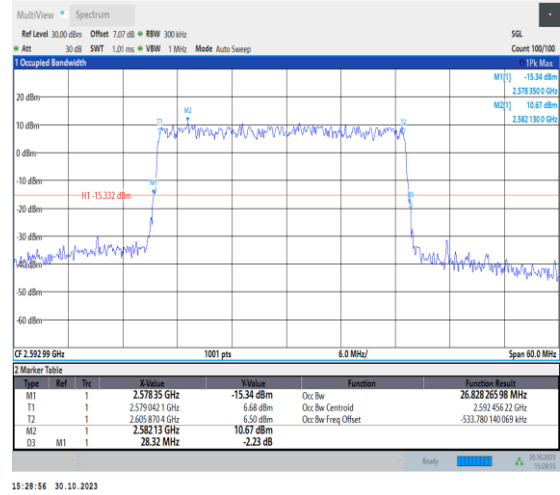
1-N41-30-30-M-5-DFT-256QAM-Outer_Full-75@0-A nt1-26.828-28.320-≤30-PASS
