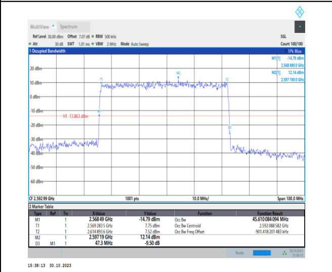
1-N41-30-50-M-5-DFT-256QAM-Outer_Full-128@0-Ant1-45.61-47.300-≤50-PASS
