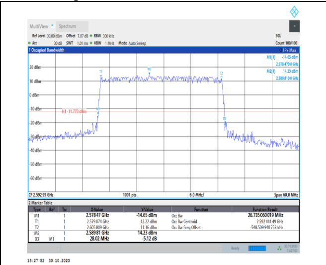
1-N41-30-30-M-1-DFT-QPSK-Outer_Full-75@0-Ant1 -26.735-28.020-≤30-PASS
