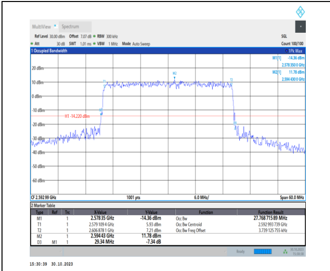
1-N41-30-30-M-8-CP-64QAM-Outer_Full-78@0-Ant1 -27.769-29.340-≤30-PASS
