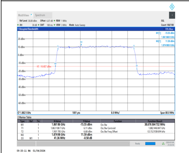
1-N25-15-40-M-9-CP-256QAM-Outer_Full-216@0-Ant nt1-38.676-41.360-≤40-PASS
