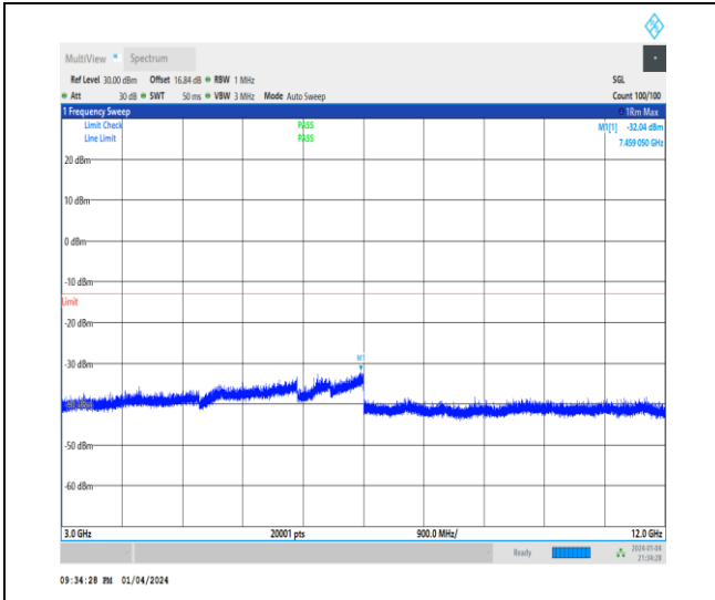
1-N25-15-40-L-1-DFT-PI2BPSK-Inner_1RB_Left-1 @ 1-3000-12000-Ant1-7459.05--32.04--13-PASS
