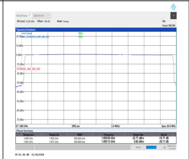
1-N25-15-25-L-6-CP-QPSK-Outer_Full-133@0-Ant1-1-seegraph-PASS-see graph
