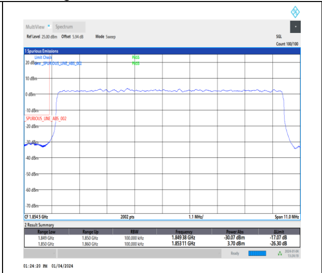
1-N25-15-10-L-3-DFT-PI2BPSK-Outer_Full-50@0-Ant1-1-seegraph-PASS-see graph
