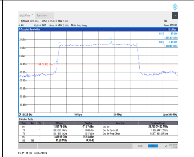
1-N25-15-40-M-6-CP-QPSK-Outer_Full-216@0-Ant1 -38.75-41.280-≤40-PASS
