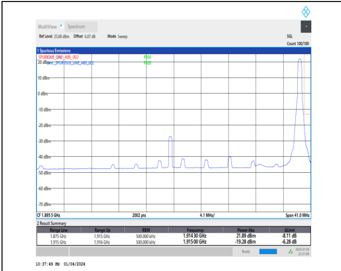
1-N25-15-40-H-2-DFT-PI2BPSK-Edge_1RB_Right-1@215-Ant1-1-seegraph-PASS-see graph
