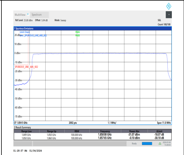
1-N25-15-10-L-6-CP-QPSK-Outer_Full-52@0-Ant1-1-seegraph-PASS-see graph
