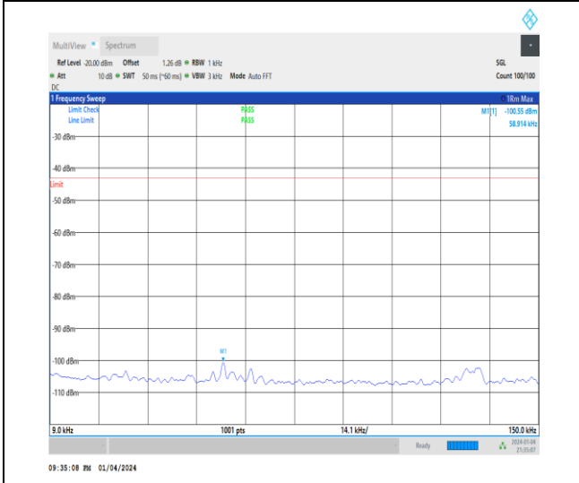
1-N25-15-40-M-1-DFT-PI2BPSK-Inner_1RB_Left-1 @ 1-0.009-0.15-Ant1-0.06--100.55--43-PASS
