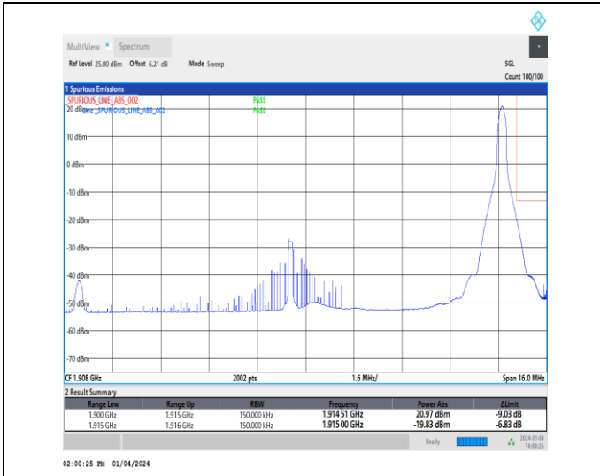
1-N25-15-15-H-2-DFT-PI2BPSK-Edge_1RB_Right-1@78-Ant1-1-seegraph-PASS-see graph
