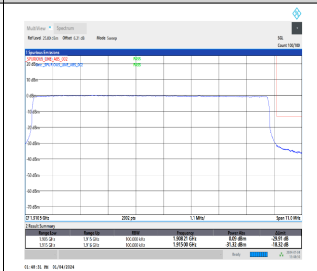
1-N25-15-10-H-6-CP-QPSK-Outer_Full-52@0-Ant1-1-seegraph-PASS-see graph
