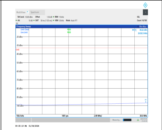
1-N25-15-40-M-1-DFT-PI2BPSK-Inner_1RB_Left-1 @ 1-0.15-30-Ant1-29.55--96.62--33-PASS
