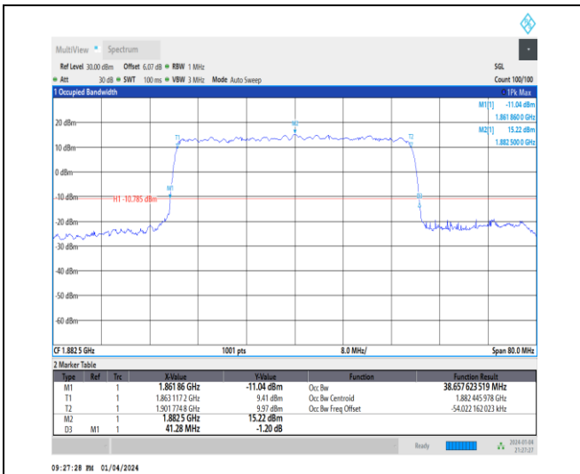
1-N25-15-40-M-7-CP-16QAM-Outer_Full-216@0-Ant 1-38.658-41.280-≤40-PASS
