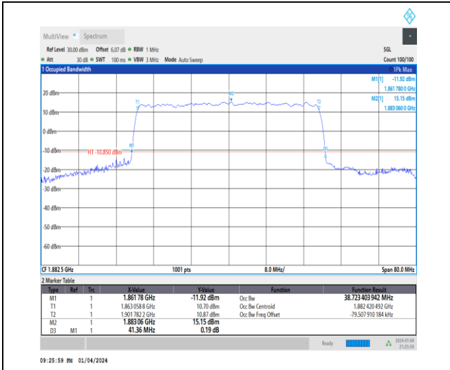
1-N25-15-40-M-3-DFT-16QAM-Outer_Full-216@0-A nt1-38.723-41.360-≤40-PASS
