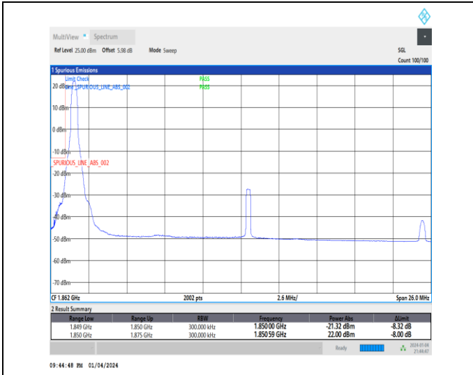
1-N25-15-25-L-1-DFT-PI2BPSK-Edge_1RB_Left-1@0-Ant1-1-seegraph-PASS-see graph
