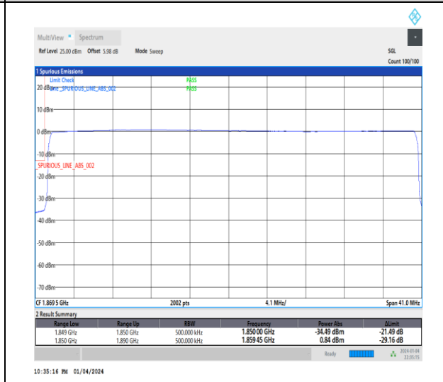
1-N25-15-40-L-6-CP-QPSK-Outer_Full-216@0-Ant1-1-seegraph-PASS-see graph
