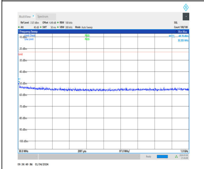
1-N25-15-40-H-1-DFT-PI2BPSK-Inner_1RB_Left-1 @ 1-30-1000-Ant1-35.34--49.78--23-PASS
