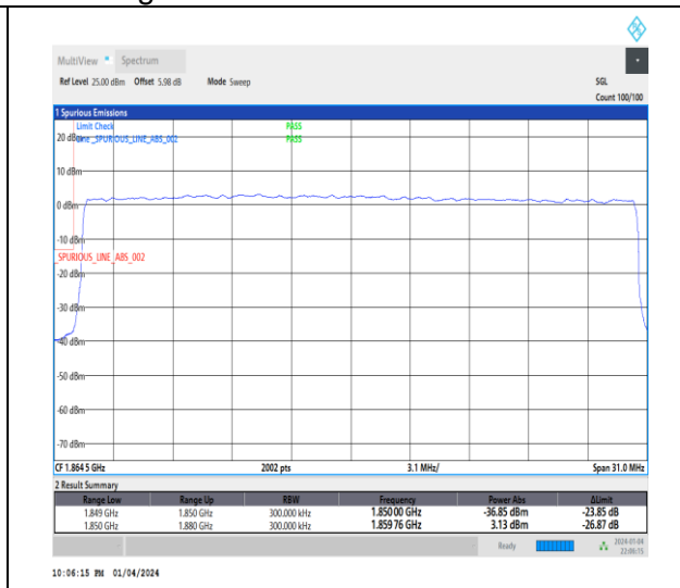
1-N25-15-30-L-3-DFT-PI2BPSK-Outer_Full-160@0-Ant1-1-seegraph-PASS-see graph
