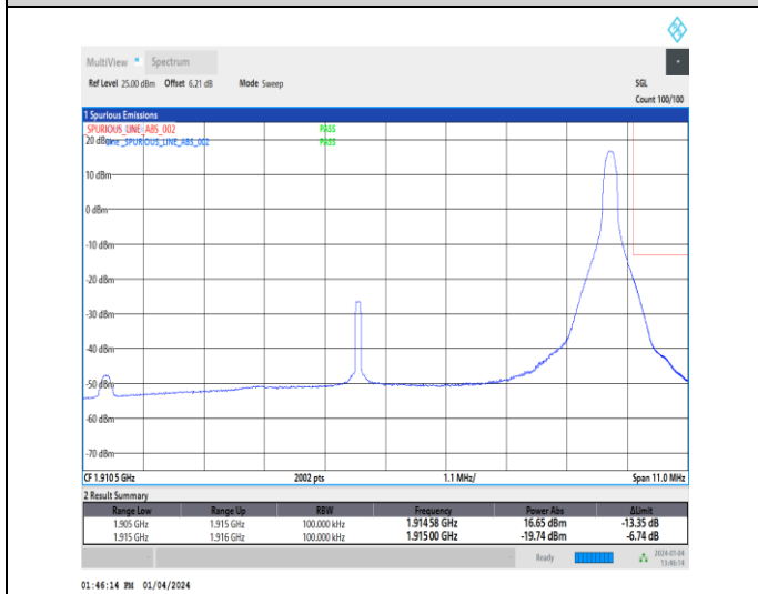
1-N25-15-10-H-5-CP-QPSK-Edge_1RB_Right-1@51-Ant1-1-seegraph-PASS-see graph
