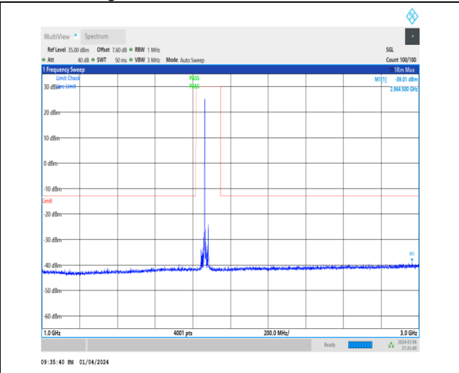
1-N25-15-40-M-1-DFT-PI2BPSK-Inner_1RB_Left-1 @ 1-1000-3000-Ant1-2964.50--39.01--13-PASS
