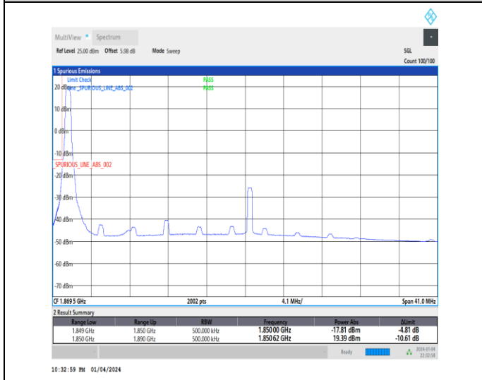
1-N25-15-40-L-4-CP-QPSK-Edge_1RB_Left-1@0-Ant1-1-seegraph-PASS-see graph
