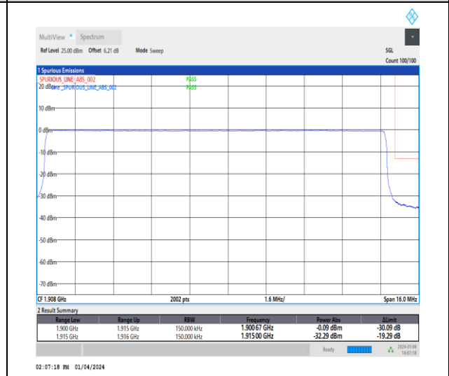
1-N25-15-15-H-6-CP-QPSK-Outer_Full-79@0-Ant1-1-seegraph-PASS-see graph
