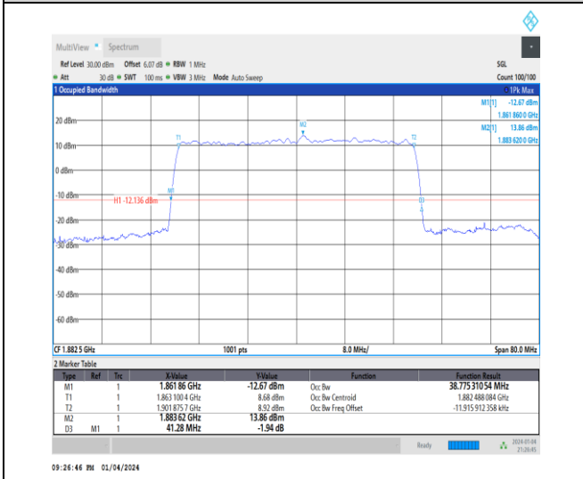
1-N25-15-40-M-5-DFT-256QAM-Outer_Full-216@0-A Ant1-38.775-41.280-≤40-PASS
