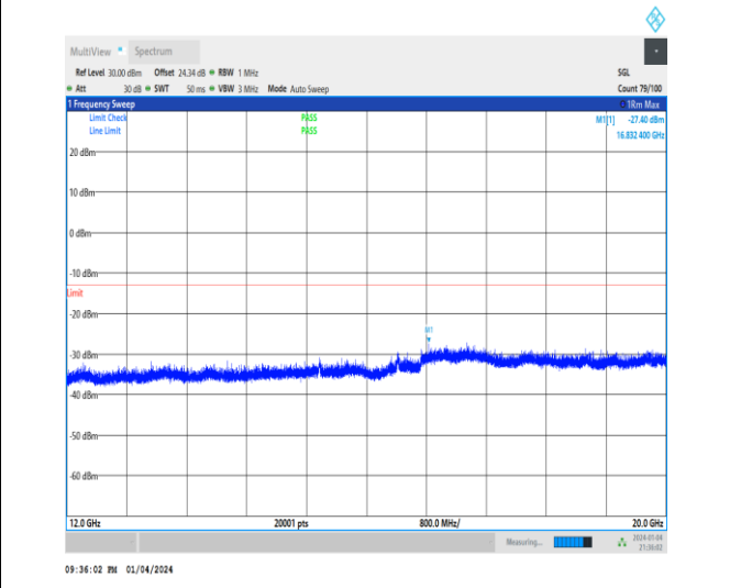
1-N25-15-40-M-1-DFT-PI2BPSK-Inner_1RB_Left-1 @ 1-12000-20000-Ant1-16832.40--27.40--13-PASS
