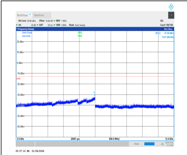
1-N25-15-40-H-1-DFT-PI2BPSK-Inner_1RB_Left-1 @ 1-3000-12000-Ant1-7471.20--31.34--13-PASS
