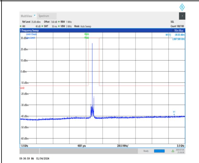
1-N25-15-40-H-1-DFT-PI2BPSK-Inner_1RB_Left-1 @ 1-1000-3000-Ant1-2867.50--39.55--13-PASS
