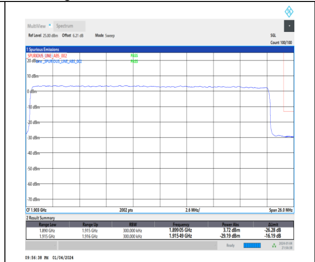
1-N25-15-25-H-3-DFT-PI2BPSK-Outer_Full-128@0-Ant1-1-seegraph-PASS-see graph
