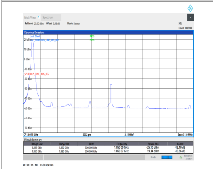
1-N25-15-30-L-4-CP-QPSK-Edge_1RB_Left-1@0-Ant1-1-seegraph-PASS-see graph
