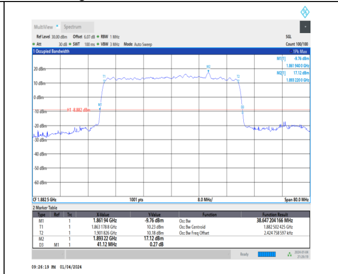
1-N25-15-40-M-4-DFT-64QAM-Outer_Full-216@0-A nt1-38.647-41.120-≤40-PASS
