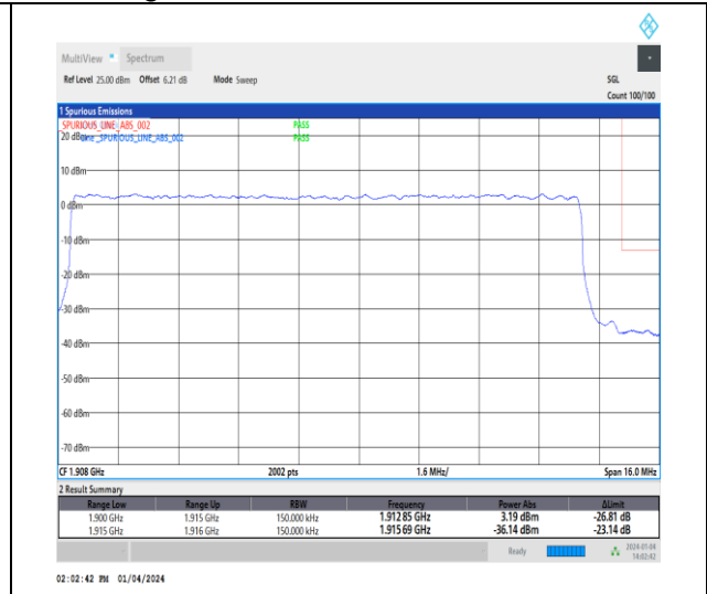
1-N25-15-15-H-3-DFT-PI2BPSK-Outer_Full-75@0-Ant1-1-seegraph-PASS-see graph
