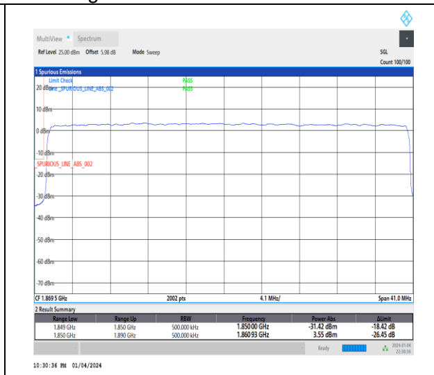
1-N25-15-40-L-3-DFT-PI2BPSK-Outer_Full-216@0-Ant1-1-seegraph-PASS-see graph
