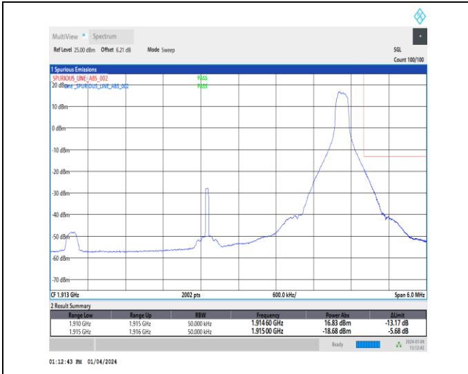
1-N25-15-5-H-2-DFT-PI2BPSK-Edge_1RB_Right-1@2-4-Ant1-1-seegraph-PASS-see graph
