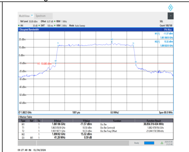
1-N25-15-40-M-8-CP-64QAM-Outer_Full-216@0-Ant 1-38.856-41.280-≤40-PASS
