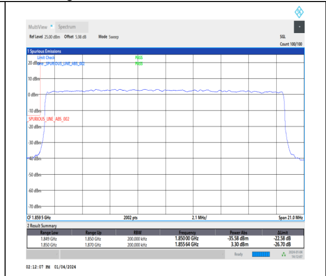
1-N25-15-20-L-3-DFT-PI2BPSK-Outer_Full-100@0-Ant1-1-seegraph-PASS-see graph
