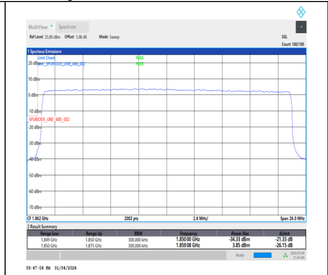
1-N25-15-25-L-3-DFT-PI2BPSK-Outer_Full-128@0-Ant1-1-seegraph-PASS-see graph
