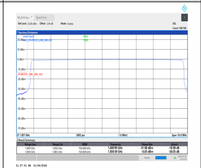
1-N25-15-15-L-6-CP-QPSK-Outer_Full-79@0-Ant1-1-seegraph-PASS-see graph
