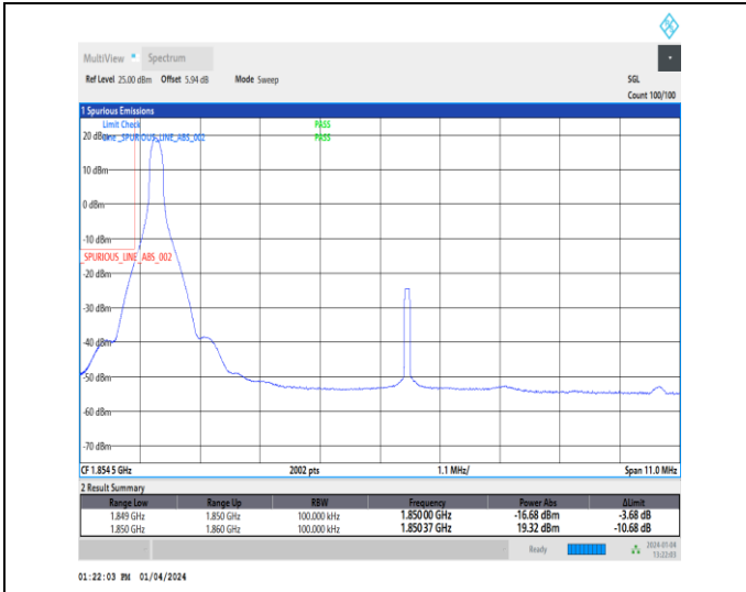
1-N25-15-10-L-1-DFT-PI2BPSK-Edge_1RB_Left-1@0-Ant1-1-seegraph-PASS-see graph
