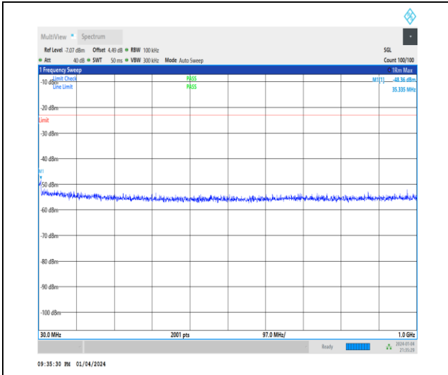
1-N25-15-40-M-1-DFT-PI2BPSK-Inner_1RB_Left-1 @ 1-30-1000-Ant1-35.34--48.36--23-PASS
