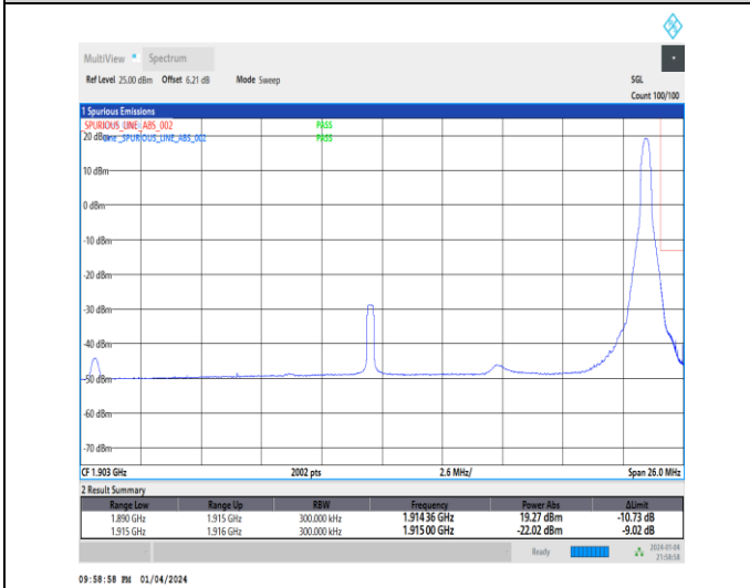
1-N25-15-25-H-5-CP-QPSK-Edge_1RB_Right-1@132-Ant1-1-seegraph-PASS-see graph
