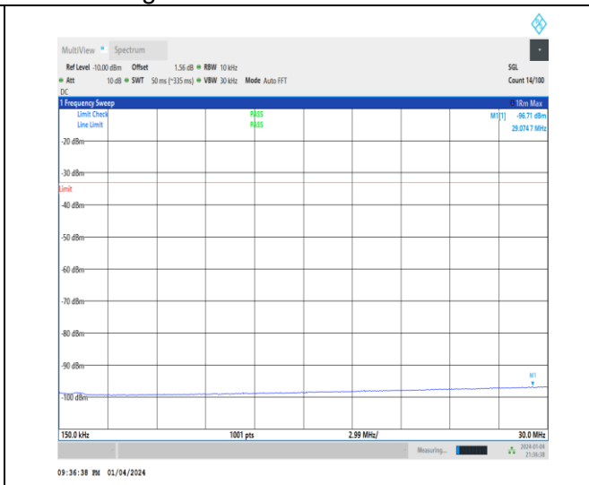
1-N25-15-40-H-1-DFT-PI2BPSK-Inner_1RB_Left-1 @ 1-0.15-30-Ant1-29.07--96.71--33-PASS
