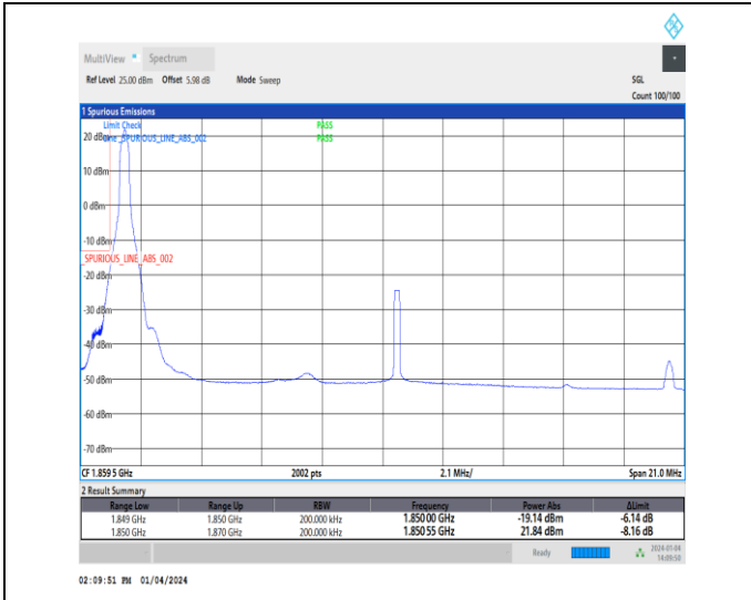
1-N25-15-20-L-1-DFT-PI2BPSK-Edge_1RB_Left-1@0-Ant1-1-seegraph-PASS-see graph
