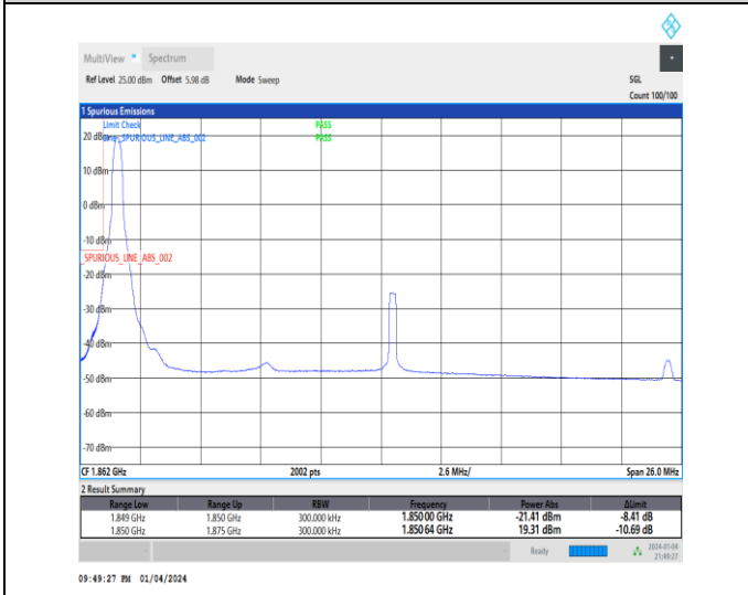
1-N25-15-25-L-4-CP-QPSK-Edge_1RB_Left-1@0-Ant1-1-seegraph-PASS-see graph
