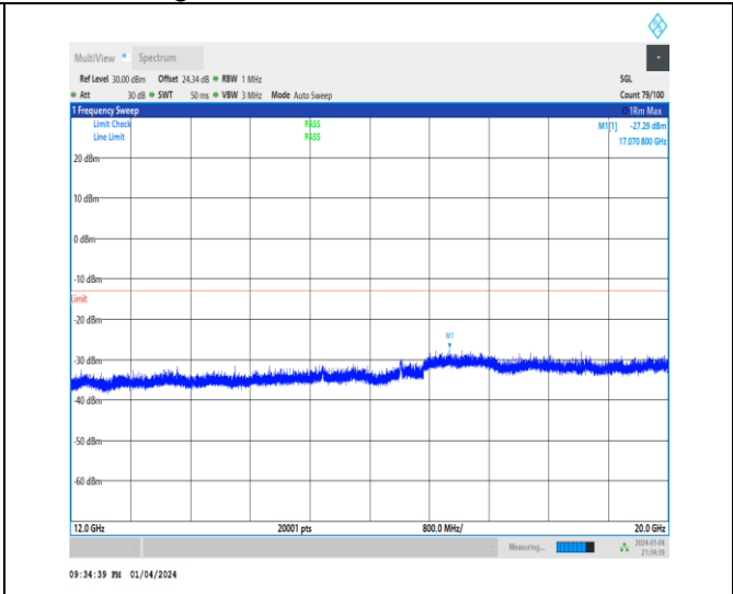
1-N25-15-40-L-1-DFT-PI2BPSK-Inner_1RB_Left-1 @ 1-12000-20000-Ant1-17070.80--27.29--13-PASS
