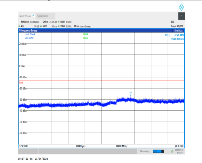
1-N25-15-40-H-1-DFT-PI2BPSK-Inner_1RB_Left-1 @ 1-12000-20000-Ant1-17408.00--27.25--13-PASS
