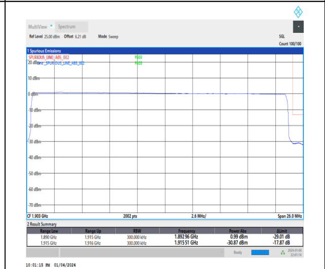
1-N25-15-25-H-6-CP-QPSK-Outer_Full-133@0-Ant1-1-seegraph-PASS-see graph
