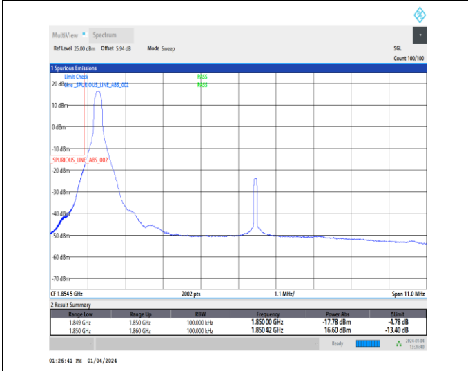
1-N25-15-10-L-4-CP-QPSK-Edge_1RB_Left-1@0-Ant1-1-seegraph-PASS-see graph
