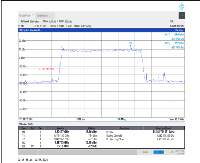
1-N25-15-15-M-9-CP-256QAM-Outer_Full-79@0-Ant 1-14.182-15.120≤15-PASS
