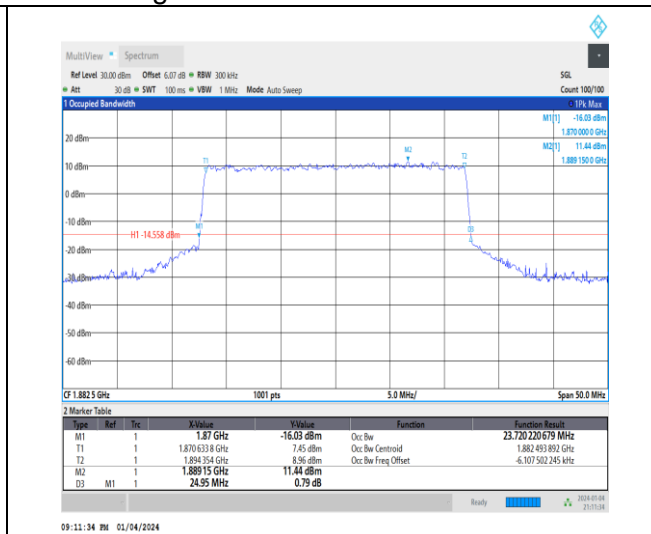
1-N25-15-25-M-6-CP-QPSK-Outer_Full-133@0-Ant1-23.72-24.950-≤25-PASS
