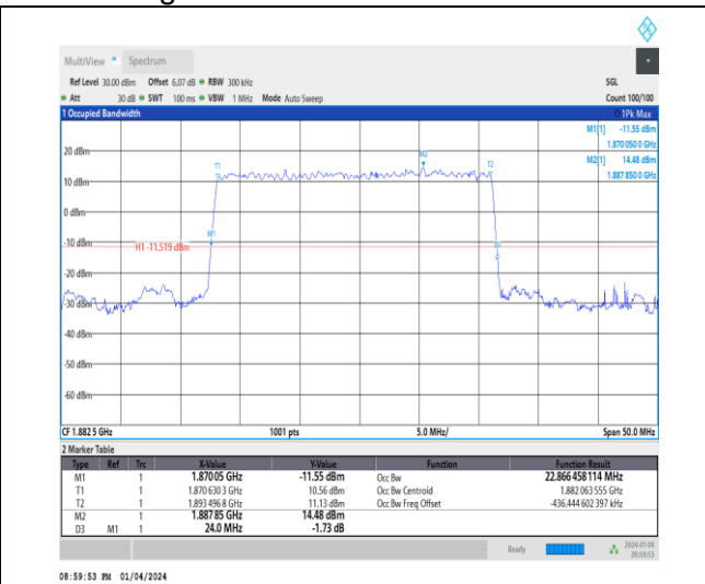
1-N25-15-25-M-2-DFT-PI2BPSK-Outer_Full-128@0-Ant1-22.866-24.000-≤25-PASS
