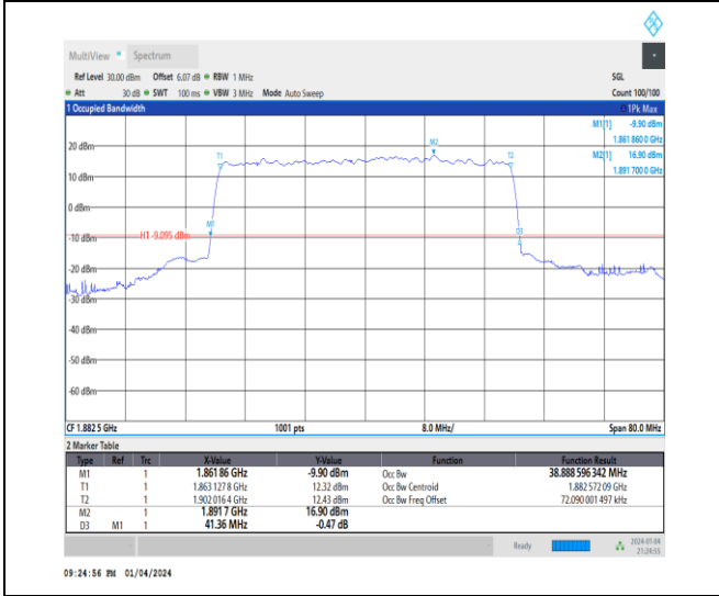
1-N25-15-40-M-1-DFT-QPSK-Outer_Full-216@0-Ant 1-38.889-41.360-≤40-PASS
