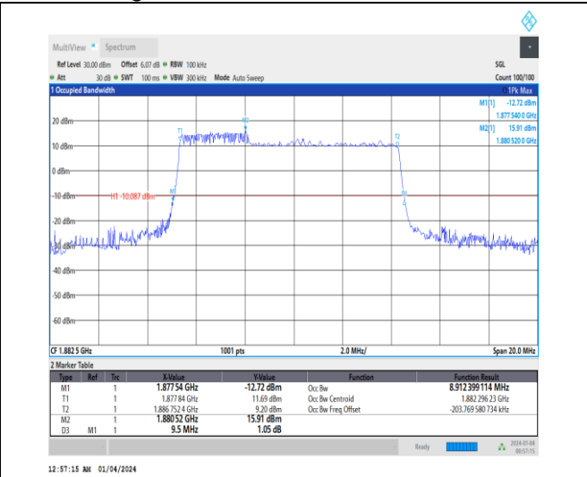
1-N25-15-10-M-1-DFT-QPSK-Outer_Full-50@0-Ant1 -8.912-9.500-≤10-PASS
