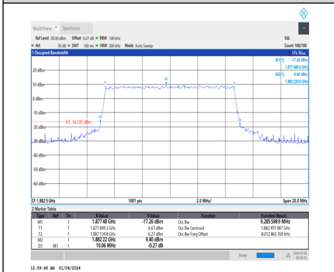
1-N25-15-10-M-6-CP-QPSK-Outer_Full-52@0-Ant1 9.286-10.060-≤10-PASS
