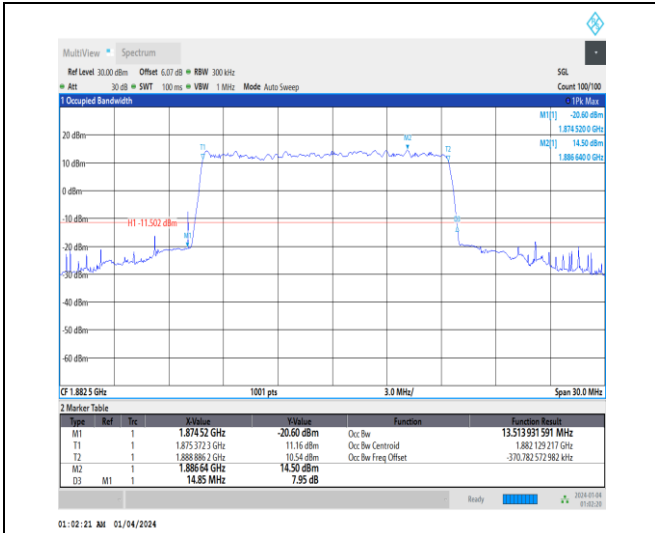
1-N25-15-15-M-3-DFT-16QAM-Outer_Full-75@0-Ant 1-13.514-14.850-≤15-PASS
