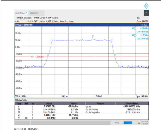
1-N25-15-5-M-5-DFT-256QAM-Outer_Full-25@0-Ant 1-4.485-5.010-≤5-PASS
