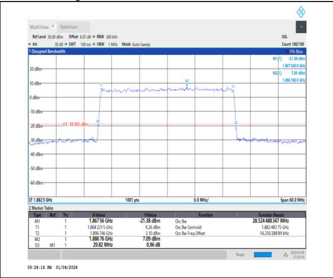
1-N25-15-30-M-9-CP-256QAM-Outer_Full-160@0-Ant nt1-28.524-29.820-≤30-PASS
