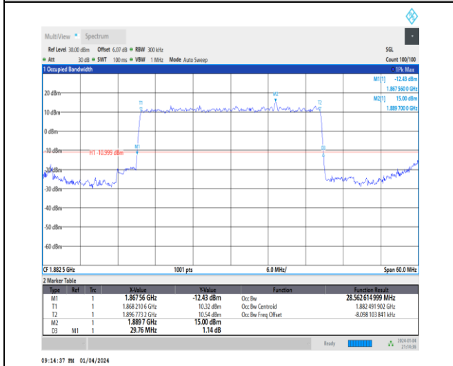
1-N25-15-30-M-2-DFT-PI2BPSK-Outer_Full-160@0-Ant1 1-28.563-29.760-≤30-PASS
