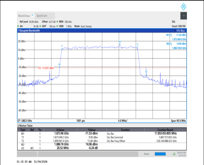
1-N25-15-20-M-1-DFT-QPSK-Outer_Full-100@0-Ant 1-17.855-20.520≤20-PASS
