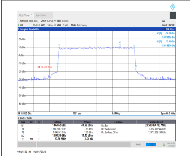
1-N25-15-30-M-6-CP-QPSK-Outer_Full-160@0-Ant1 -28.507-29.760-≤30-PASS
