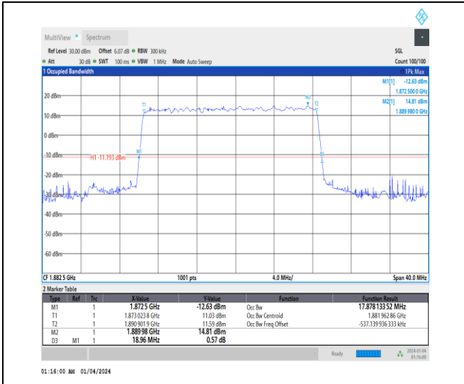
1-N25-15-20-M-2-DFT-PI2BPSK-Outer_Full-100@0-Ant1-17.878-18.960-≤20-PASS
