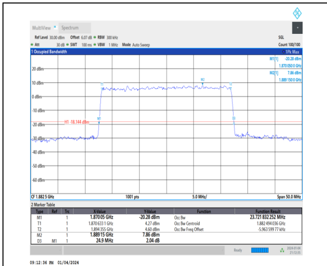
1-N25-15-25-M-9-CP-256QAM-Outer_Full-133@0-A nt1-23.722-24.900-≤25-PASS
