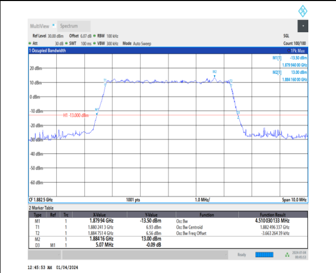
1-N25-15-5-M-8-CP-64QAM-Outer_Full-25@0-Ant1- 4.51-5.070-≤5-PASS
