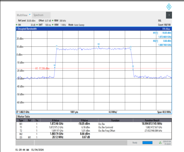
1-N25-15-20-M-9-CP-256QAM-Outer_Full-106@0-A nt1-18.995-20.120-≤20-PASS
