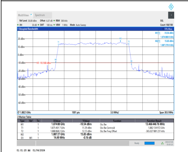
1-N25-15-15-M-1-DFT-QPSK-Outer_Full-75@0-Ant1 -13.466-14.490-≤15-PASS
