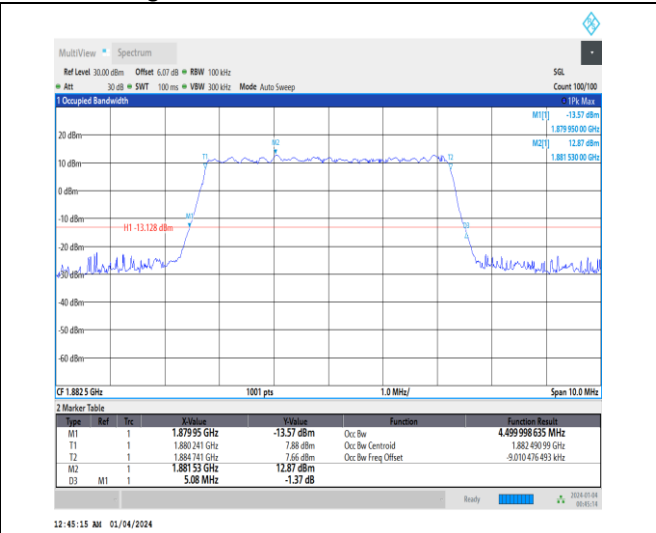
1-N25-15-5-M-6-CP-QPSK-Outer_Full-25@0-Ant1-4. 5-5.080-≤5-PASS
