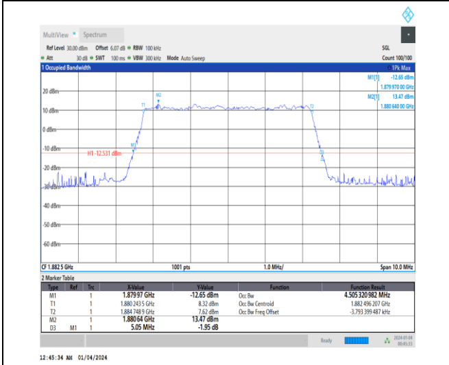
1-N25-15-5-M-7-CP-16QAM-Outer_Full-25@0-Ant1- 4.505-5.050-≤5-PASS
