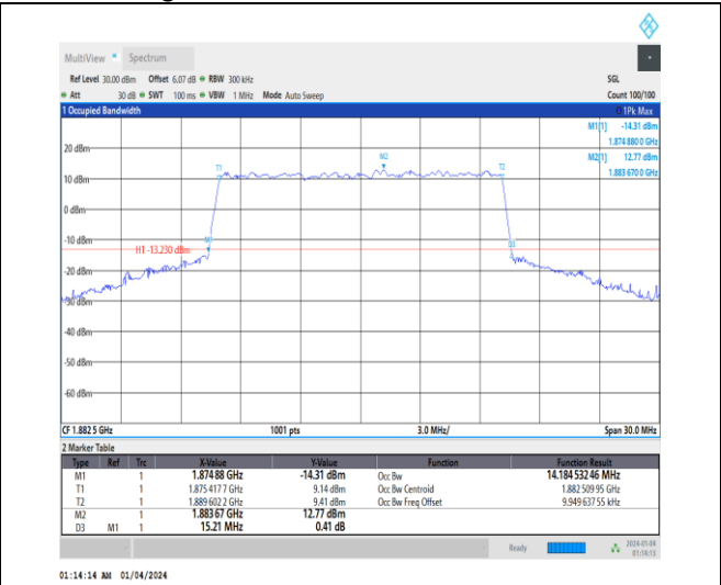
1-N25-15-15-M-8-CP-64QAM-Outer_Full-79@0-Ant1 -14.185-15.210≤15-PASS
