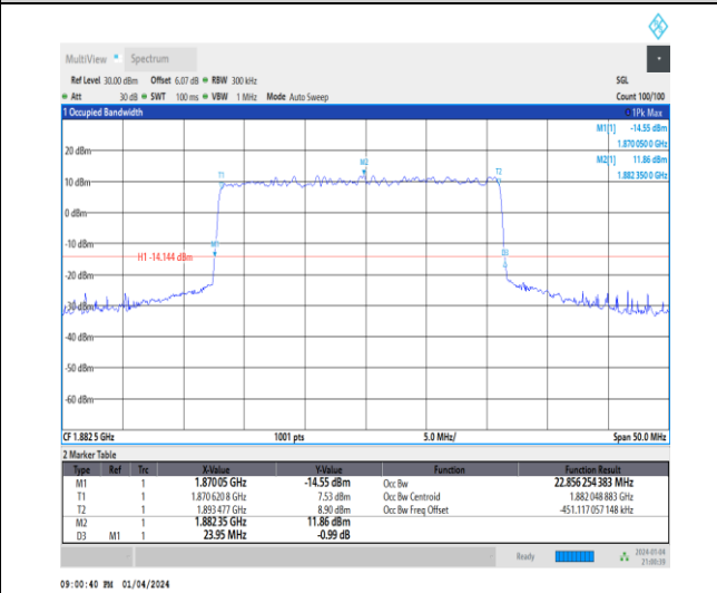
1-N25-15-25-M-4-DFT-64QAM-Outer_Full-128@0-Ant1-22.856-23.950-≤25-PASS
