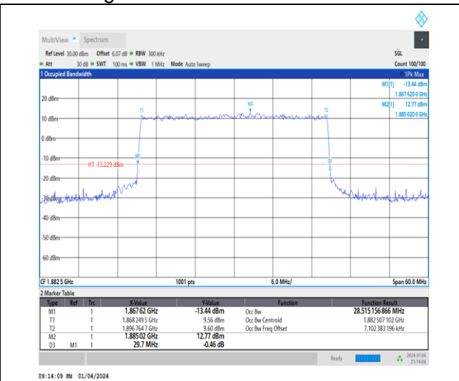
1-N25-15-30-M-1-DFT-QPSK-Outer_Full-160@0-Ant 1-28.515-29.700-≤30-PASS
