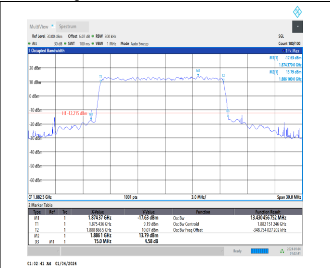
1-N25-15-15-M-4-DFT-64QAM-Outer_Full-75@0-Ant 1-13.43-15.000-≤15-PASS
