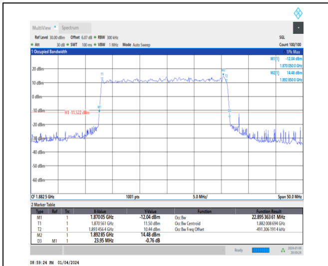
1-N25-15-25-M-1-DFT-QPSK-Outer_Full-128@0-Ant 1-22.895-23.950-≤25-PASS
