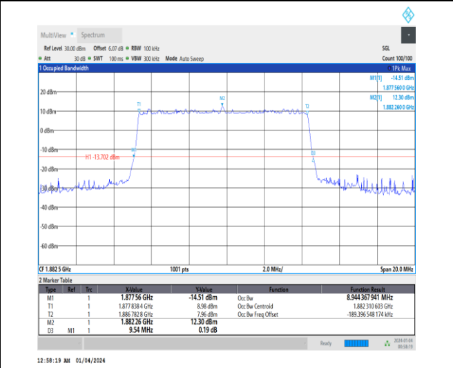
1-N25-15-10-M-3-DFT-16QAM-Outer_Full-50@0-Ant1 -8.944-9.540-≤10-PASS
