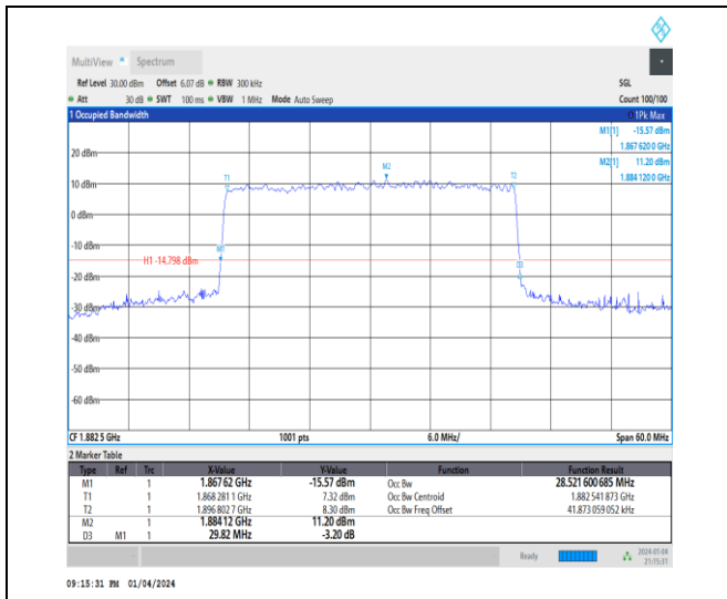
1-N25-15-30-M-4-DFT-64QAM-Outer_Full-160@0-A nt1-28.522-29.820-≤30-PASS
