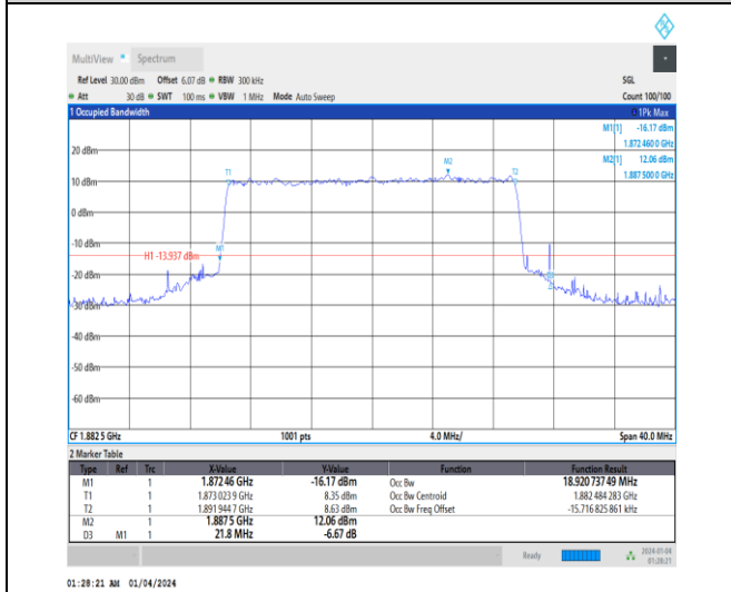
1-N25-15-20-M-8-CP-64QAM-Outer_Full-106@0-Ant 1-18.921-21.800-≤20-PASS
