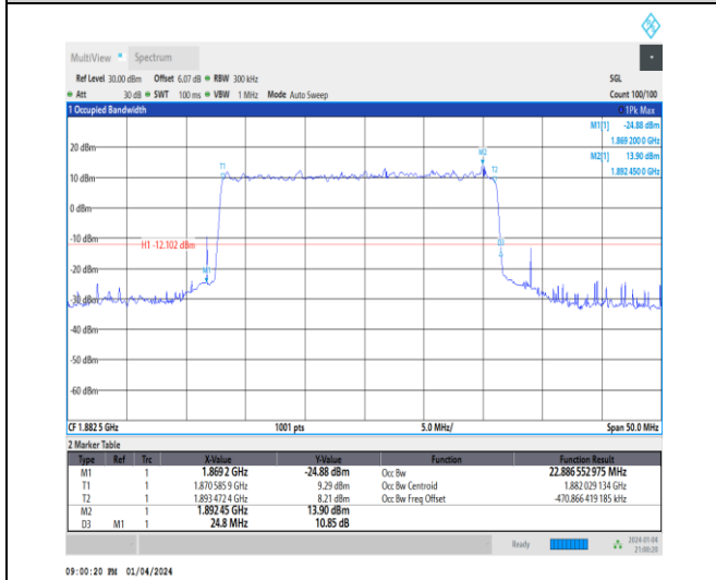
1-N25-15-25-M-3-DFT-16QAM-Outer_Full-128@0-Ant1-22.887-24.800-≤25-PASS
