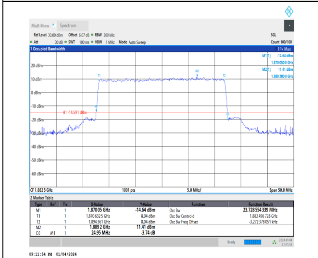
1-N25-15-25-M-7-CP-16QAM-Outer_Full-133@0-Ant1-23.729-24.950-≤25-PASS
