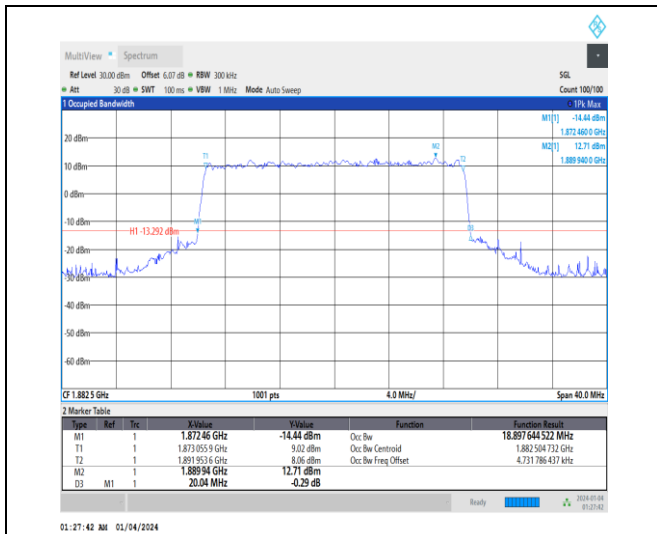
1-N25-15-20-M-6-CP-QPSK-Outer_Full-106@0-Ant1 -18.898-20.040-≤20-PASS
