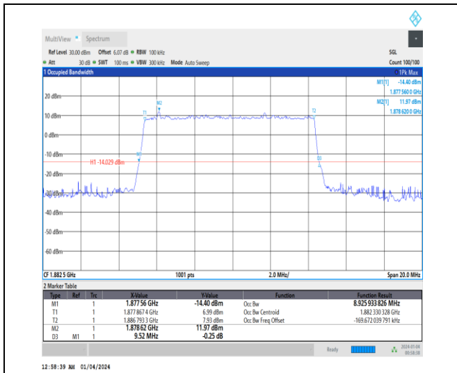
1-N25-15-10-M-4-DFT-64QAM-Outer_Full-50@0-Ant 1-8.926-9.520-≤10-PASS
