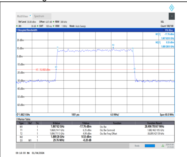
1-N25-15-30-M-5-DFT-256QAM-Outer_Full-160@0-A Ant1-28.497-29.760-≤30-PASS
