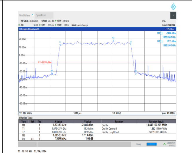
1-N25-15-15-M-2-DFT-PI2BPSK-Outer_Full-75@0-Ant1 -13.443-15.990-≤15-PASS
