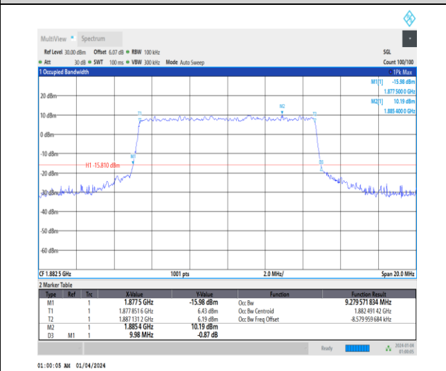
1-N25-15-10-M-7-CP-16QAM-Outer_Full-52@0-Ant1 -9.28-9.980-≤10-PASS
