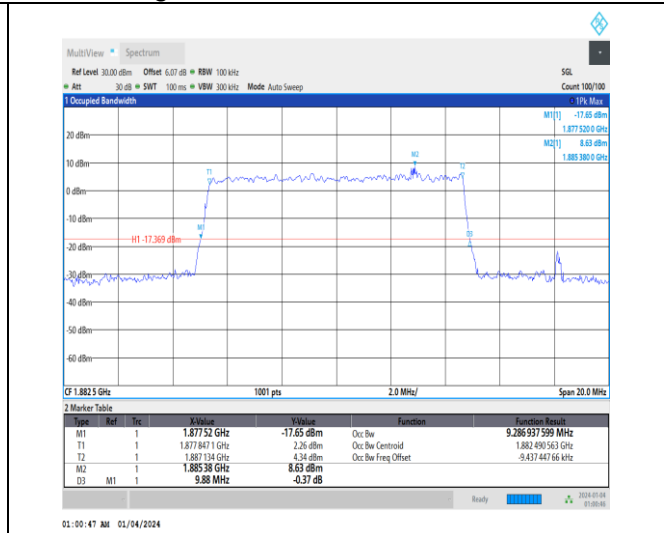
1-N25-15-10-M-9-CP-256QAM-Outer_Full-52@0-Ant 1-9.287-9.880-≤10-PASS
