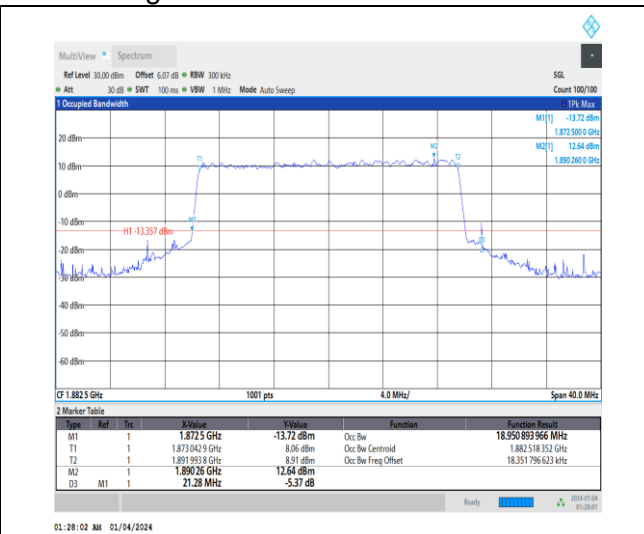
1-N25-15-20-M-7-CP-16QAM-Outer_Full-106@0-Ant 1-18.951-21.280-≤20-PASS
