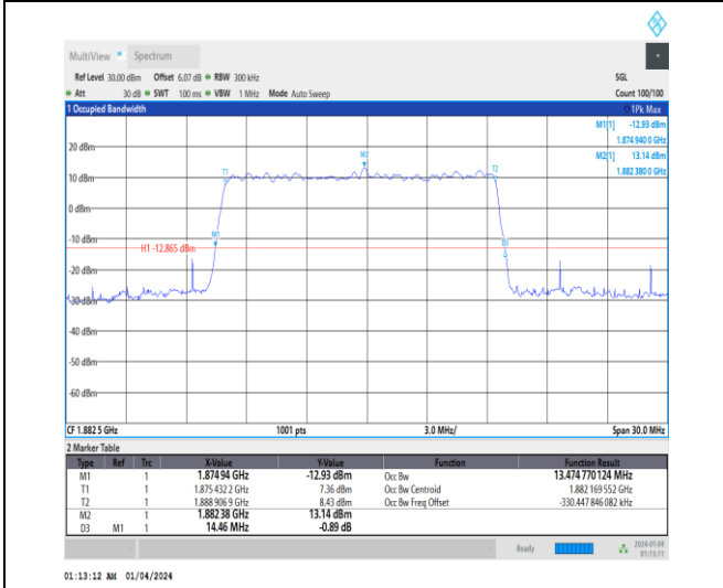
1-N25-15-15-M-5-DFT-256QAM-Outer_Full-75@0-A nt1-13.475-14.460-≤15-PASS
