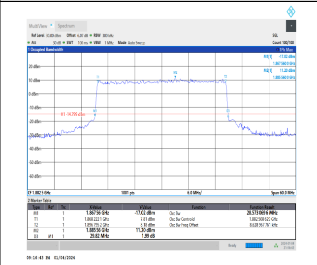
1-N25-15-30-M-7-CP-16QAM-Outer_Full-160@0-Ant1 1-28.573-29.820-≤30-PASS
