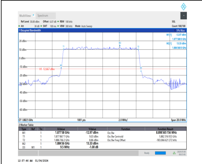
1-N25-15-10-M-2-DFT-PI2BPSK-Outer_Full-50@0-Ant1 -8.899-9.500-≤10-PASS
