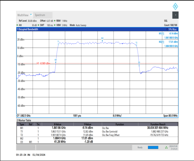
1-N25-15-40-M-2-DFT-PI2BPSK-Outer_Full-216@0-Ant Ant1-38.654-41.280-≤40-PASS
