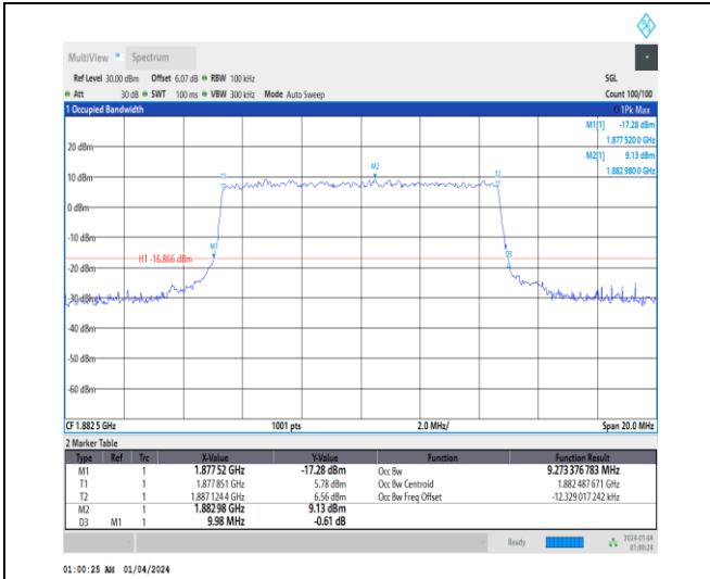
1-N25-15-10-M-8-CP-64QAM-Outer_Full-52@0-Ant1 -9.273-9.980-≤10-PASS
