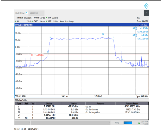
1-N25-15-15-M-7-CP-16QAM-Outer_Full-79@0-Ant1 -14.166-16.530≤15-PASS
