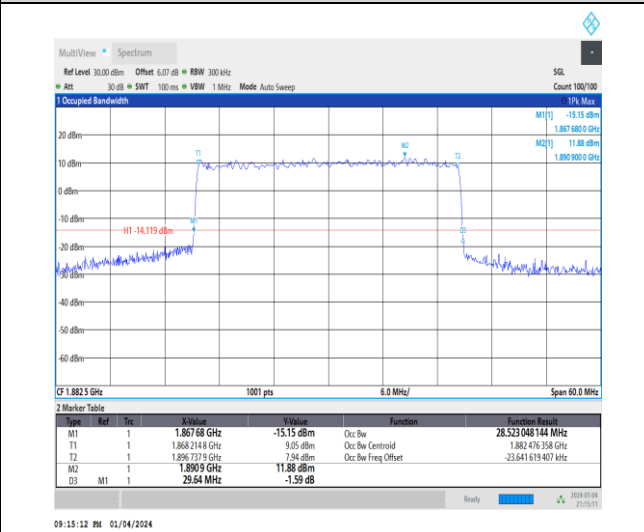
1-N25-15-30-M-3-DFT-16QAM-Outer_Full-160@0-A nt1-28.523-29.640-≤30-PASS
