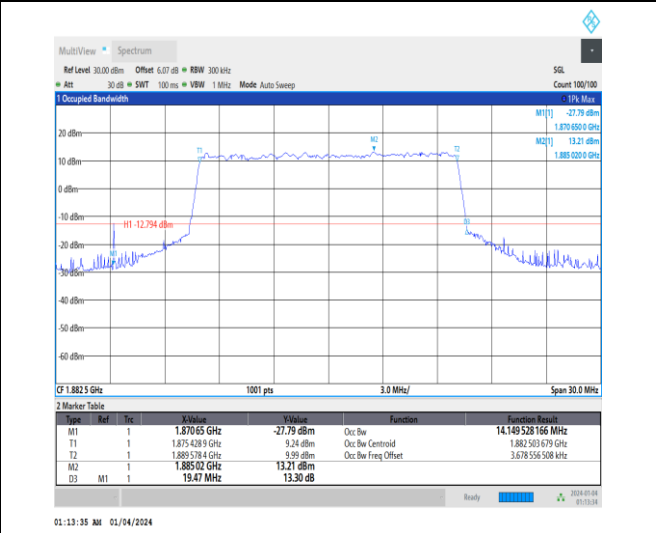
1-N25-15-15-M-6-CP-QPSK-Outer_Full-79@0-Ant1 14.15-19.470-≤15-PASS
