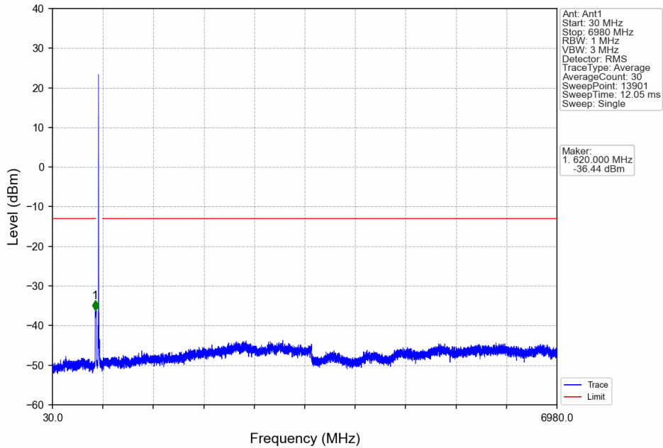
Band71_20MHz_64QAM_LCH_673MHz_RB_1_0_NTNV
